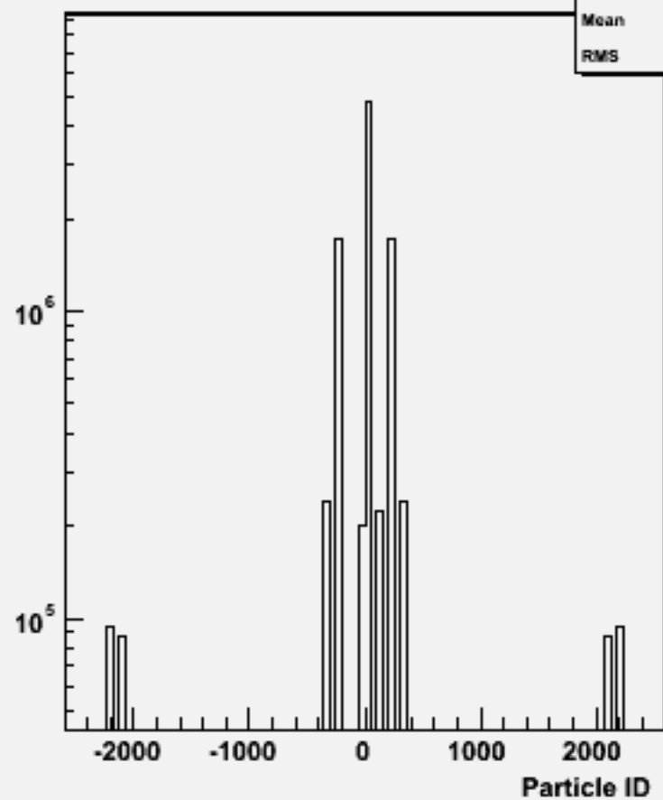
Particle ID : w104741 bbh_o
