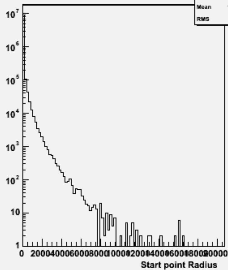
Start point R : w104741 bbh_o
