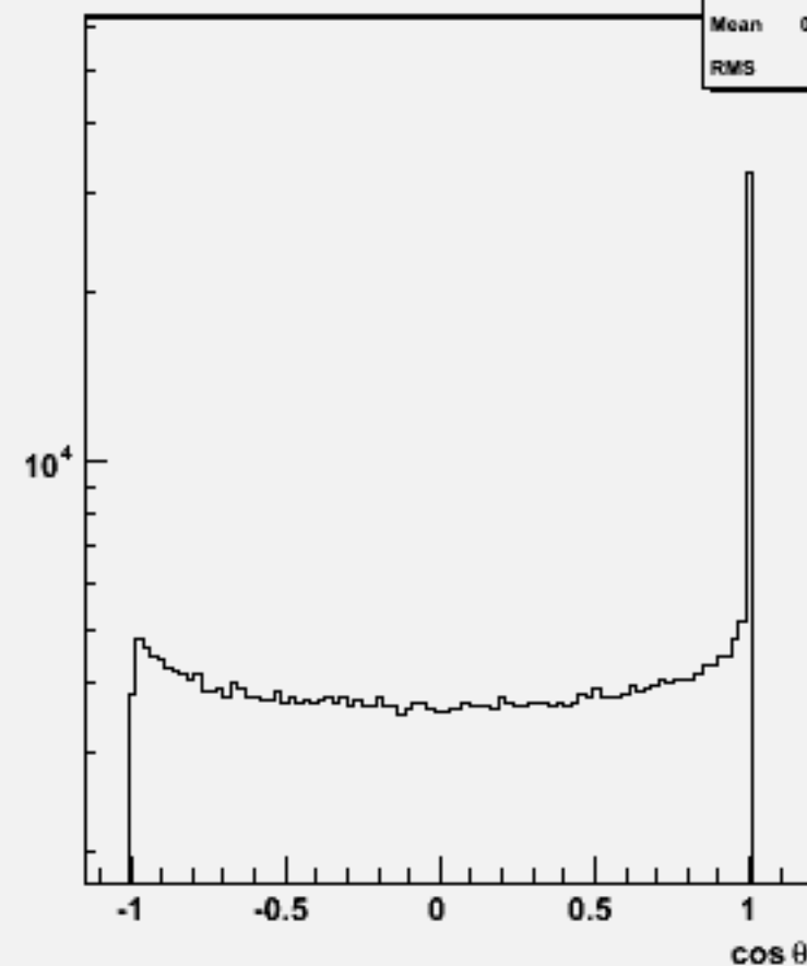
Jet cos \theta (All jets)w104741 bbh_o
