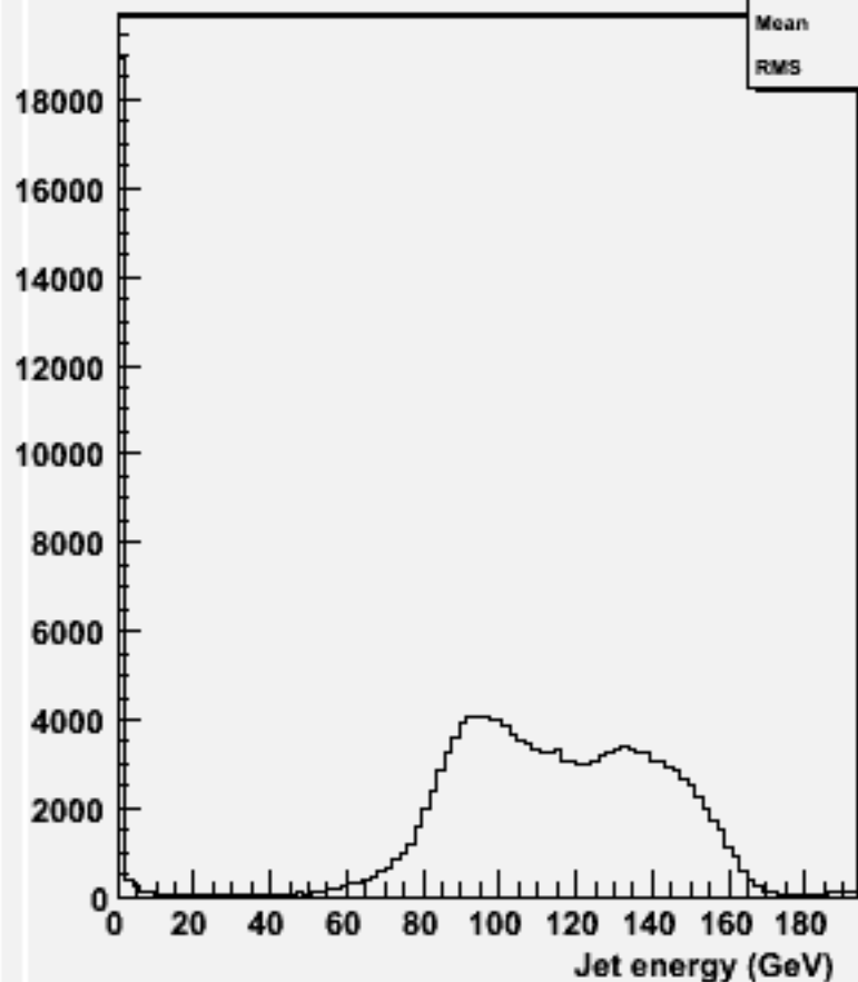
energy for 2-jets :w104741 bbh_o
