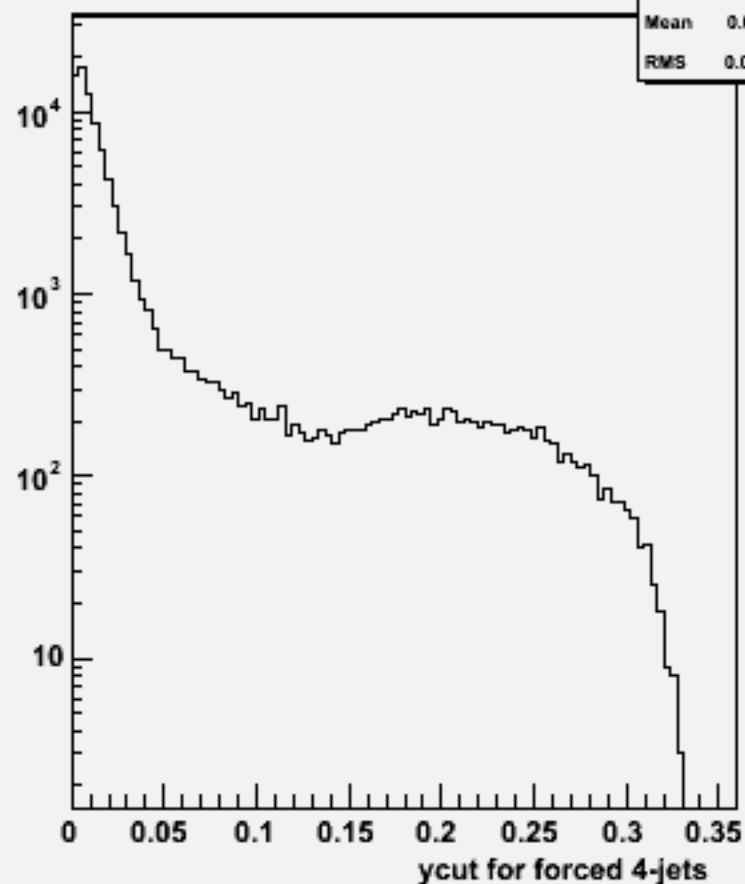
Ycut for 4-jets :w104741 bbh_o
