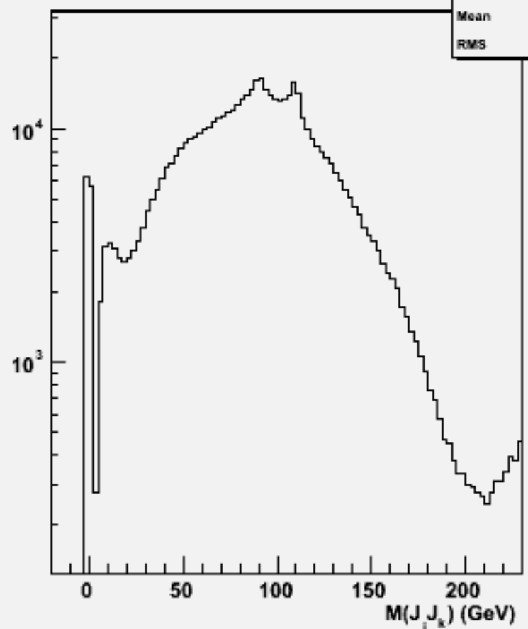
2jets mass(All comb)w104741 bbh_o
