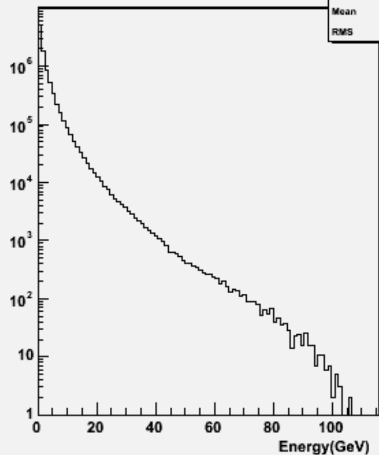
Particle Energy : w104741 bbh_o
