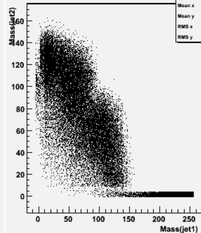
Jet mass for forced 2-jets : w104741 bbh_o
