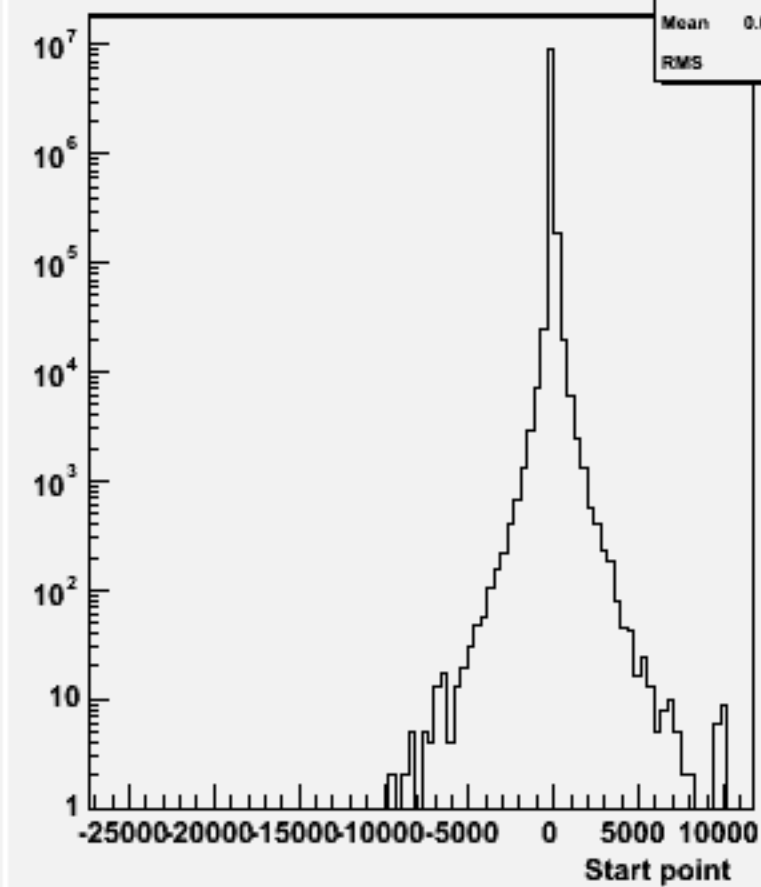
Start point Z : w104741 bbh_o
