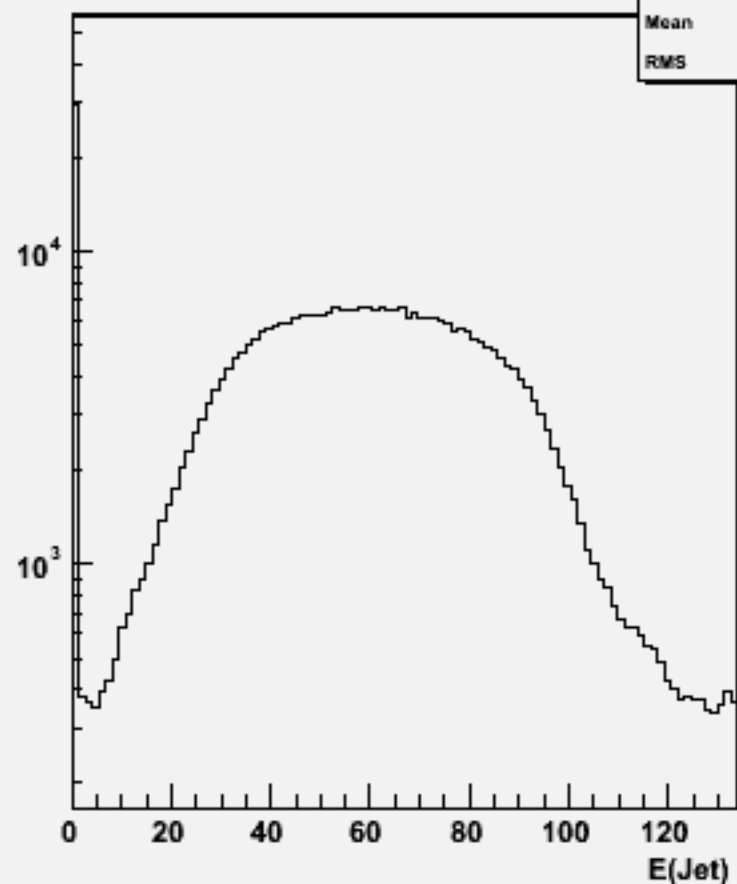
Jet energies(All jets)w104741 bbh_o
