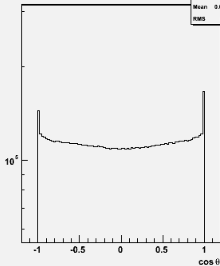
Particle cosθ : w104741 bbh_o
