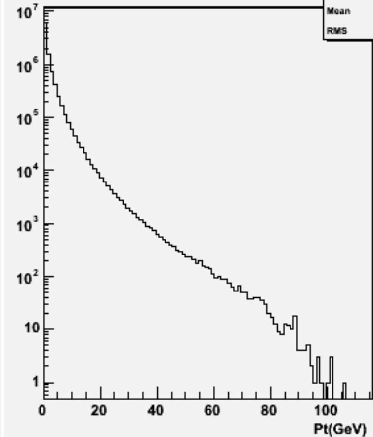
Particle Pt : w104741 bbh_o
