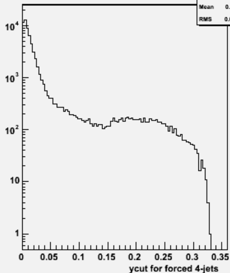
Ycut for 4-jets :w104738 ssh_o
