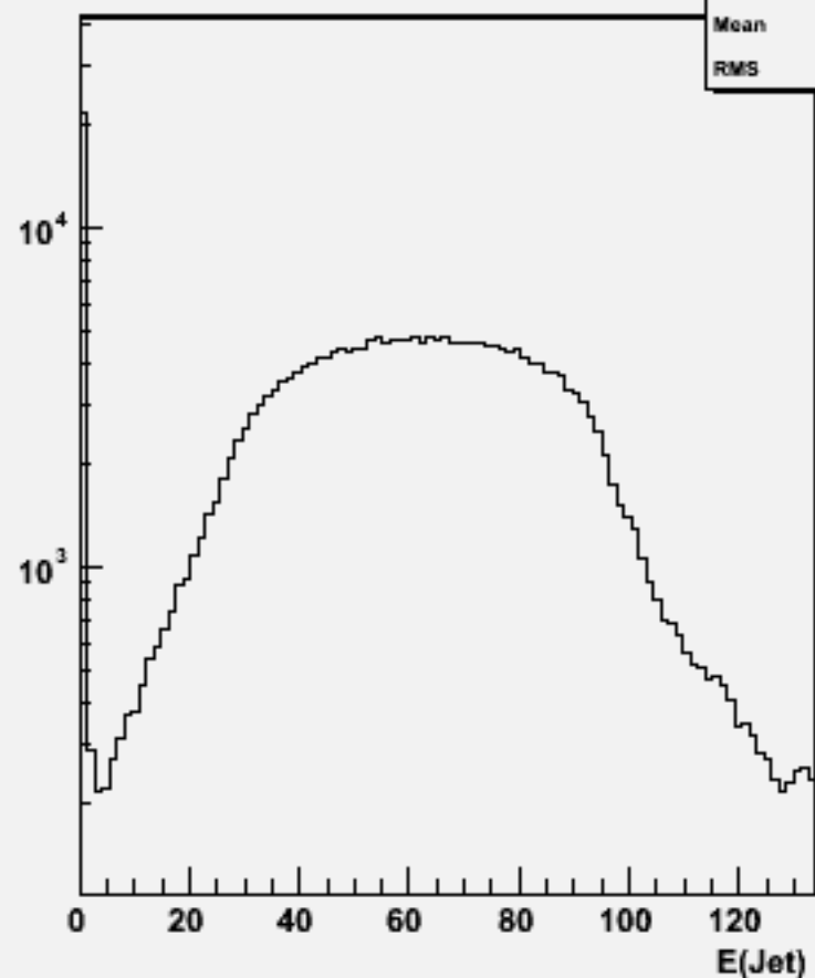
Jet energies(All jets)w104738 ssh_o
