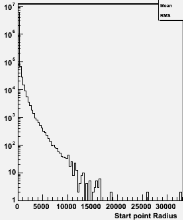
Start point R : w104738 ssh_o
