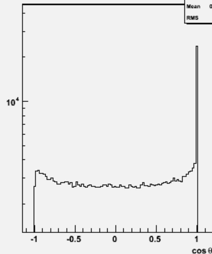
Jet cosθ (All jets)w104738 ssh_o
