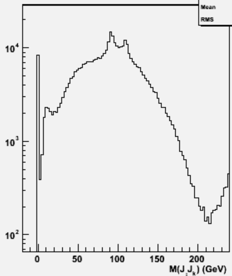
2jets mass(All comb)w104738 ssh_o
