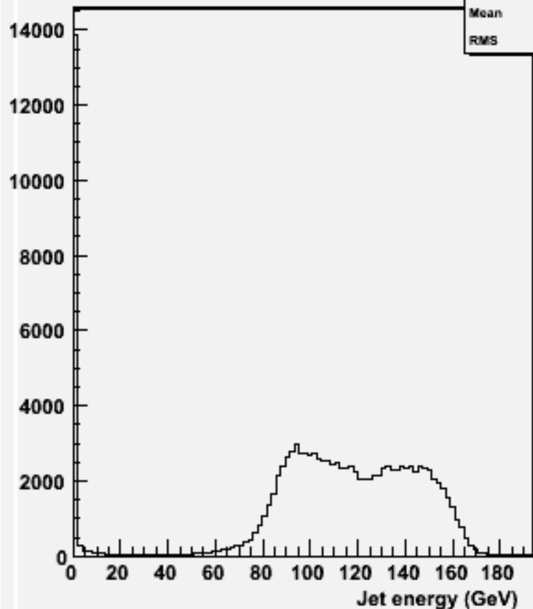
energy for 2-jets :w104738 ssh_o
