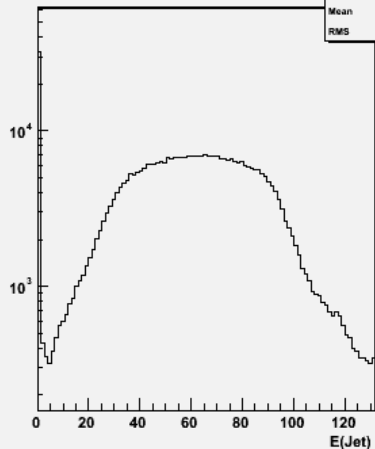
Jet energies(All jets)w104737 ssh_o
