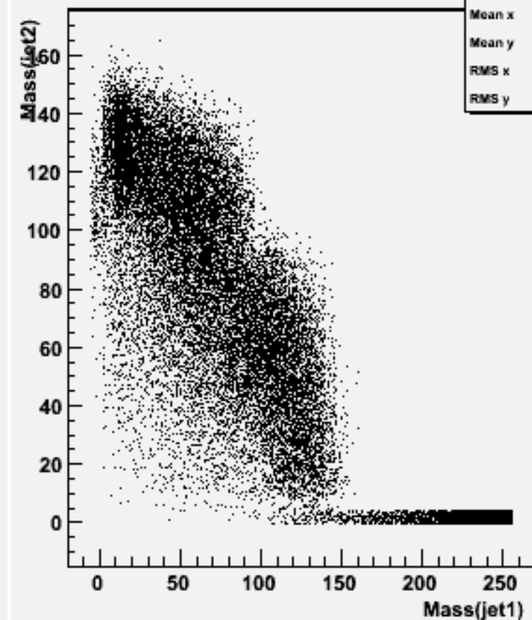
Jet mass for forced 2-jets : w104737 ssh_o
