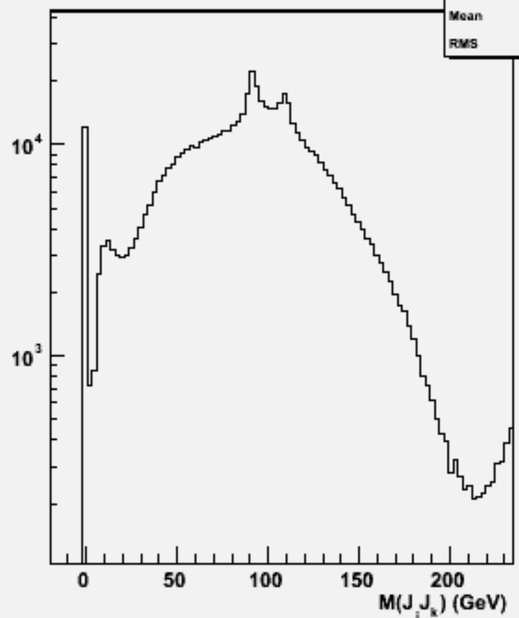
2jets mass(All comb)w104737 ssh_o
