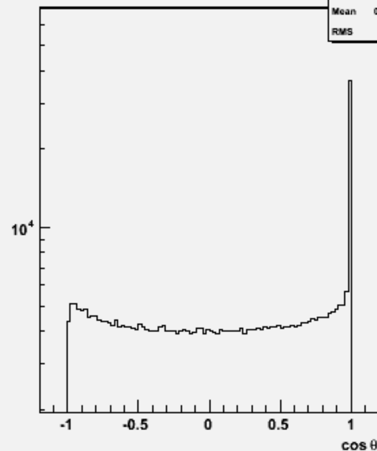
Jet cos \theta (All jets)w104737 ssh_o
