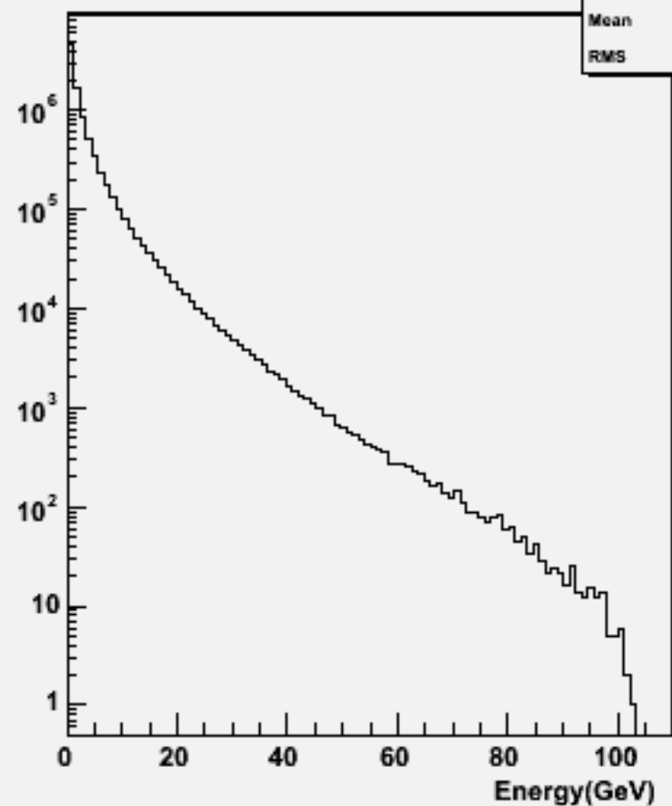
Start point R : w104737 ssh_o
