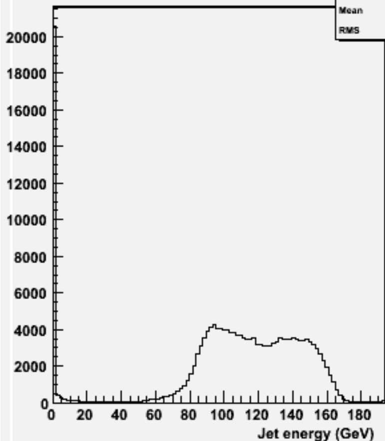
energy for 2-jets :w104737 ssh_o
