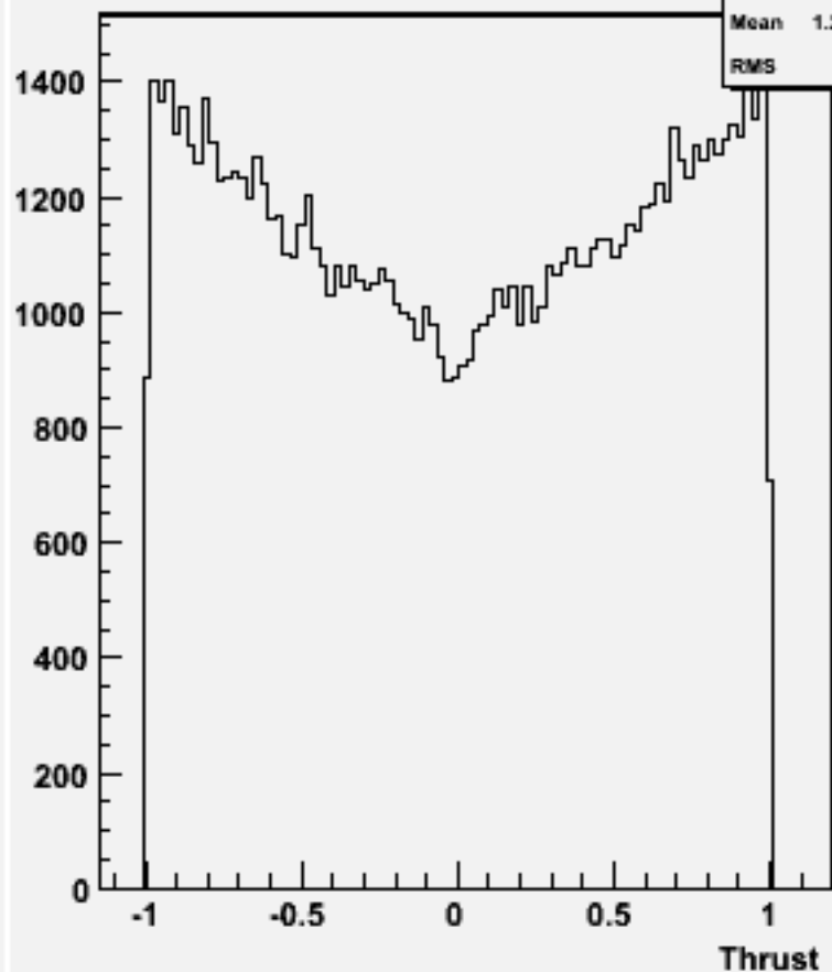
energy for 2-jets :w104737 ssh_o
