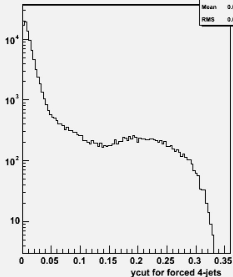
Ycut for 4-jets :w104737 ssh_o
