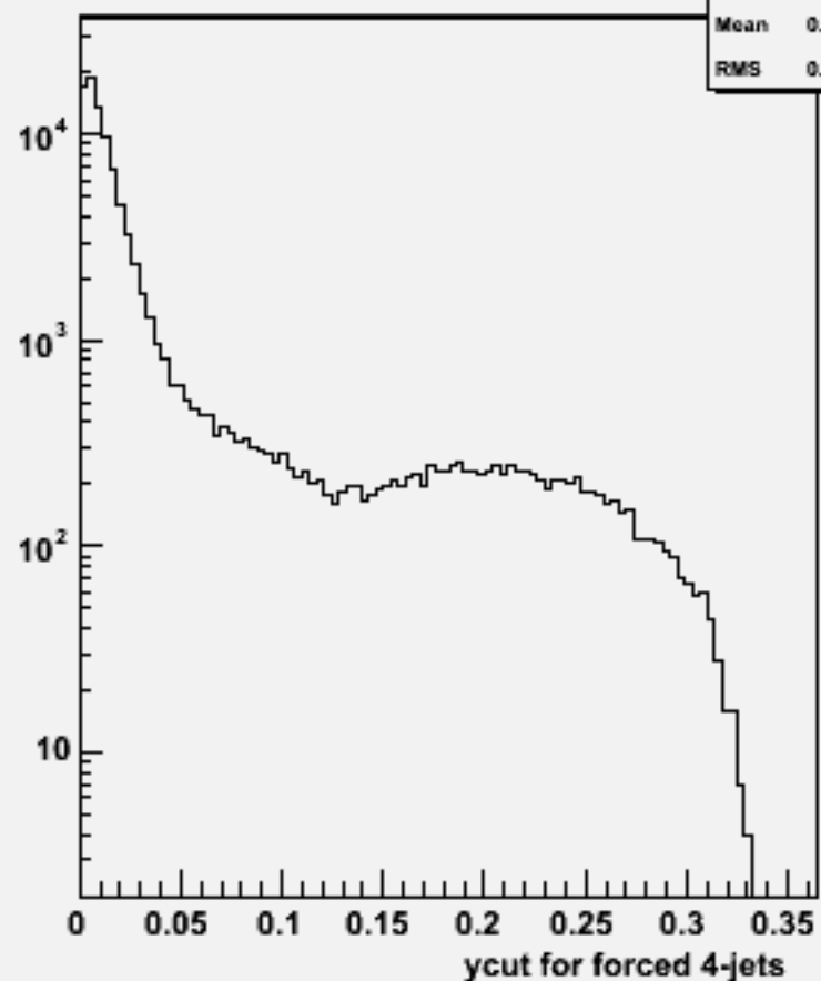
Ycut for 4-jets :w104733 ddh_o
