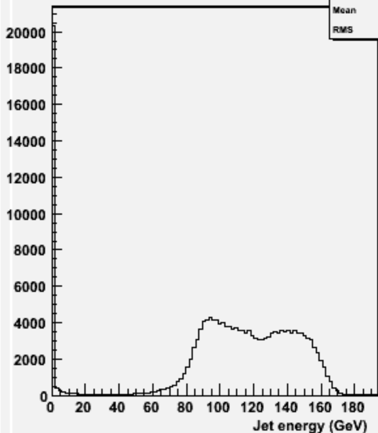
energy for 2-jets :w104733 ddh_o
