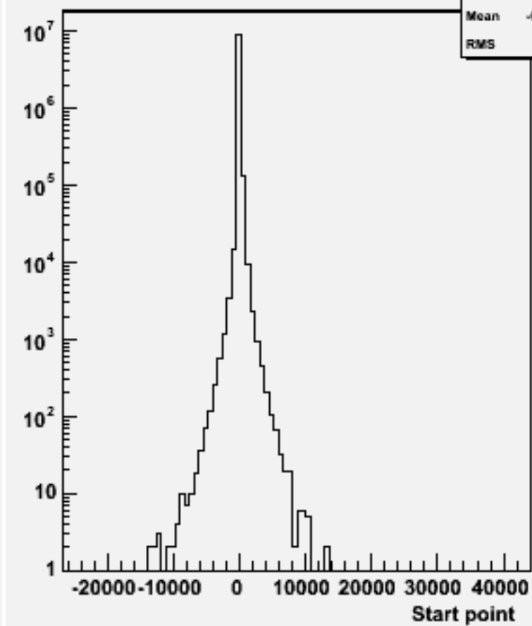
Start point Z : w104733 ddh_o
