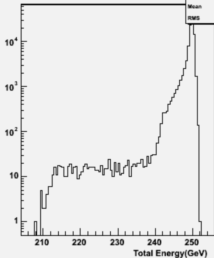
Total Energy (inc. \nu ): w104733 ddh_o
