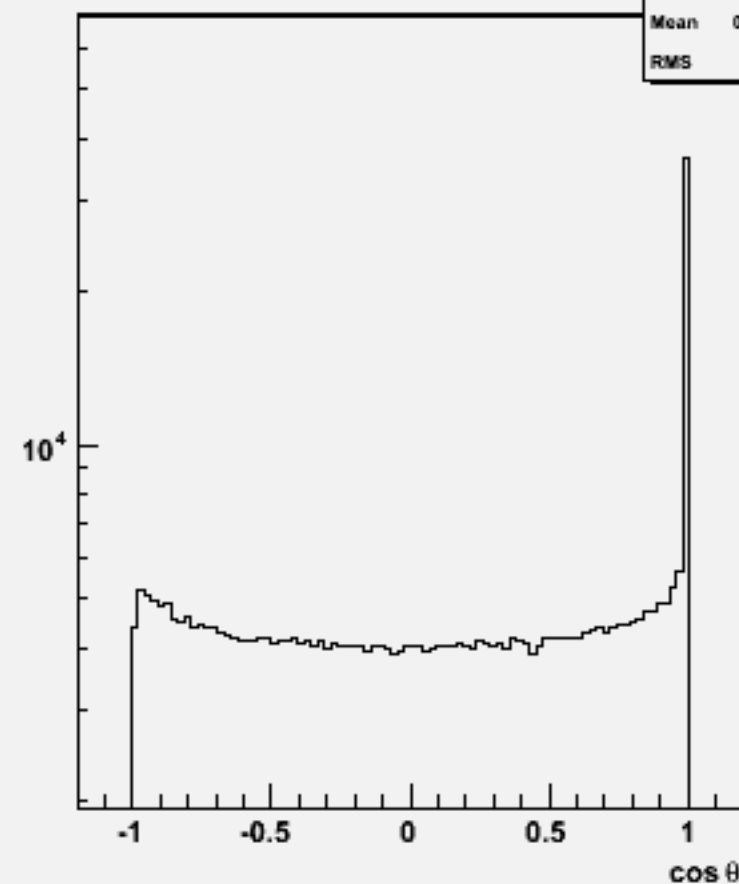
Jet cos \theta (All jets)w104733 ddh_o
