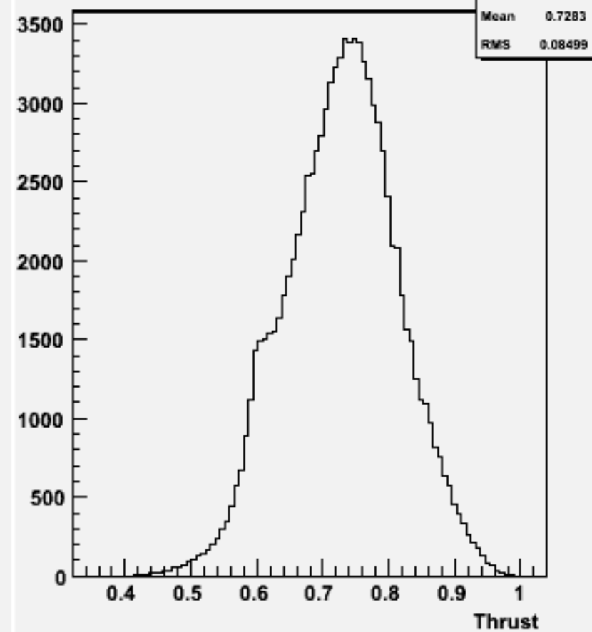
Thrust w104733 ddh_o
