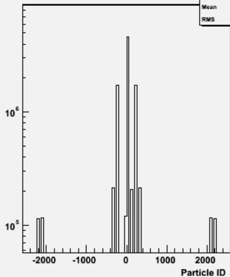
Particle ID : w104733 ddh_o
