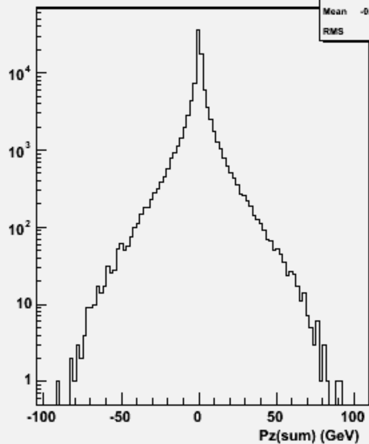
Pz Sum: w104733 ddh_o
