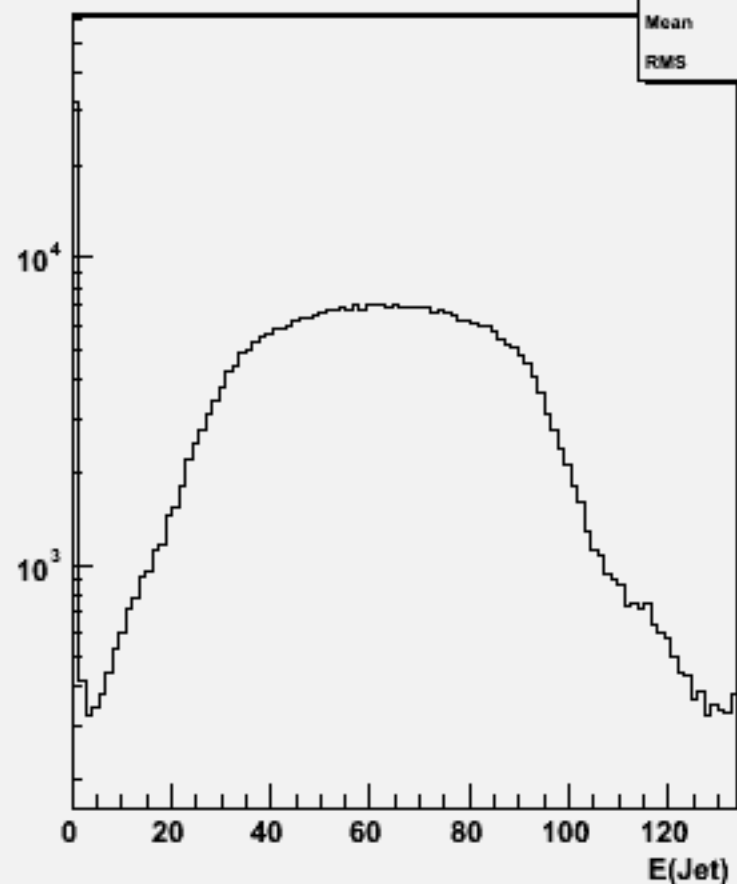
Jet energies(All jets)w104733 ddh_o
