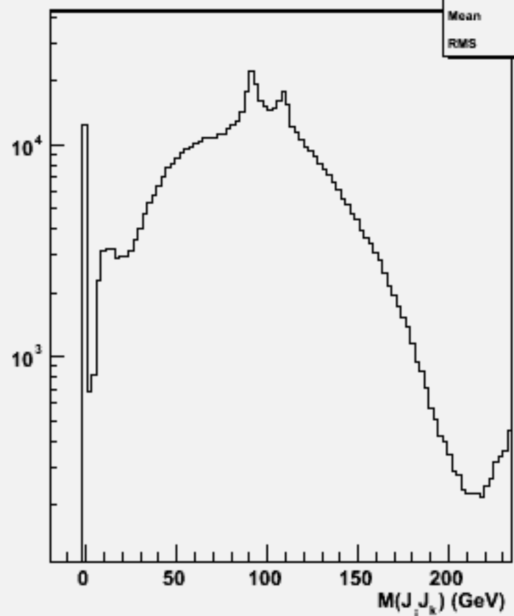
2jets mass(All comb)w104733 ddh_o
