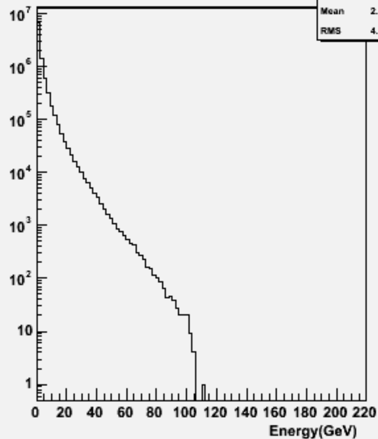
Particle Energy : w104733 ddh_o
