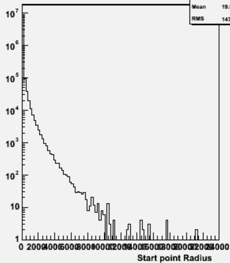
Start point R : w104733 ddh_o
