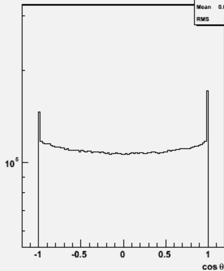
Particle cosθ : w104733 ddh_o
