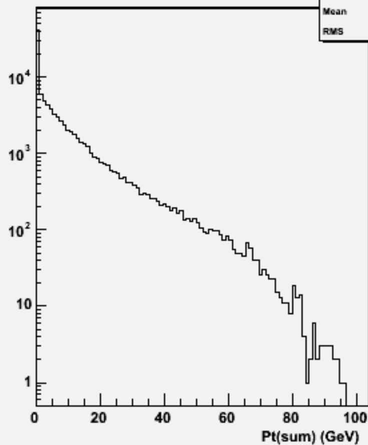
Pt Sum: w104733 ddh_o
