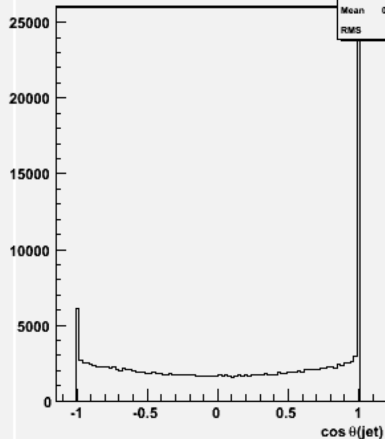
cos \theta for 2-jets :w104733 ddh_o
