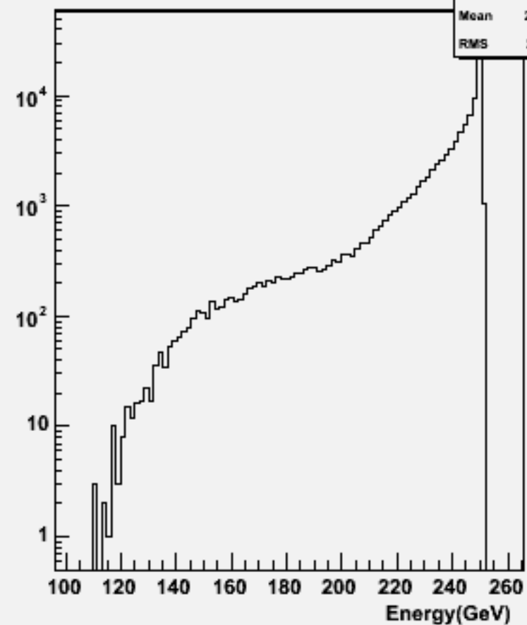
Total Energy (w/o \nu ): w104733 ddh_o
