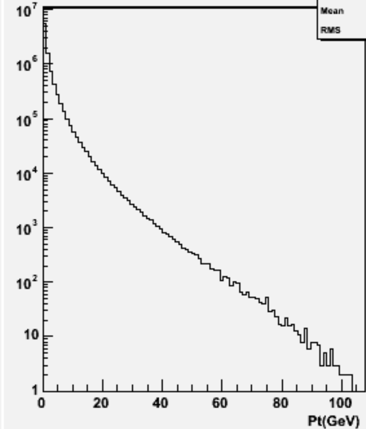
Particle Pt : w104733 ddh_o
