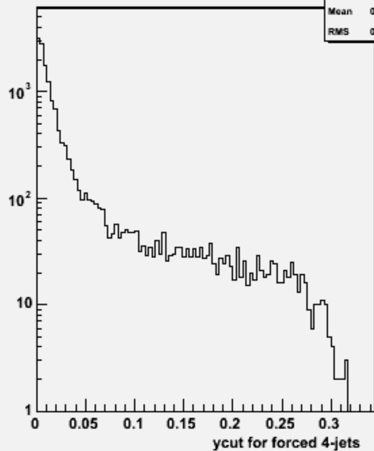
Ycut for 4-jets :w104730 e3e3h_o
