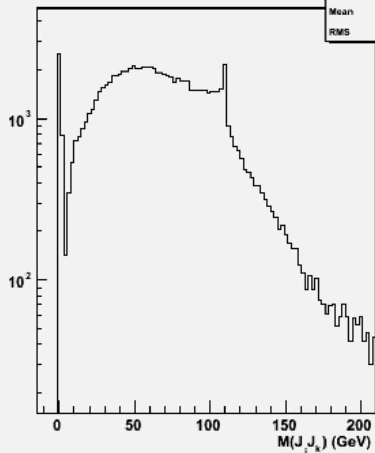
2jets mass(All comb)w104730 e3e3h_o
