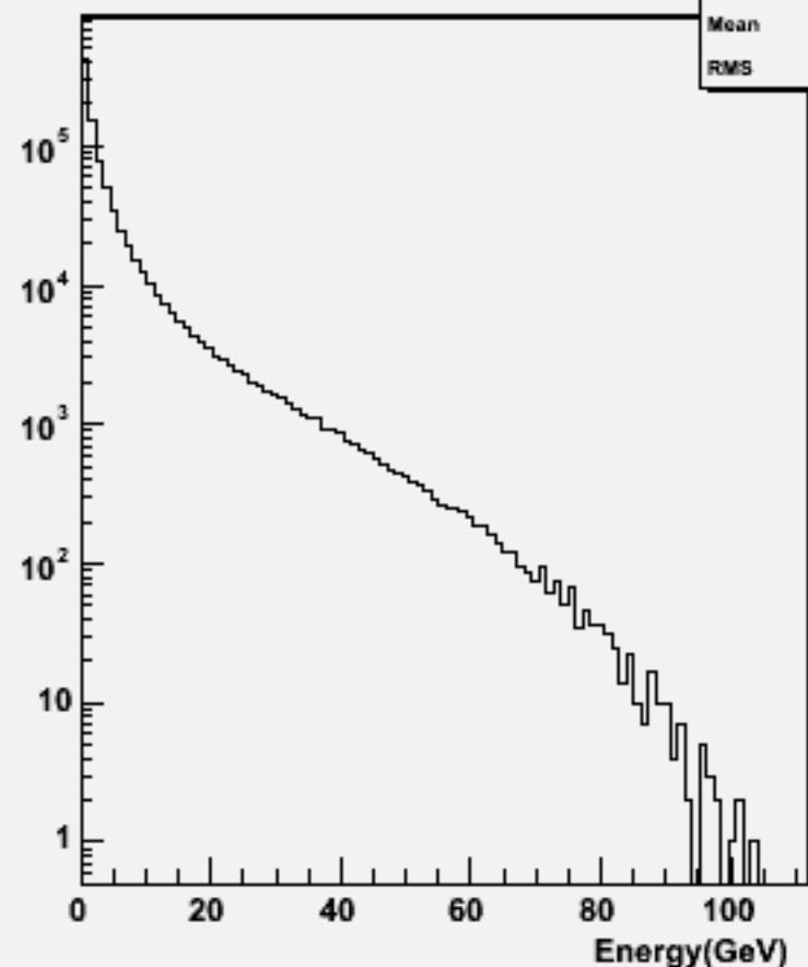
Particle Energy : w104730 e3e3h_o
