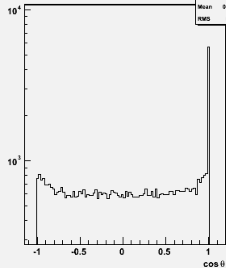
Jet cos \theta (All jets)w104730 e3e3h_o
