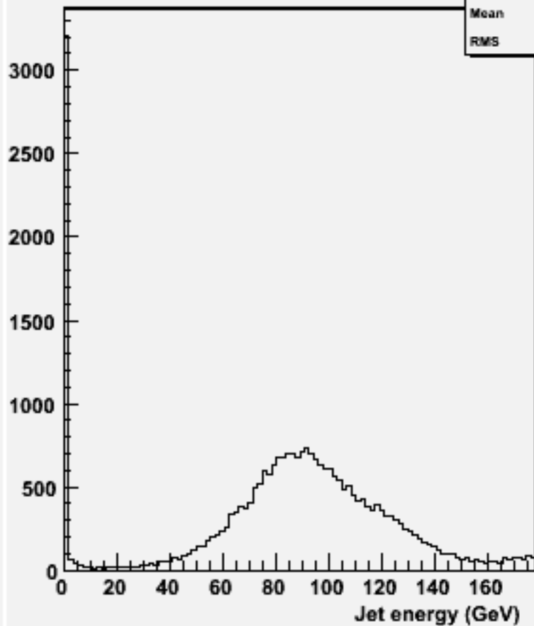
energy for 2-jets :w104730 e3e3h_o
