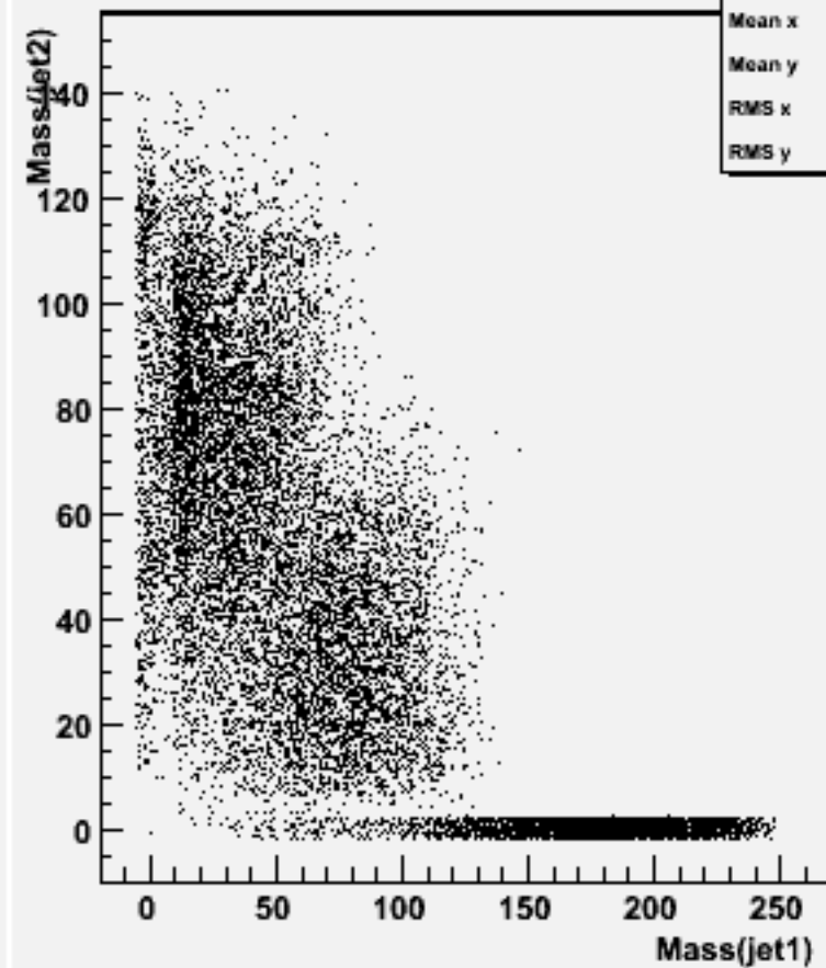
Jet mass for forced 2-jets : w104730 e3e3h_o
