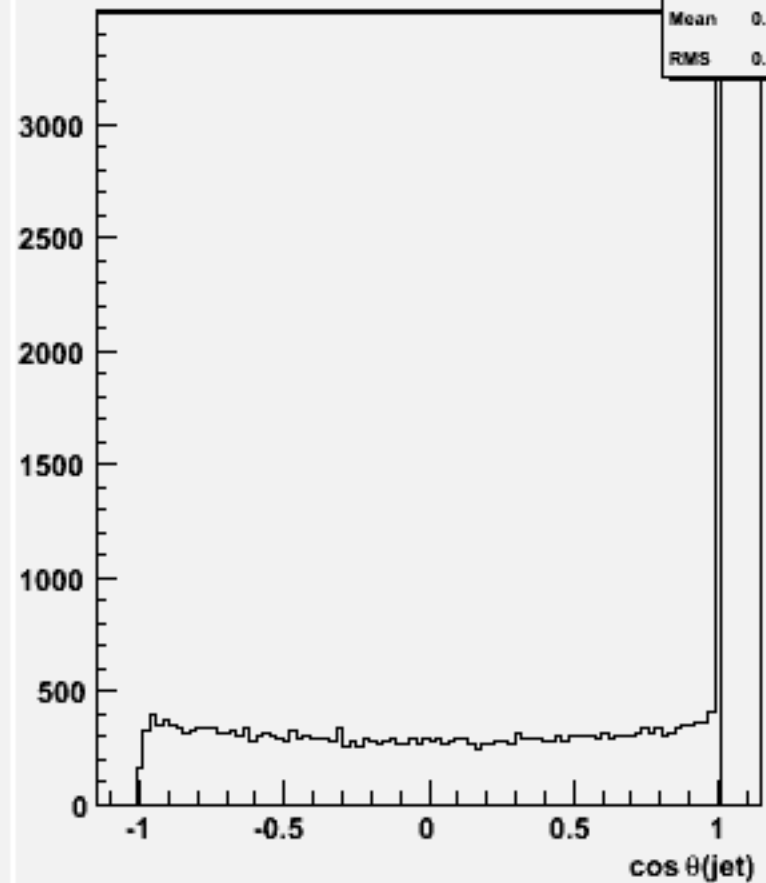
cos \theta for 2-jets :w104730 e3e3h_o
