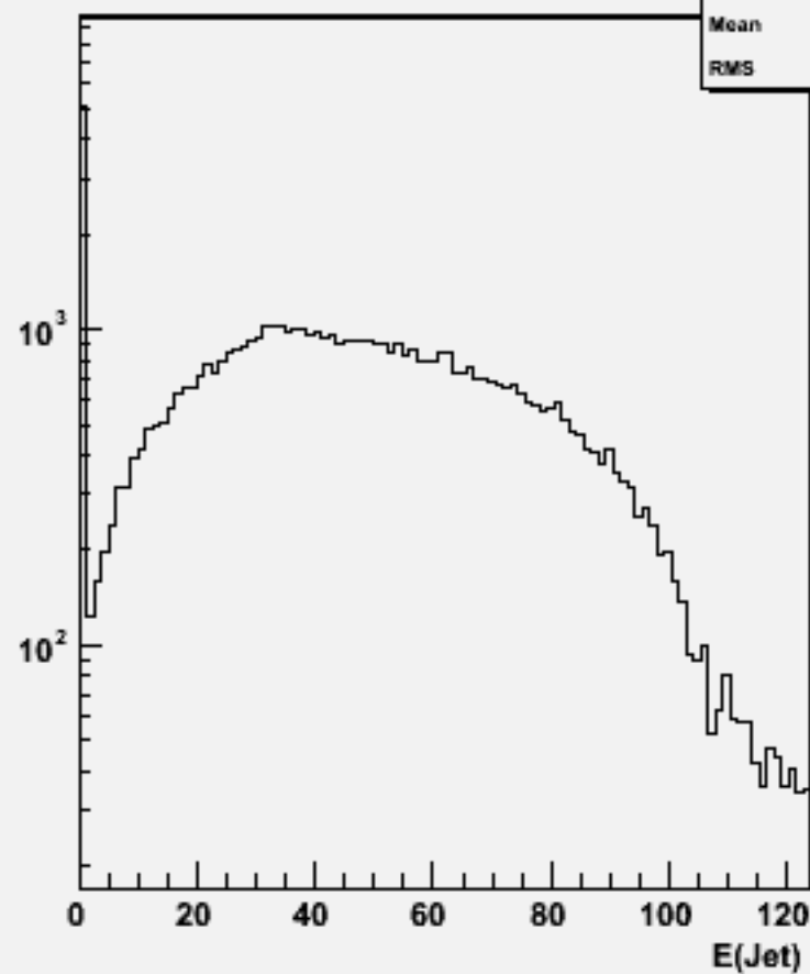
Jet energies(All jets)w104730 e3e3h_o
