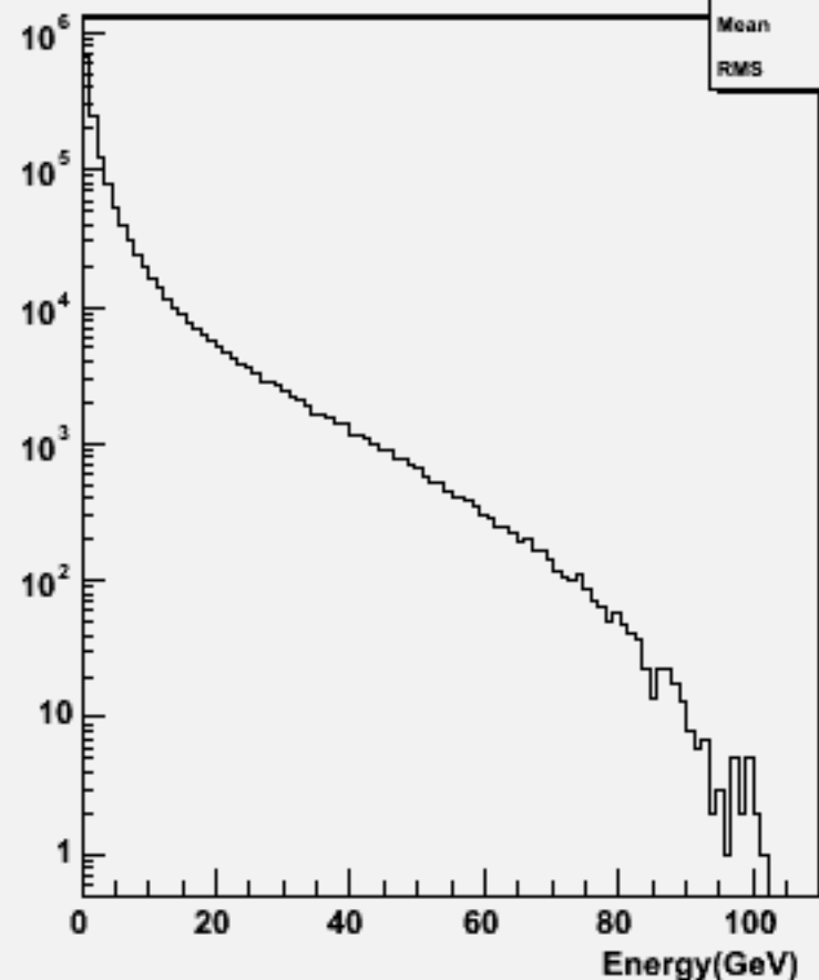
Particle Energy : w104729 e3e3h_o
