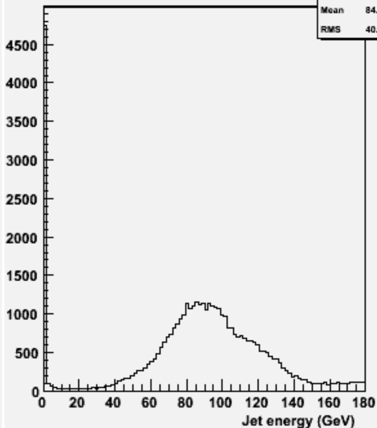
energy for 2-jets :w104729 e3e3h_o
