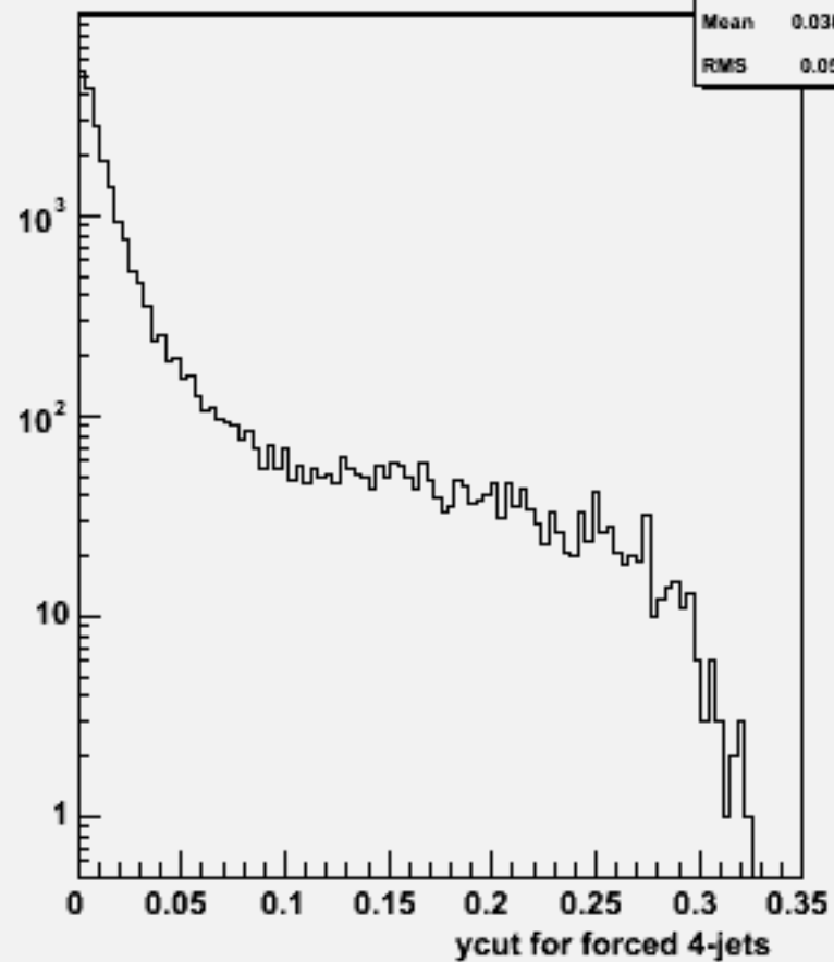
Ycut for 4-jets :w104729 e3e3h_o
