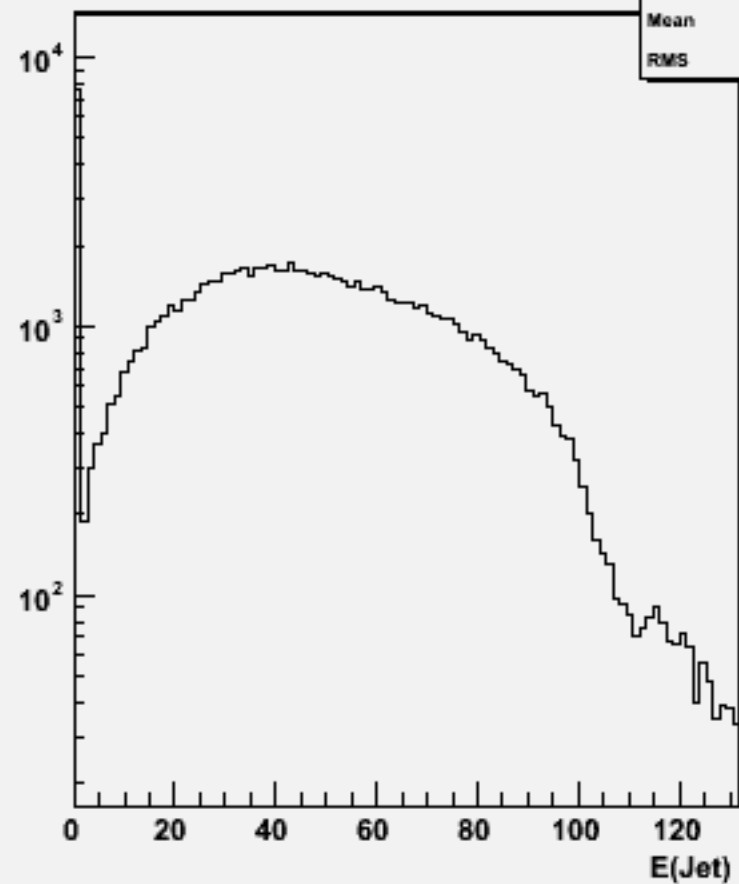
Jet energies(All jets)w104729 e3e3h_o
