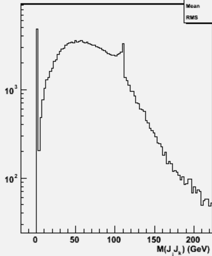
2jets mass(All comb)w104729 e3e3h_o
