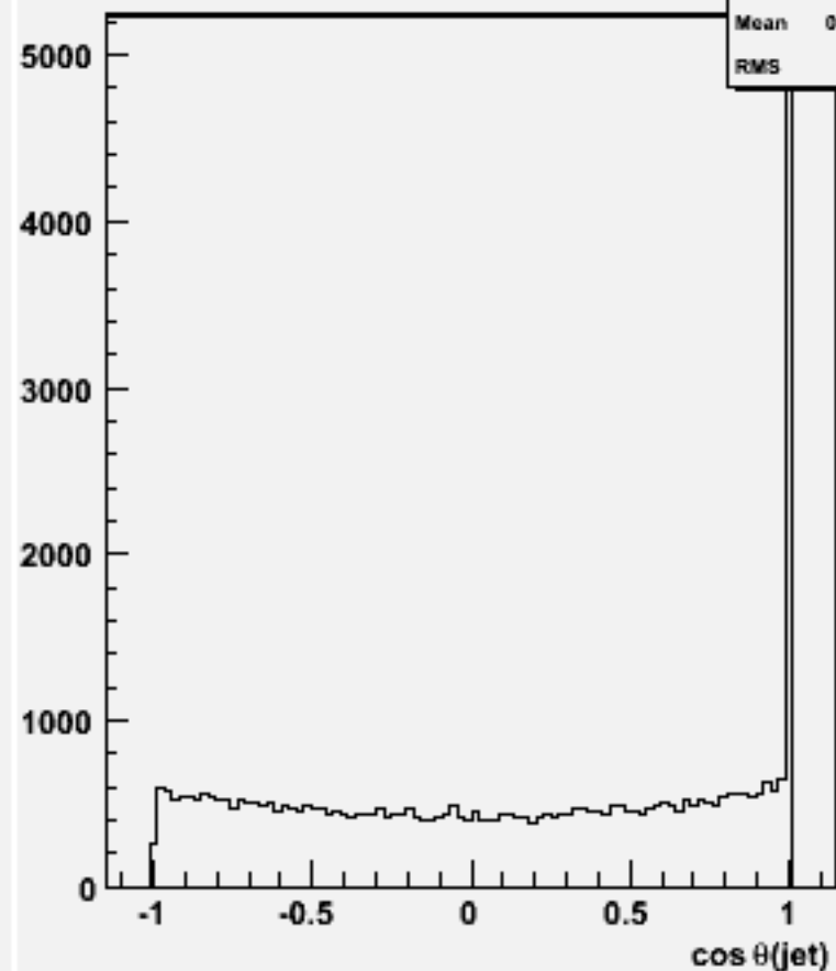
cos \theta for 2-jets :w104729 e3e3h_o
