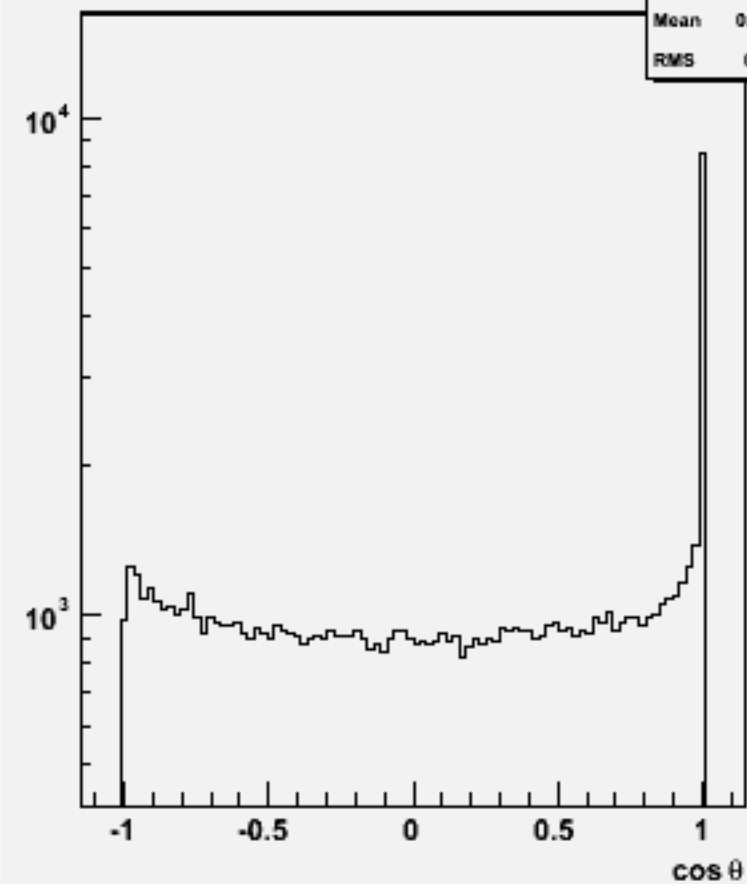
Jet cos \theta (All jets)w104729 e3e3h_o
