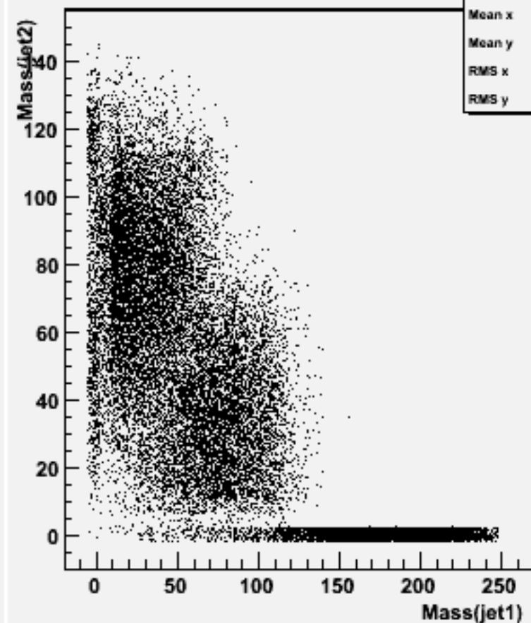
Jet mass for forced 2-jets : w104729 e3e3h_o
