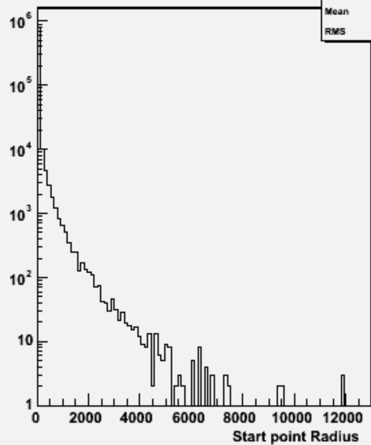
Start point R : w104726 e2e2h_o
