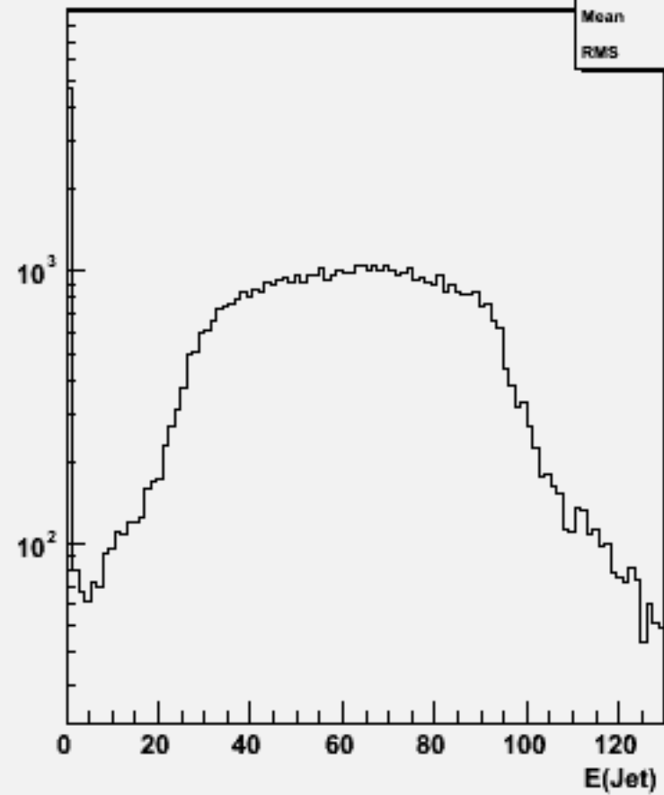
Jet energies(All jets)w104726 e2e2h_o
