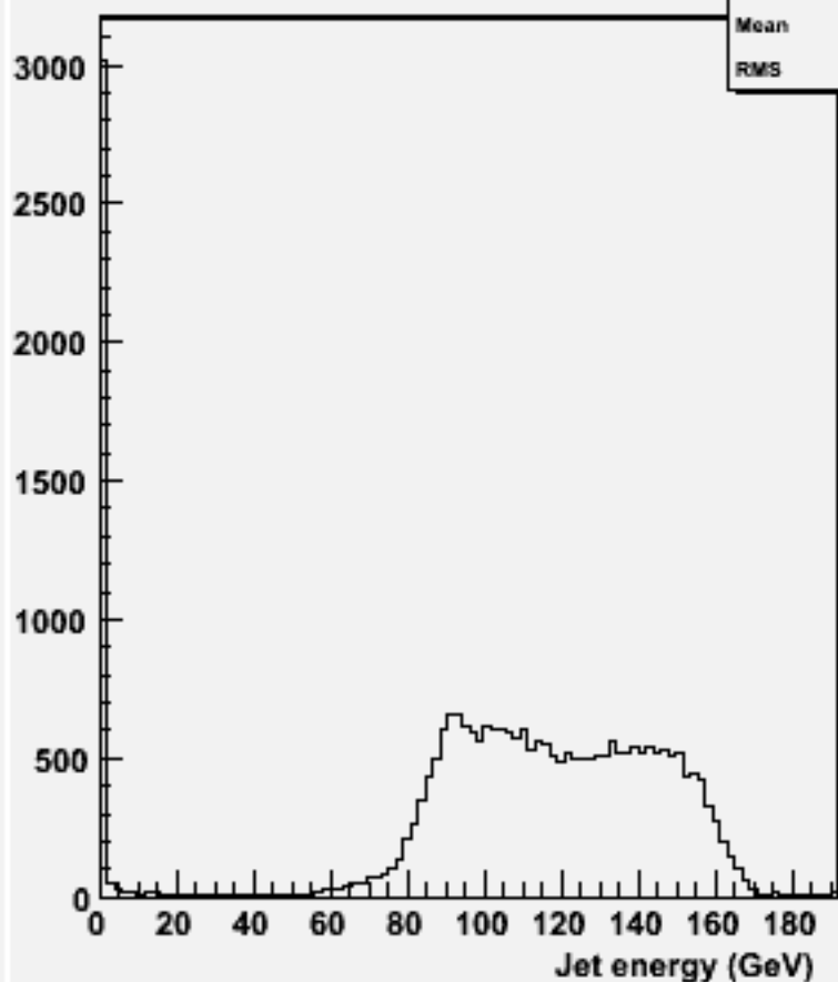
energy for 2-jets :w104726 e2e2h_o
