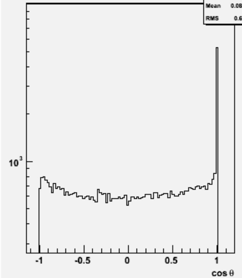
Jet cos \theta (All jets)w104726 e2e2h_o
