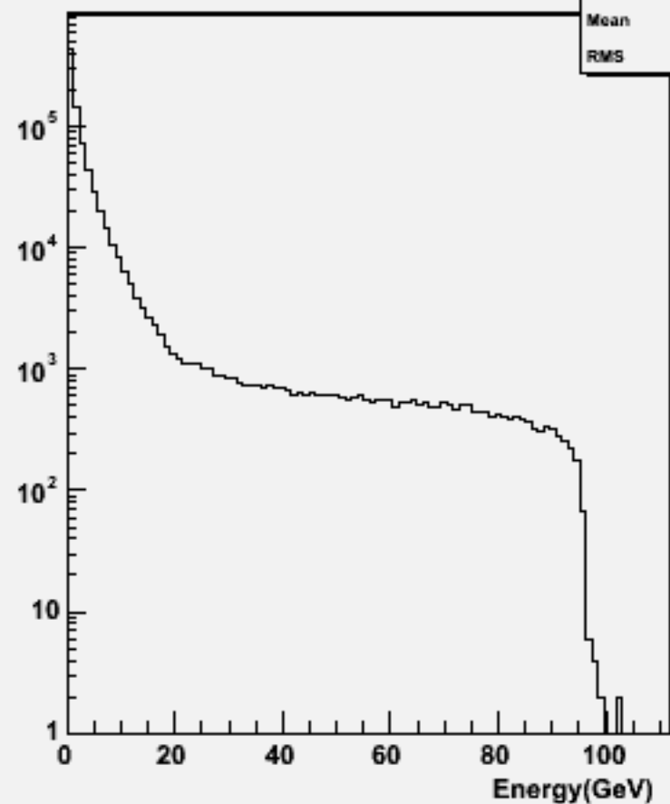
Particle Energy : w104726 e2e2h_o
