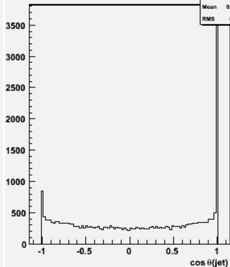
cos \theta for 2-jets :w104726 e2e2h_o
