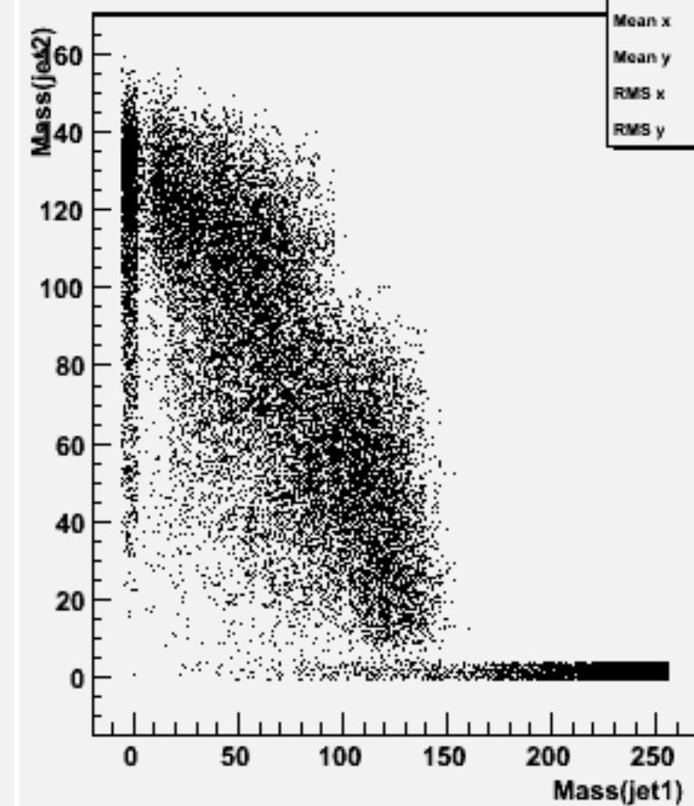
Jet mass for forced 2-jets : w104725 e2e2h_o
