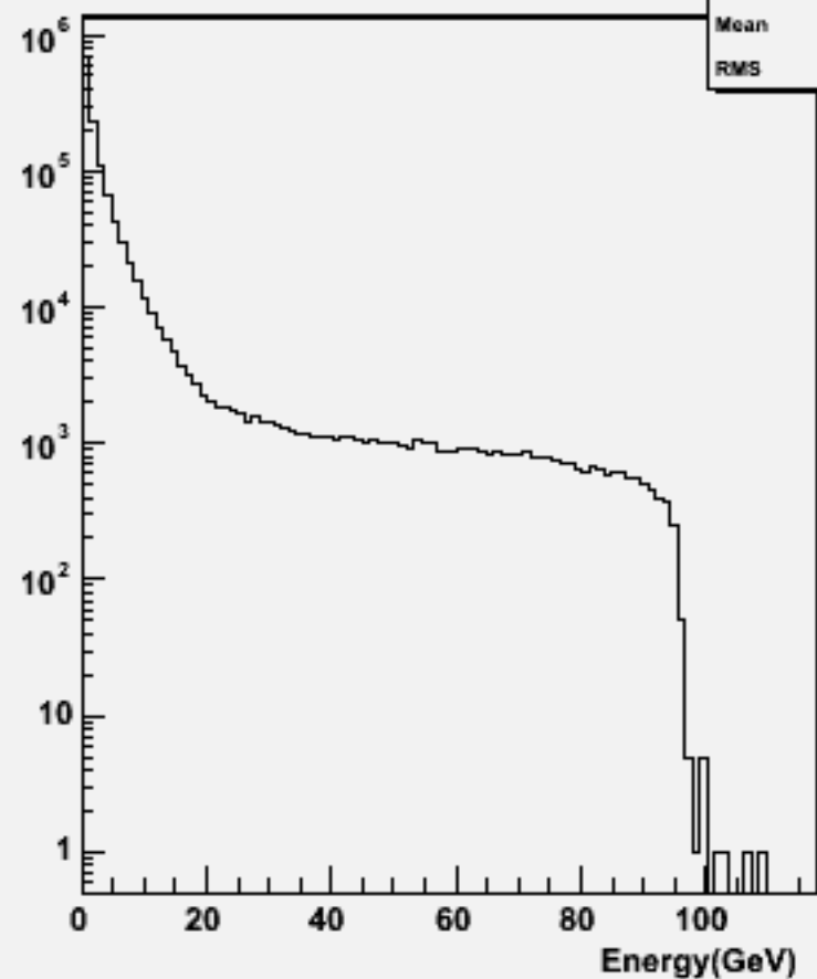
Particle Energy : w104725 e2e2h_o
