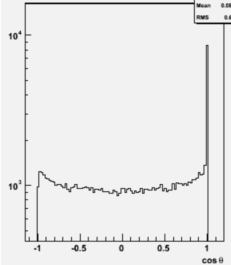
Jet cos \theta (All jets)w104725 e2e2h_o
