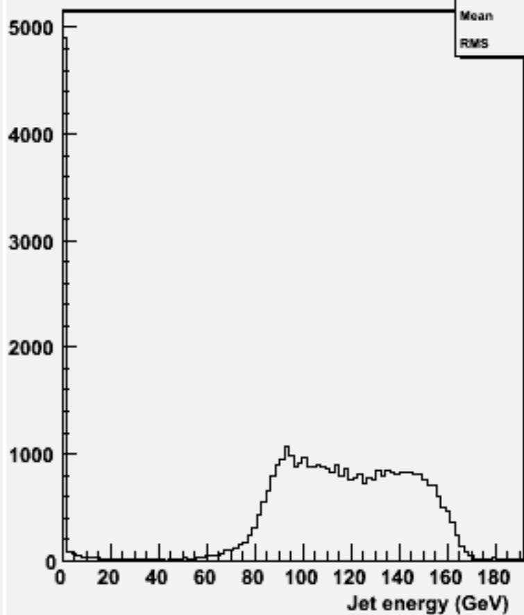
energy for 2-jets :w104725 e2e2h_o
