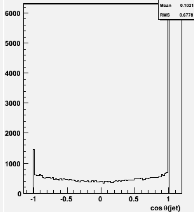
cos \theta for 2-jets :w104725 e2e2h_o
