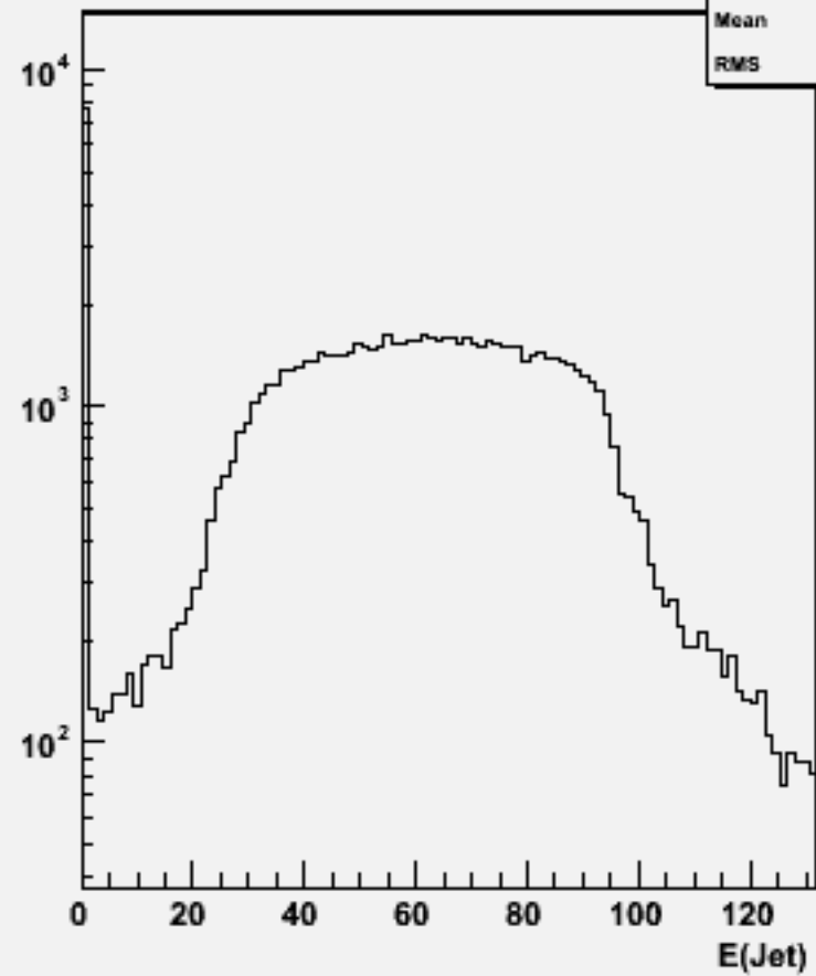
Jet energies(All jets)w104725 e2e2h_o
