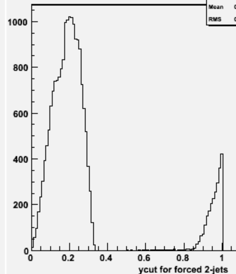
Ycut for 2-jets :w104725 e2e2h_o
