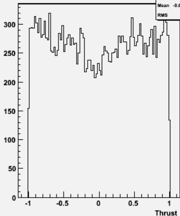
cos \Theta (thrust) w104725 e2e2h_o
