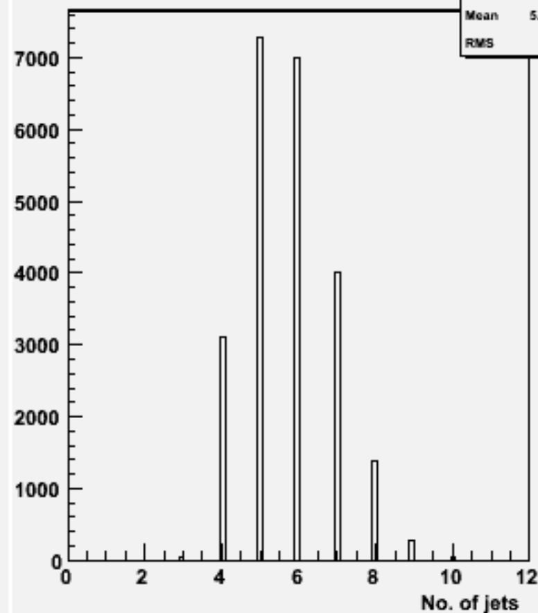
No. jets (ycut=0.001) : w104725 e2e2h_o
