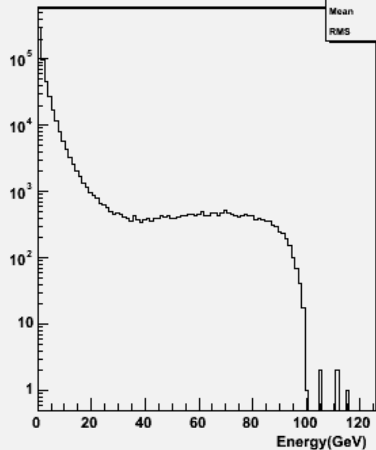
Particle Energy : w104723 e1e1h_o
