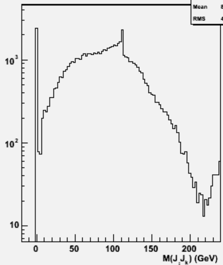
2jets mass(All comb)w104723 e1e1h_o
