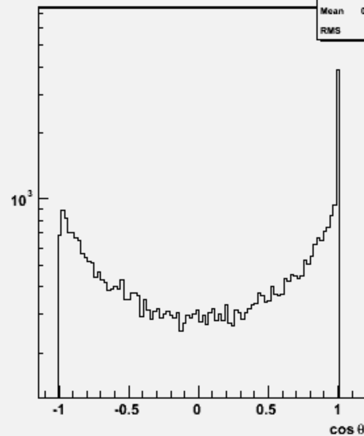
Jet cos \theta (All jets)w104723 e1e1h_o
