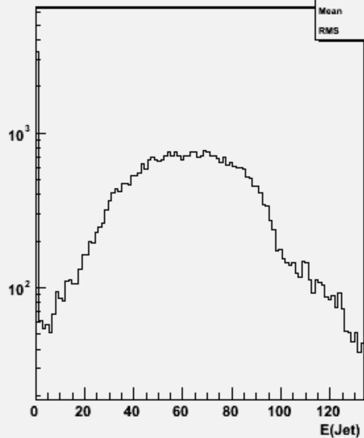
Jet energies(All jets)w104723 e1e1h_o
