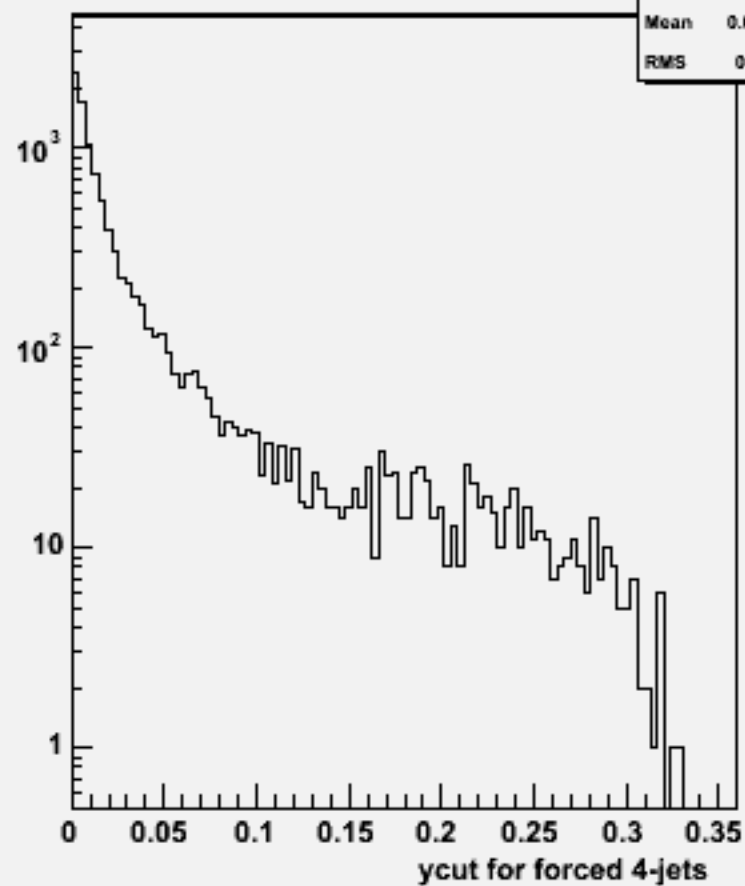
Ycut for 4-jets :w104723 e1e1h_o
