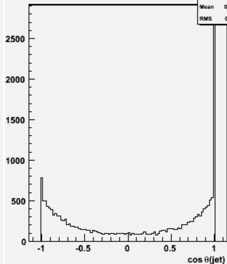
cos \theta for 2-jets :w104723 e1e1h_o
