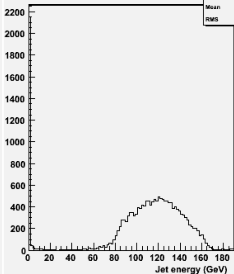
energy for 2-jets :w104723 e1e1h_o
