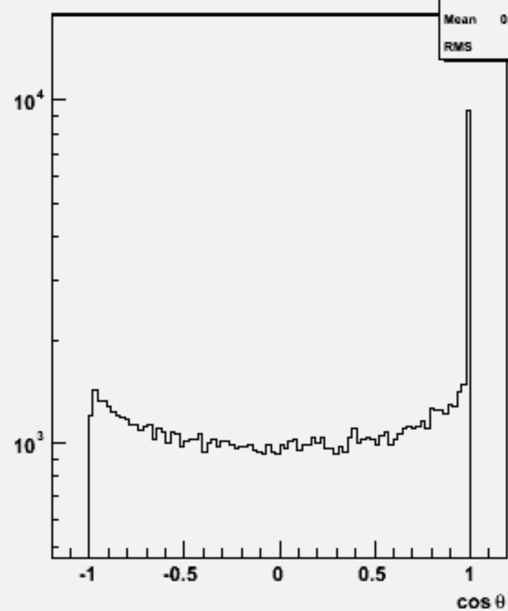
Jet cosθ (All jets)w104721 e1e1h_o
