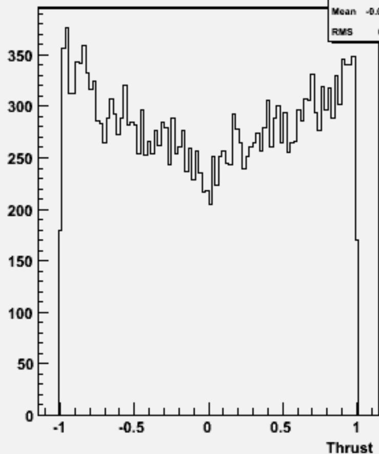
cos \Theta (thrust) w104721 e1e1h_o
