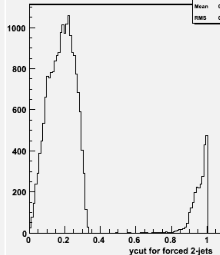
Ycut for 2-jets :w104721 e1e1h_o
