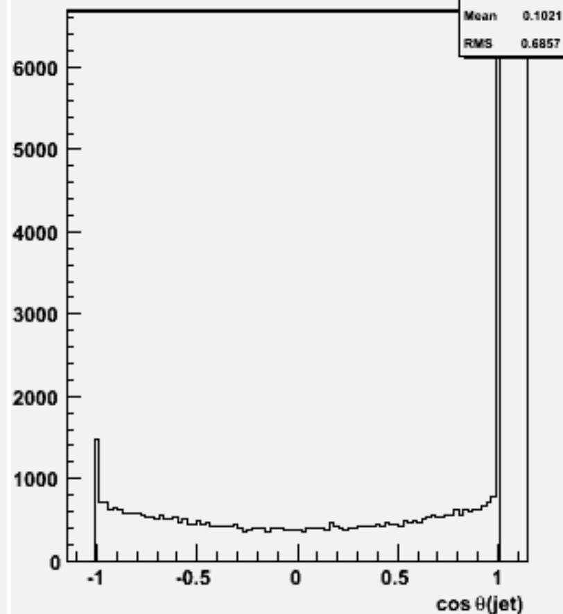
cos \theta for 2-jets :w104721 e1e1h_o
