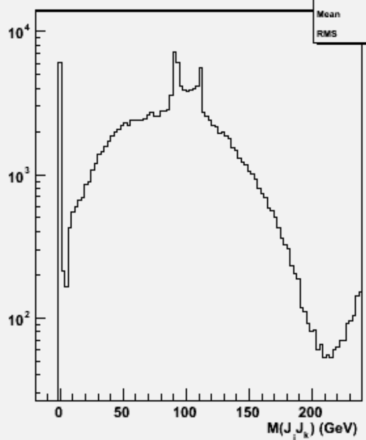
2jets mass(All comb)w104721 e1e1h_o
