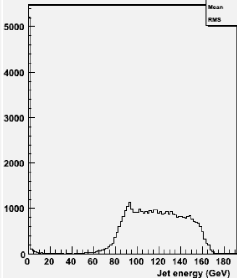
energy for 2-jets :w104721 e1e1h_o
