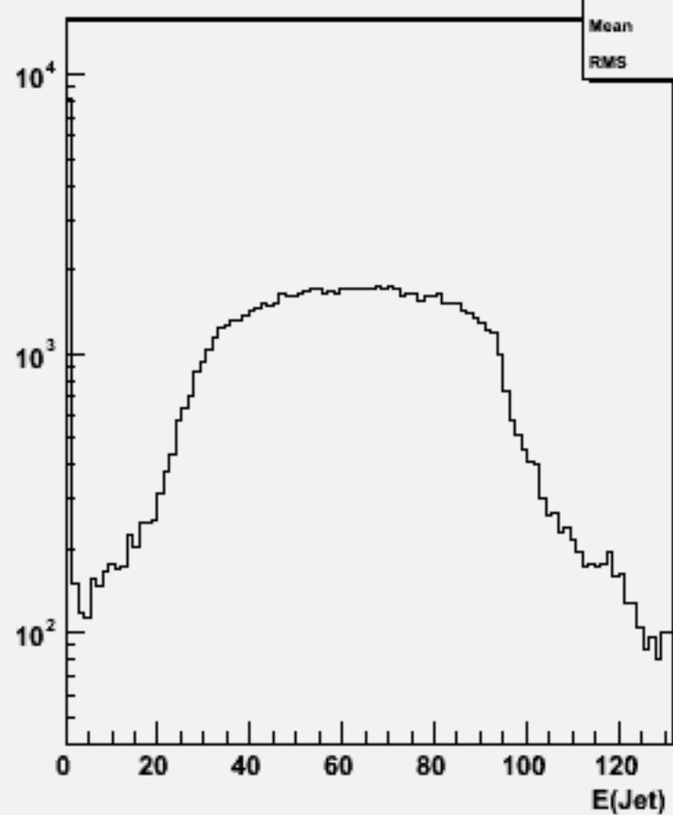
Jet energies(All jets)w104721 e1e1h_o
