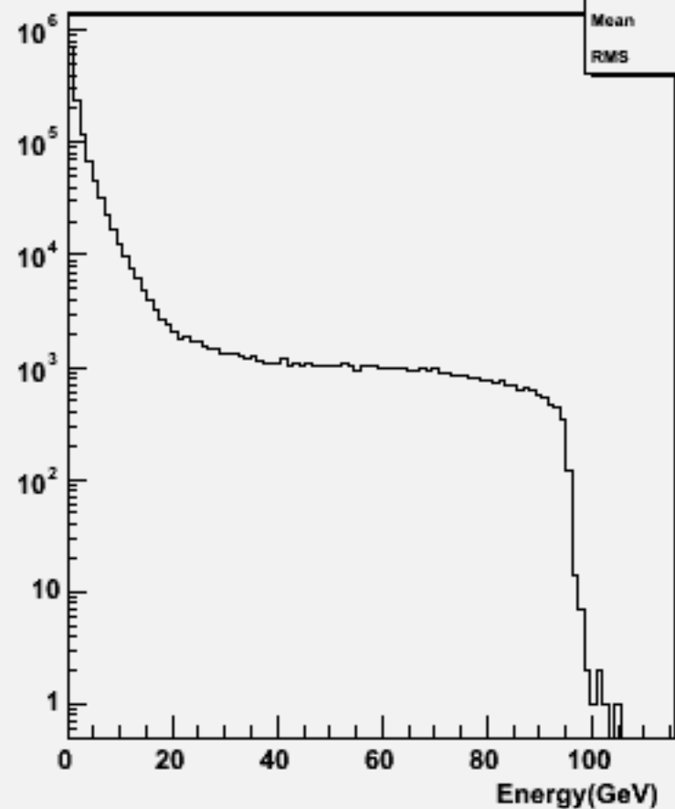
Particle Energy : w104721 e1e1h_o
