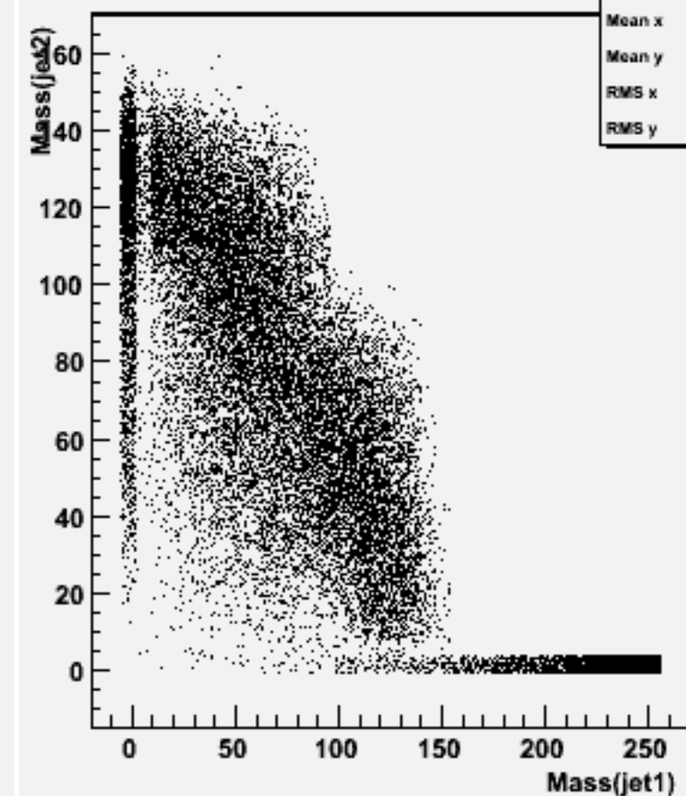
Jet mass for forced 2-jets : w104721 e1e1h_o
