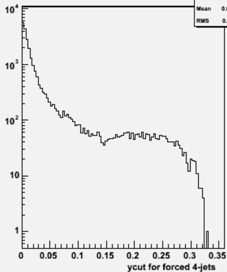
Ycut for 4-jets :w104721 e1e1h_o
