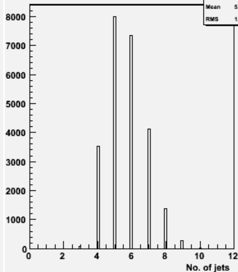
No. jets (ycut=0.001) : w104721 e1e1h_o
