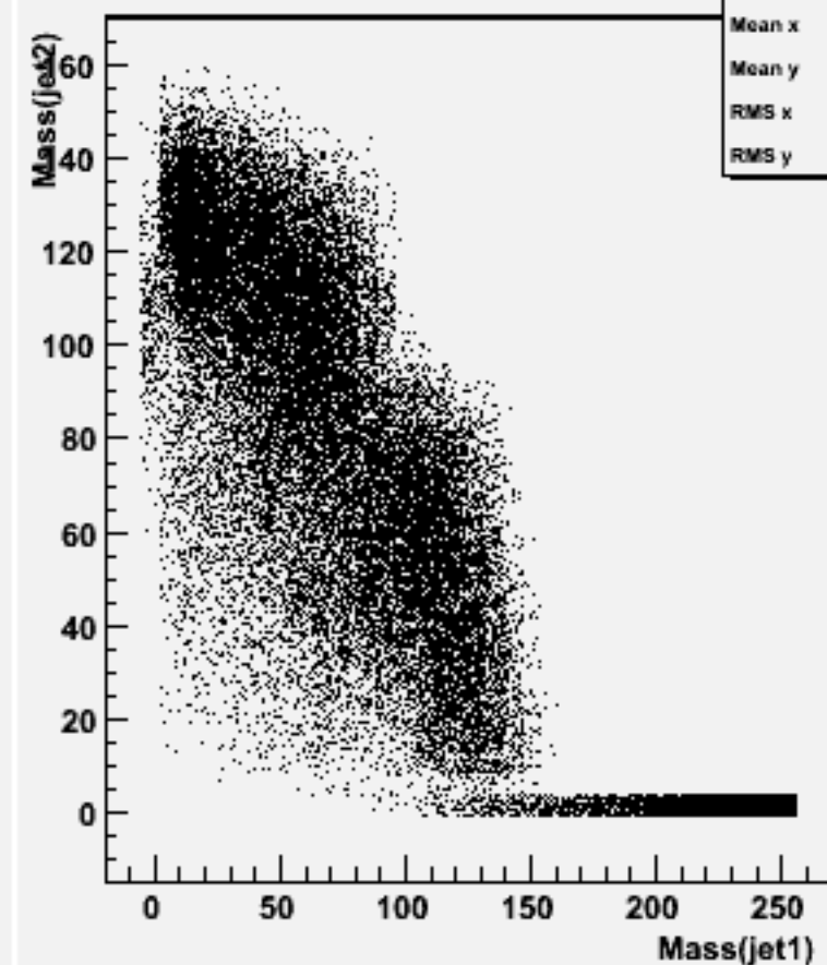
Jet mass for forced 2-jets : w104718 cch_o
