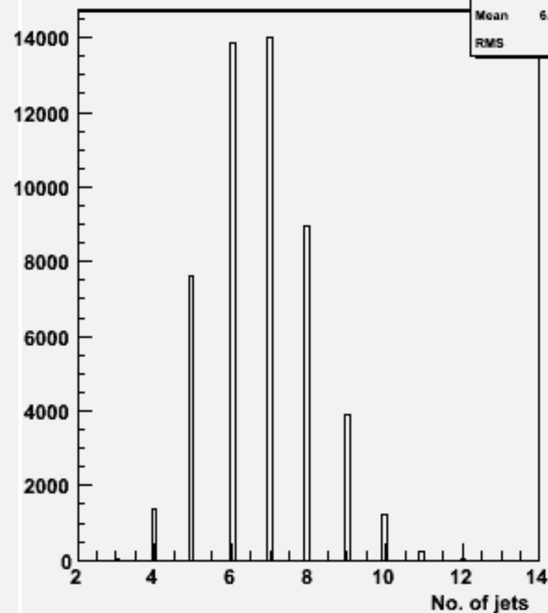
No. jets (ycut=0.001) : w104718 cch_o
