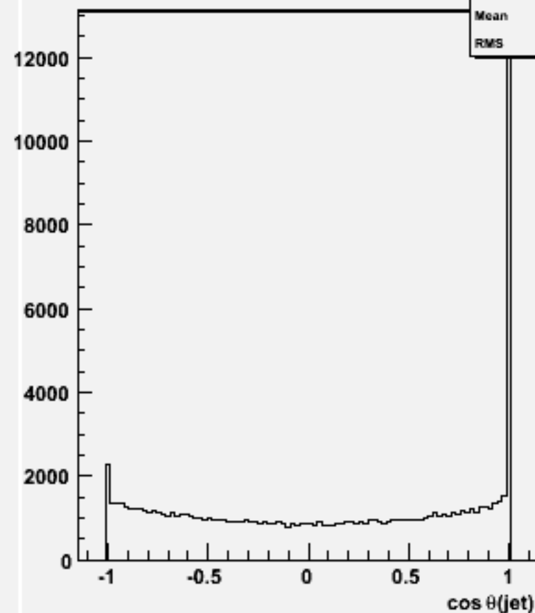
cos \Theta for 2-jets :w104718 cch_o
