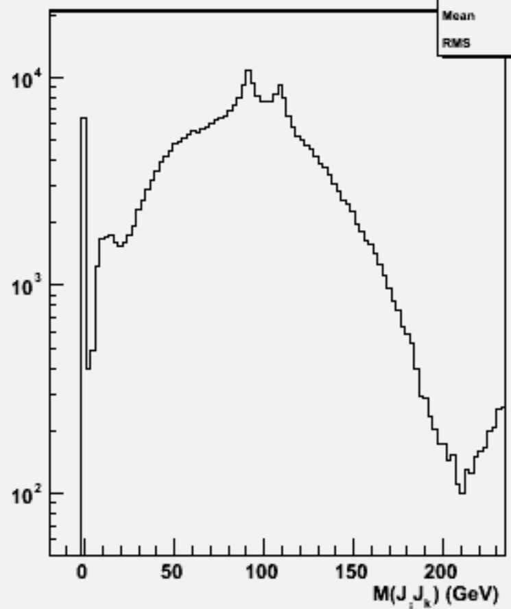
2jets mass(All comb)w104718 cch_o
