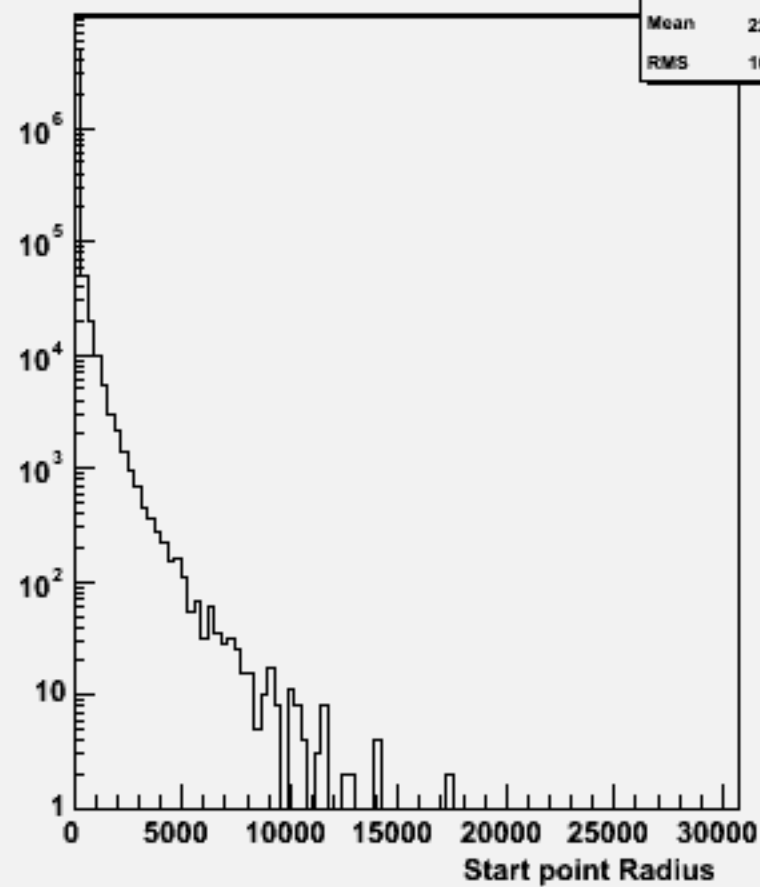
Start point R : w104718 cch_o
