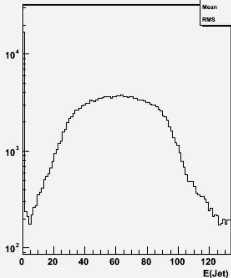
Jet energies(All jets)w104718 cch_o
