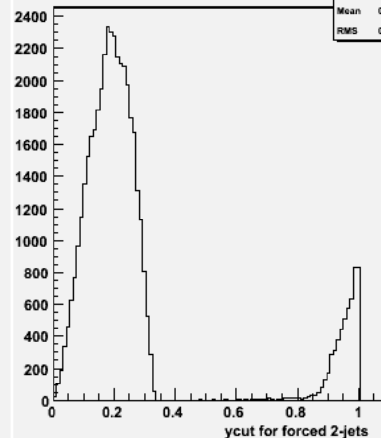
Ycut for 2-jets :w104718 cch_o
