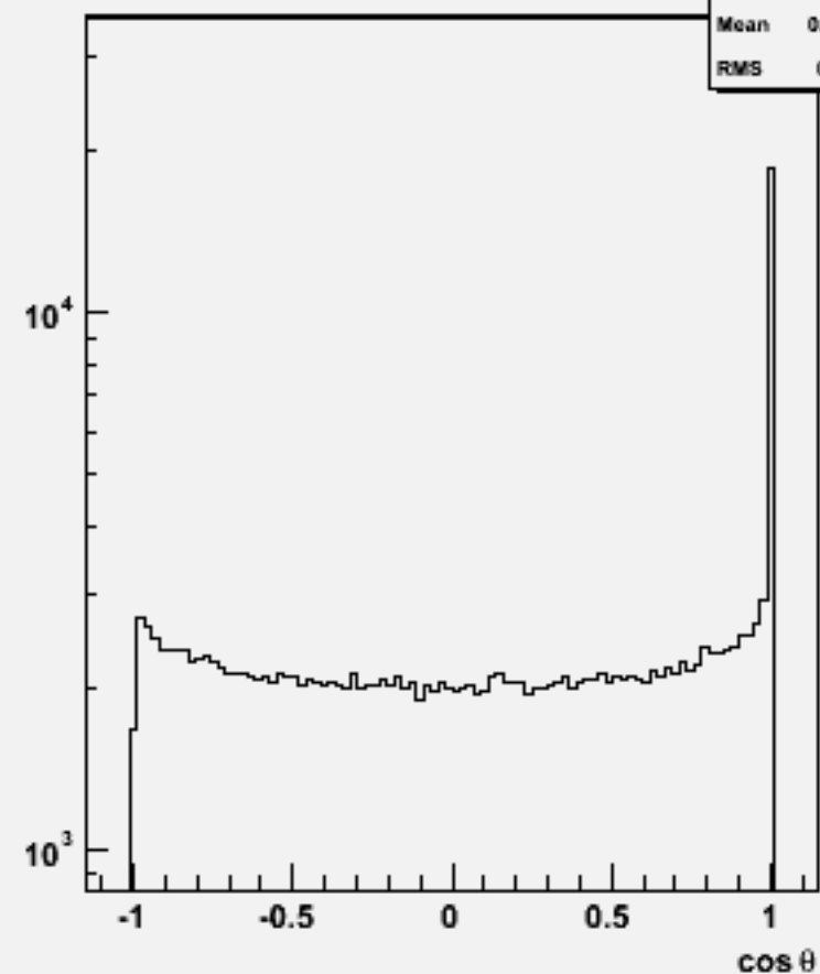
Jet cosθ (All jets)w104718 cch_o
