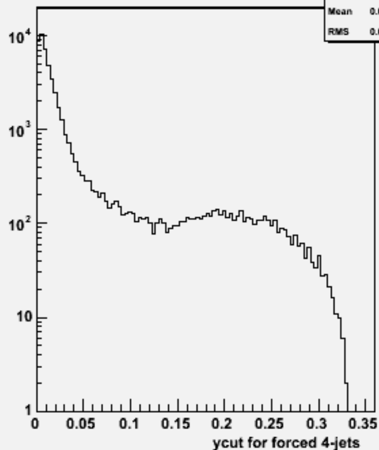
Ycut for 4-jets :w104718 cch_o
