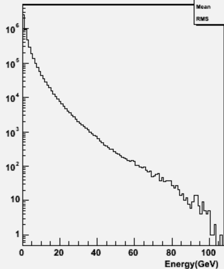
Start point R : w104718 cch_o
