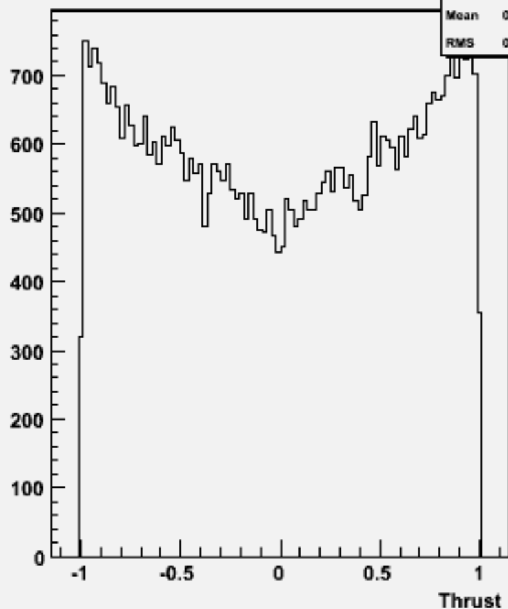
cos \Theta (thrust) w104718 cch_o
