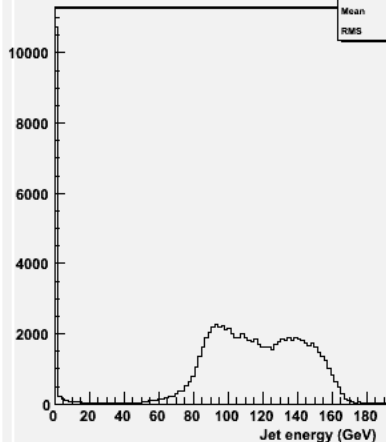
energy for 2-jets :w104718 cch_o
