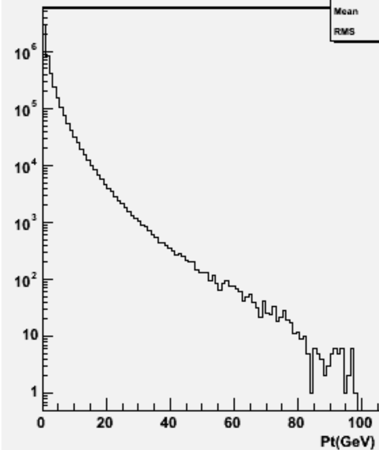
Start point Z : w104718 cch_o
