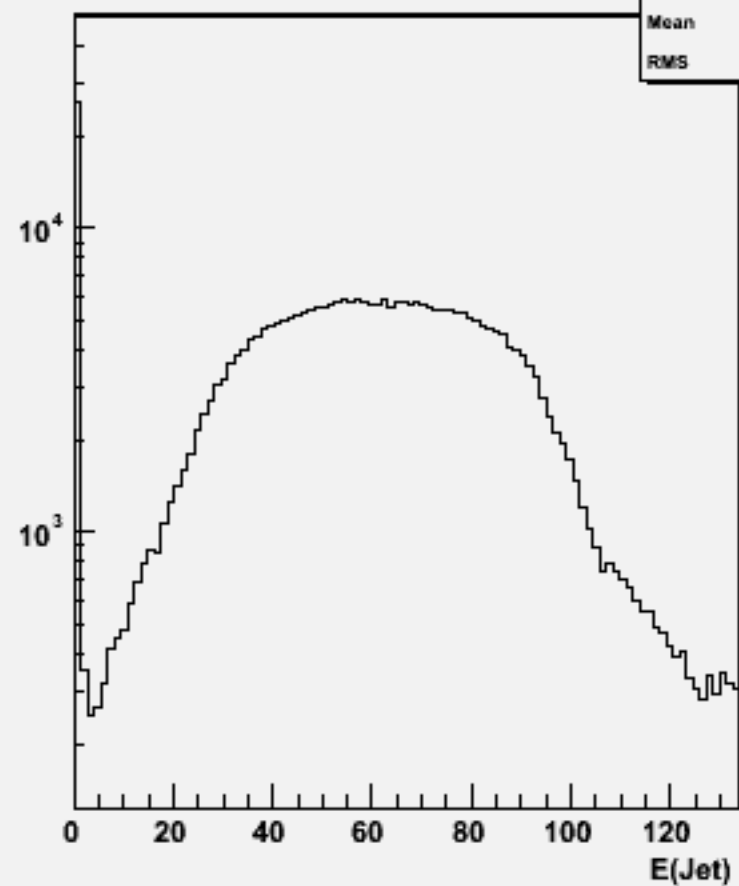
Jet energies(All jets)w104717 cch_o
