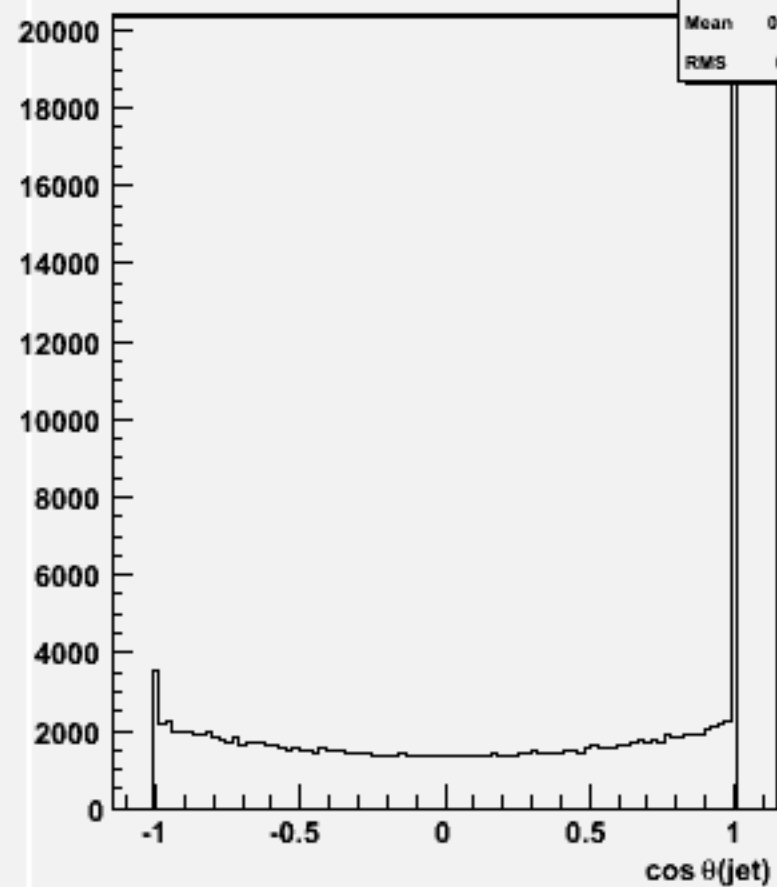
cos \theta for 2-jets :w104717 cch_o
