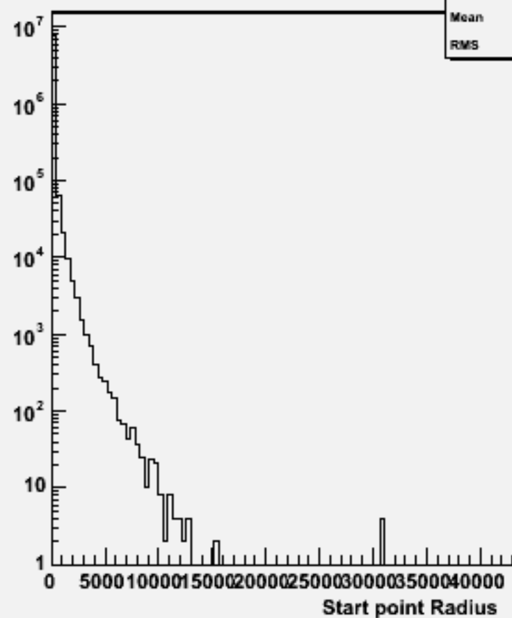
Start point R : w104717 cch_o
