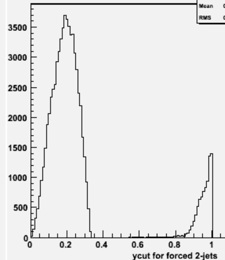
Ycut for 2-jets :w104717 cch_o
