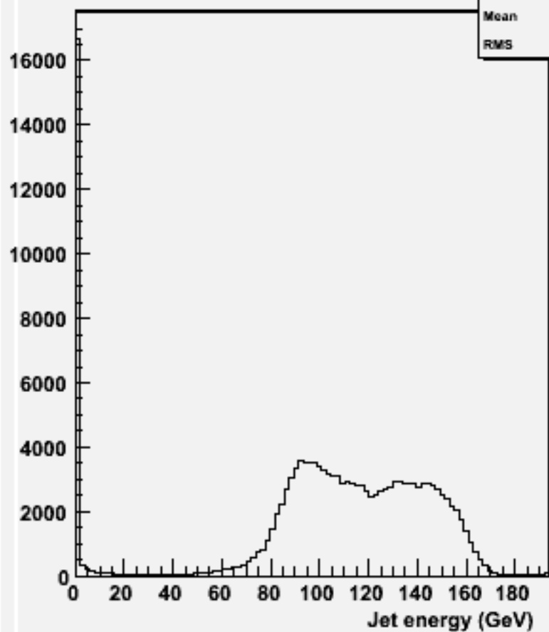
energy for 2-jets :w104717 cch_o
