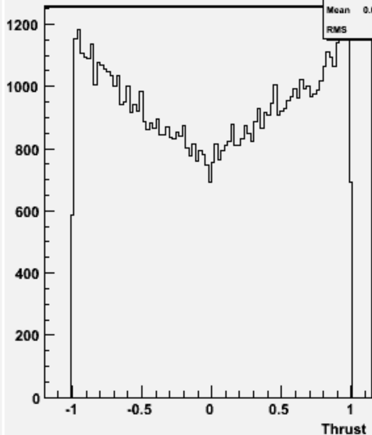
cos \Theta (thrust) w104717 cch_o
