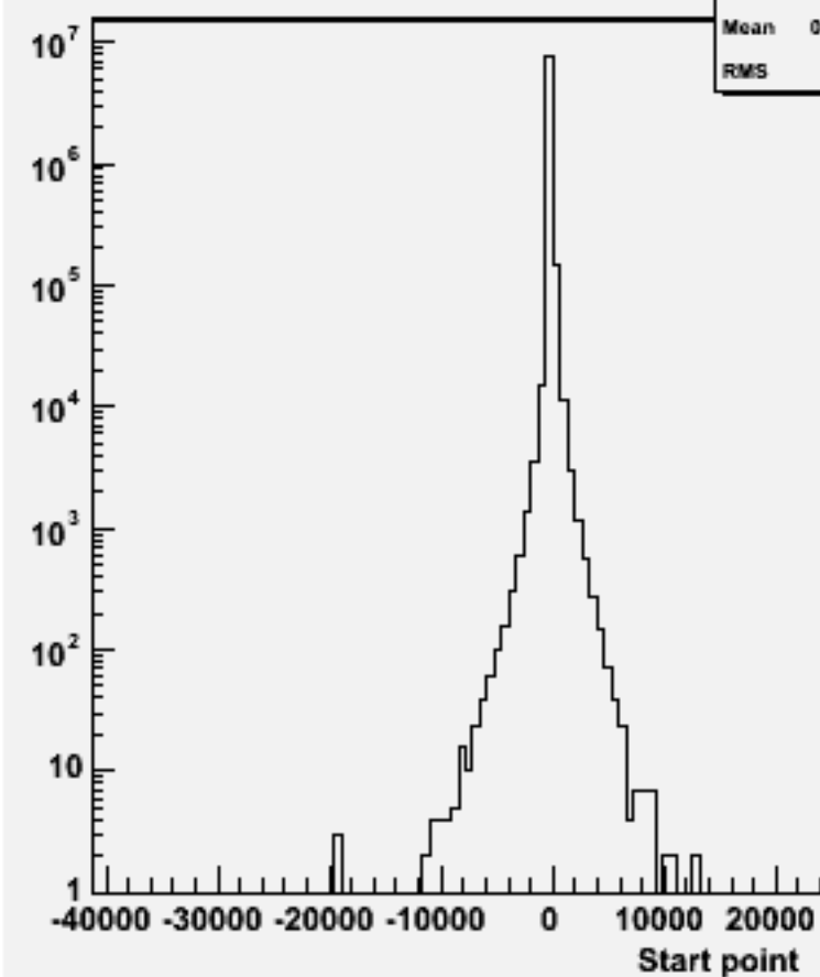
Start point Z : w104717 cch_o
