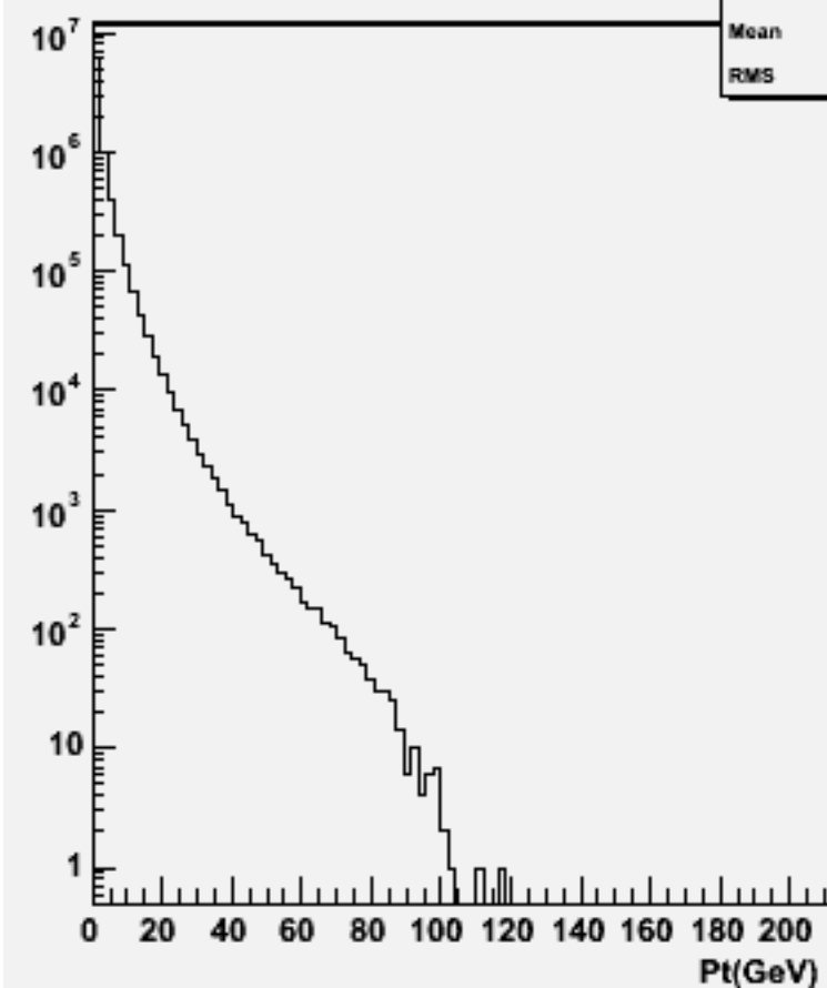
Particle Pt : w104717 cch_o
