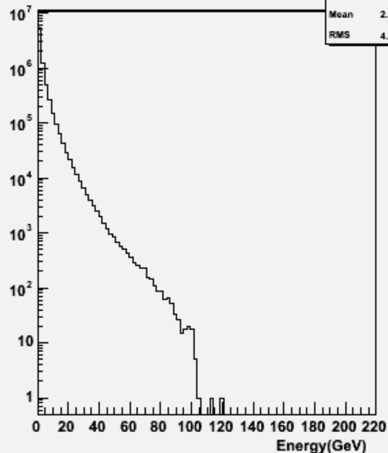
Particle Energy : w104717 cch_o
