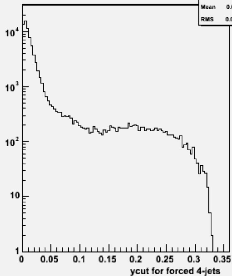
Ycut for 4-jets :w104717 cch_o
