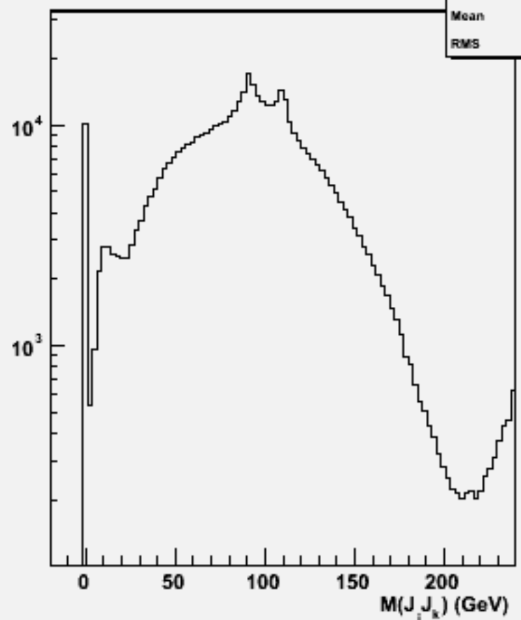
2jets mass(All comb)w104717 cch_o
