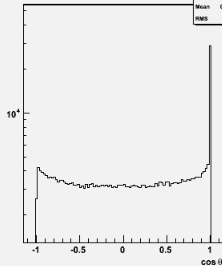
Jet cos \theta (All jets)w104717 cch_o
