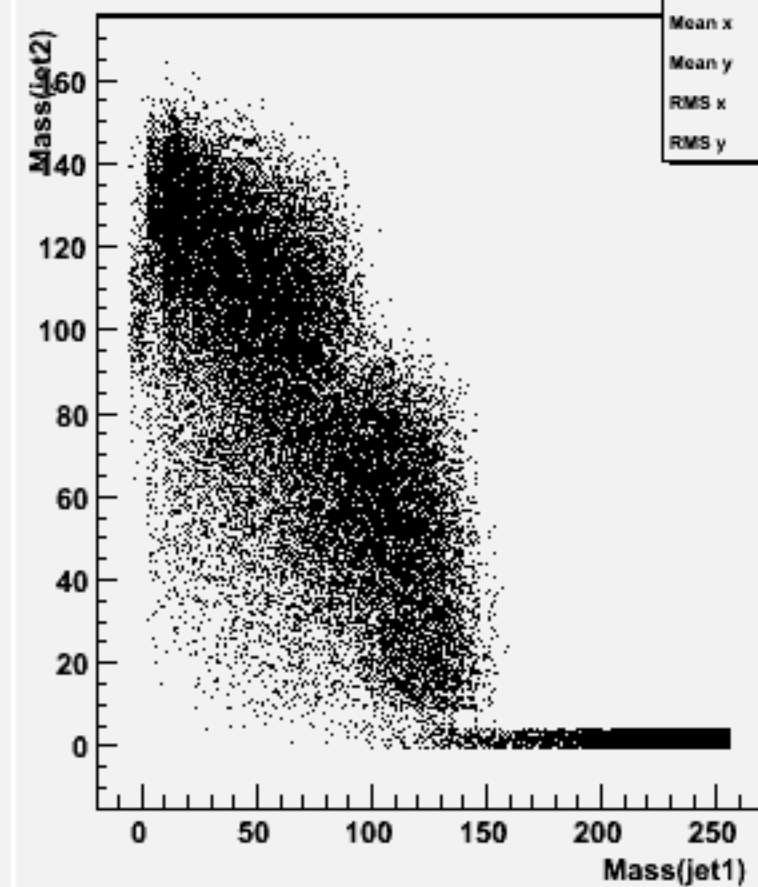
Jet mass for forced 2-jets : w104717 cch_o
