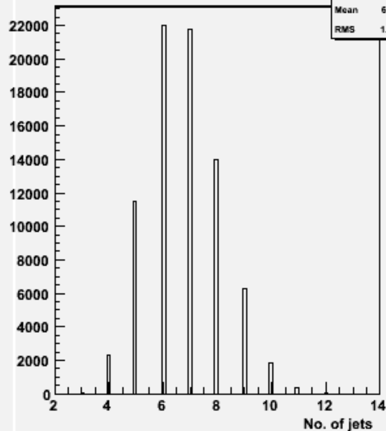
No. jets (ycut=0.001) : w104717 cch_o
