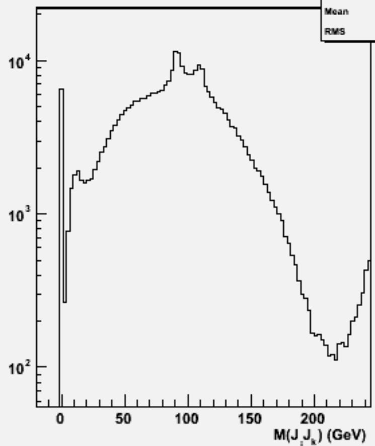
2jets mass(All comb)w104714 uu h _o
