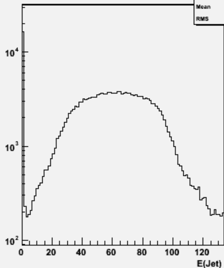
Jet energies(All jets)w104714 uu h _o
