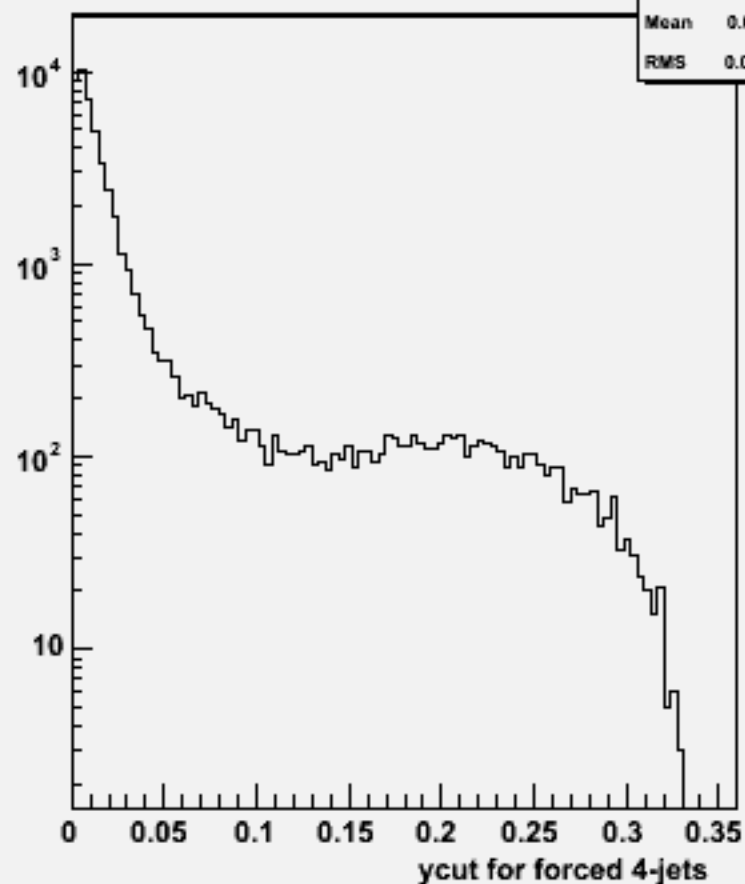
Ycut for 4-jets :w104714 uu h _o
