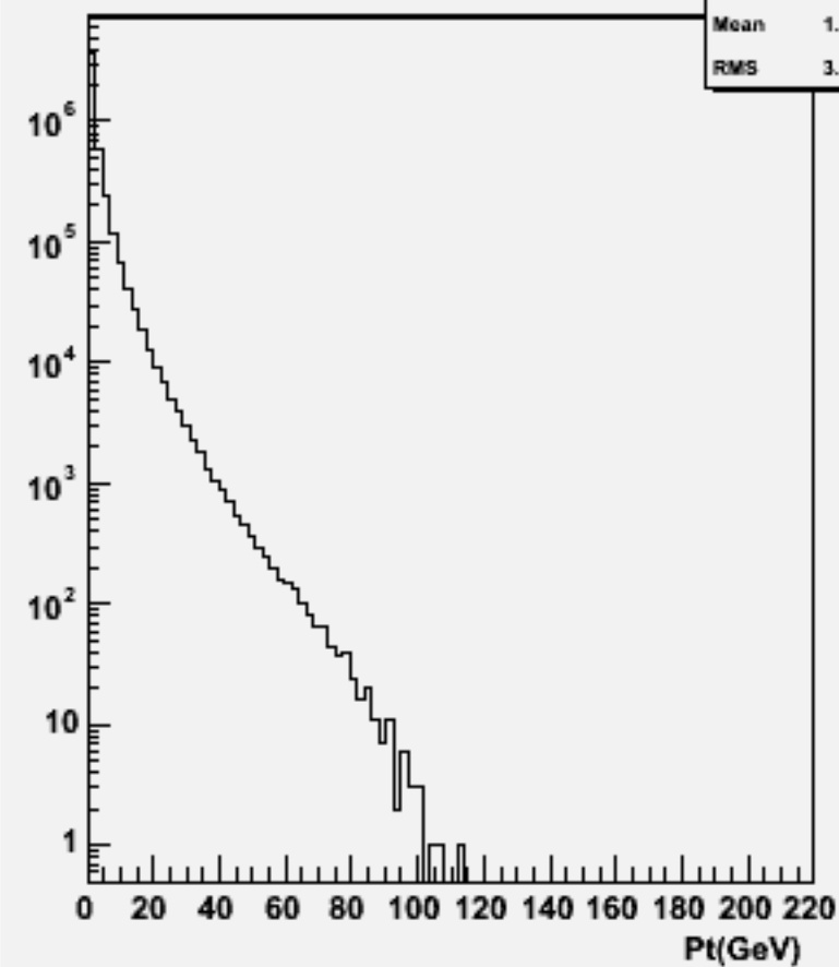
Particle Pt : w104714 uuh_o
