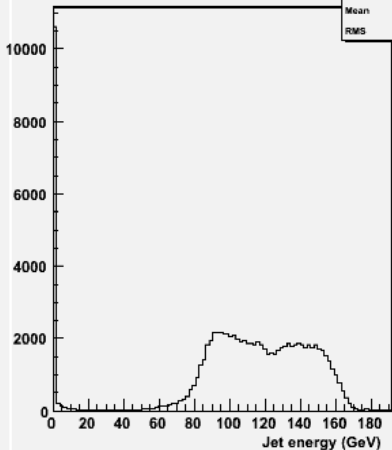
energy for 2-jets :w104714 uuh_o
