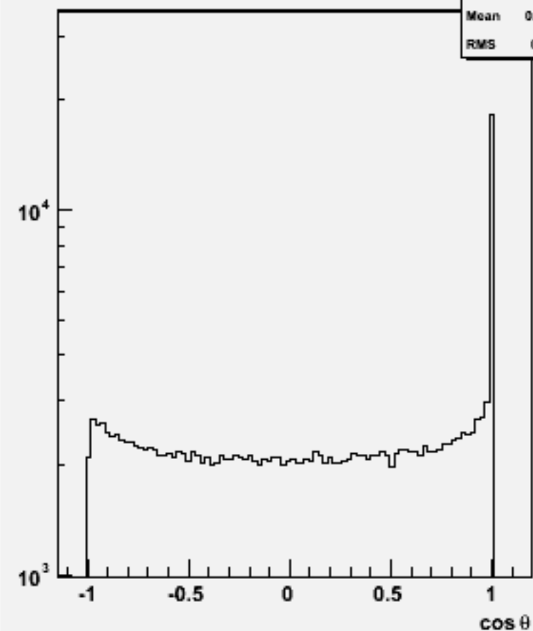
Jet cos \theta (All jets)w104714 uu h _o
