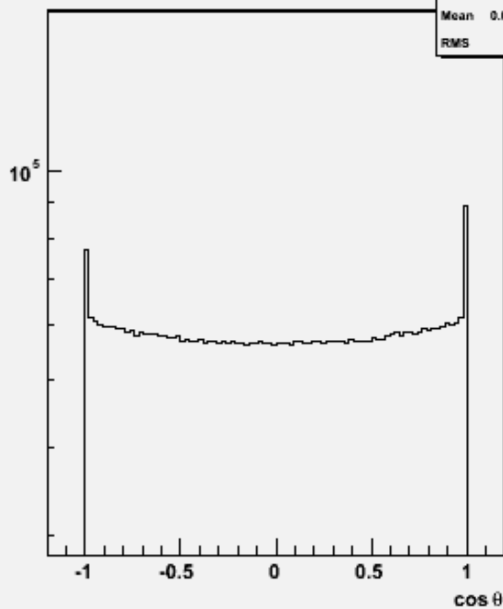
Particle \cos\theta : w104714 uuh_o
