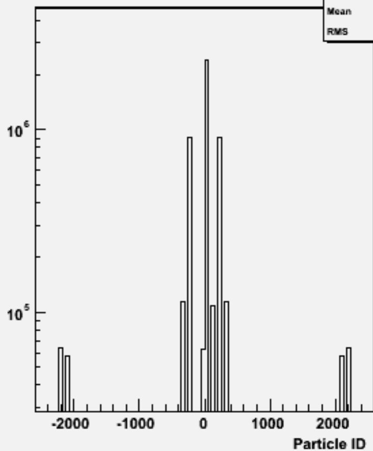
Particle ID : w104714 uuh_o
