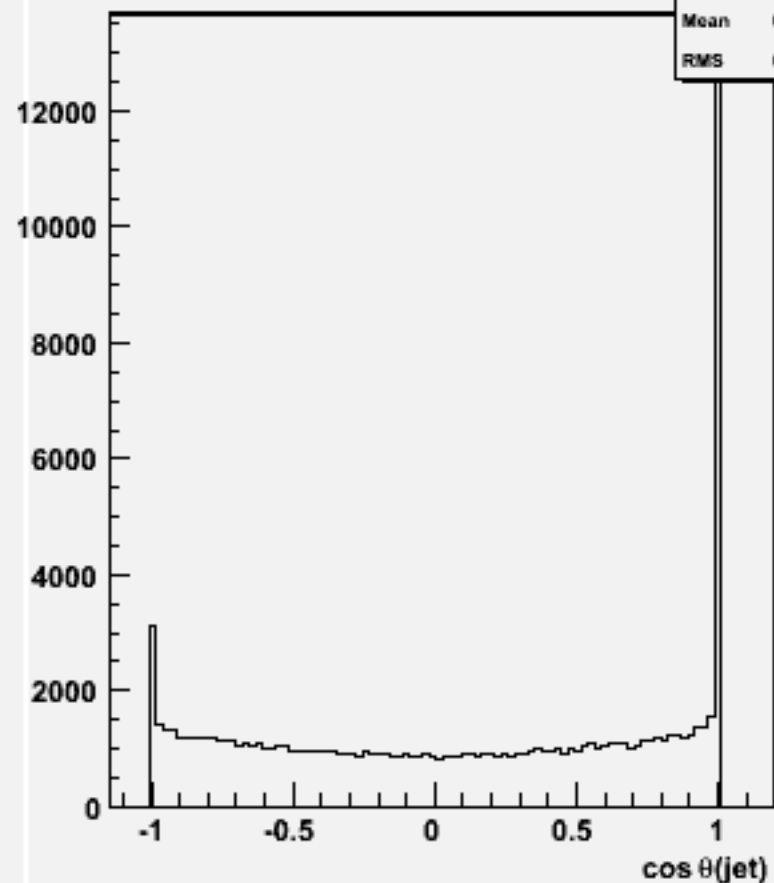
cos \theta for 2-jets :w104714 uuh_o
