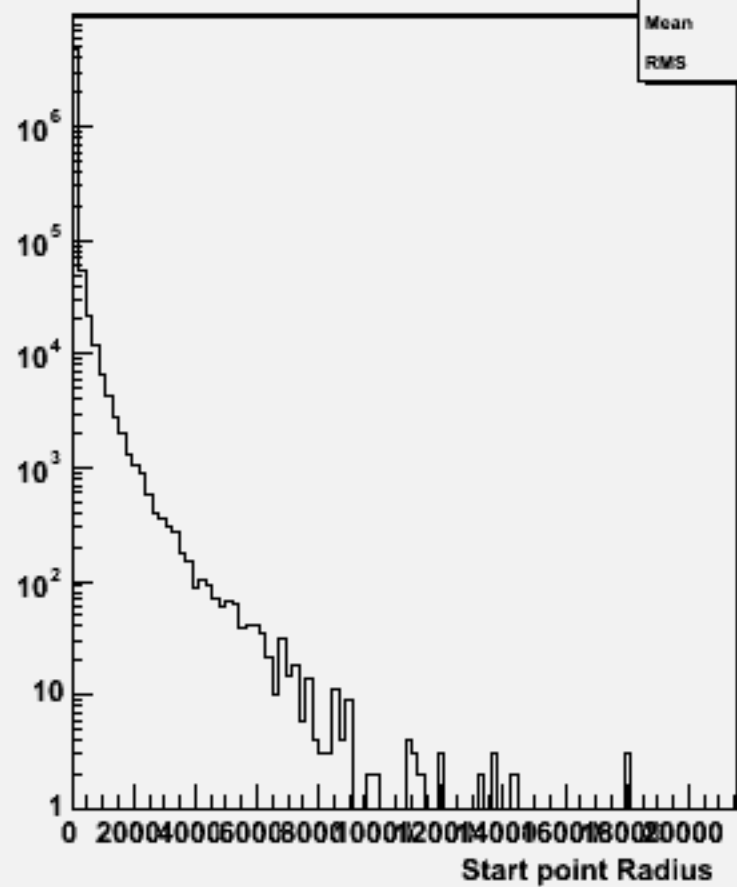
Start point R : w104714 uuh_o
