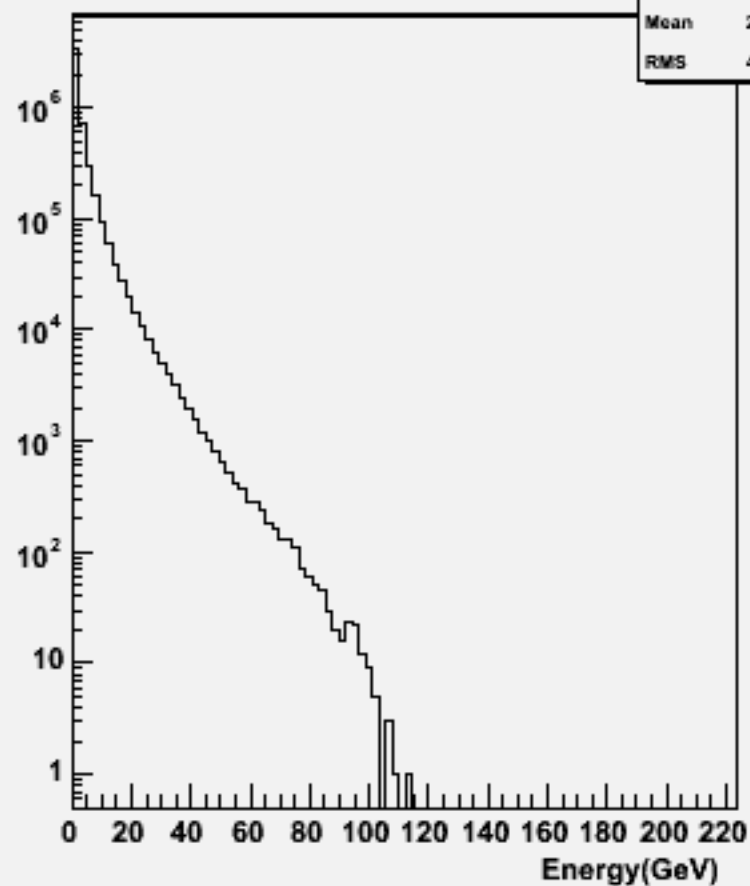
Particle Energy : w104714 uuh_o
