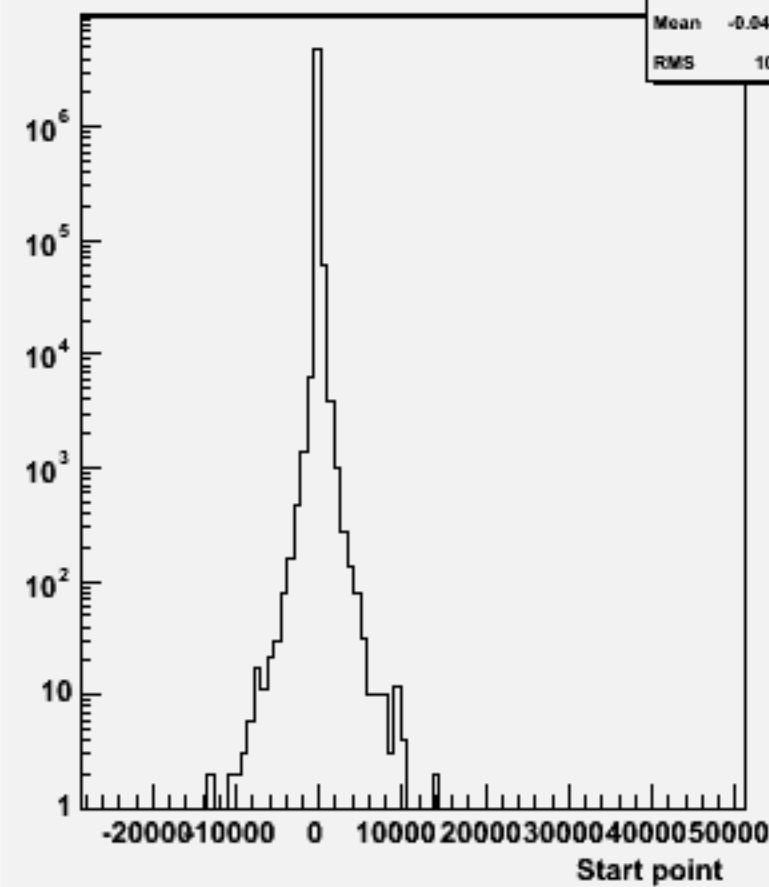
Start point Z : w104714 uuh_o
