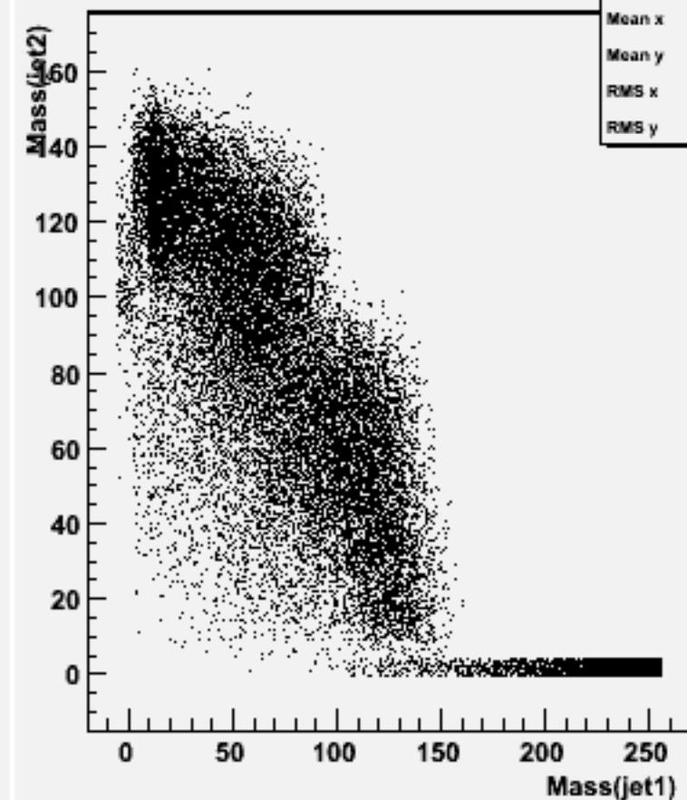
Jet mass for forced 2-jets : w104714 uuh_o
