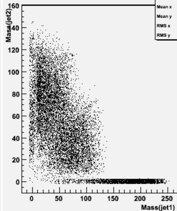
Jet mass for forced 2-jets : w104680 e3e3h_o
