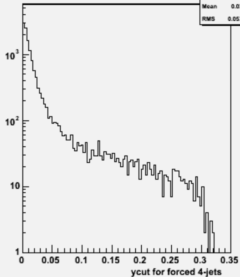
Ycut for 4-jets :w104680 e3e3h_o
