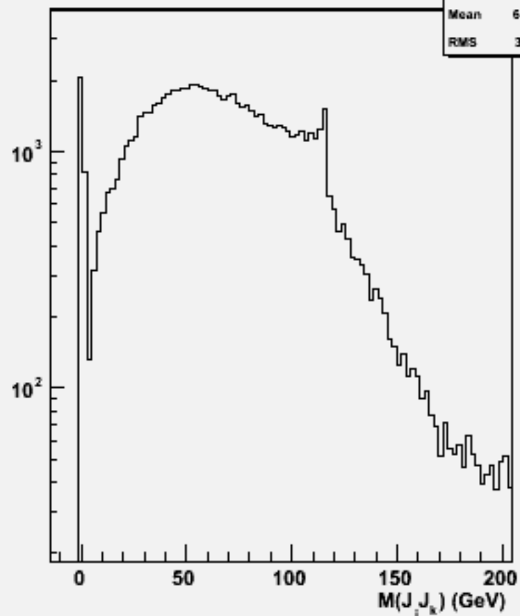
2jets mass(All comb)w104680 e3e3h_o
