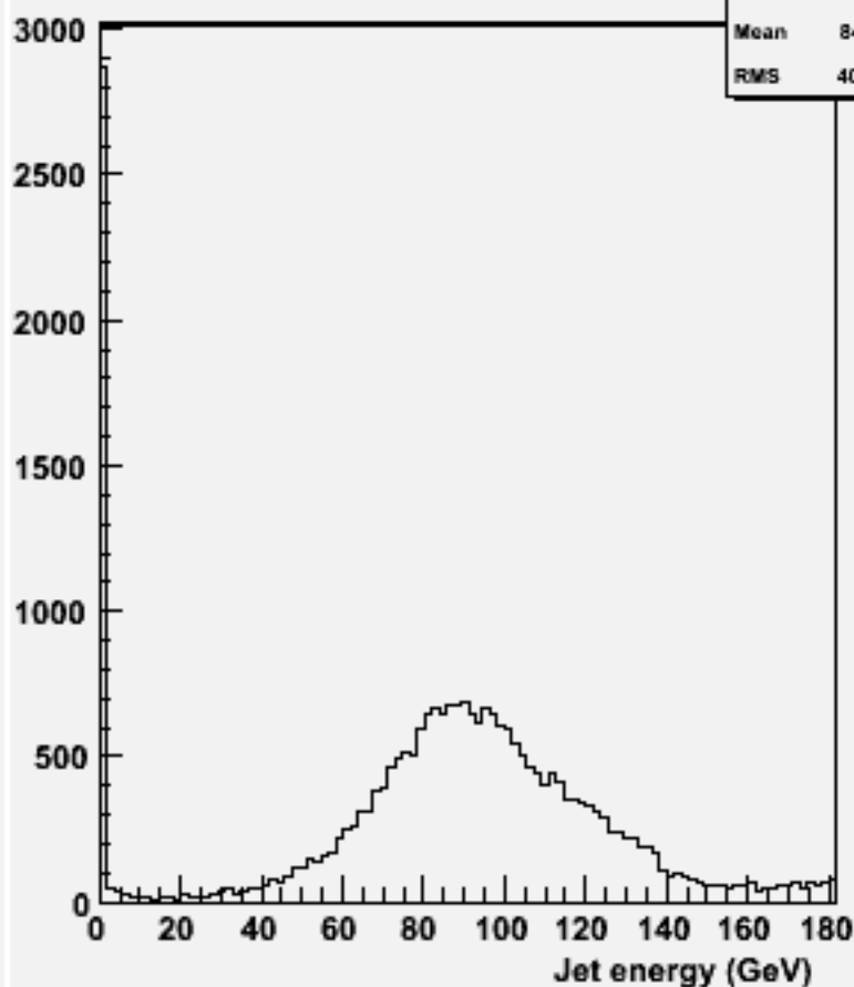
energy for 2-jets :w104680 e3e3h_o
