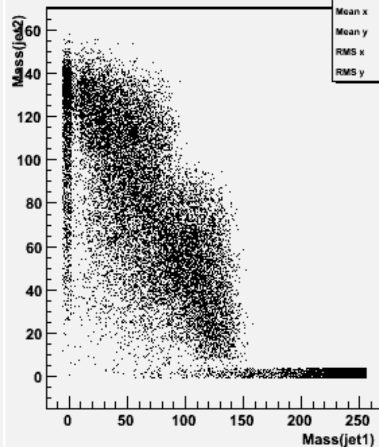
Jet mass for forced 2-jets : w104675 e2e2h_o
