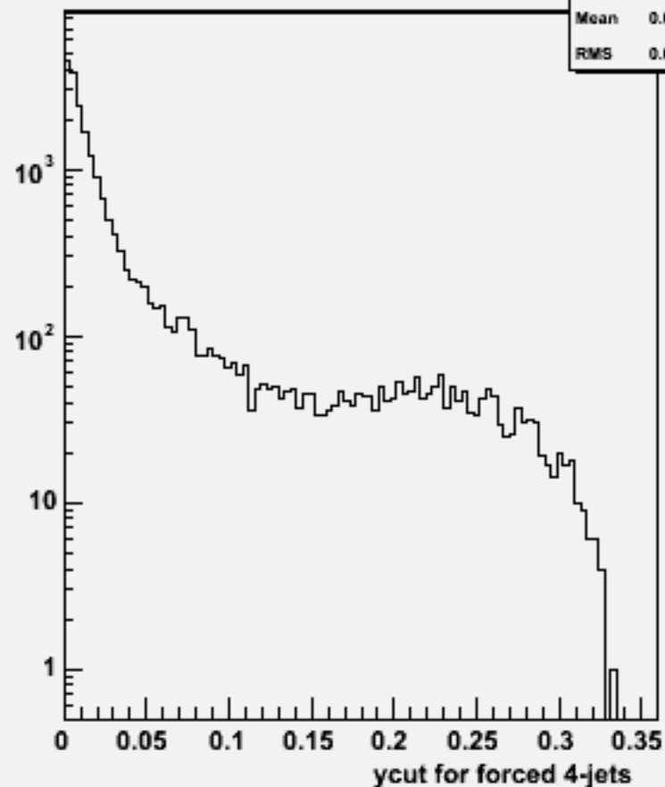
Ycut for 4-jets :w104675 e2e2h_o
