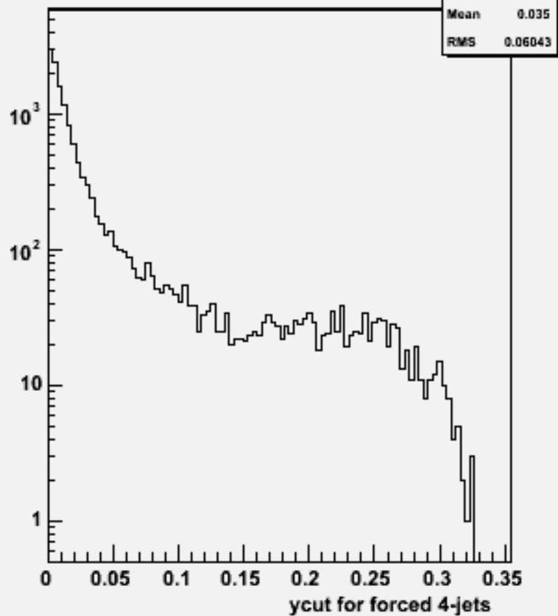
Ycut for 4-jets :w104672 e1e1h_o
