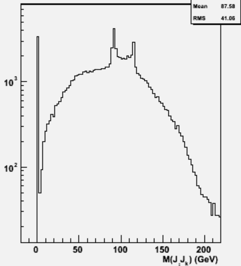
2jets mass(All comb)w104672 e1e1h_o
