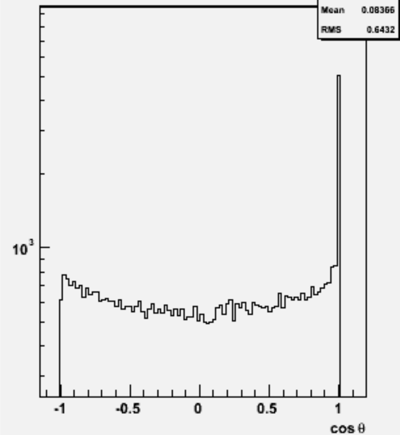
Jet cosθ (All jets)w104672 e1e1h_o
