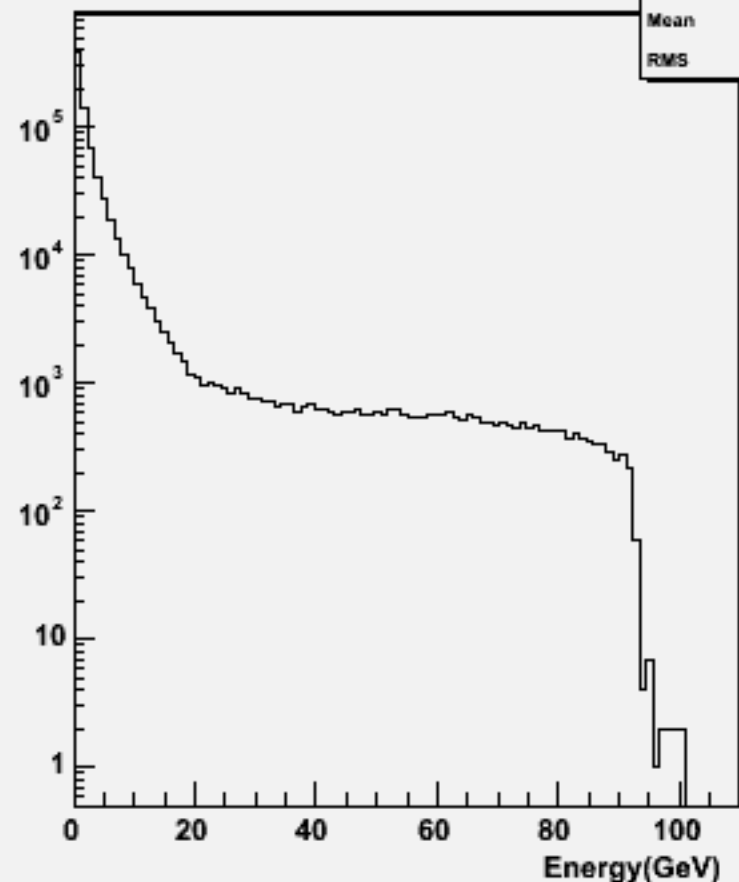
Particle Energy : w104672 e1e1h_o
