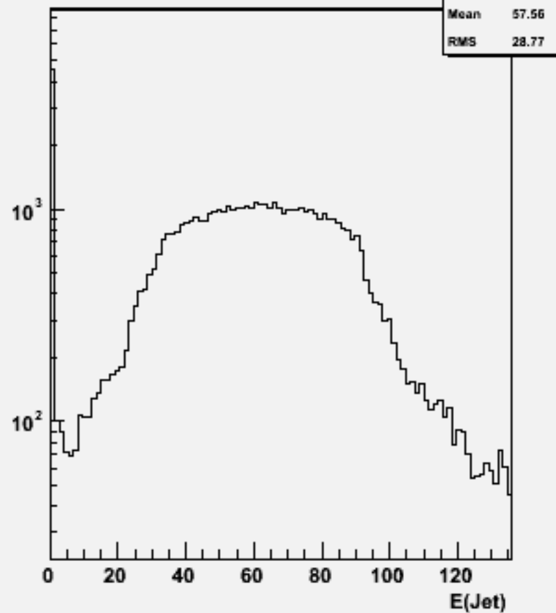
Jet energies(All jets)w104672 e1e1h_o
