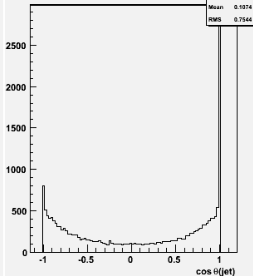
cos \theta for 2-jets :w104670 e1e1h_o
