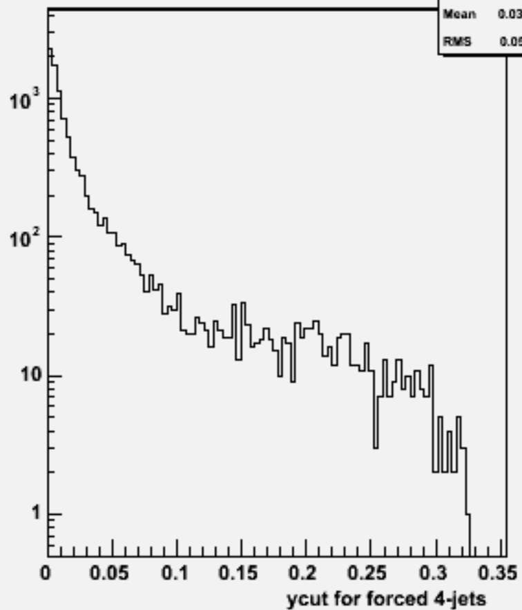
Ycut for 4-jets :w104670 e1e1h_o
