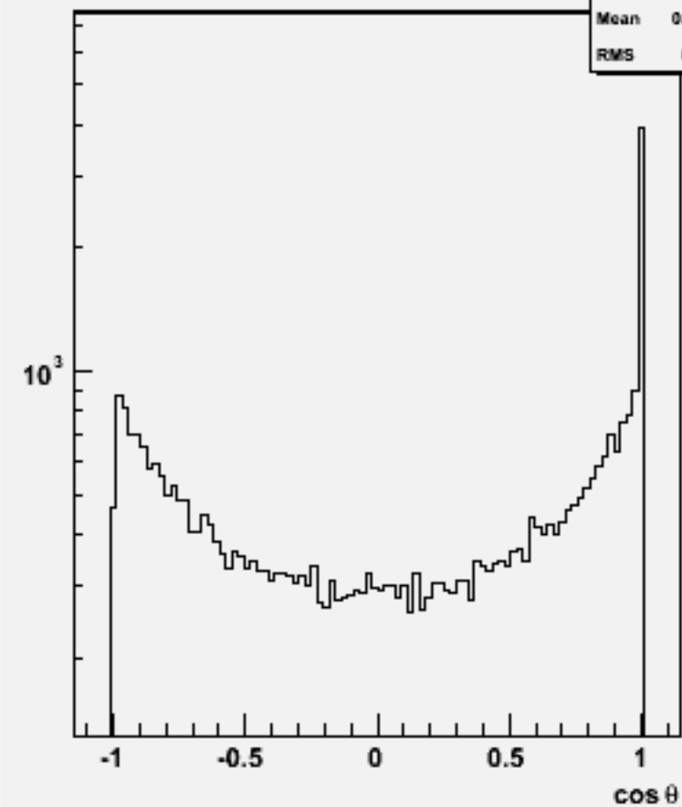
Jet cos \theta (All jets)w104670 e1e1h_o
