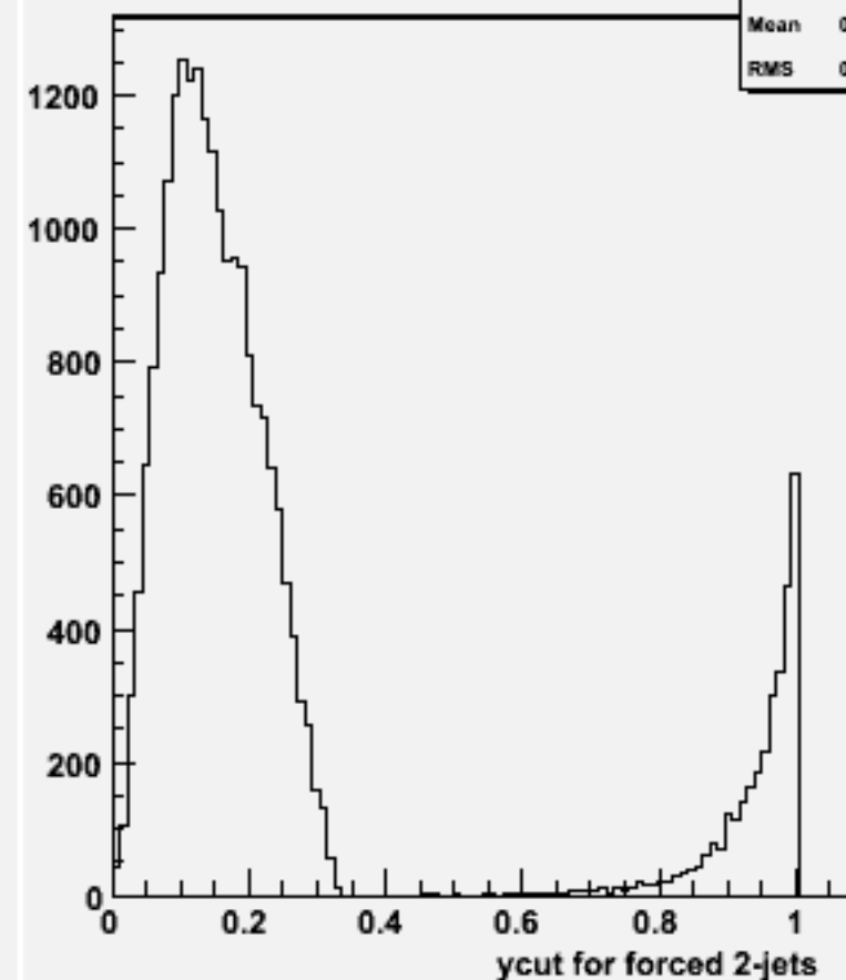
Ycut for 2-jets :w104633 ddh_o
