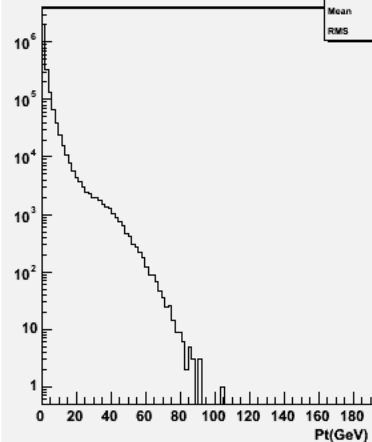
Particle Pt : w104633 ddh_o
