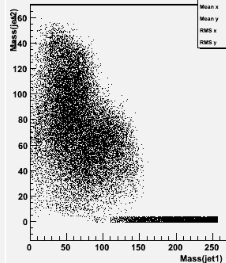
Jet mass for forced 2-jets : w104633 ddh_o
