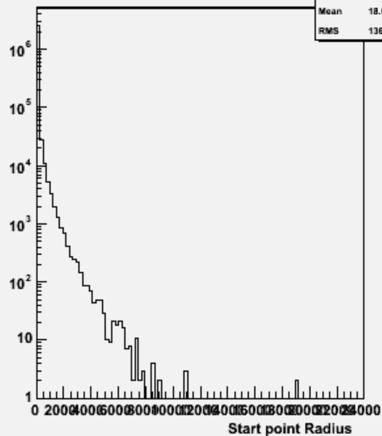
Start point R : w104633 ddh_o
