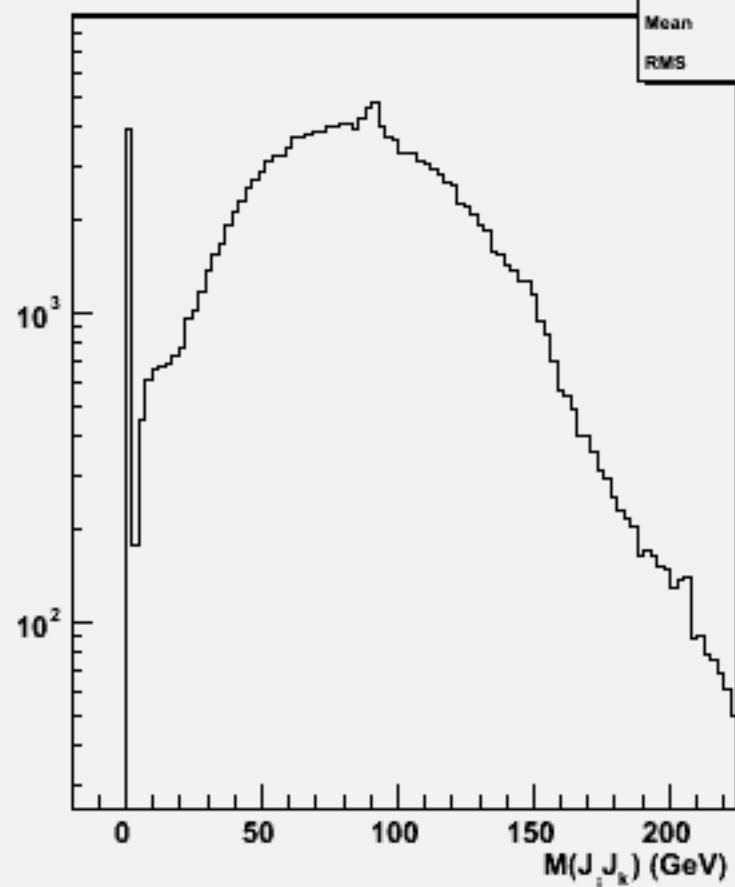
2jets mass(All comb)w104633 ddh_o
