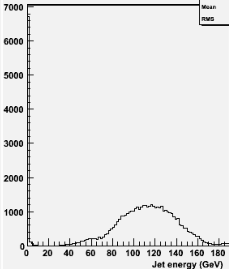
energy for 2-jets :w104633 ddh_o
