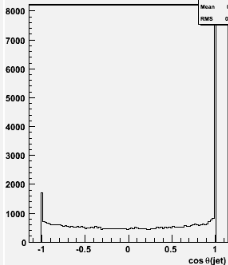
cos \theta for 2-jets :w104633 ddh_o
