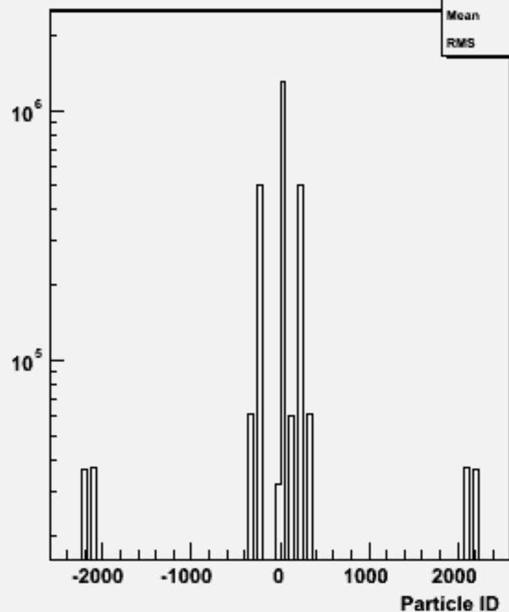
Particle ID : w104633 ddh_o
