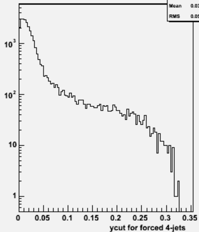
Ycut for 4-jets :w104633 ddh_o
