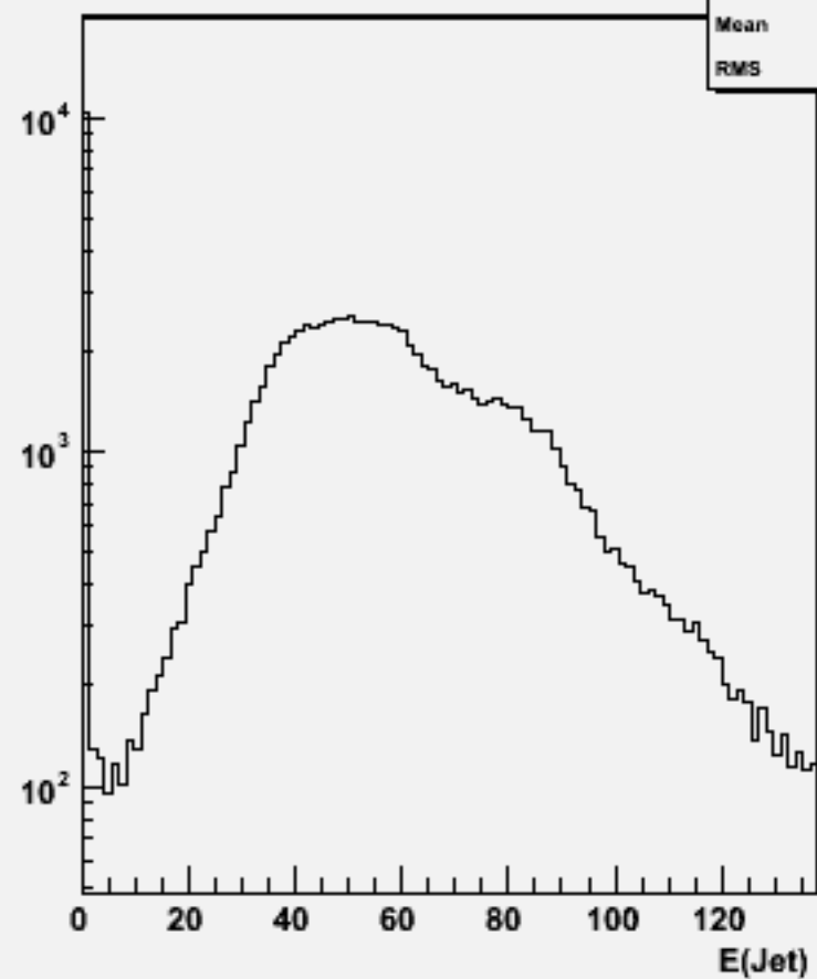
Jet energies(All jets)w104633 ddh_o
