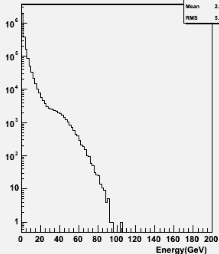
Particle Energy : w104633 ddh_o
