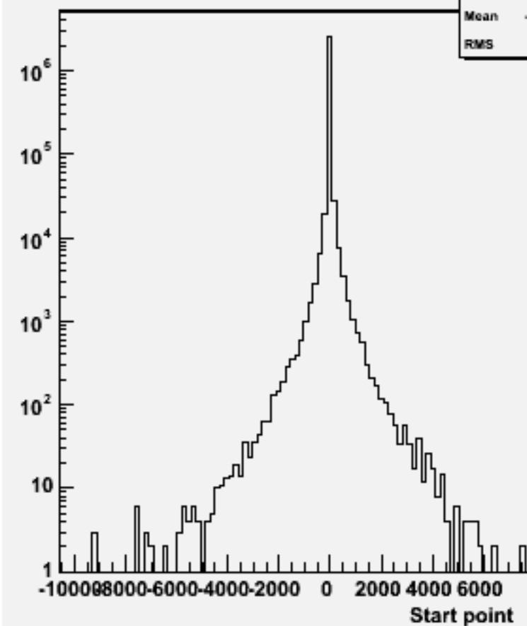
Start point Z : w104633 ddh_o
