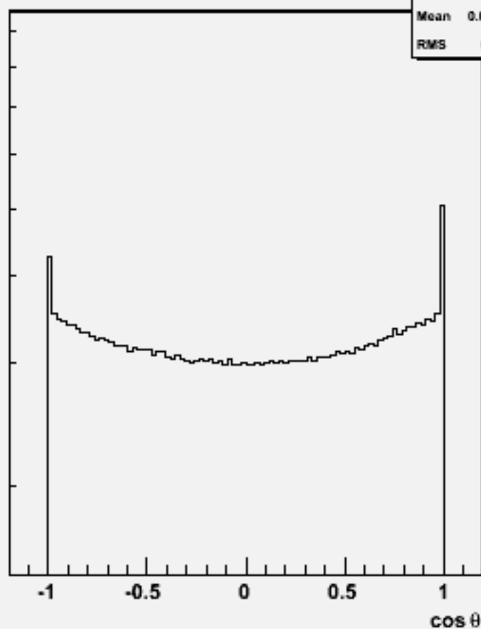
Particle cos \theta : w104633 ddh_o
