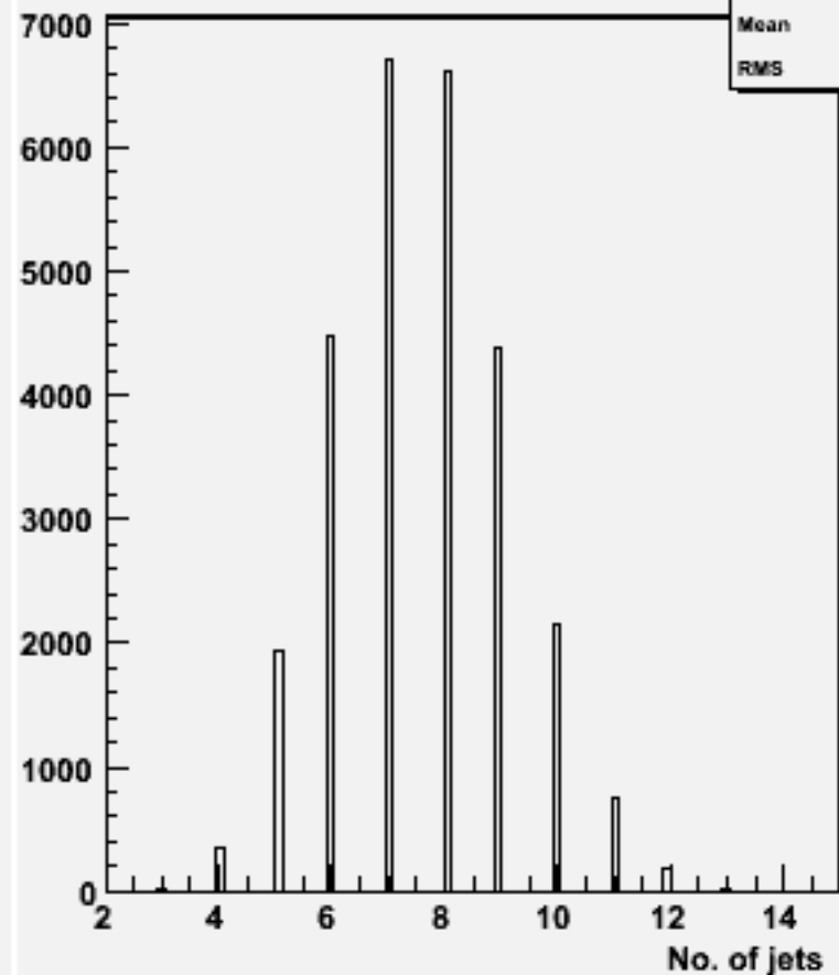
No. jets (ycut=0.001) : w104633 ddh_o
