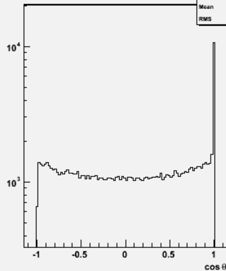
Jet cos \theta (All jets)w104633 ddh_o
