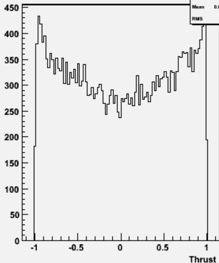
cos \Theta (thrust) w104633 ddh_o
