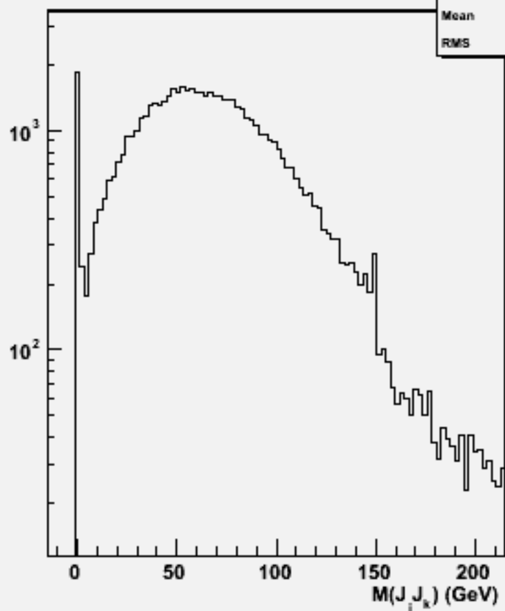
2jets mass(All comb)w104630 e3e3h_o
