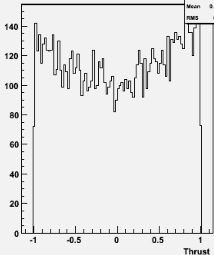
cos \Theta (thrust) w104630 e3e3h_o
