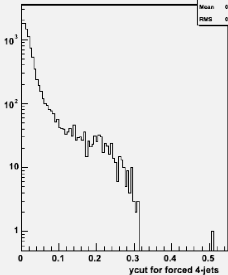
Ycut for 4-jets :w104630 e3e3h_o
