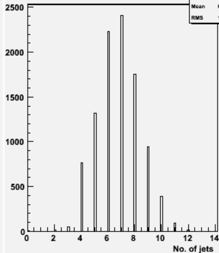
No. jets (ycut=0.001) : w104630 e3e3h_o
