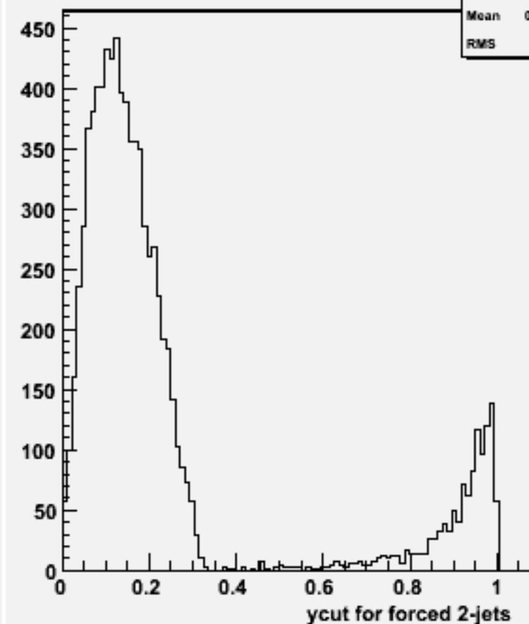
Ycut for 2-jets :w104630 e3e3h_o
