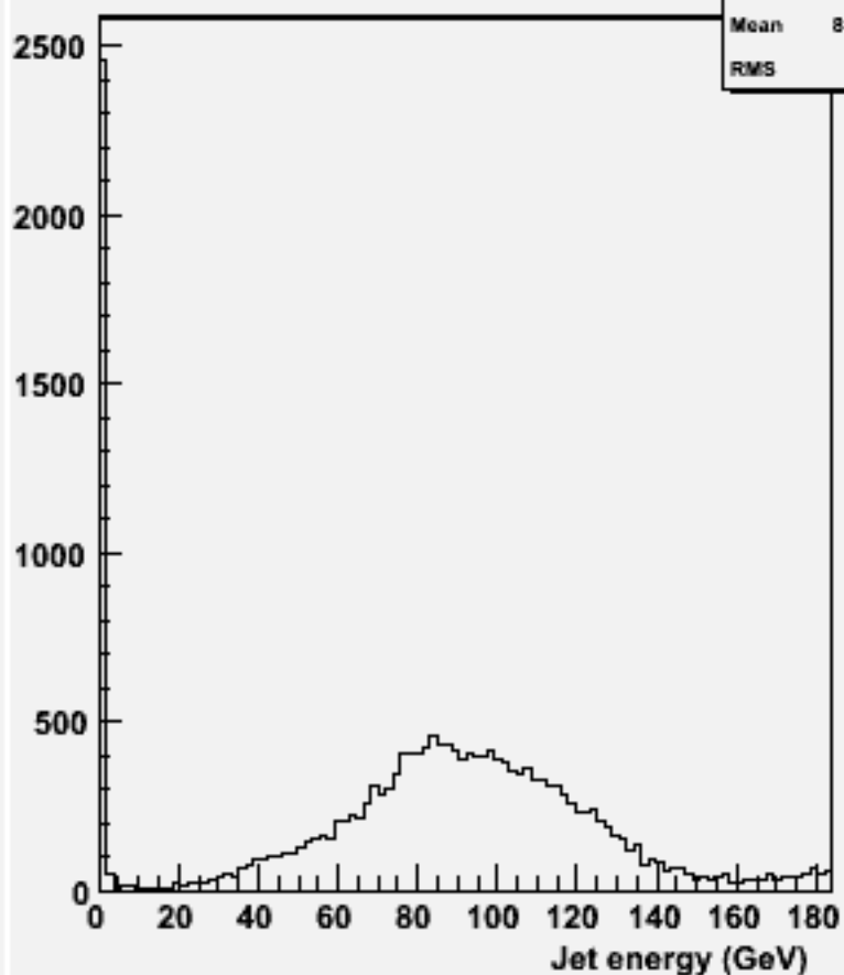
energy for 2-jets :w104630 e3e3h_o
