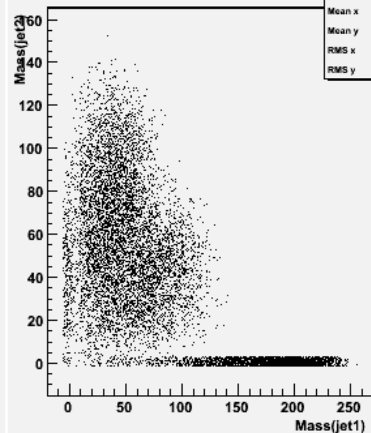
Jet mass for forced 2-jets : w104630 e3e3h_o
