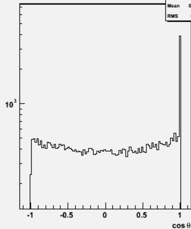
Jet cos \theta (All jets)w104630 e3e3h_o
