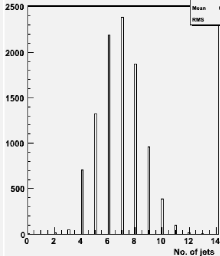
No. jets (ycut=0.001) : w104629 e3e3h_o
