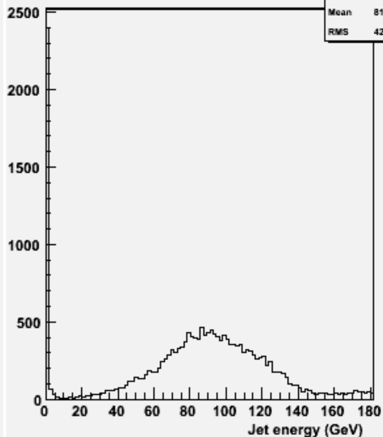
energy for 2-jets :w104629 e3e3h_o
