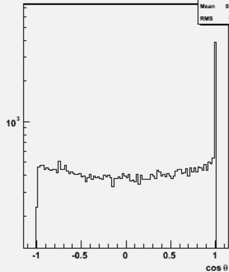
Jet cos \theta (All jets)w104629 e3e3h_o
