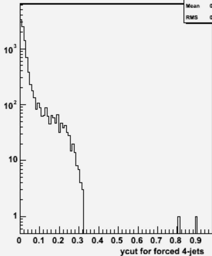
Ycut for 4-jets :w104629 e3e3h_o
