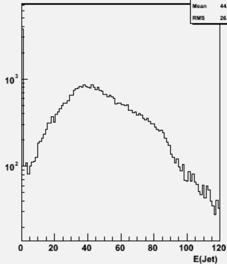
Jet energies(All jets)w104629 e3e3h_o
