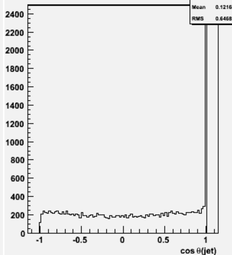
cos \theta for 2-jets :w104629 e3e3h_o
