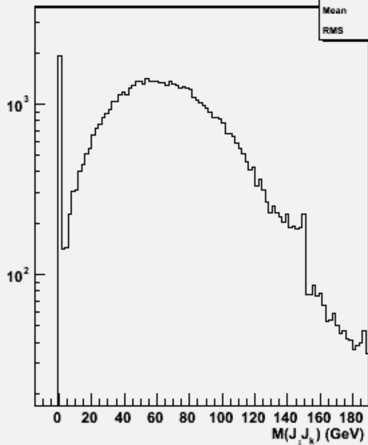
2jets mass(All comb)w104629 e3e3h_o
