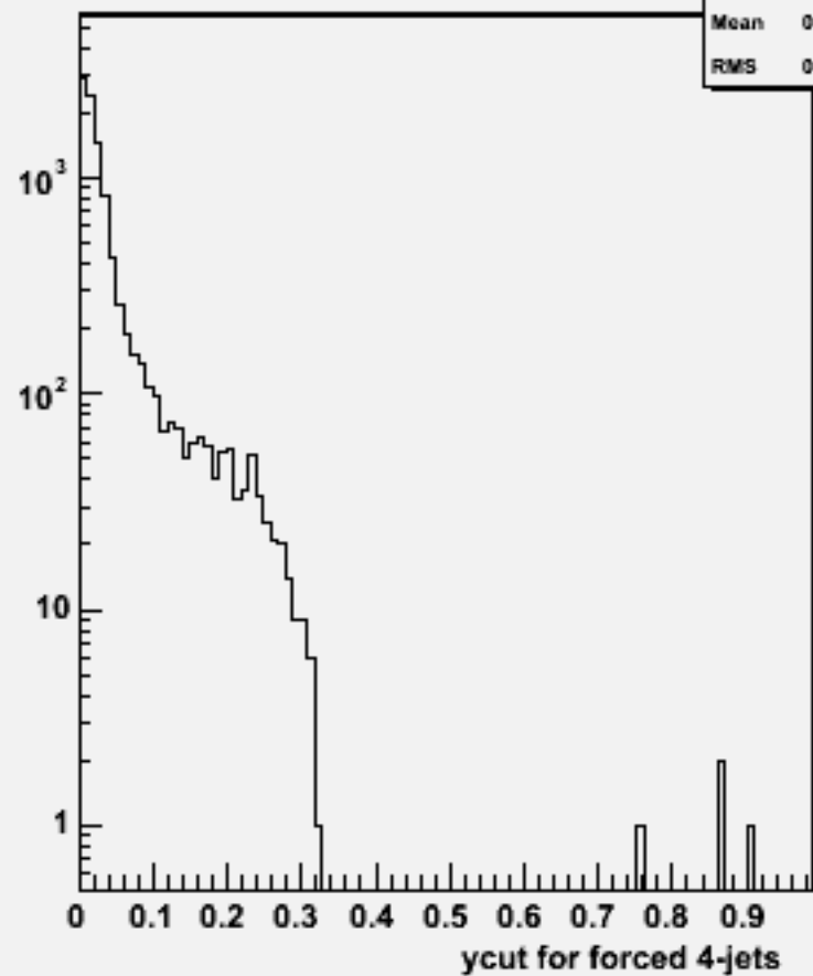
Ycut for 4-jets :w104626 e2e2h_o
