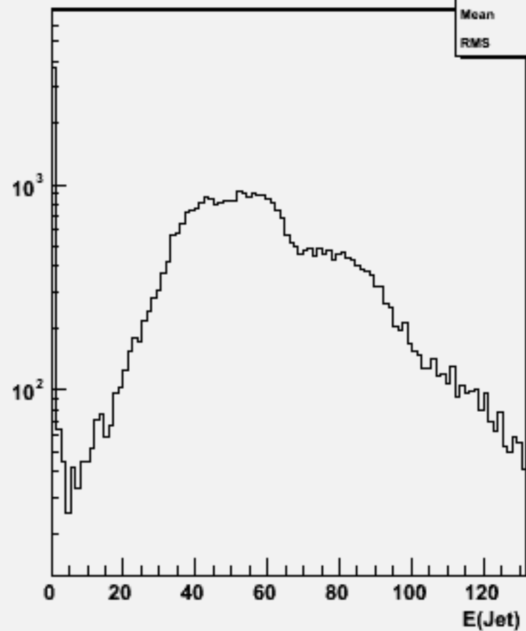
Jet energies(All jets)w104626 e2e2h_o
