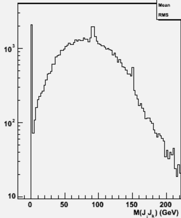
2jets mass(All comb)w104626 e2e2h_o
