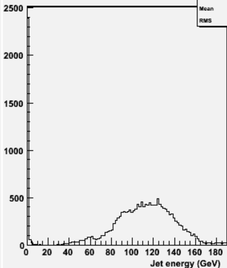
energy for 2-jets :w104626 e2e2h_o
