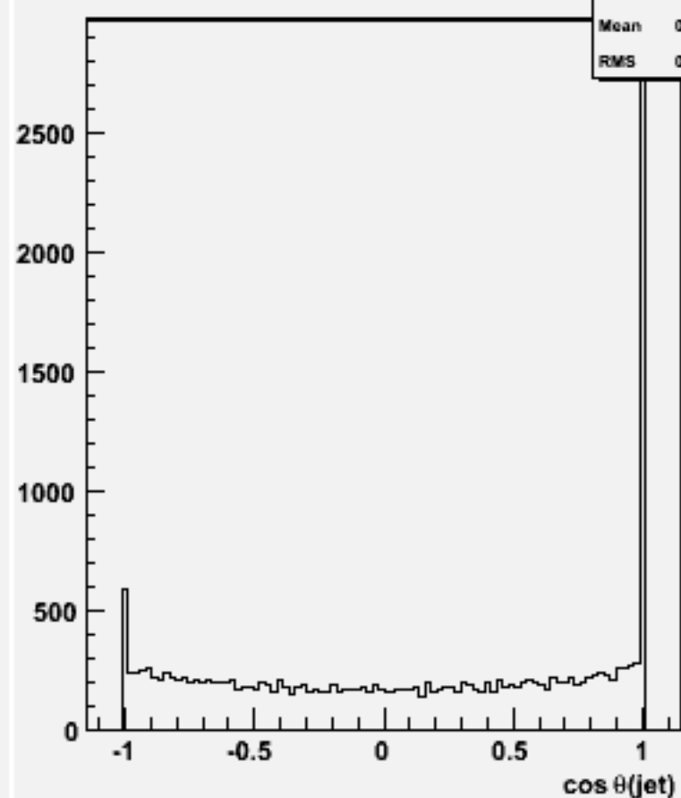
cos \theta for 2-jets :w104626 e2e2h_o
