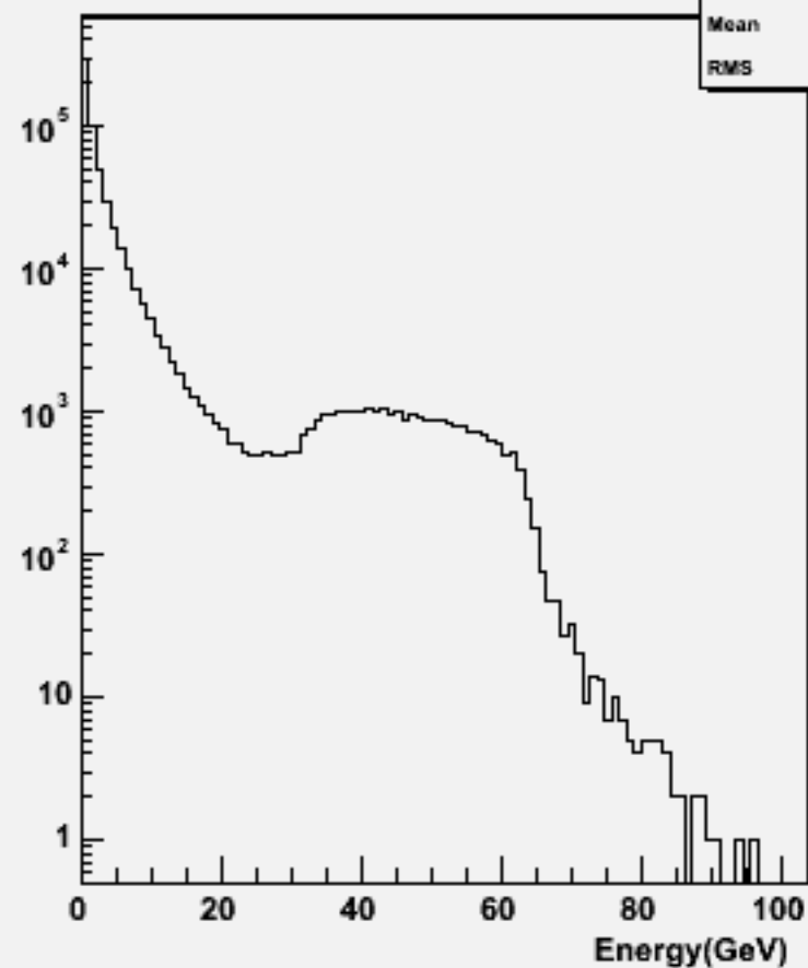
Particle Energy : w104626 e2e2h_o
