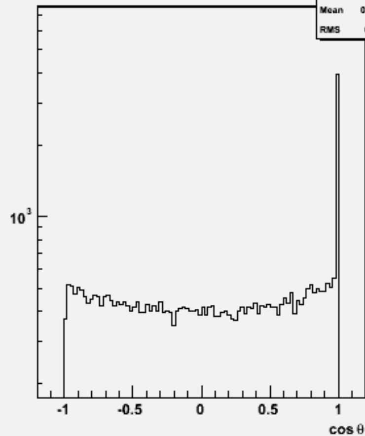
Jet cos \theta (All jets)w104626 e2e2h_o
