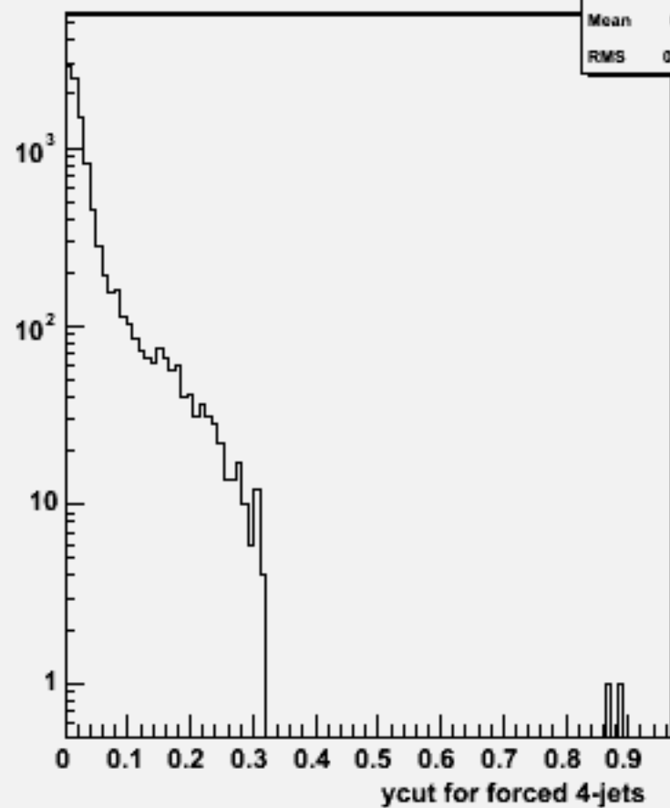
Ycut for 4-jets :w104625 e2e2h_o
