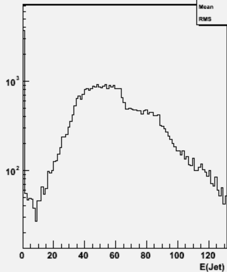
Jet energies(All jets)w104625 e2e2h_o
