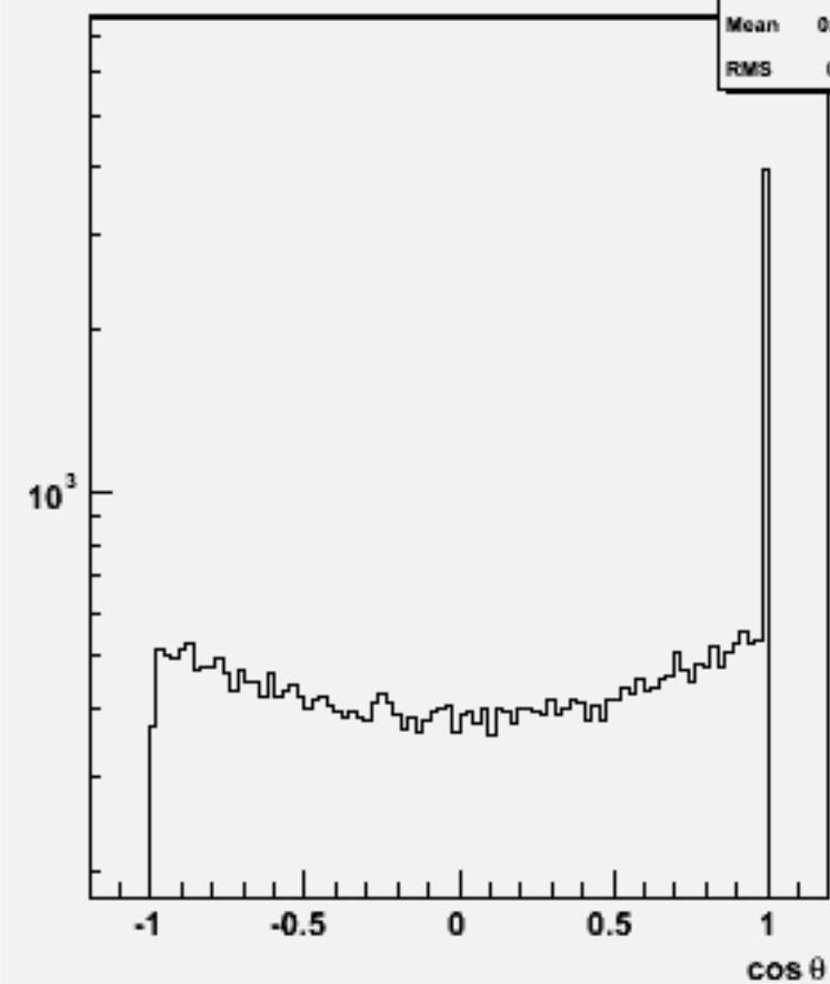
Jet cos \theta (All jets)w104625 e2e2h_o
