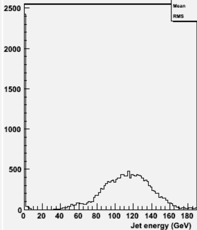
energy for 2-jets :w104625 e2e2h_o
