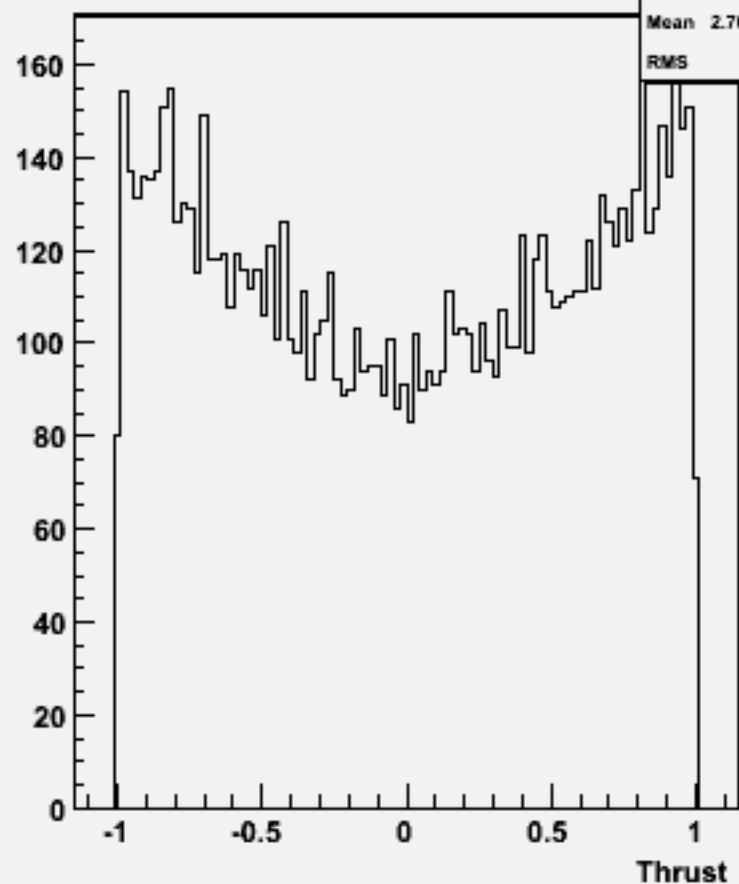
cos \Theta (thrust) w104625 e2e2h_o
