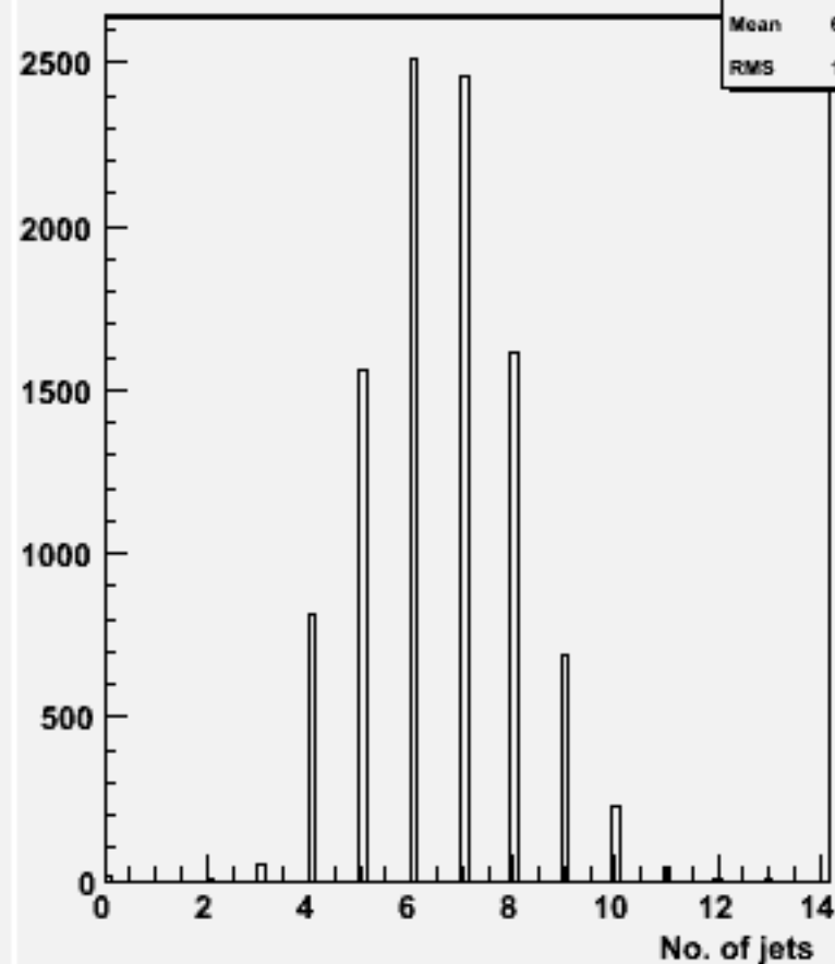
No. jets (ycut=0.001) : w104625 e2e2h_o
