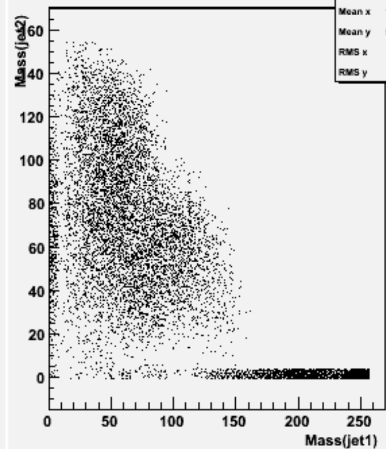
Jet mass for forced 2-jets : w104625 e2e2h_o
