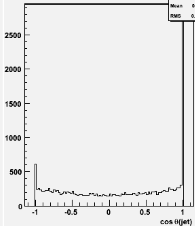
cos \theta for 2-jets :w104625 e2e2h_o
