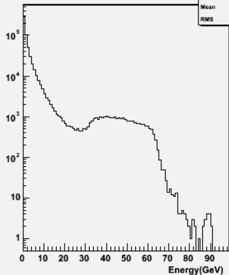
Particle Energy : w104625 e2e2h_o
