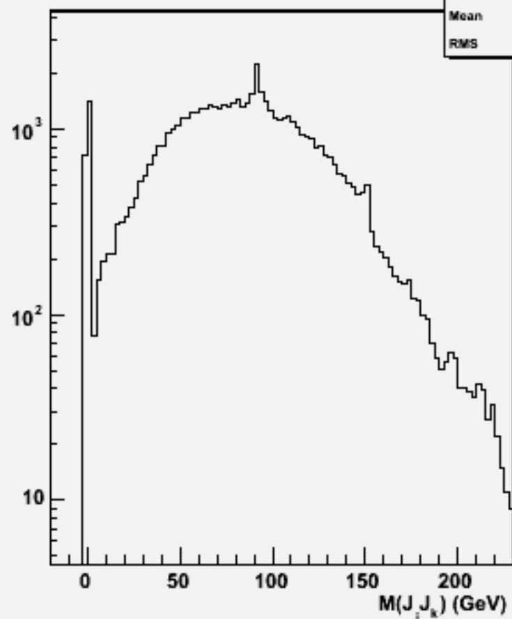
2jets mass(All comb)w104625 e2e2h_o
