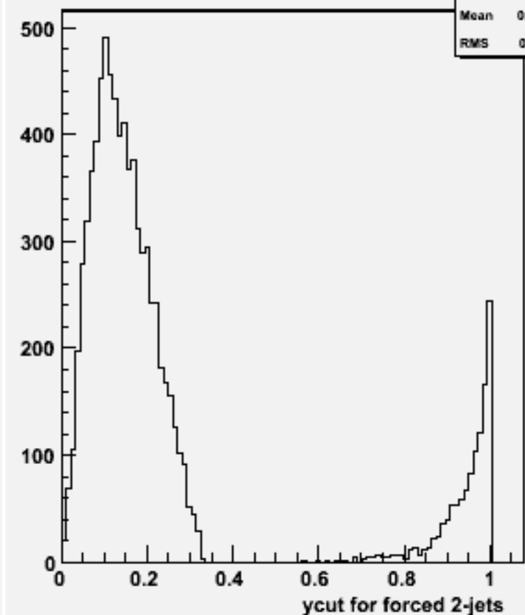
Ycut for 2-jets :w104625 e2e2h_o
