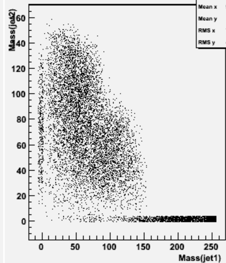
Jet mass for forced 2-jets : w104623 e1e1h_o
