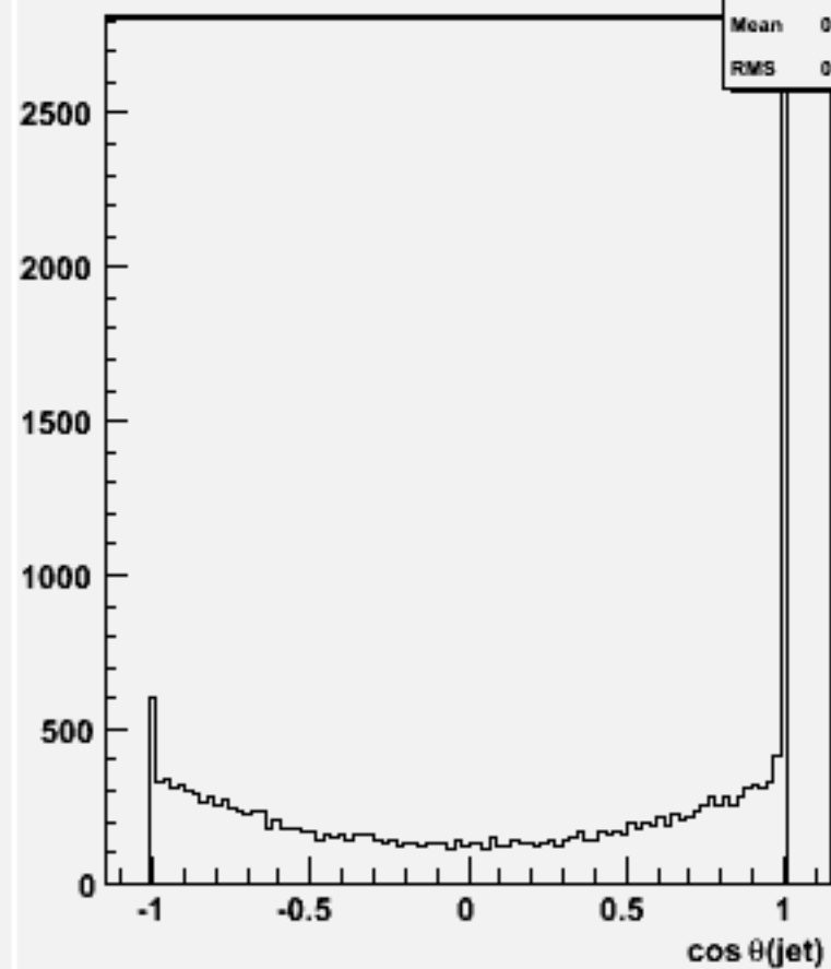
cos \theta for 2-jets :w104623 e1e1h_o
