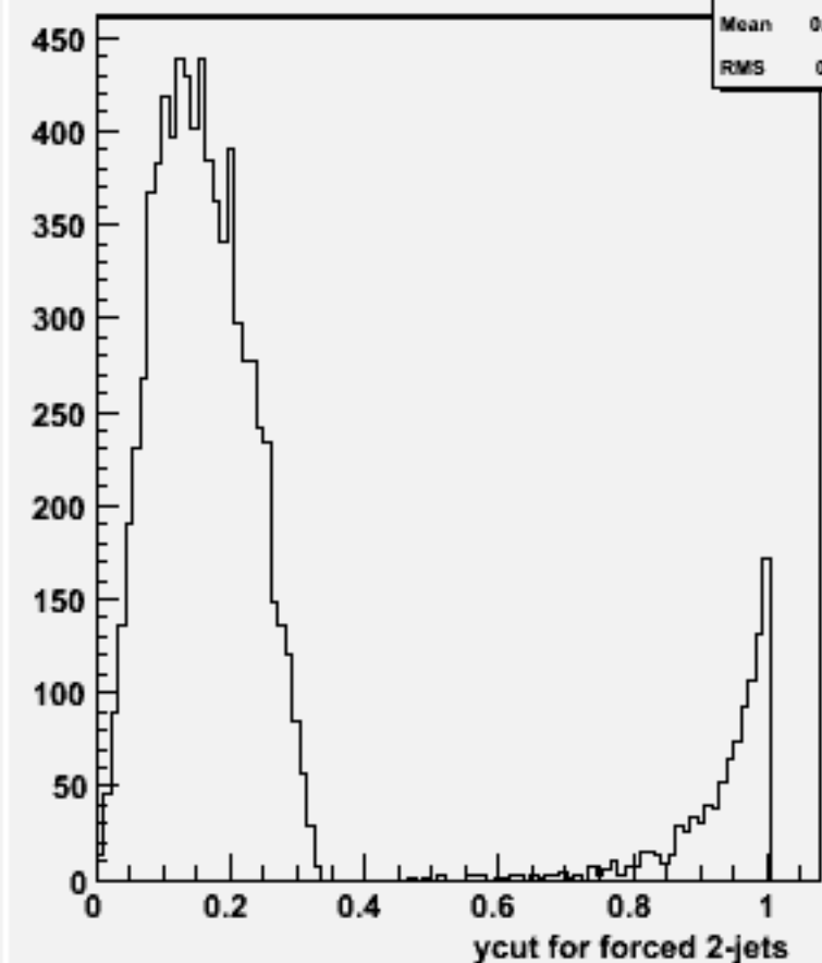
Ycut for 2-jets :w104623 e1e1h_o
