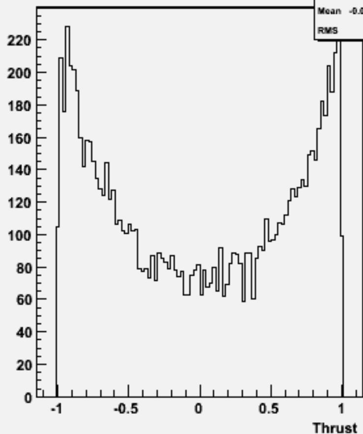
cos \Theta (thrust) w104623 e1e1h_o
