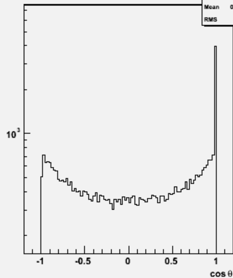
Jet cos \theta (All jets)w104623 e1e1h_o
