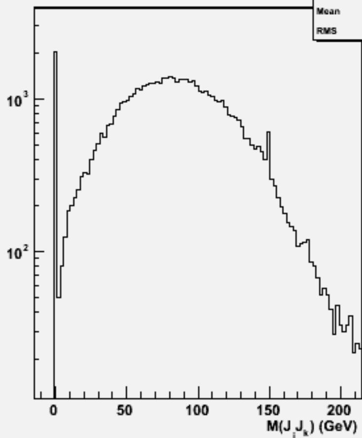
2jets mass(All comb)w104623 e1e1h_o
