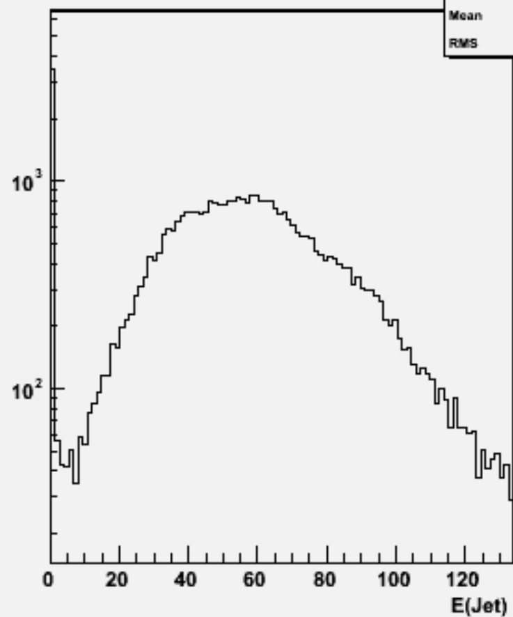
Jet energies(All jets)w104623 e1e1h_o
