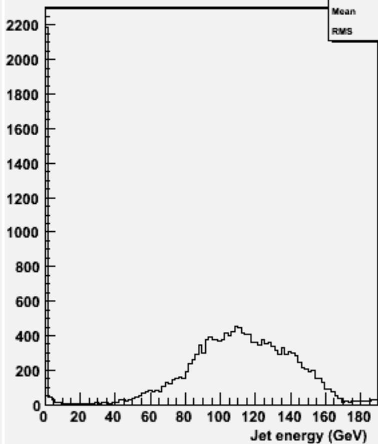
energy for 2-jets :w104623 e1e1h_o
