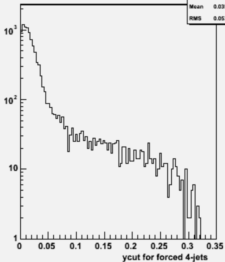
Ycut for 4-jets :w104623 e1e1h_o
