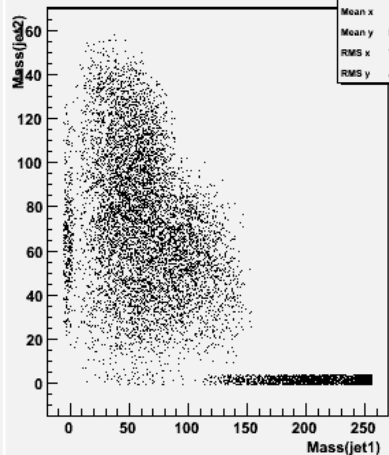
Jet mass for forced 2-jets : w104621 e1e1h_o
