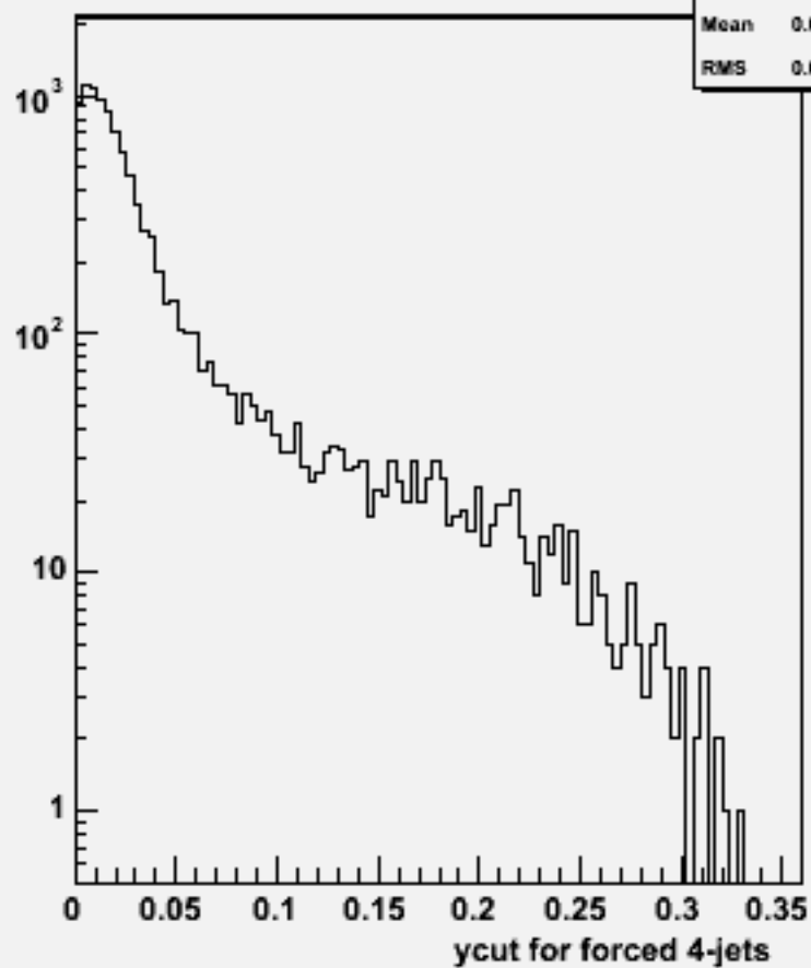
Ycut for 4-jets :w104621 e1e1h_o
