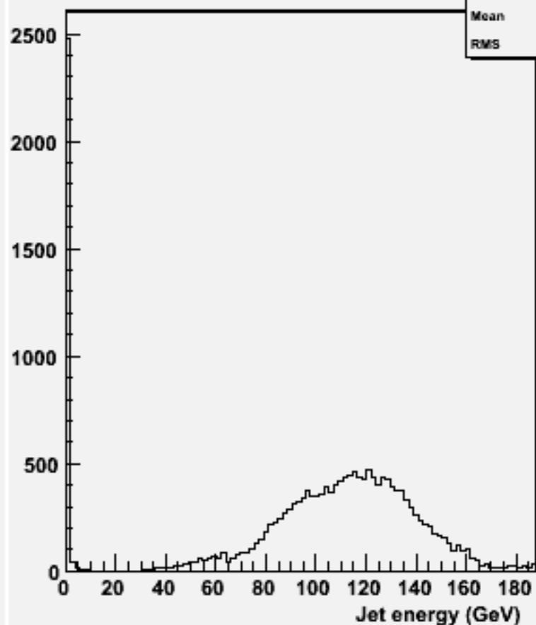
energy for 2-jets :w104621 e1e1h_o
