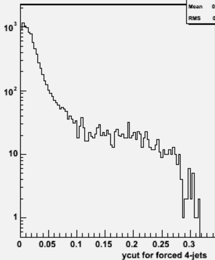
Ycut for 4-jets :w104620 e1e1h_o
