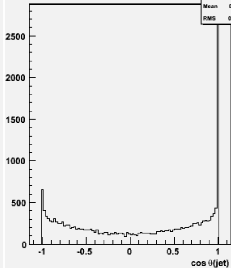
cos \theta for 2-jets :w104620 e1e1h_o
