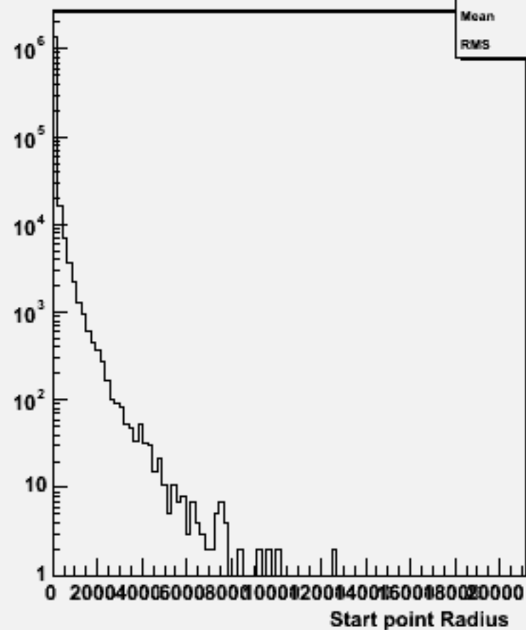
Start point R : w104618 cch_o
