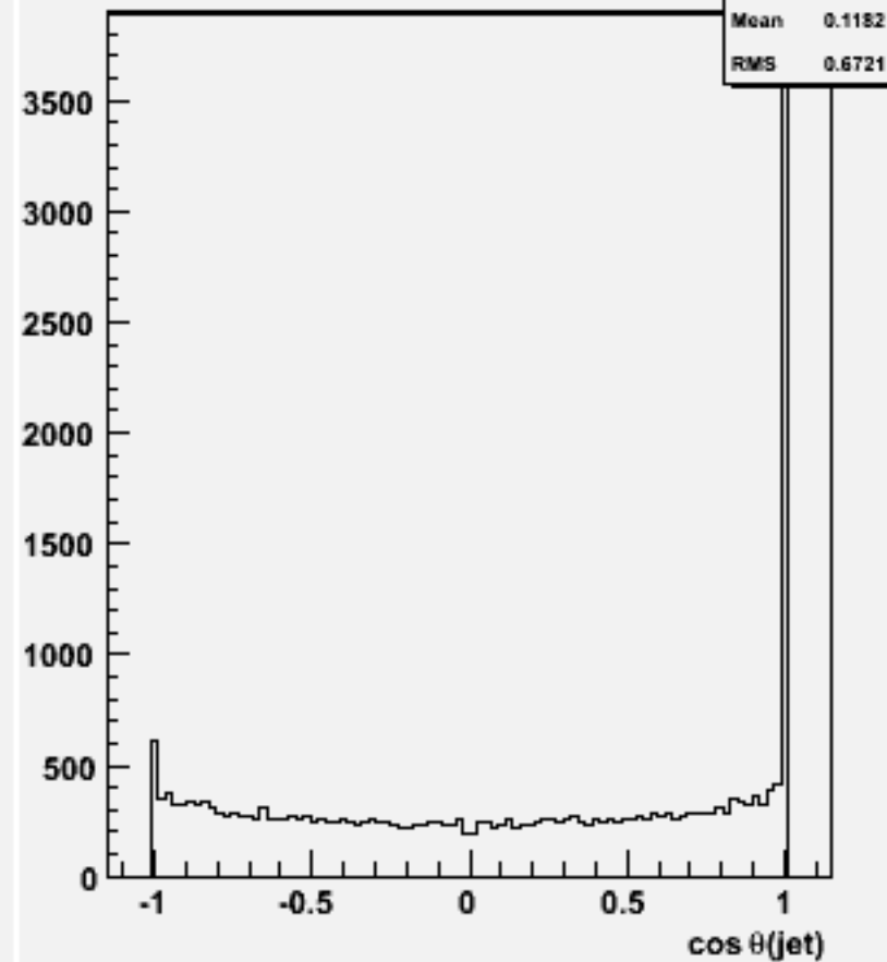
cos \Theta for 2-jets :w104618 cch_o
