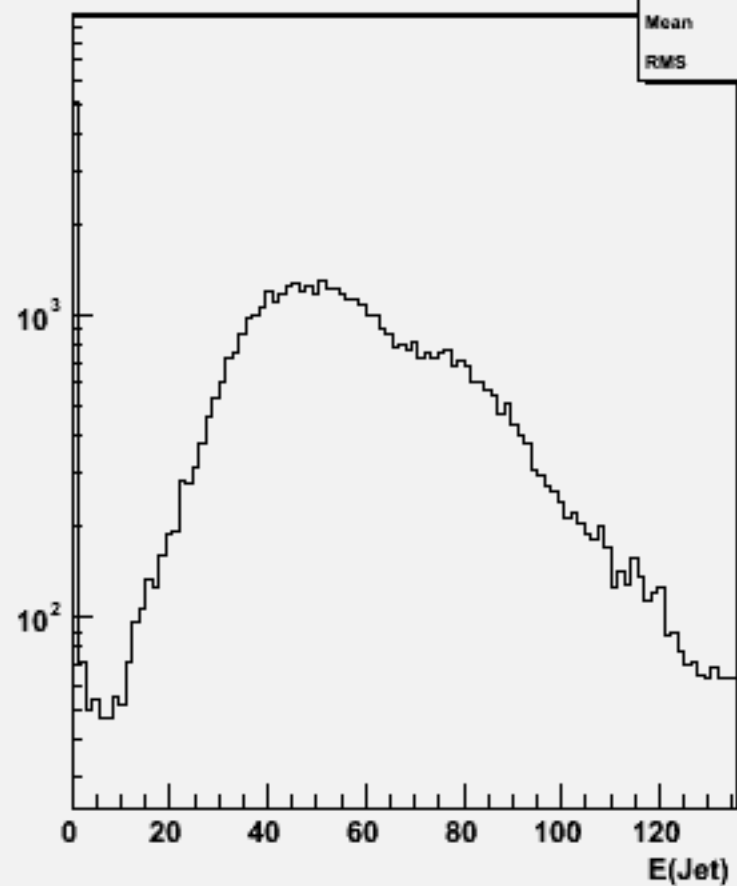
Jet energies(All jets)w104618 cch_o
