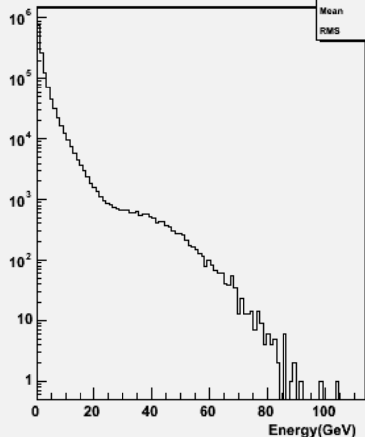
Start point R : w104618 cch_o
