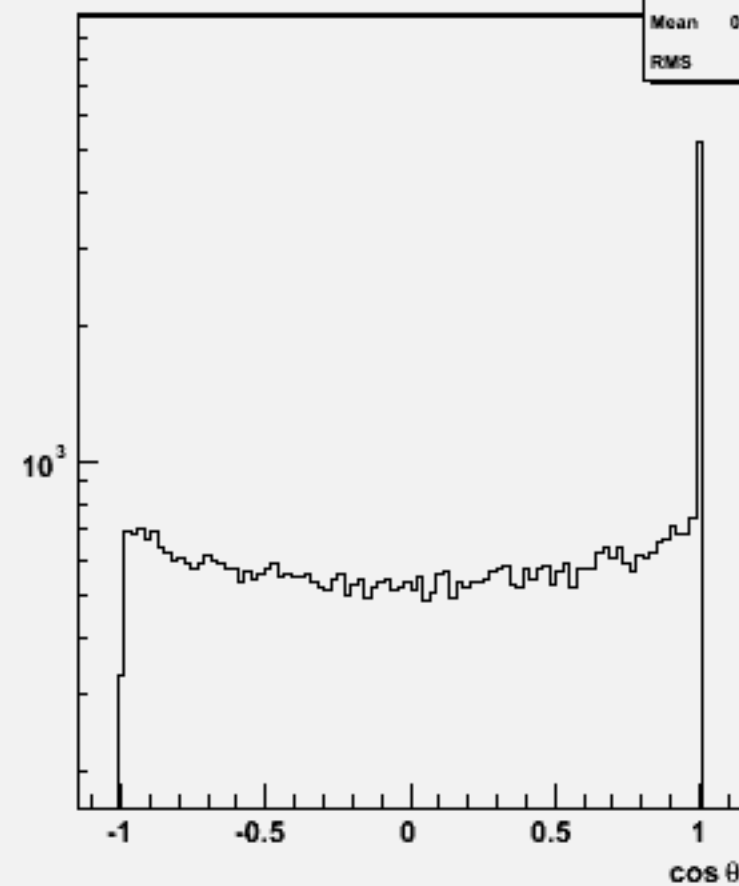
Jet cos \theta (All jets)w104618 cch_o
