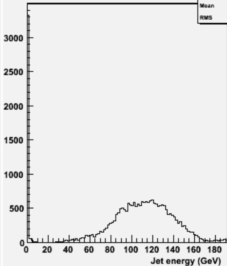
energy for 2-jets :w104618 cch_o
