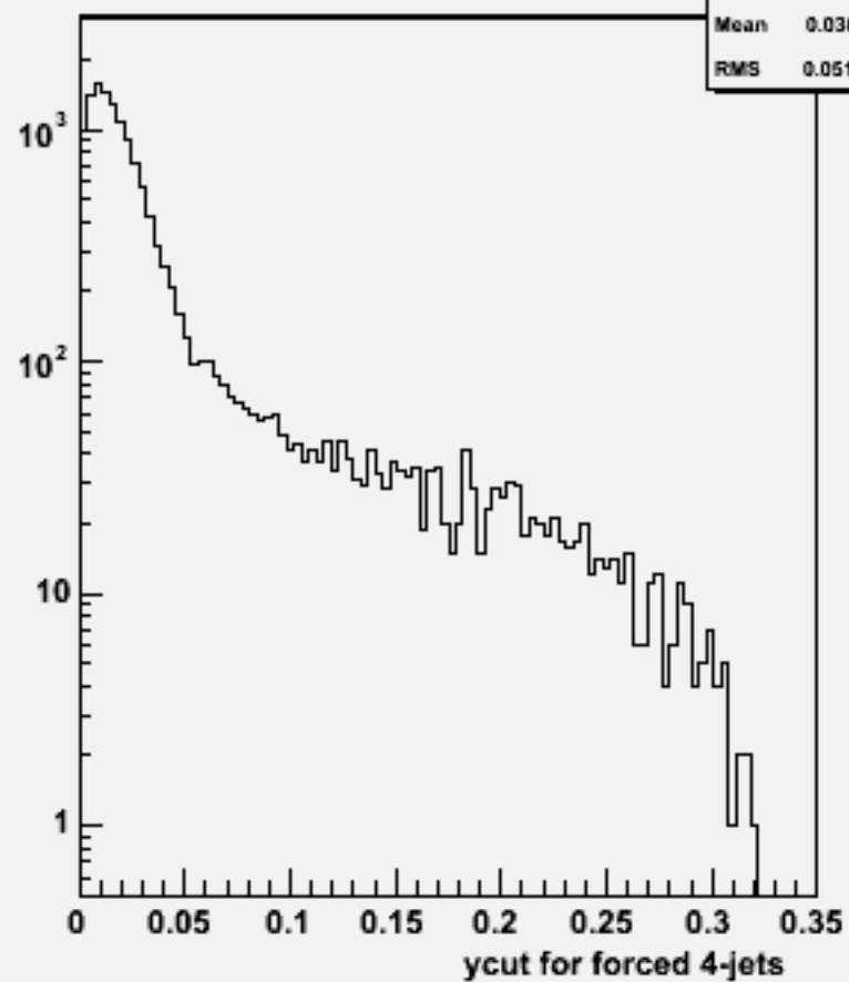
Ycut for 4-jets :w104618 cch_o
