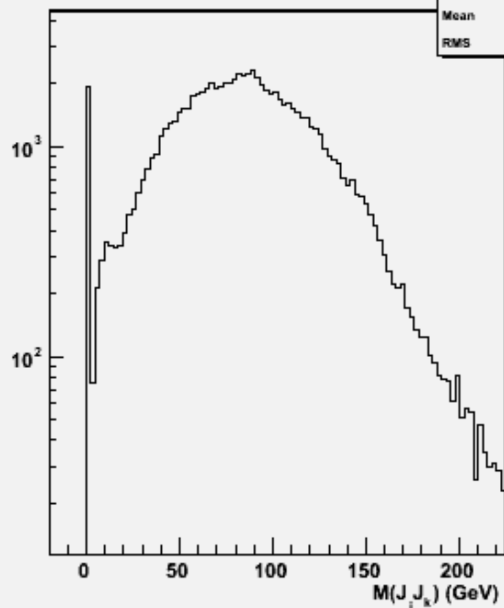
2jets mass(All comb)w104618 cch_o
