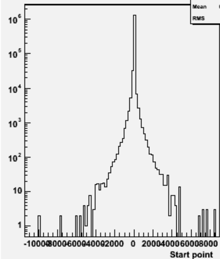
Start point Z : w104618 cch_o
