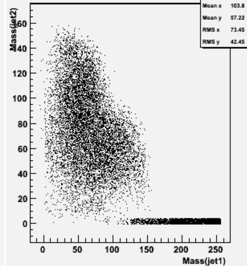
Jet mass for forced 2-jets : w104618 cch_o
