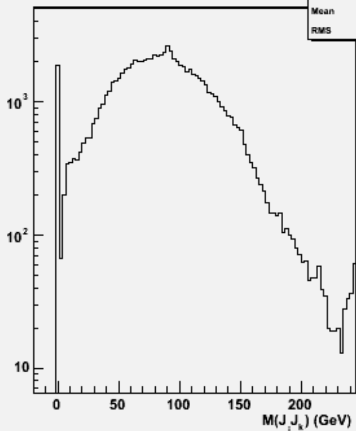
2jets mass(All comb)w104614 uuh_o
