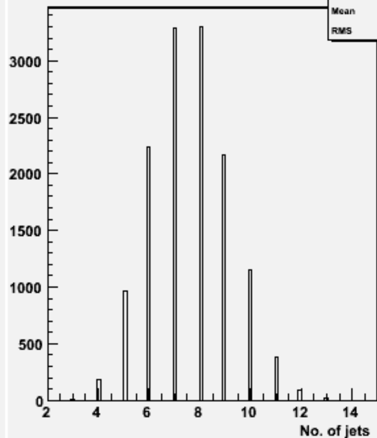
No. jets (ycut=0.001) : w104614 uuh_o
