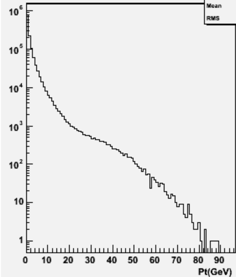
Start point Z : w104614 uuh_o
