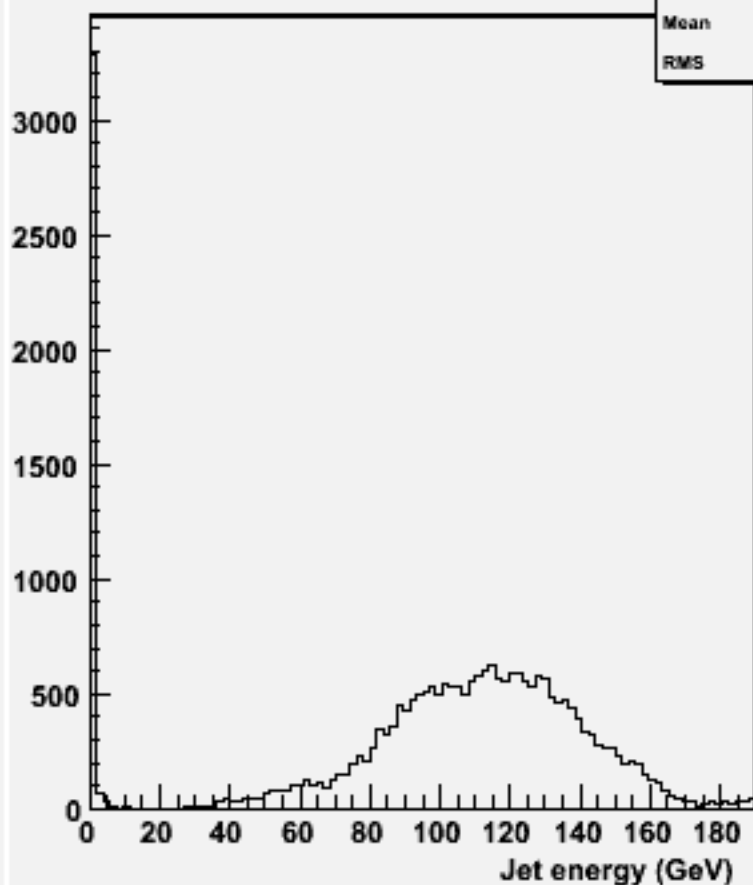
energy for 2-jets :w104614 uuh_o
