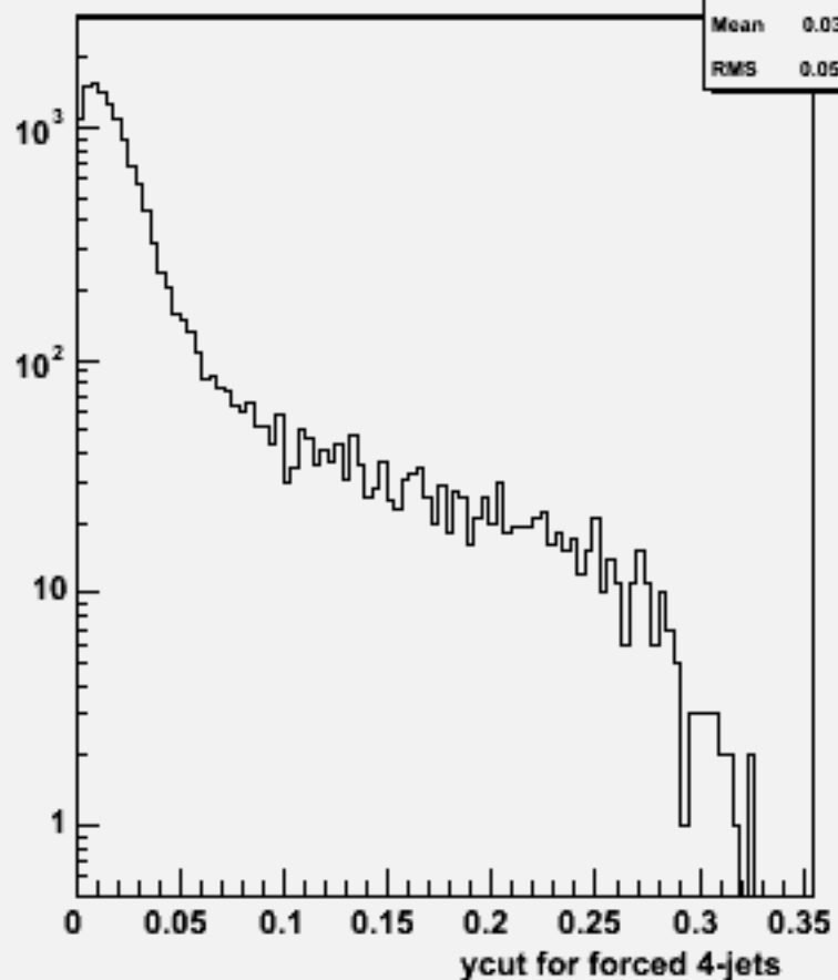
Ycut for 4-jets :w104614 uuh_o
