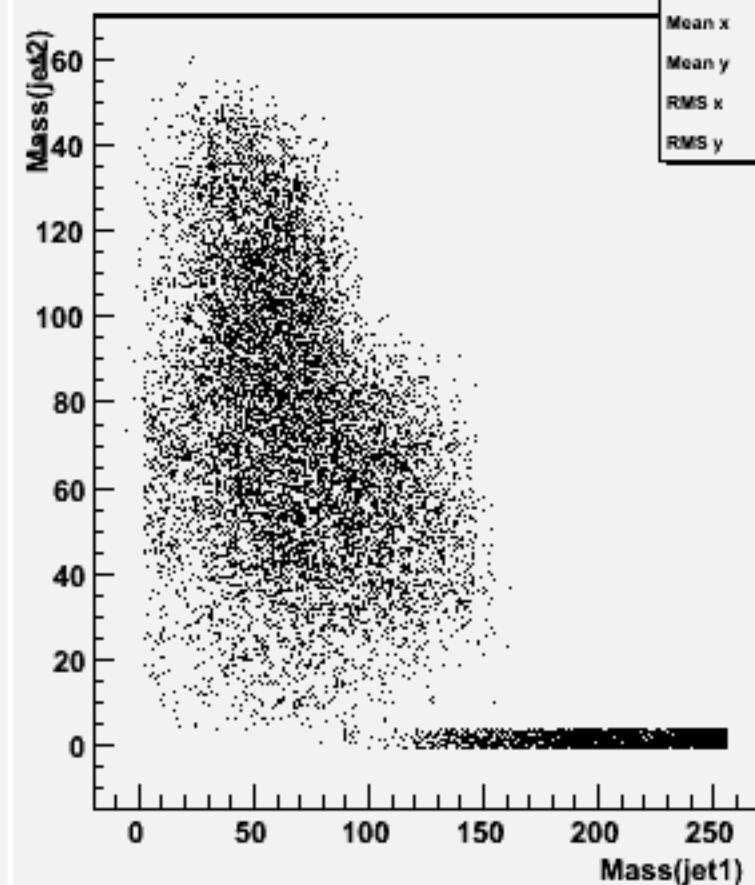
Jet mass for forced 2-jets : w104614 uuh_o
