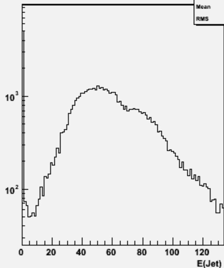
Jet energies(All jets)w104614 uuh_o
