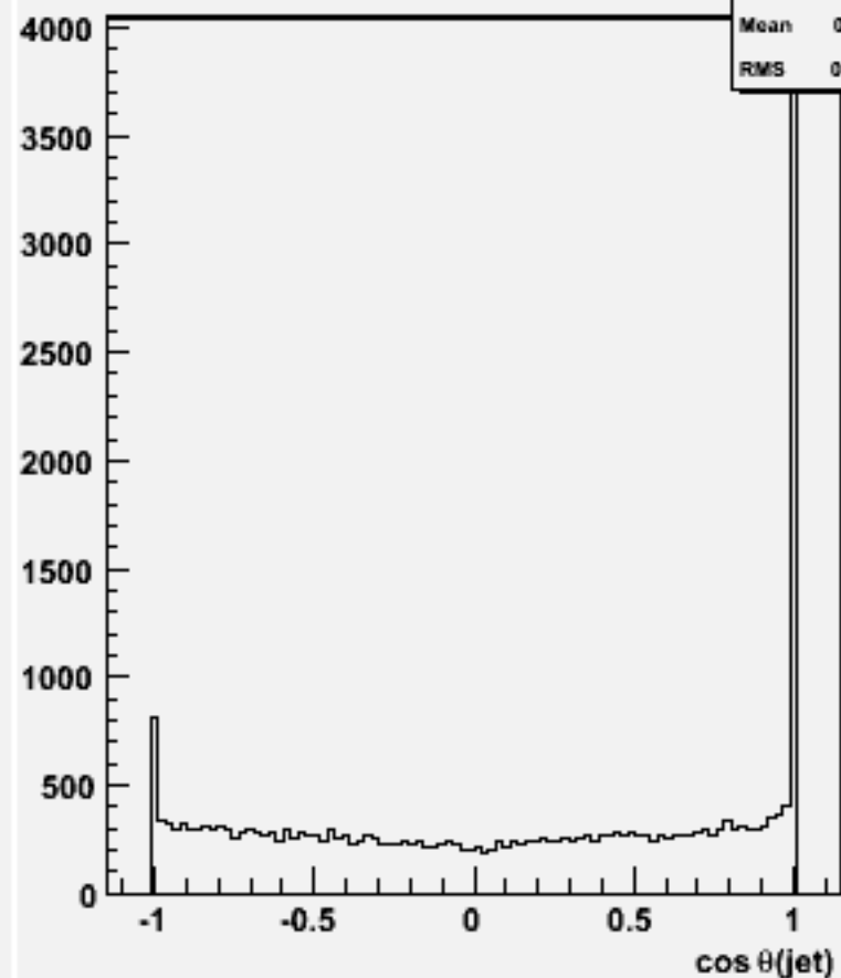
cos \theta for 2-jets :w104614 uuh_o
