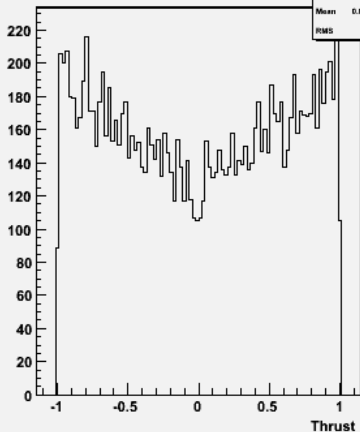
cos \Theta (thrust) w104614 uuh_o
