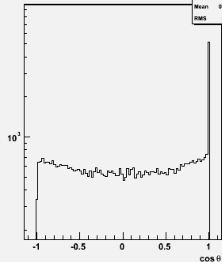
Jet cos \theta (All jets)w104614 uuh_o
