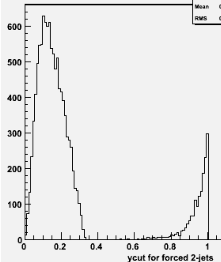
Ycut for 2-jets :w104614 uuh_o
