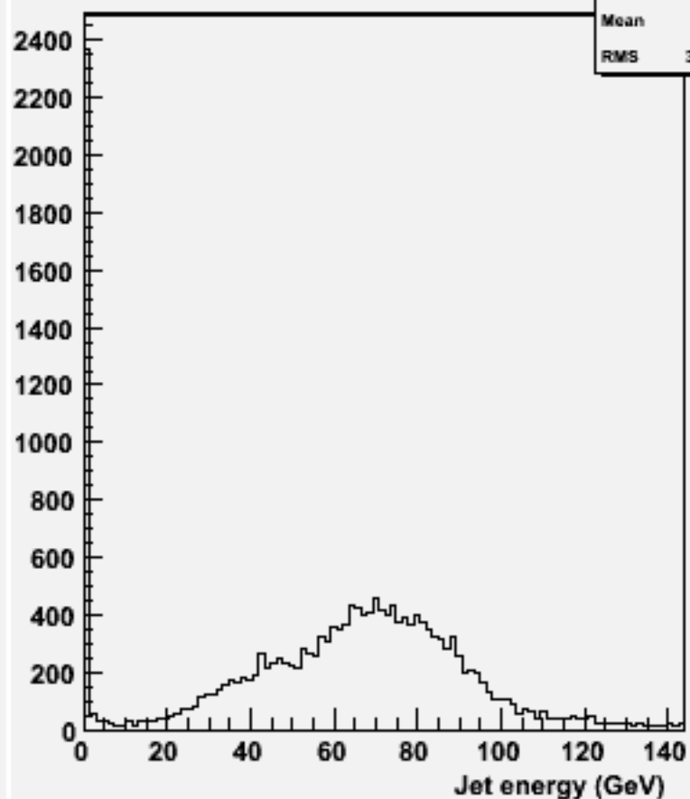
energy for 2-jets :w104610 n3n3h_o
