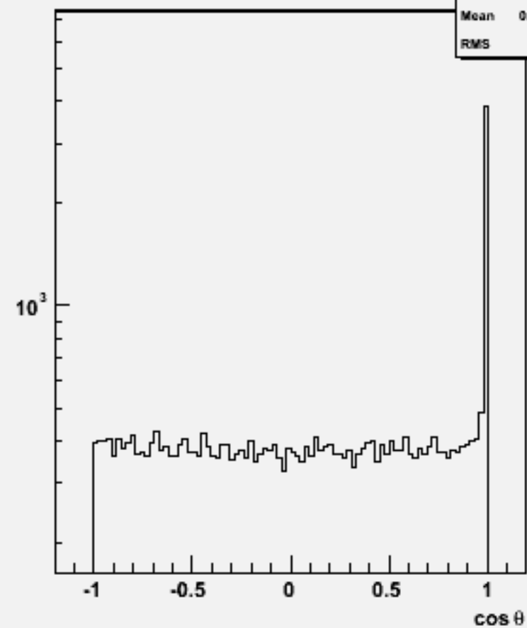
Jet cos \theta (All jets)w104610 n3n3h_o
