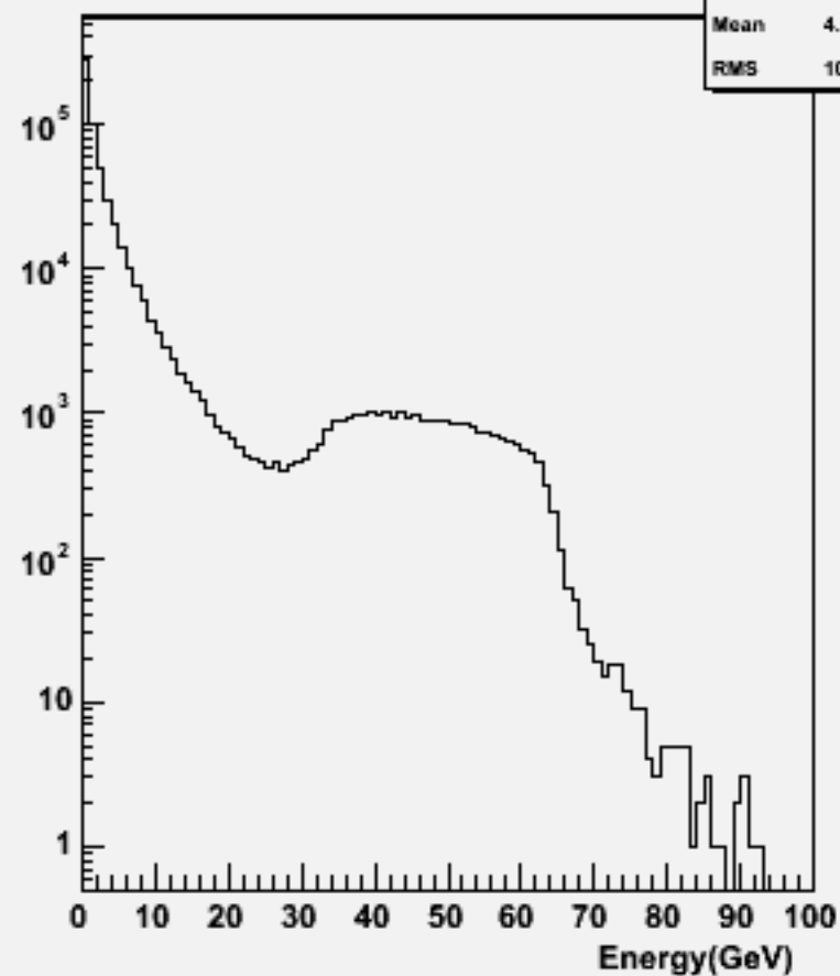
Particle Energy : w104610 n3n3h_o
