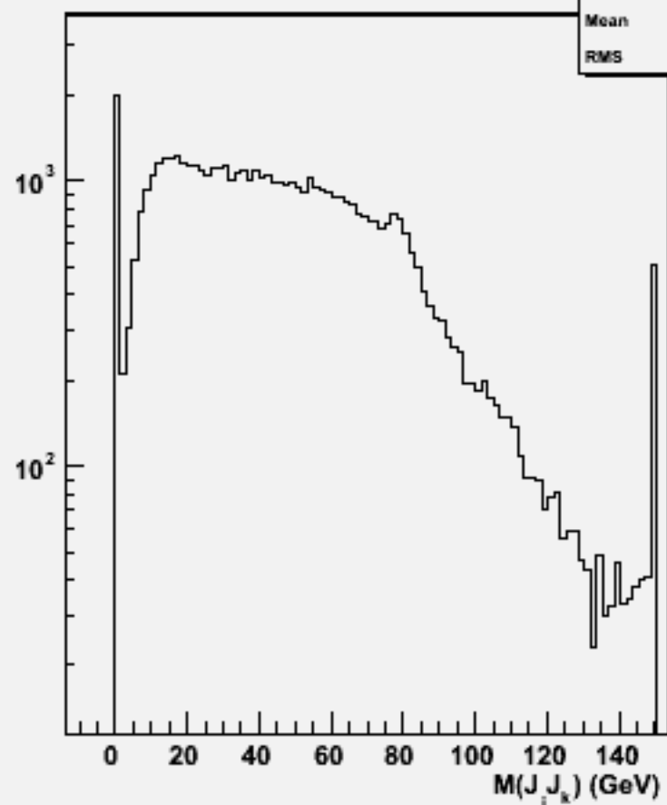
2jets mass(All comb)w104610 n3n3h_o
