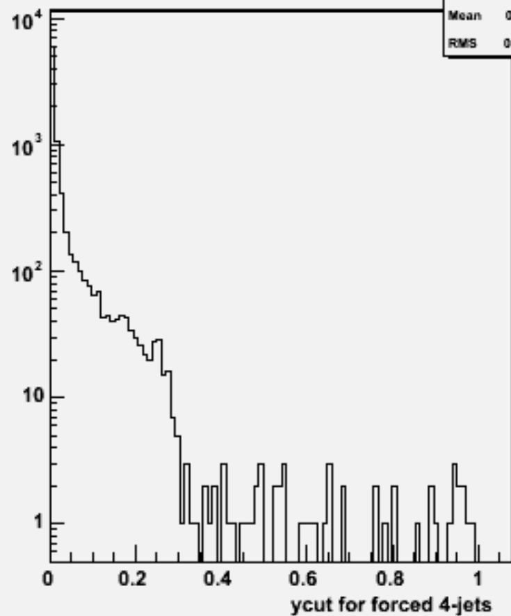
Ycut for 4-jets :w104610 n3n3h_o
