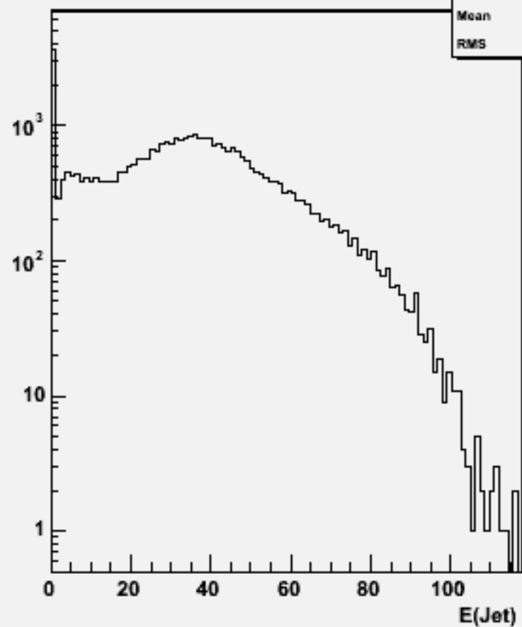
Jet energies(All jets)w104610 n3n3h_o
