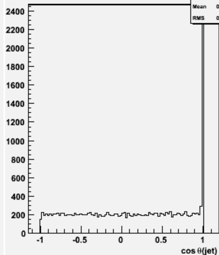
cos \theta for 2-jets :w104610 n3n3h_o
