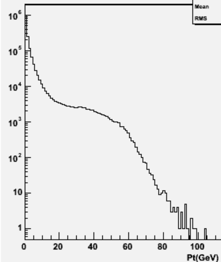
Particle Pt : w104601 n1n1h_o
