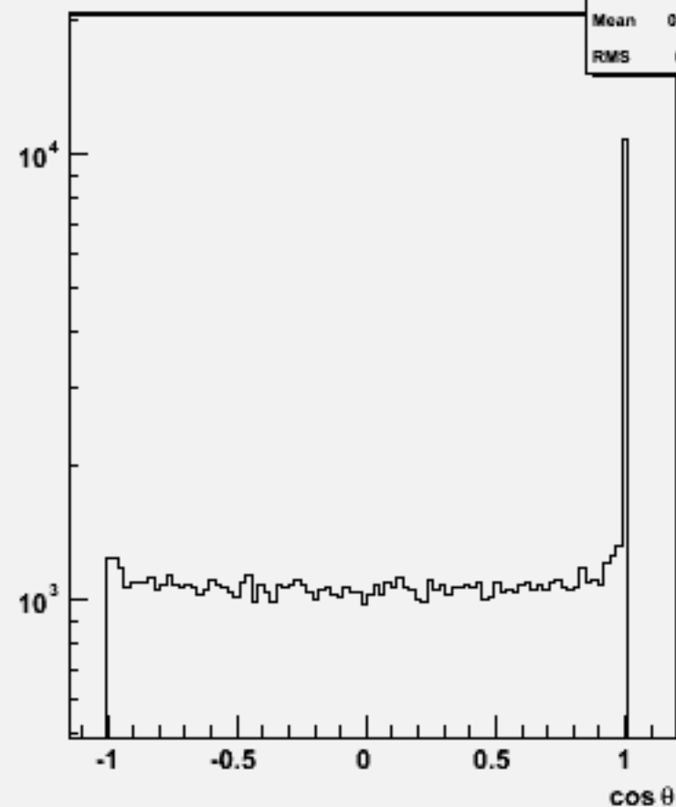
Jet cos \theta (All jets)w104601 n1n1h_o
