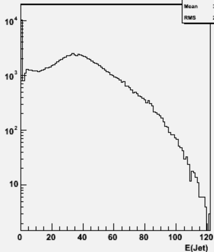
Jet energies(All jets)w104601 n1n1h_o
