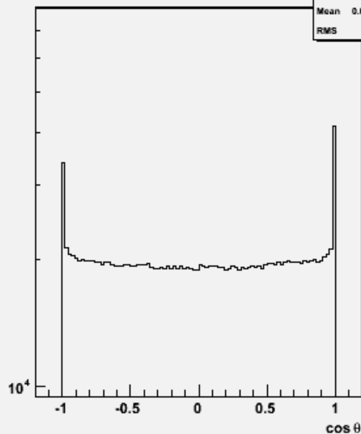
Particle cosθ : w104601 n1n1h_o
