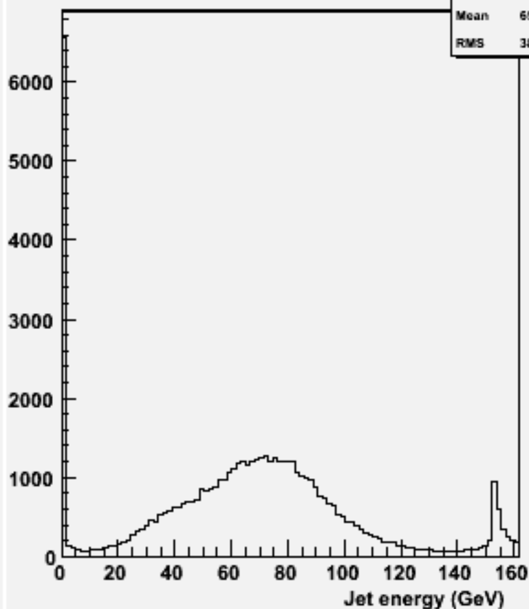
energy for 2-jets :w104601 n1n1h_o
