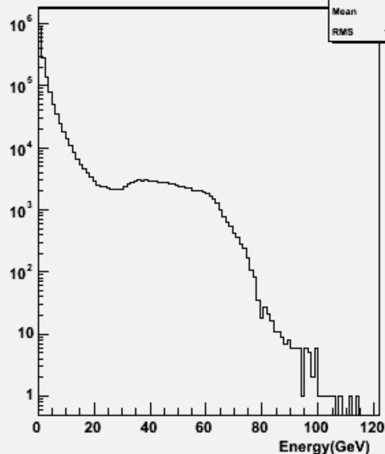
Particle Energy : w104601 n1n1h_o
