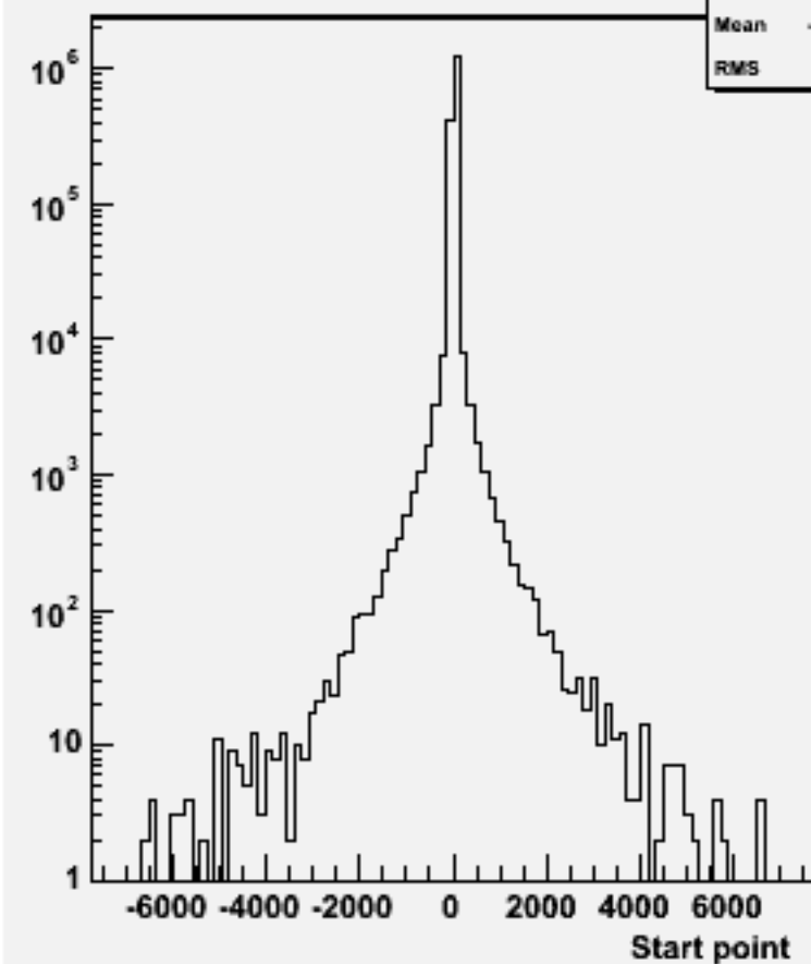
Start point Z : w104601 n1n1h_o
