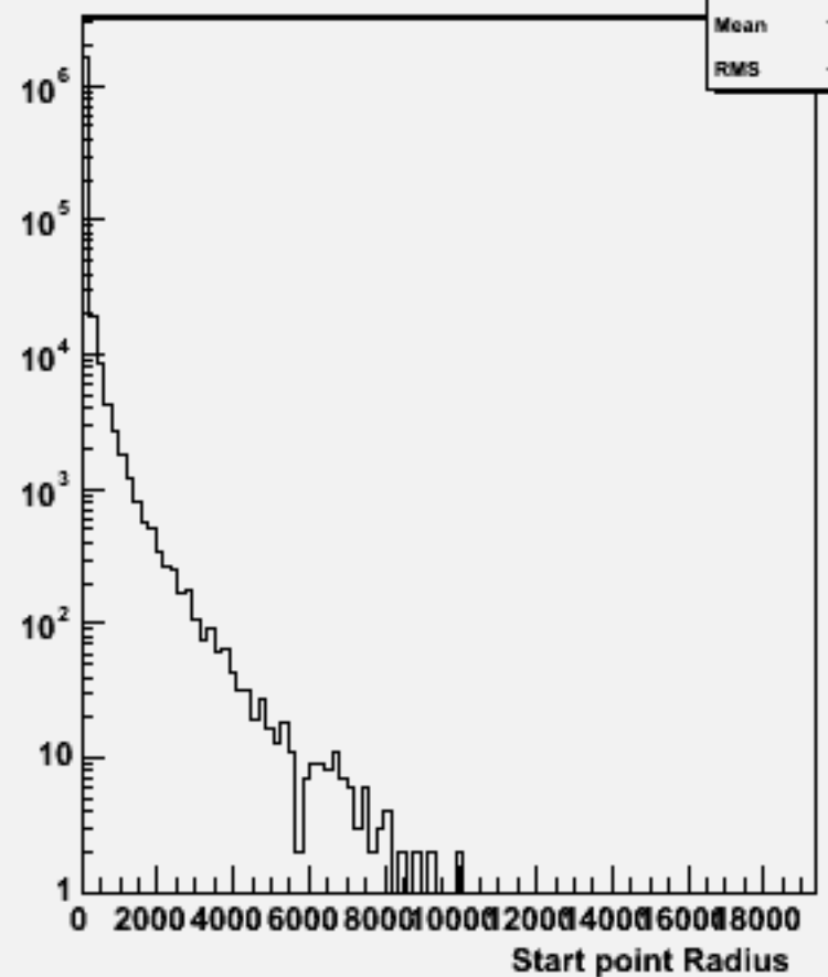
Start point R : w104601 n1n1h_o
