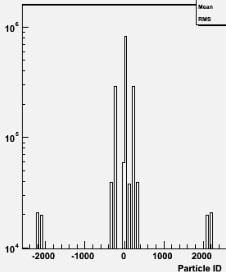
Particle ID : w104601 n1n1h_o
