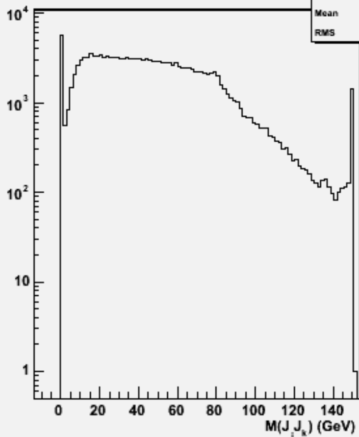
2jets mass(All comb)w104601 n1n1h_o
