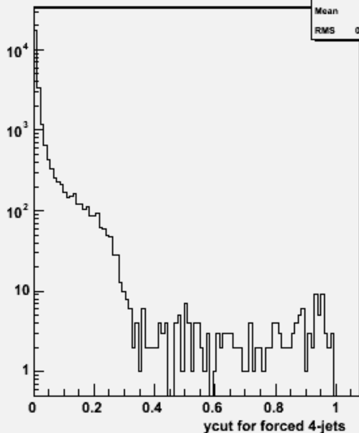
Ycut for 4-jets :w104601 n1n1h_o
