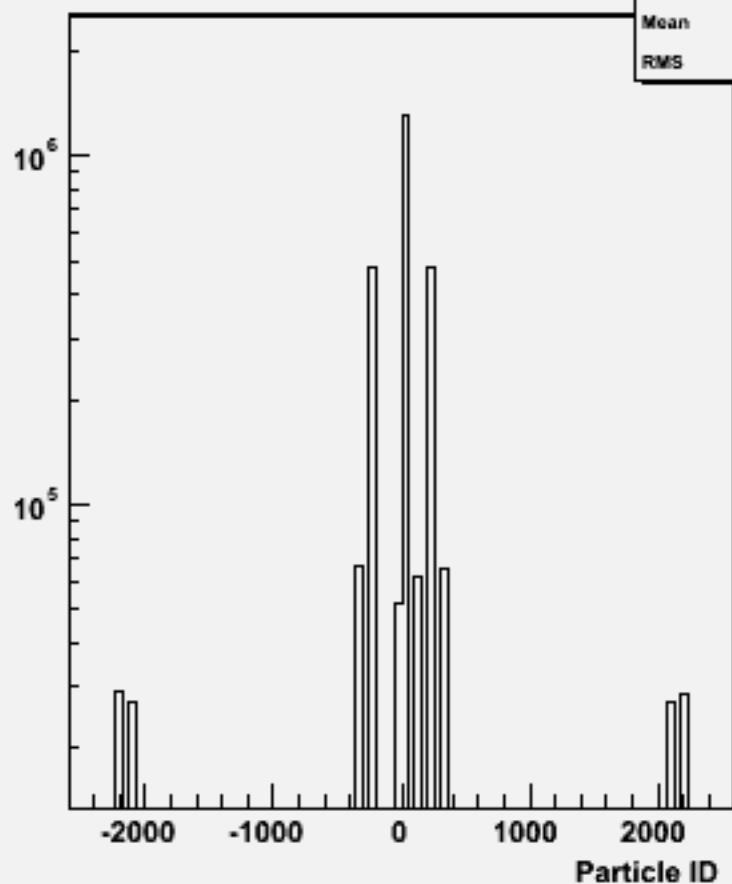
Particle ID : w104592 bbh_o
