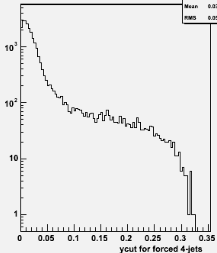
Ycut for 4-jets :w104592 bbh_o
