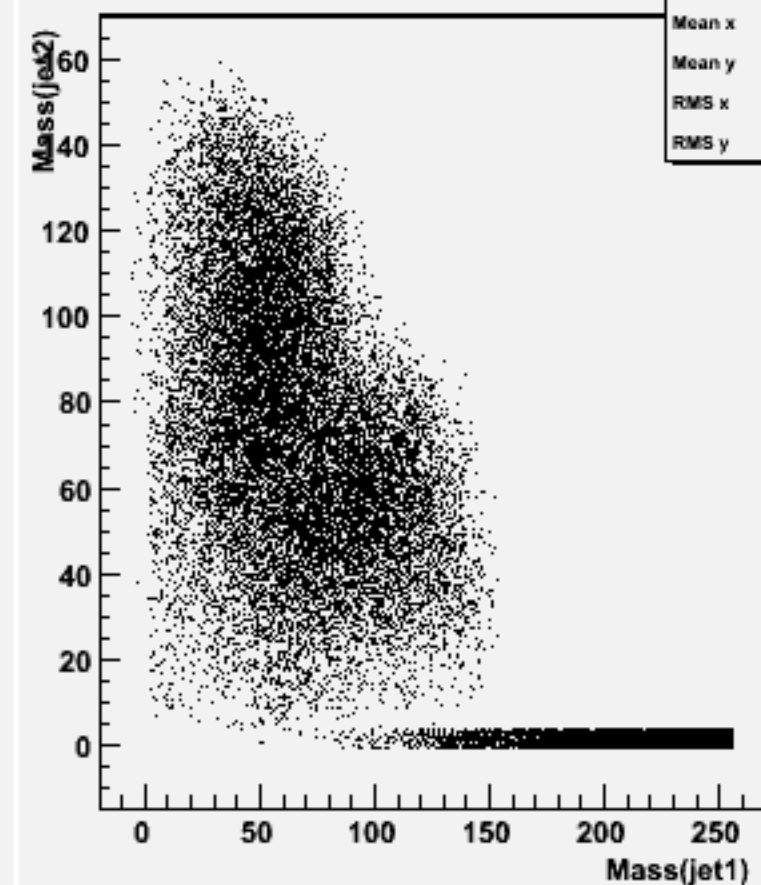
Jet mass for forced 2-jets : w104592 bbh_o
