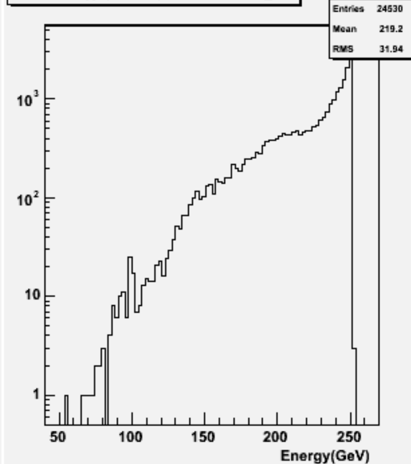
Total Energy (w/o \nu ): w104592 bbh_o
