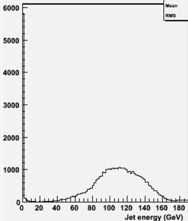
energy for 2-jets :w104592 bbh_o
