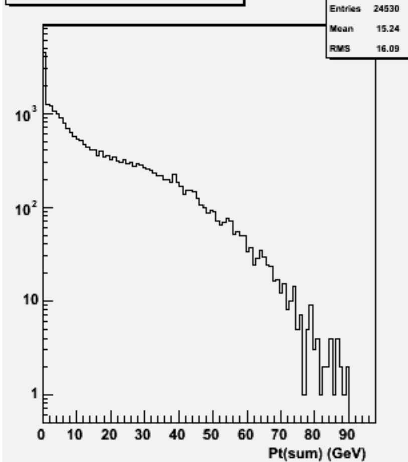
Pt Sum: w104592 bbh_o
