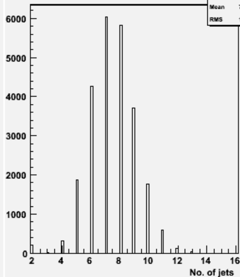
No. jets (ycut=0.001) : w104592 bbh_o
