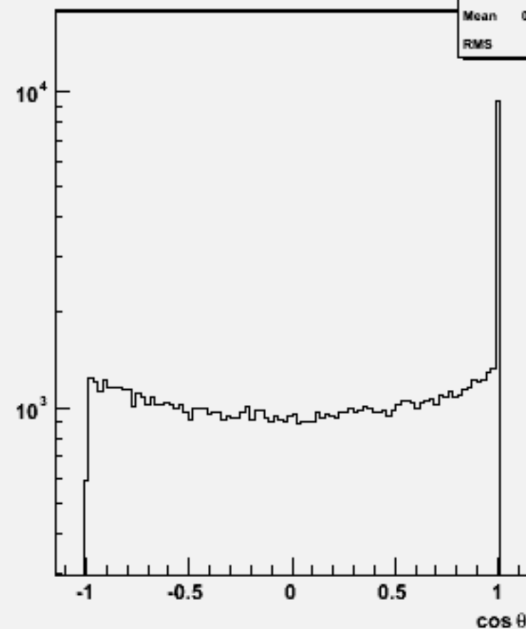
Jet cos \theta (All jets)w104592 bbh_o
