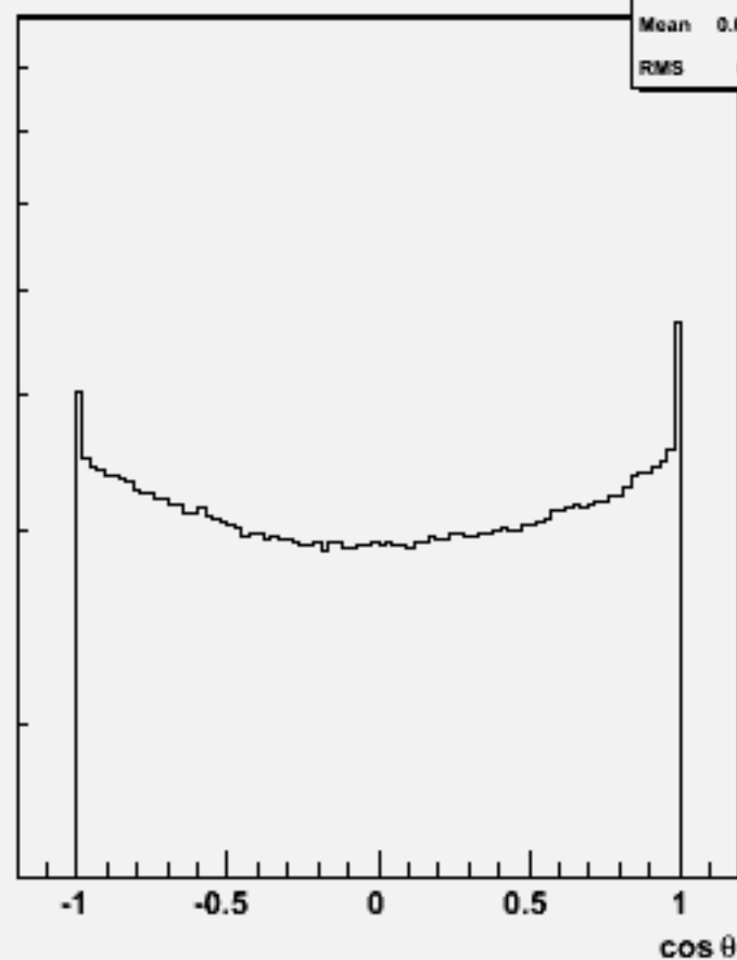
Particle \cos\theta : w104592 bbh_o
