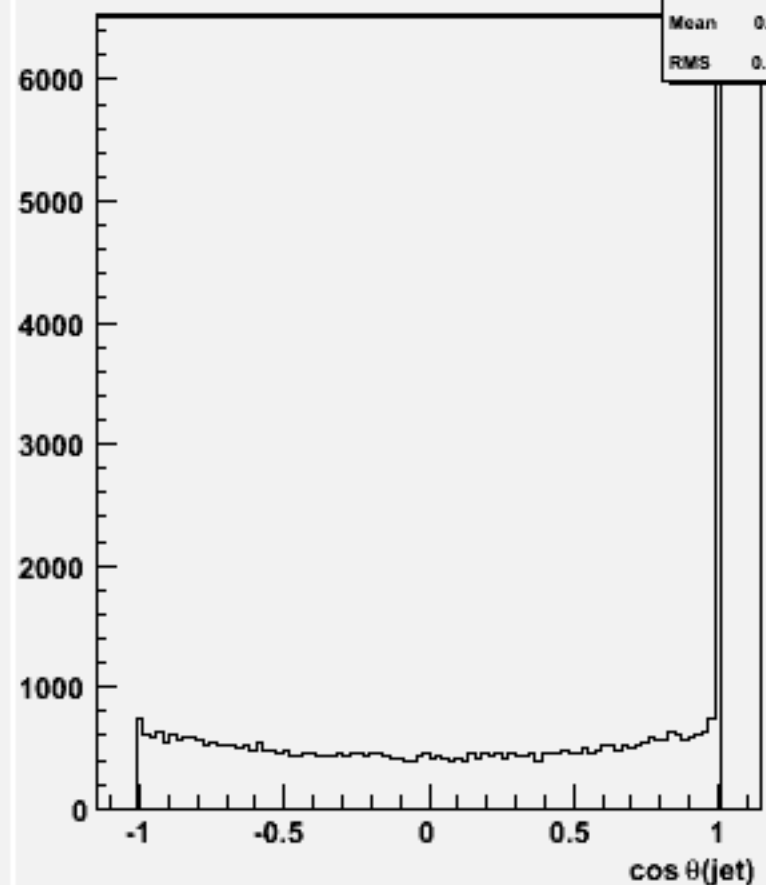
cos \theta for 2-jets :w104592 bbh_o
