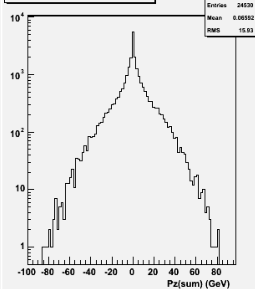
Pz Sum: w104592 bbh_o
