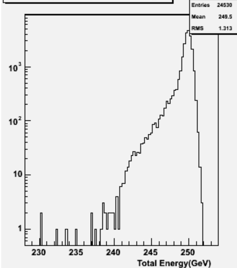
Total Energy (inc. \nu ): w104592 bbh_o
