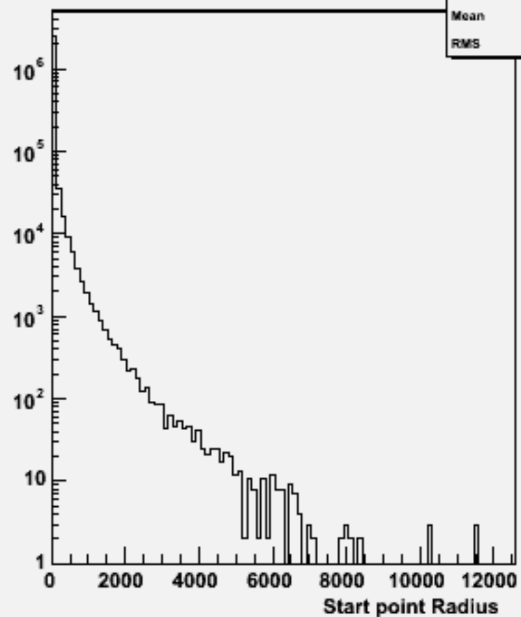
Start point R : w104592 bbh_o
