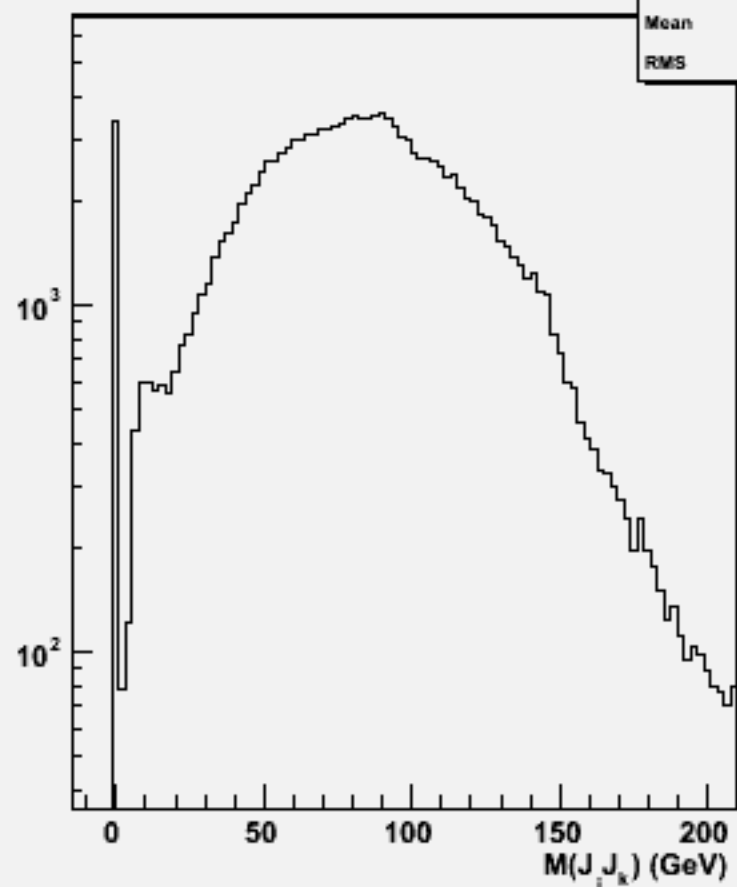
2jets mass(All comb)w104592 bbh_o
