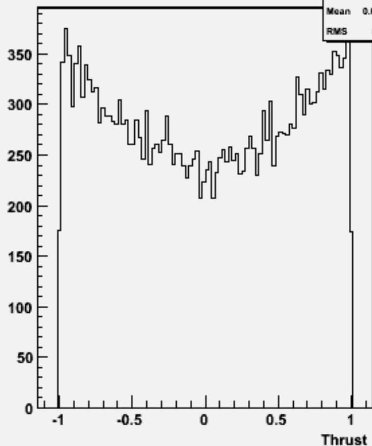
cos \Theta (thrust) w104592 bbh_o
