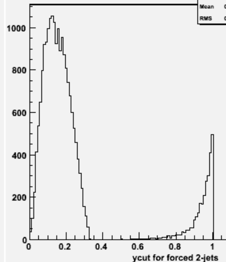
Ycut for 2-jets :w104592 bbh_o
