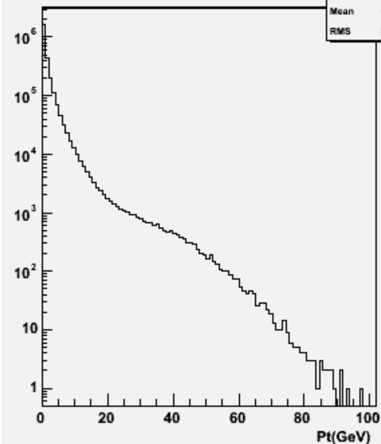
Particle Pt : w104592 bbh_o
