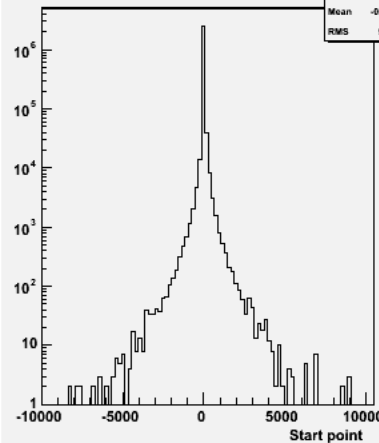
Start point Z : w104592 bbh_o
