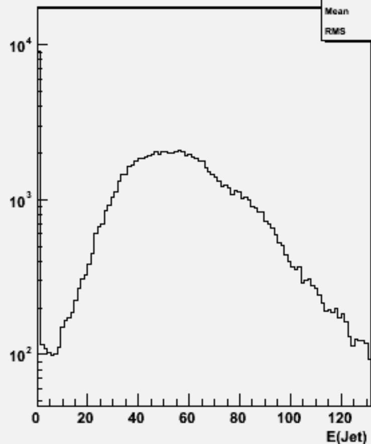
Jet energies(All jets)w104592 bbh_o
