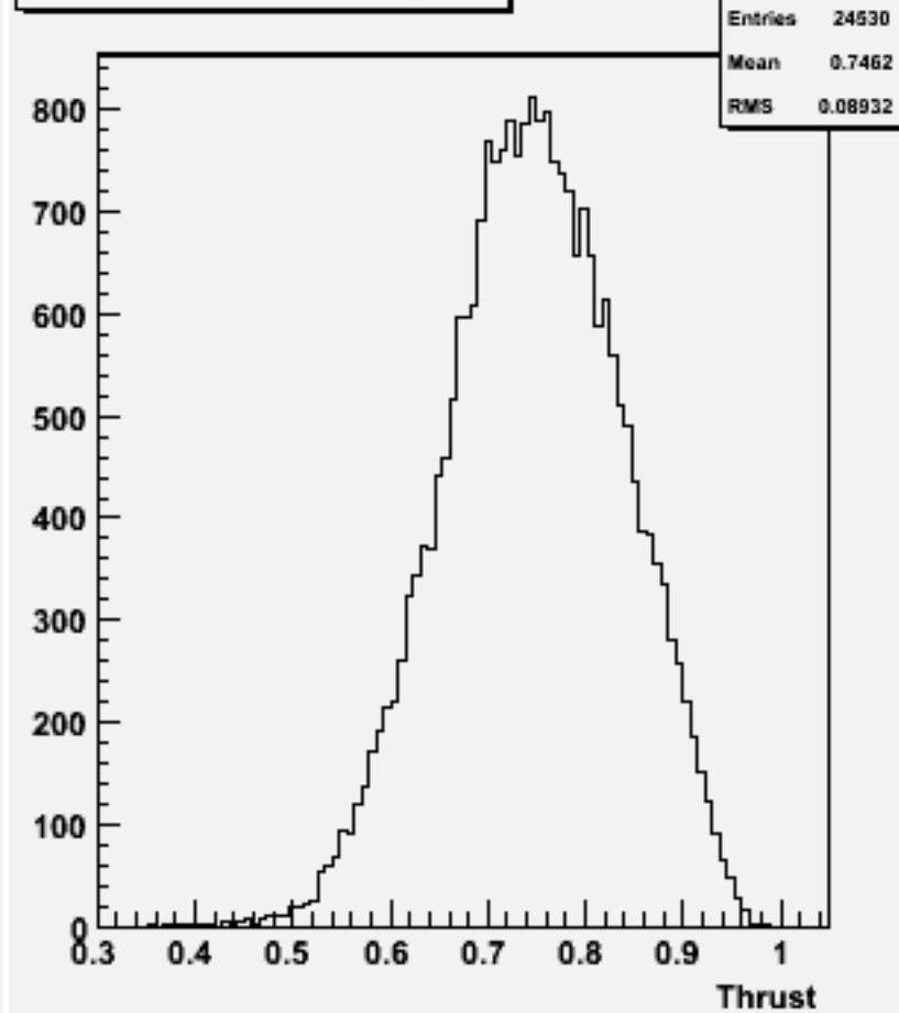
Thrust w104592 bbh_o
