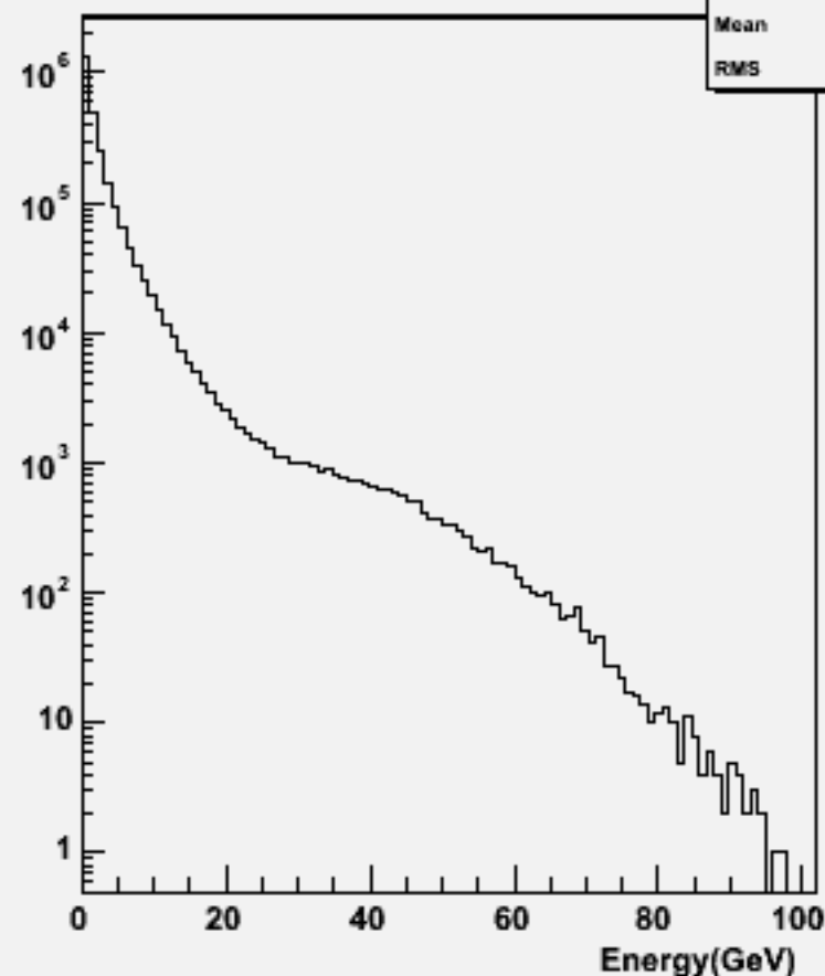
Particle Energy : w104592 bbh_o
