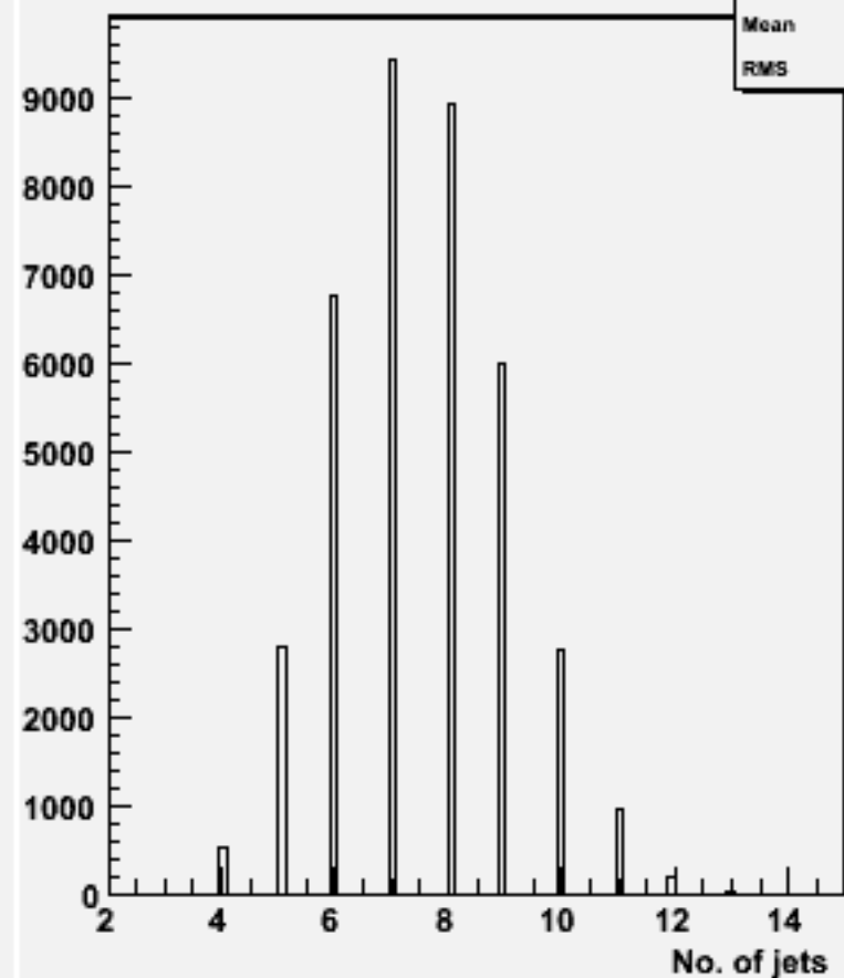
No. jets (ycut=0.001) : w104591 bbh_o
