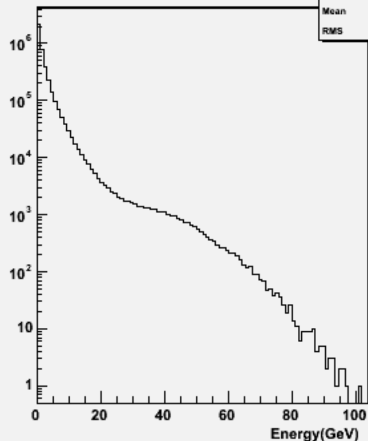
Start point R : w104591 bbh_o
