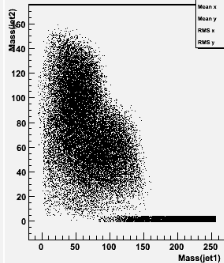
Jet mass for forced 2-jets : w104591 bbh_o
