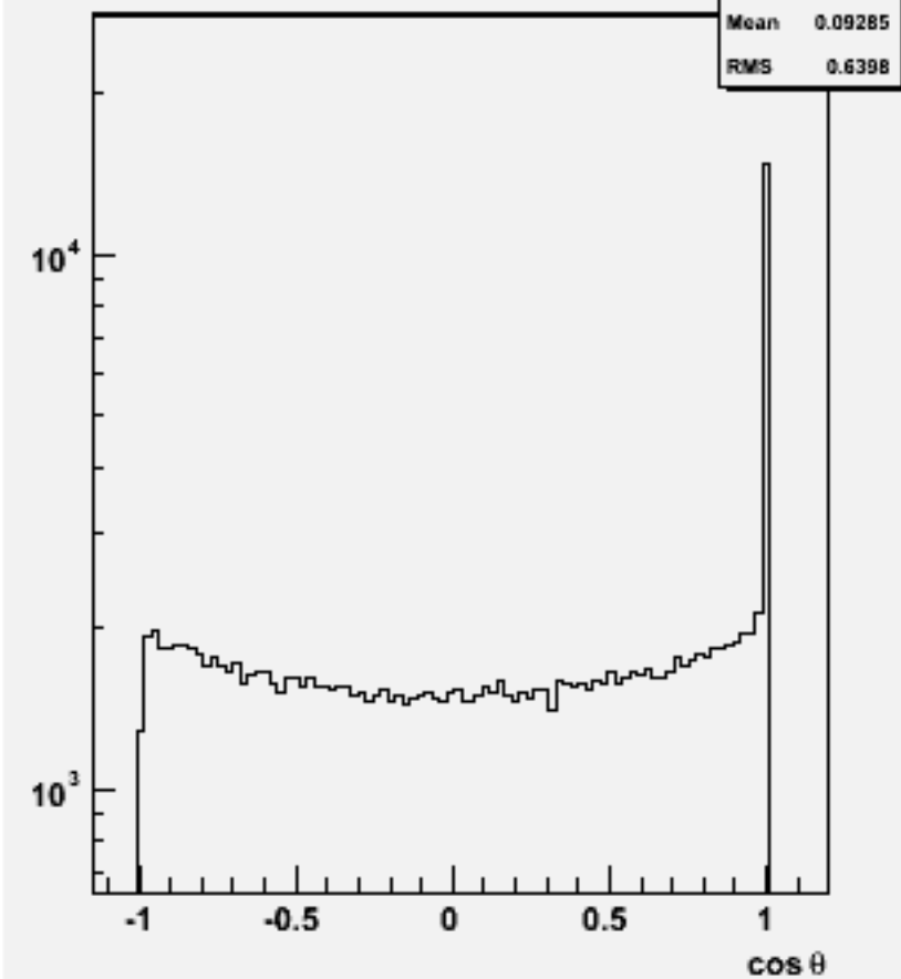
Jet cos \theta (All jets)w104591 bbh_o
