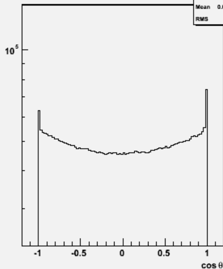
Particle \cos\theta : w104591 bbh_o
