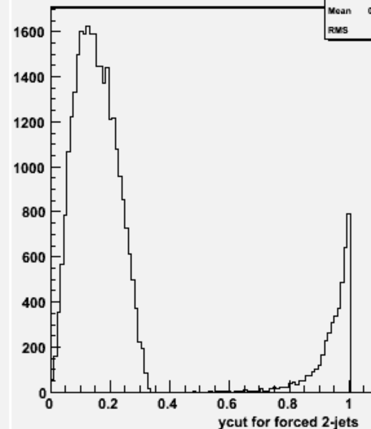
Ycut for 2-jets :w104591 bbh_o
