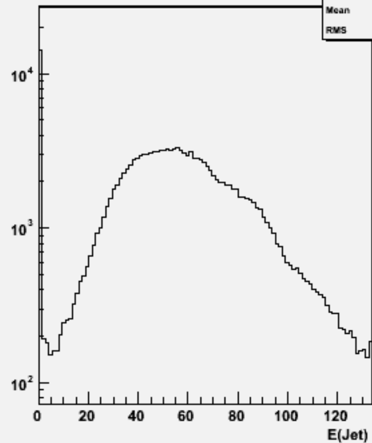
Jet energies(All jets)w104591 bbh_o
