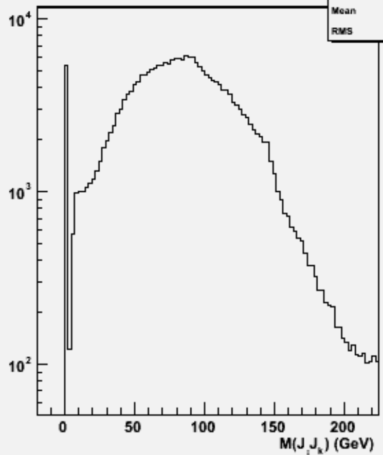
2jets mass(All comb)w104591 bbh_o
