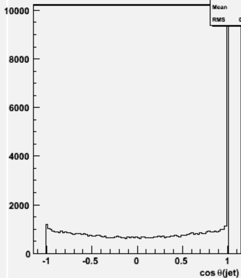
cos \theta for 2-jets :w104591 bbh_o
