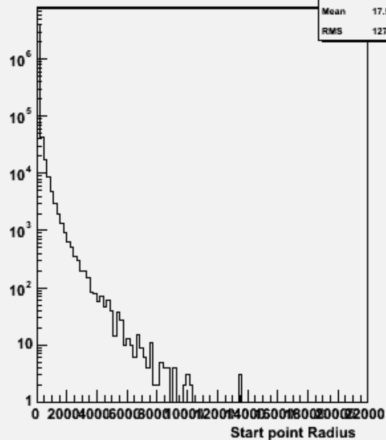
Start point R : w104591 bbh_o
