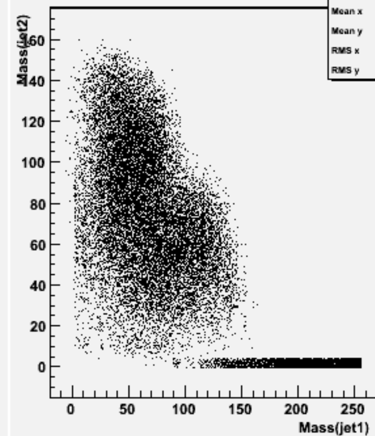
Jet mass for forced 2-jets : w104584 ddh_o
