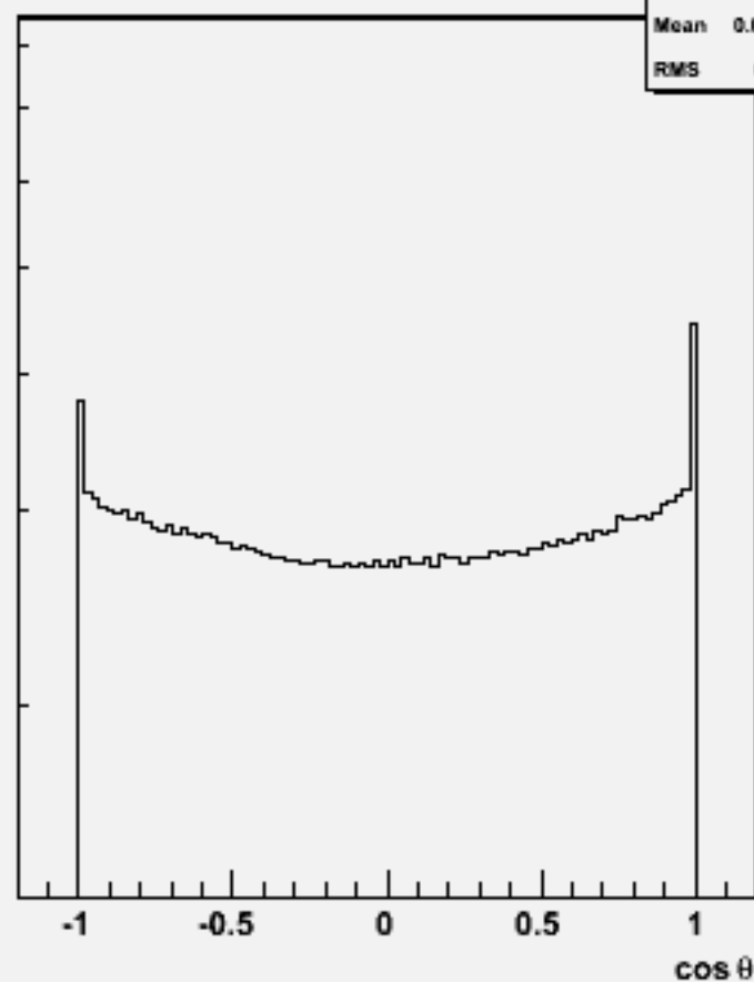
Particle \cos\theta : w104584 ddh_o
