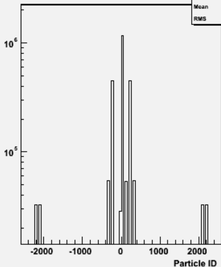
Particle ID : w104584 ddh_o
