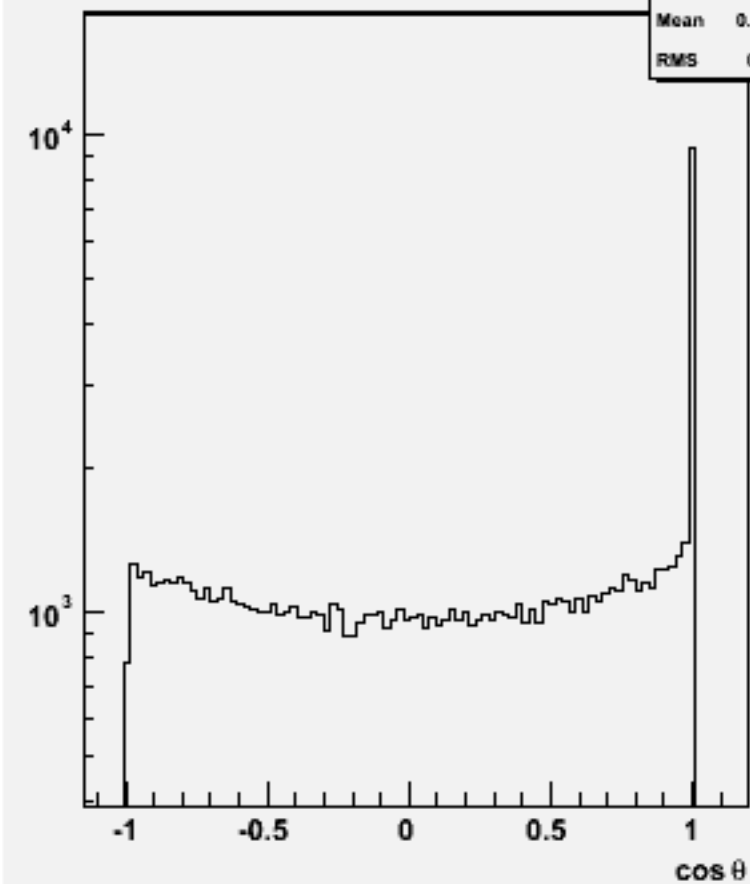
Jet cos \theta (All jets)w104584 ddh_o
