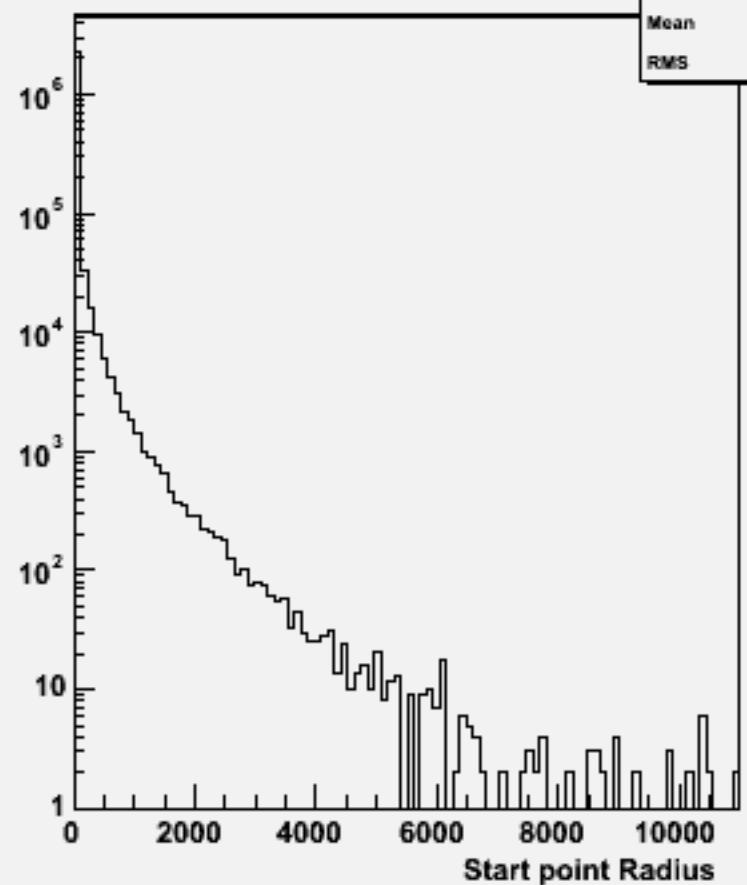
Start point R : w104584 ddh_o
