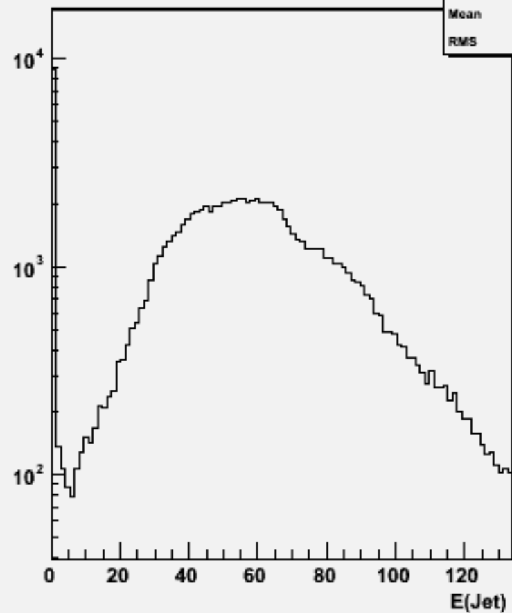
Jet energies(All jets)w104584 ddh_o
