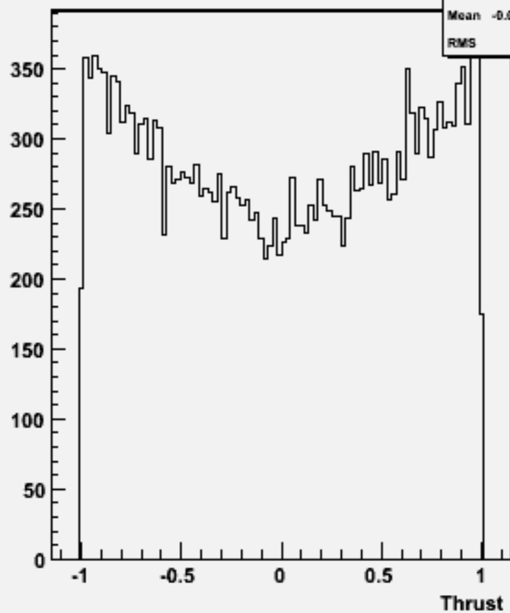
cos \Theta (thrust) w104584 ddh_o
