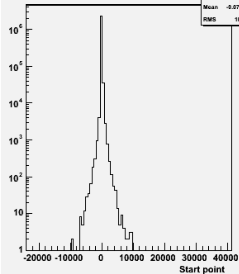
Start point Z : w104584 ddh_o
