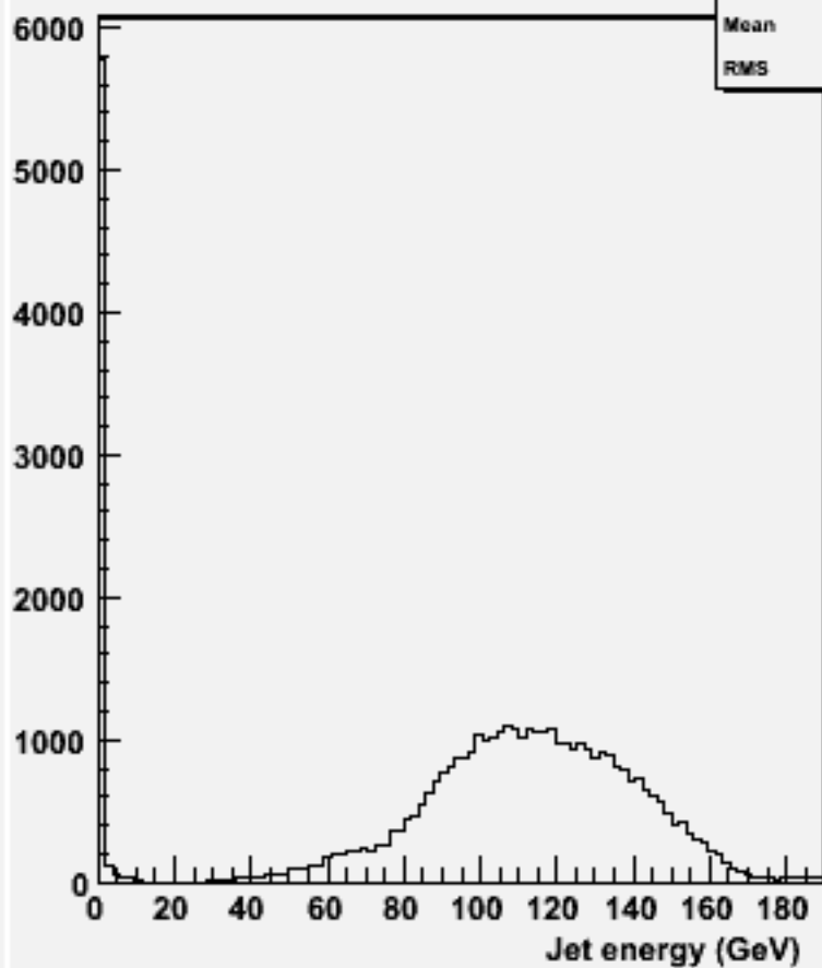
energy for 2-jets :w104584 ddh_o
