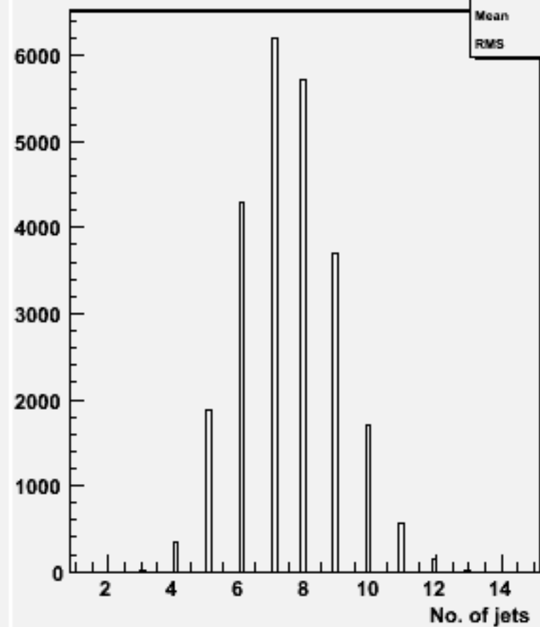
No. jets (ycut=0.001) : w104584 ddh_o
