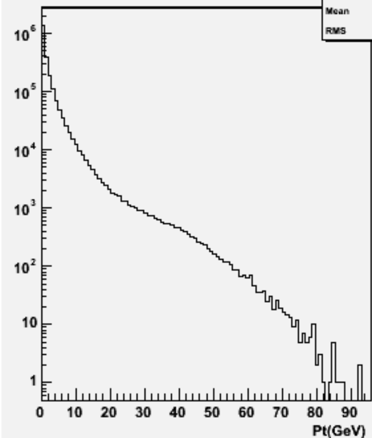
Particle Pt : w104584 ddh_o
