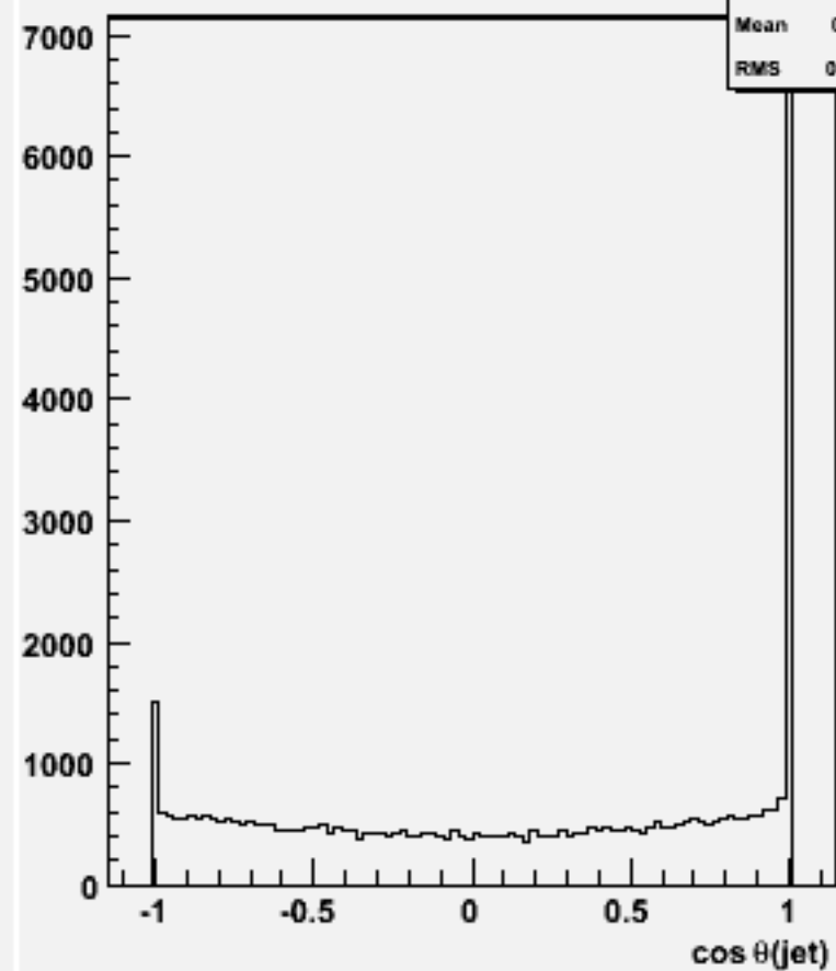
cos \theta for 2-jets :w104584 ddh_o
