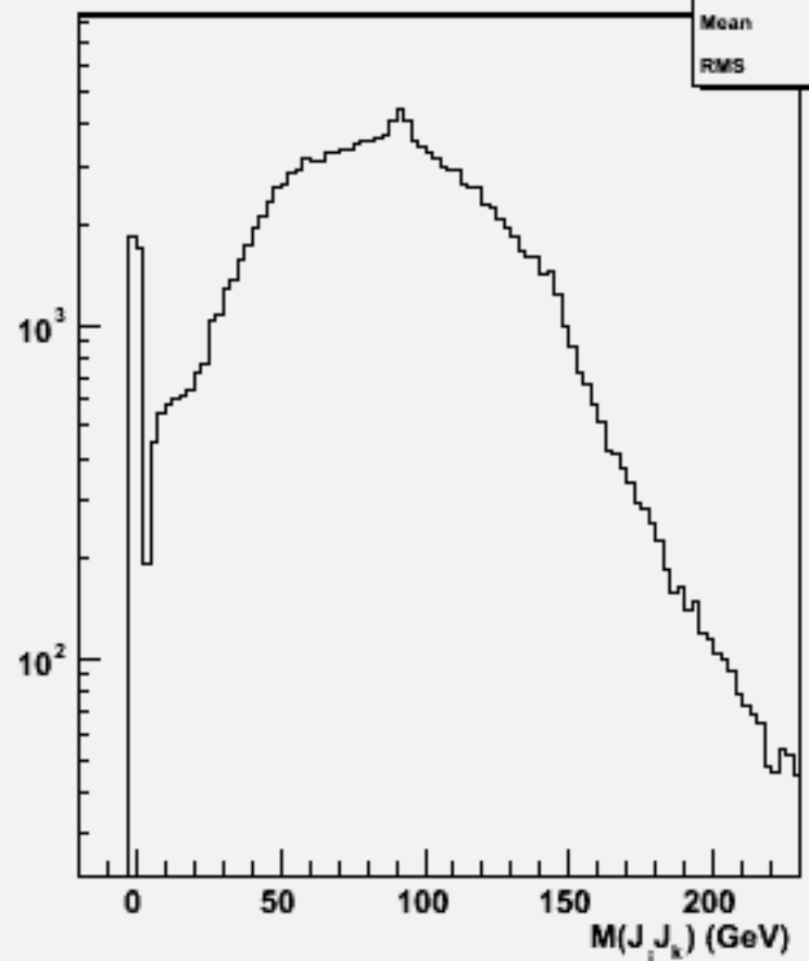
2jets mass(All comb)w104584 ddh_o
