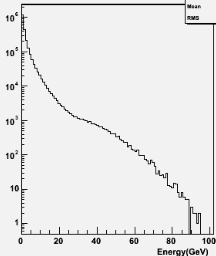
Particle Energy : w104584 ddh_o
