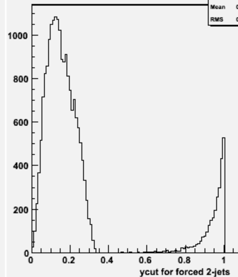
Ycut for 2-jets :w104584 ddh_o
