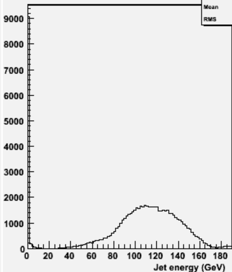
energy for 2-jets :w104583 ddh_o
