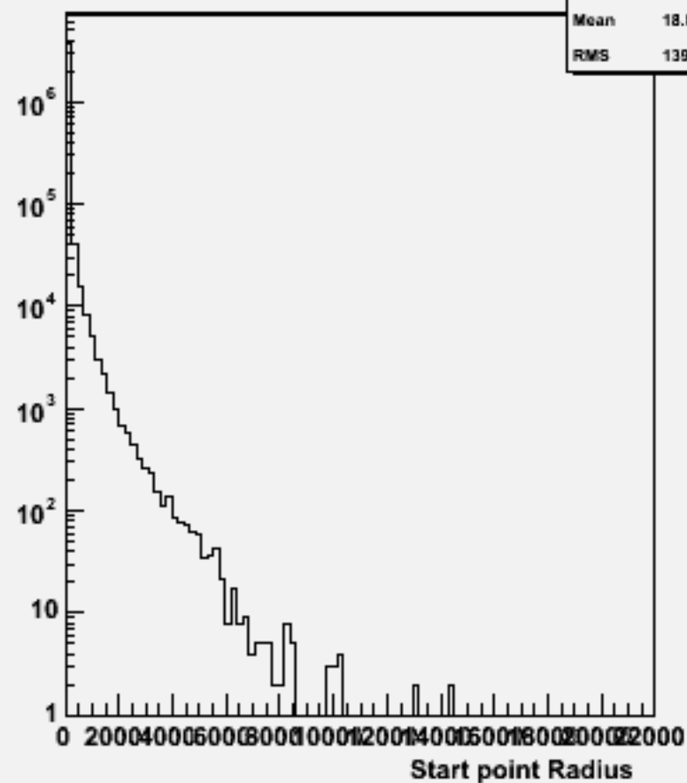
Start point R : w104583 ddh_o
