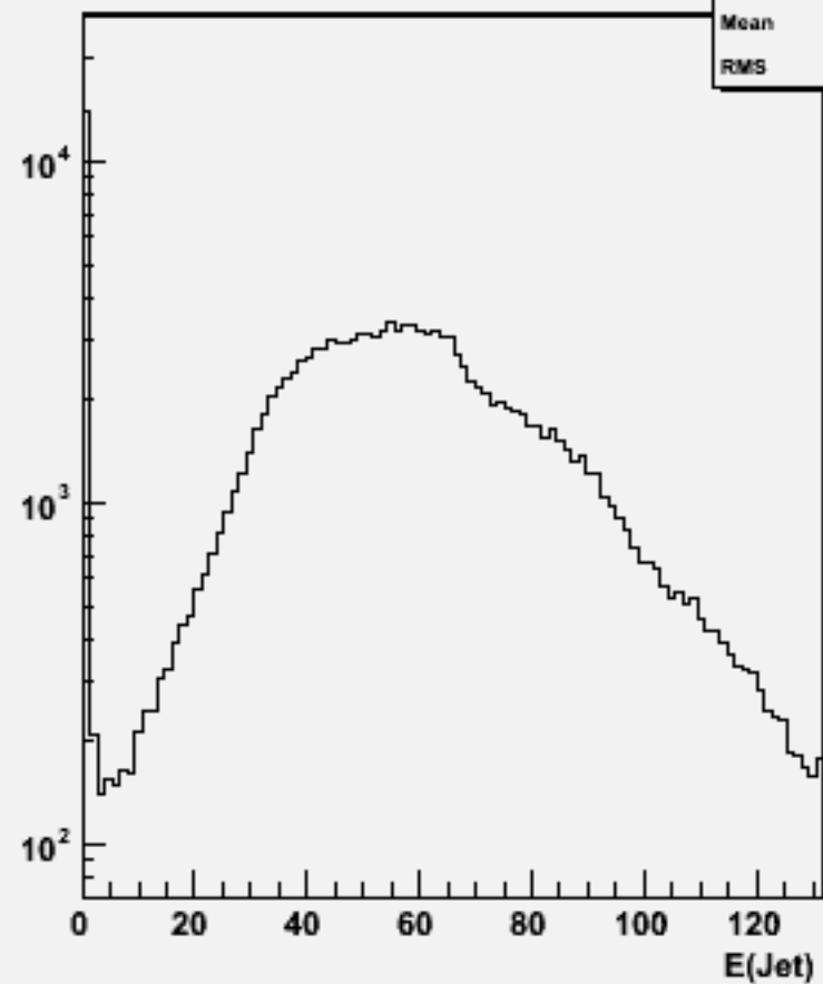
Jet energies(All jets)w104583 ddh_o
