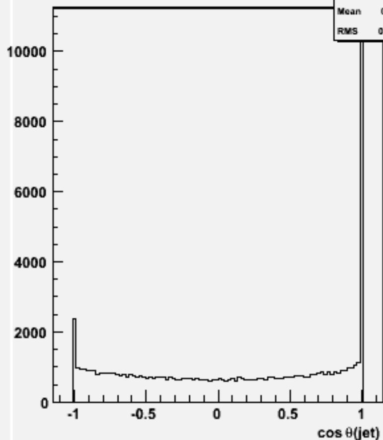
cos \theta for 2-jets :w104583 ddh_o
