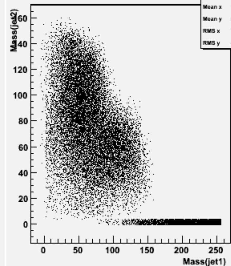
Jet mass for forced 2-jets : w104583 ddh_o
