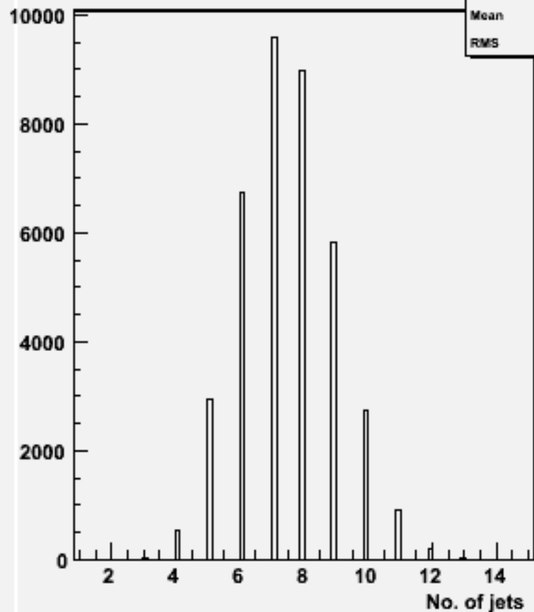
No. jets (ycut=0.001) : w104583 ddh_o
