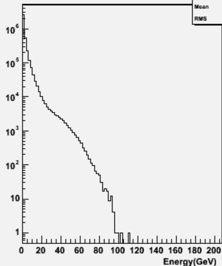
Particle Energy : w104583 ddh_o
