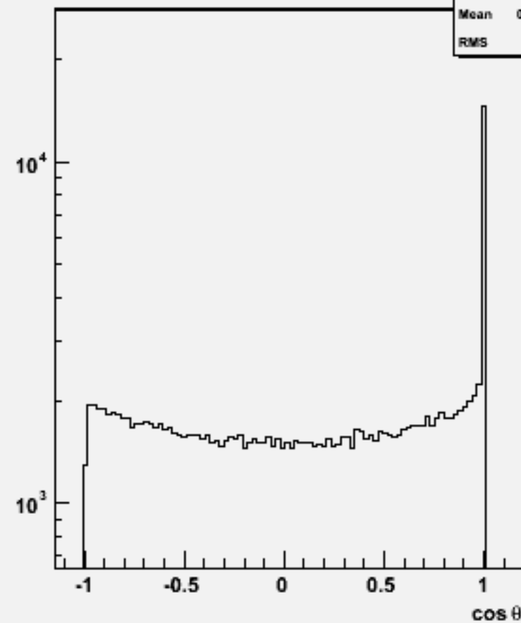
Jet cos \theta (All jets)w104583 ddh_o
