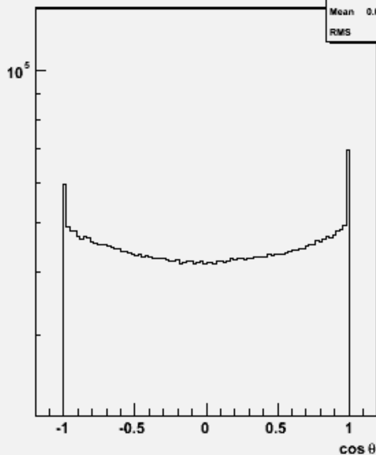
Particle cosθ : w104583 ddh_o
