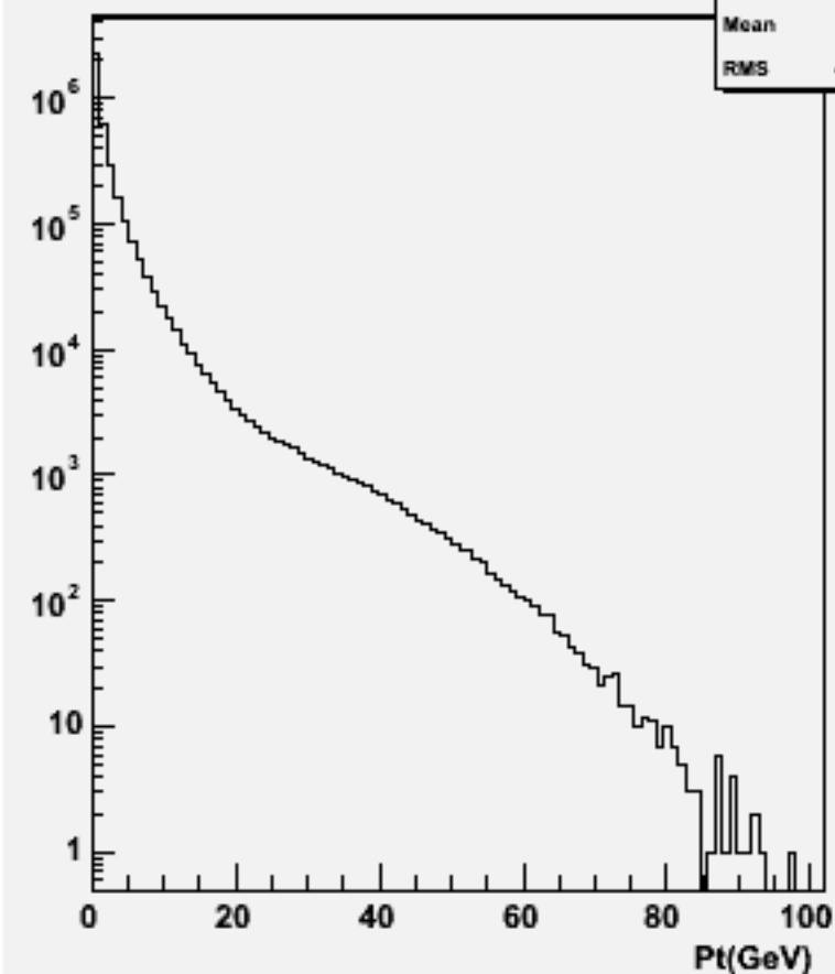
Particle Pt : w104583 ddh_o
