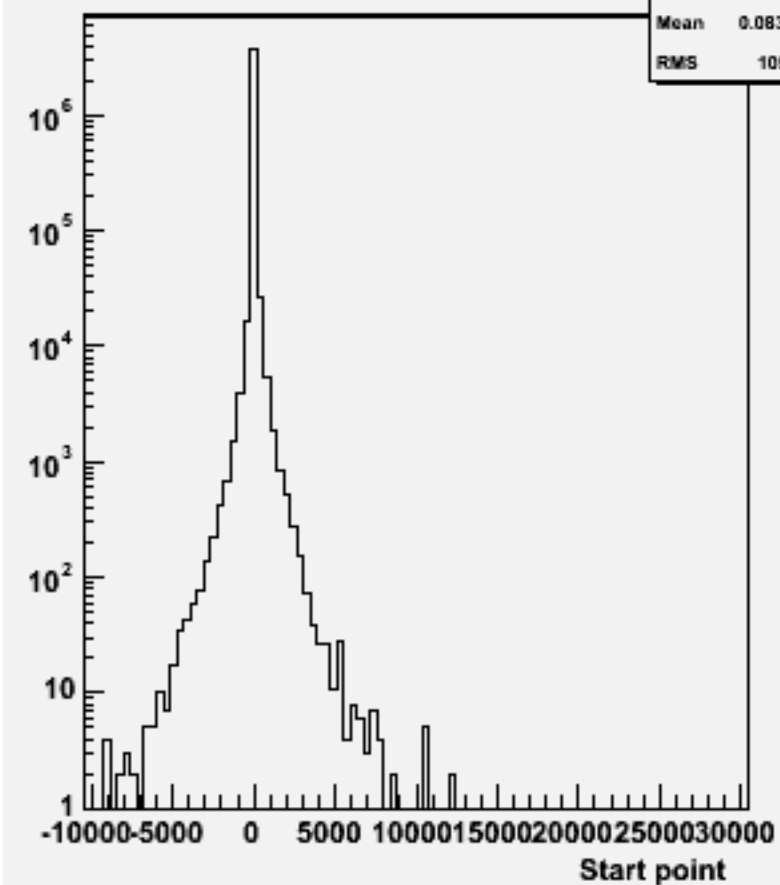
Start point Z : w104583 ddh_o
