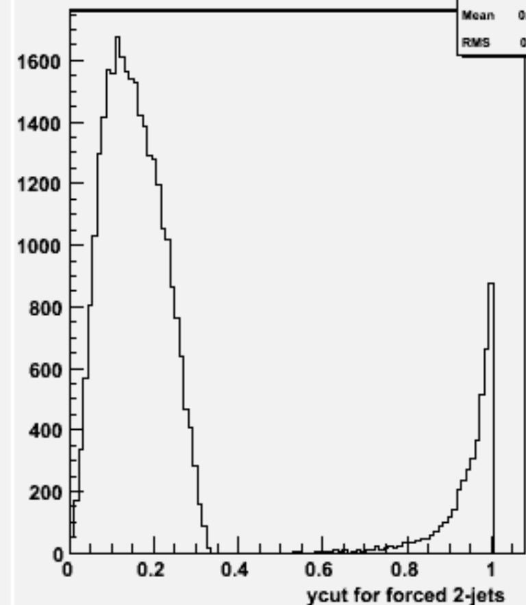
Ycut for 2-jets :w104583 ddh_o
