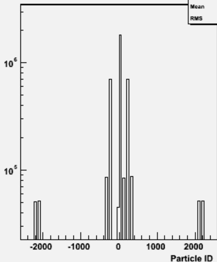
Particle ID : w104583 ddh_o
