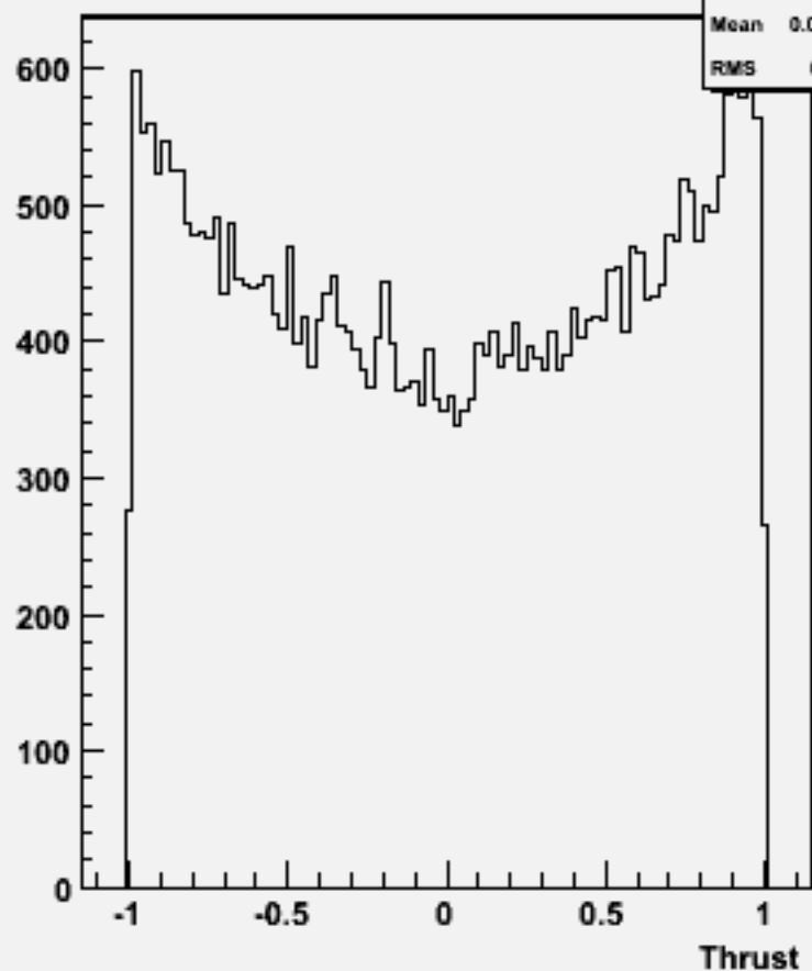
cos \Theta (thrust) w104583 ddh_o
