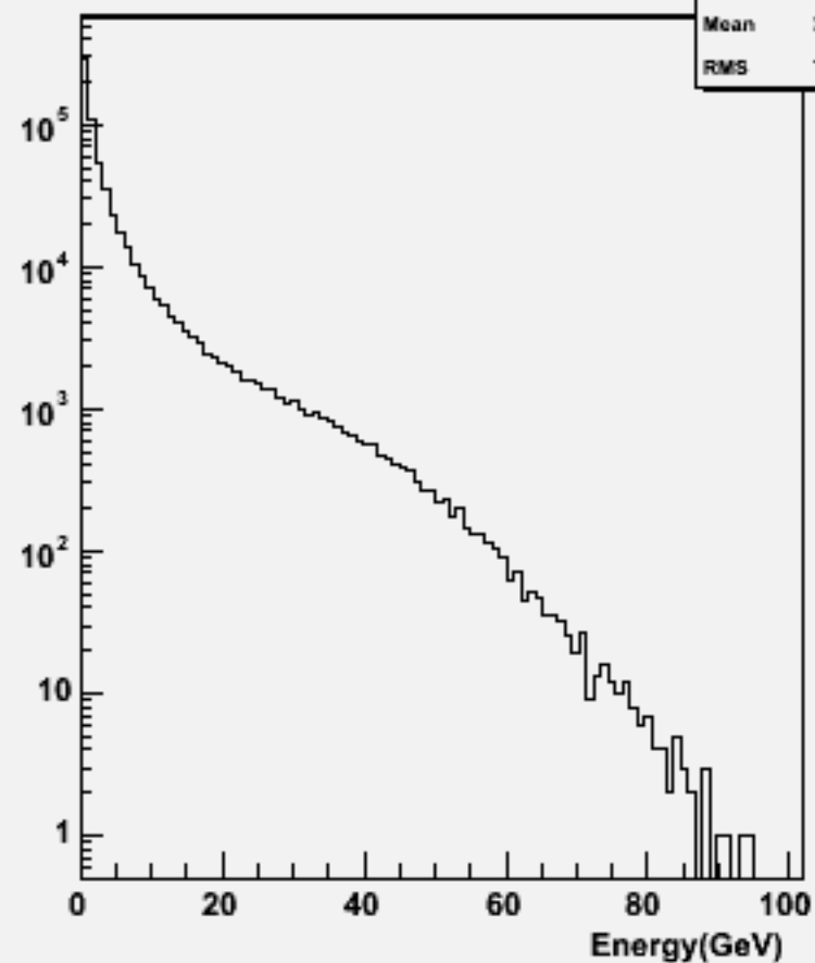
Particle Energy : w104579 e3e3h_o
