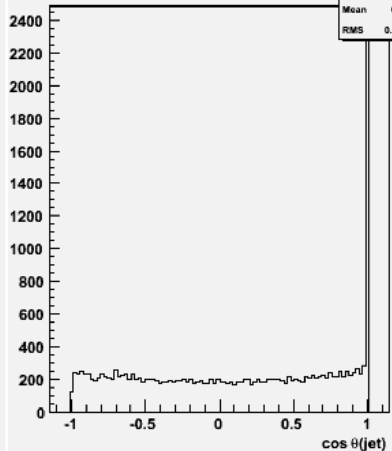
cos \theta for 2-jets :w104579 e3e3h_o
