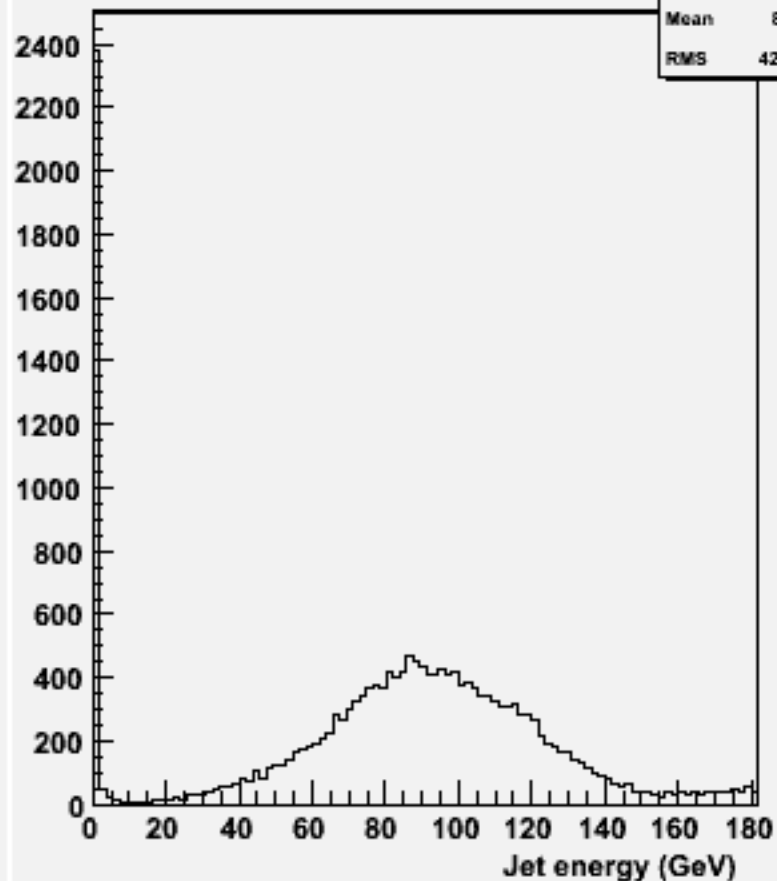
energy for 2-jets :w104579 e3e3h_o
