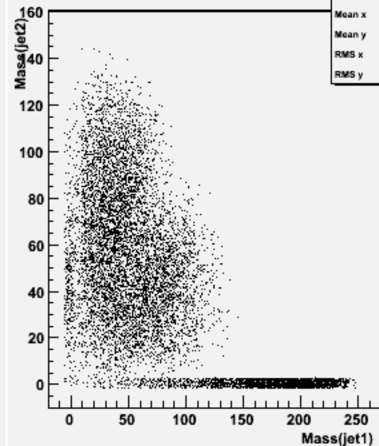
Jet mass for forced 2-jets : w104579 e3e3h_o
