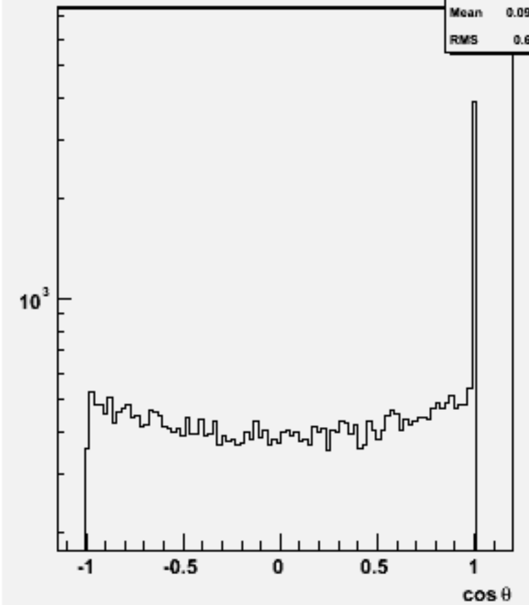
Jet cos \theta (All jets)w104579 e3e3h_o
