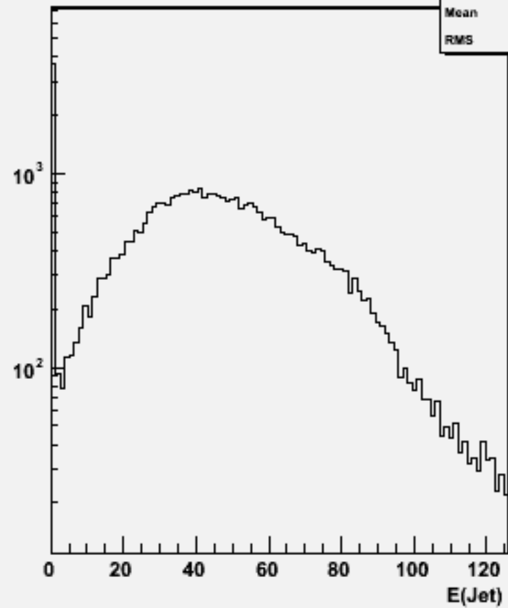
Jet energies(All jets)w104579 e3e3h_o
