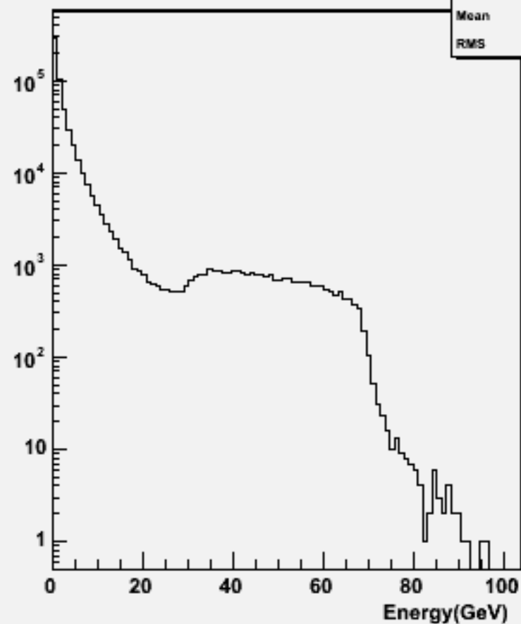
Particle Energy : w104576 e2e2h_o
