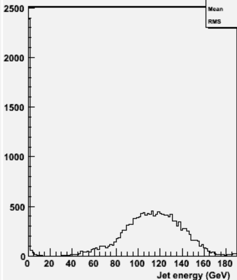
energy for 2-jets :w104576 e2e2h_o
