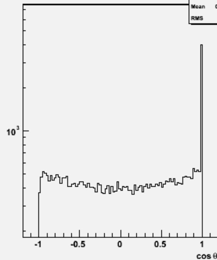
Jet cos \theta (All jets)w104576 e2e2h_o
