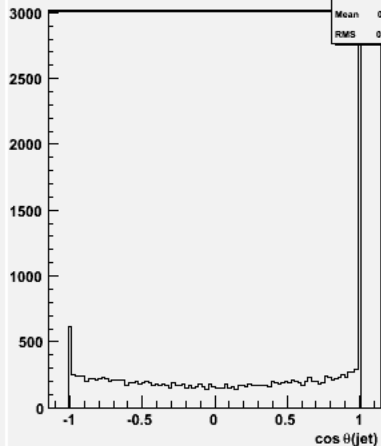
cos \theta for 2-jets :w104576 e2e2h_o
