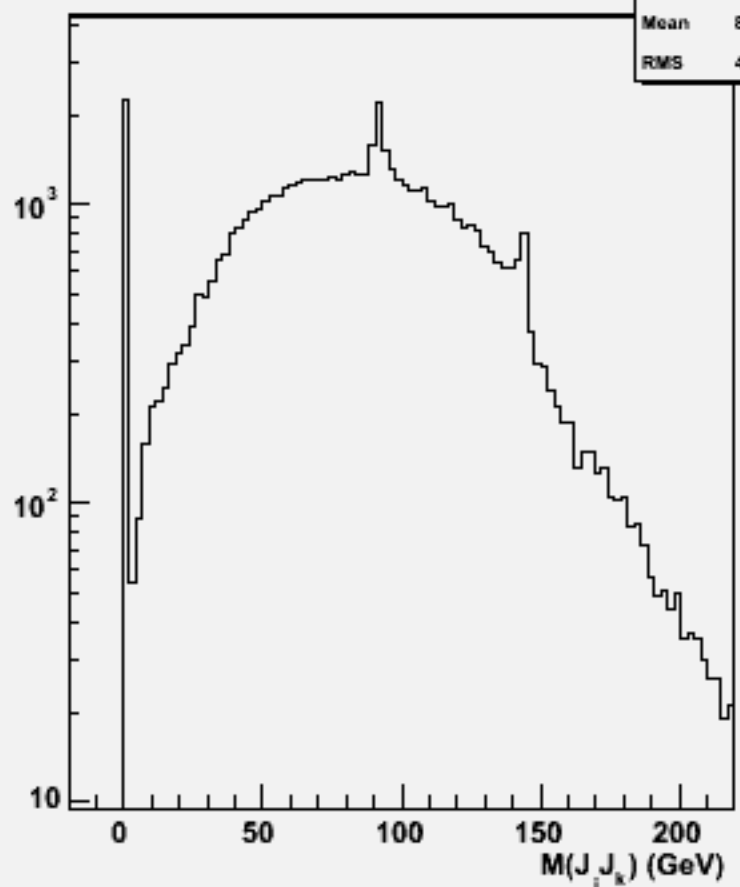
2jets mass(All comb)w104576 e2e2h_o
