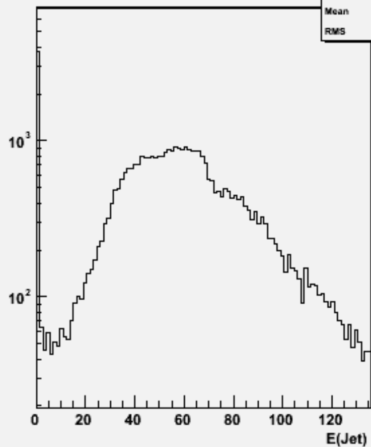
Jet energies(All jets)w104576 e2e2h_o
