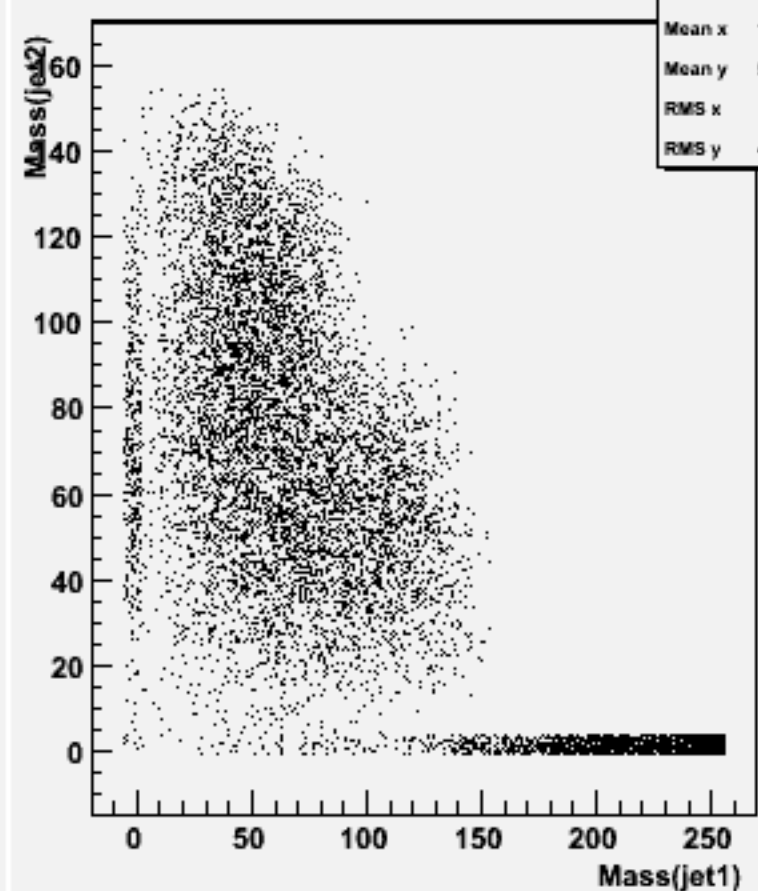
Jet mass for forced 2-jets : w104576 e2e2h_o
