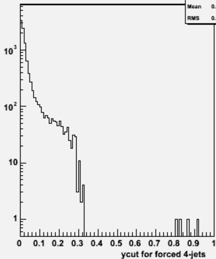
Ycut for 4-jets :w104576 e2e2h_o
