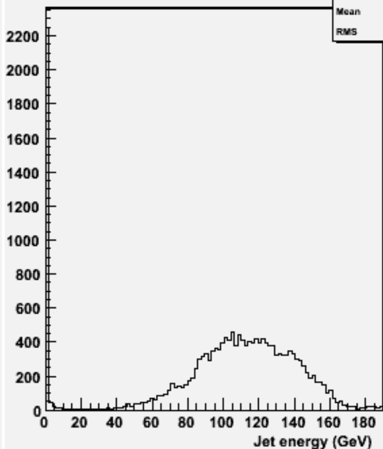
energy for 2-jets :w104573 e1e1h_o
