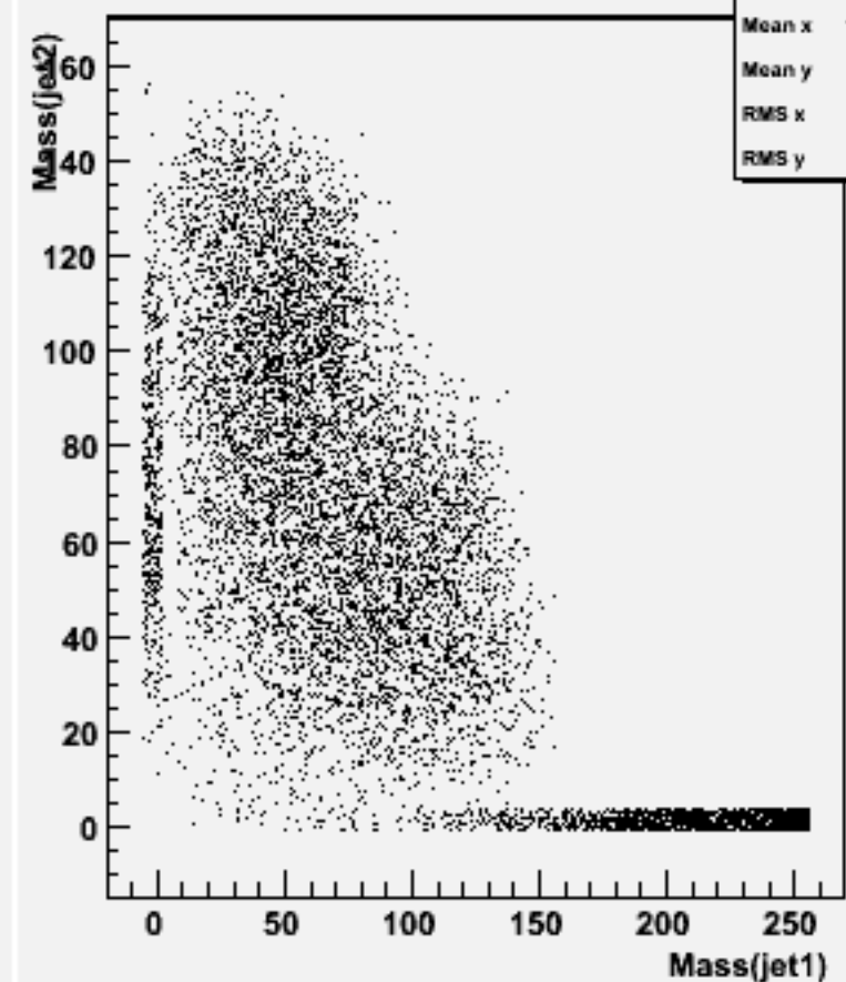
Jet mass for forced 2-jets : w104573 e1e1h_o
