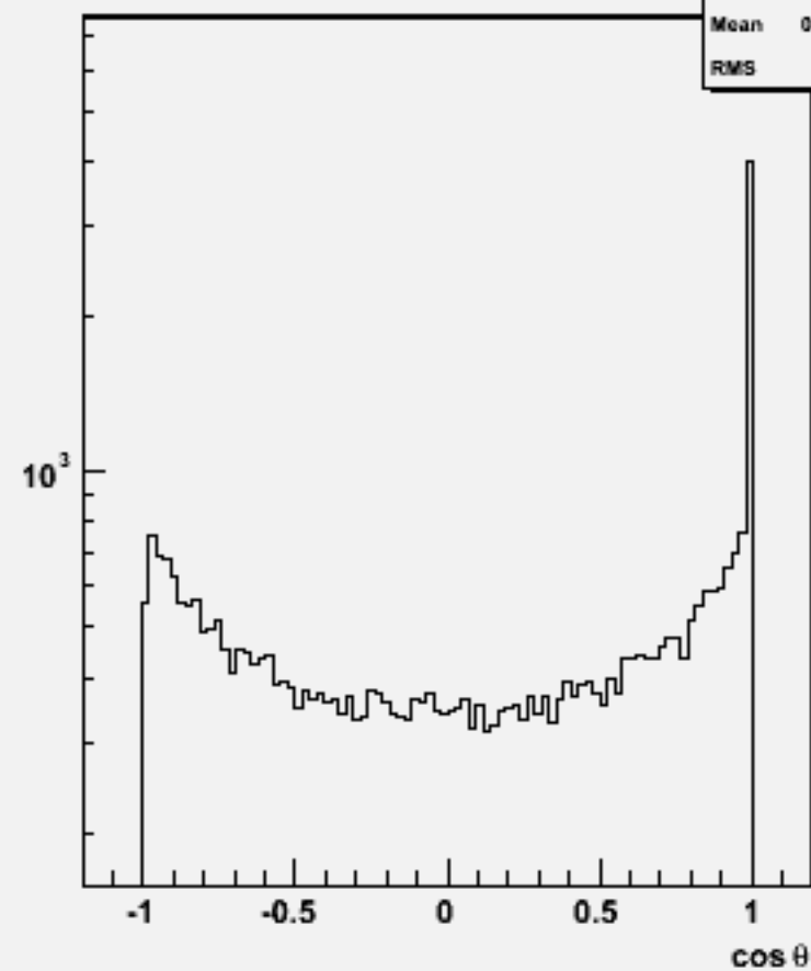
Jet cos \theta (All jets)w104573 e1e1h_o
