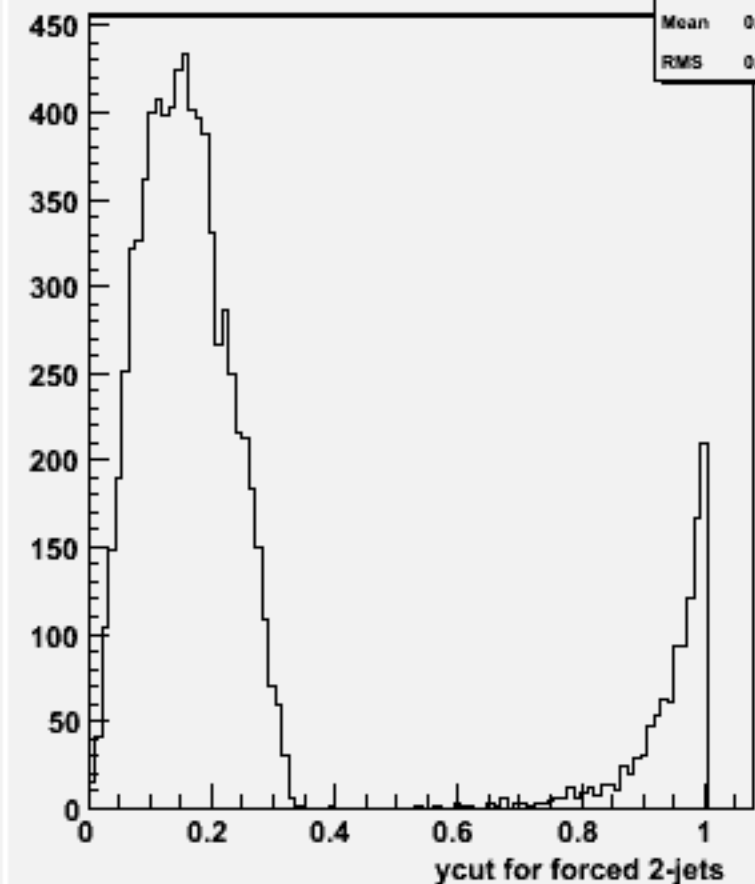
Ycut for 2-jets :w104573 e1e1h_o
