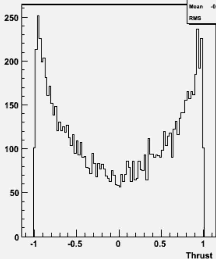
cos \Theta (thrust) w104573 e1e1h_o
