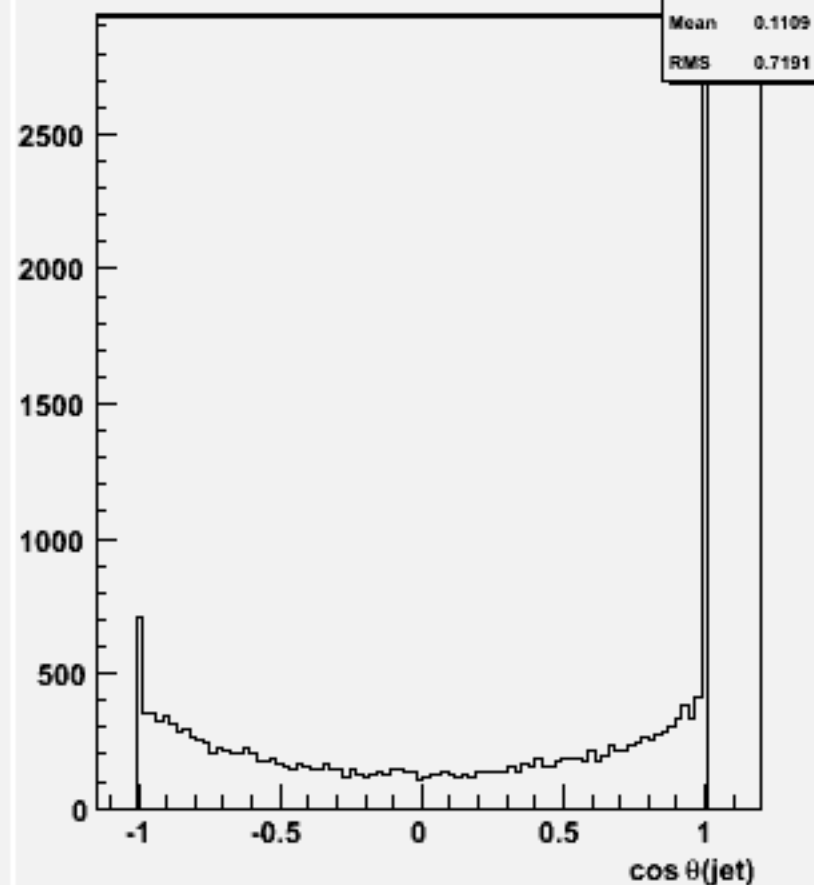
cos \theta for 2-jets :w104573 e1e1h_o
