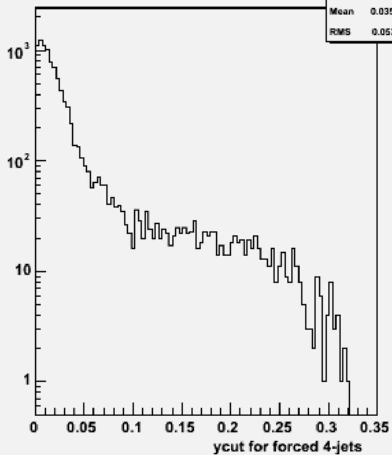
Ycut for 4-jets :w104573 e1e1h_o
