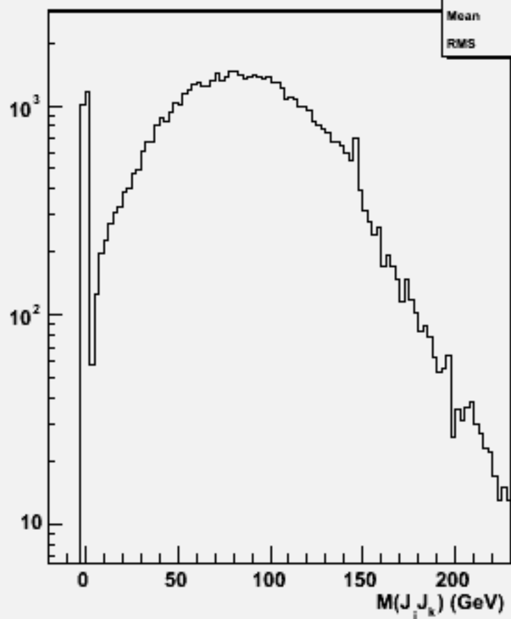
2jets mass(All comb)w104573 e1e1h_o
