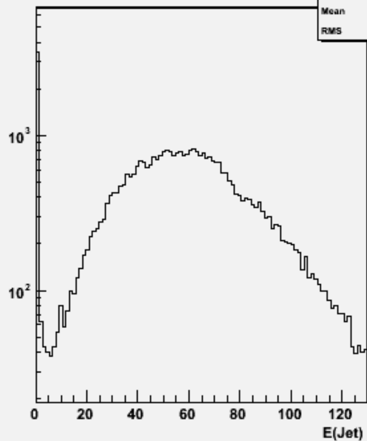
Jet energies(All jets)w104573 e1e1h_o
