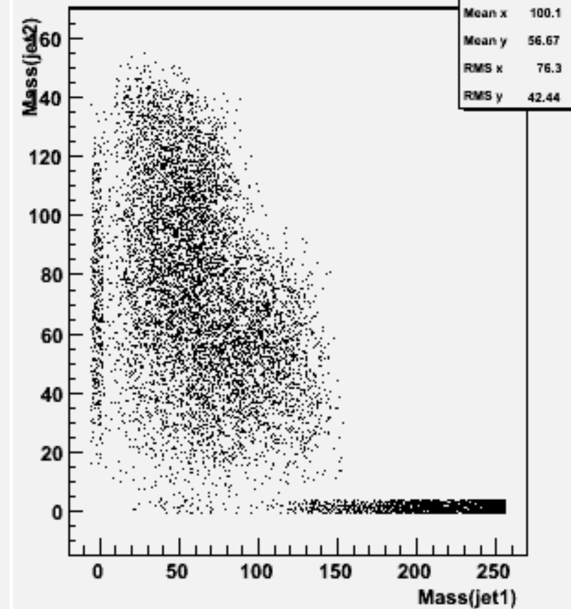
Jet mass for forced 2-jets : w104572 e1e1h_o
