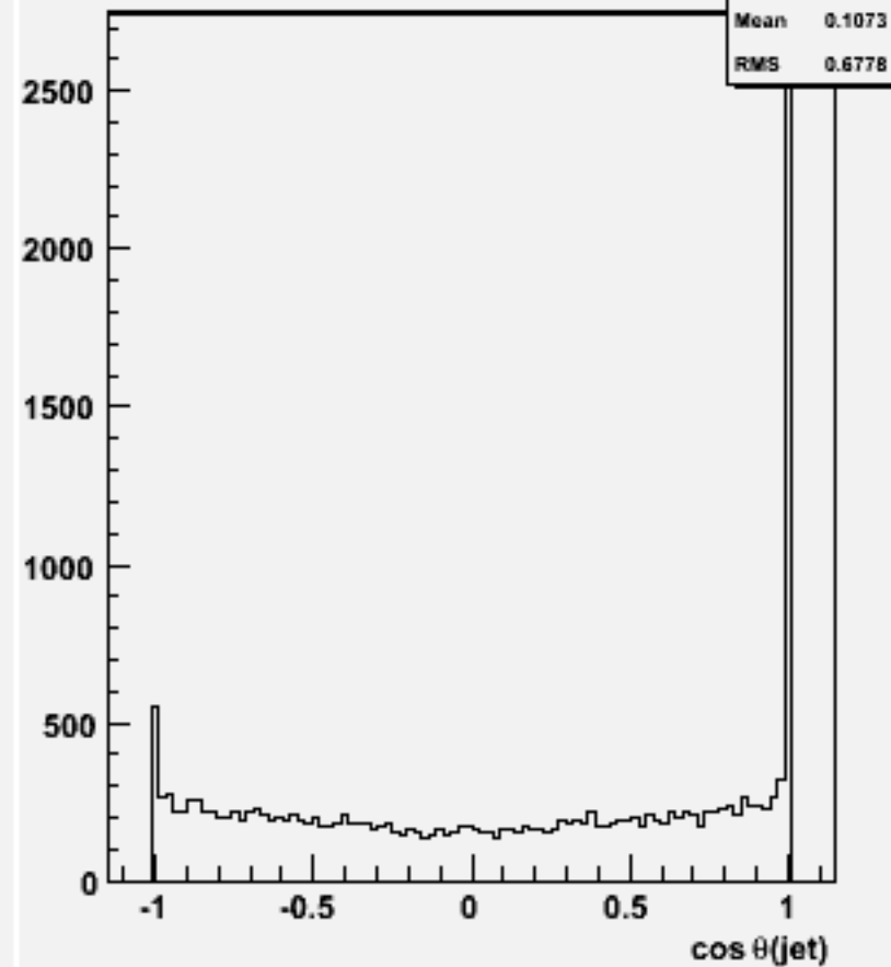
cos \theta for 2-jets :w104572 e1e1h_o
