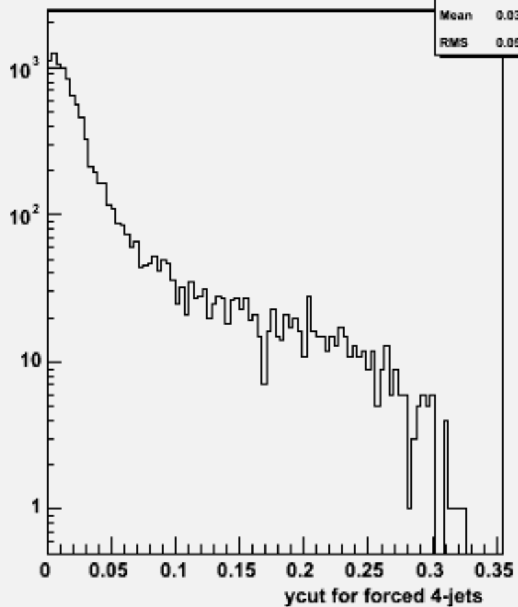
Ycut for 4-jets :w104572 e1e1h_o
