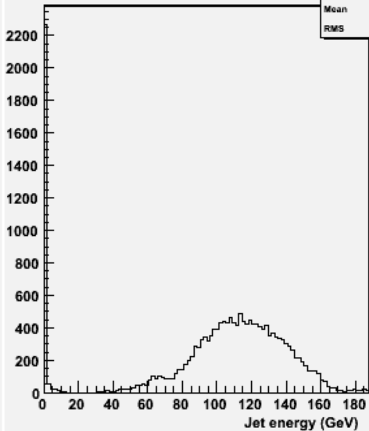
energy for 2-jets :w104572 e1e1h_o
