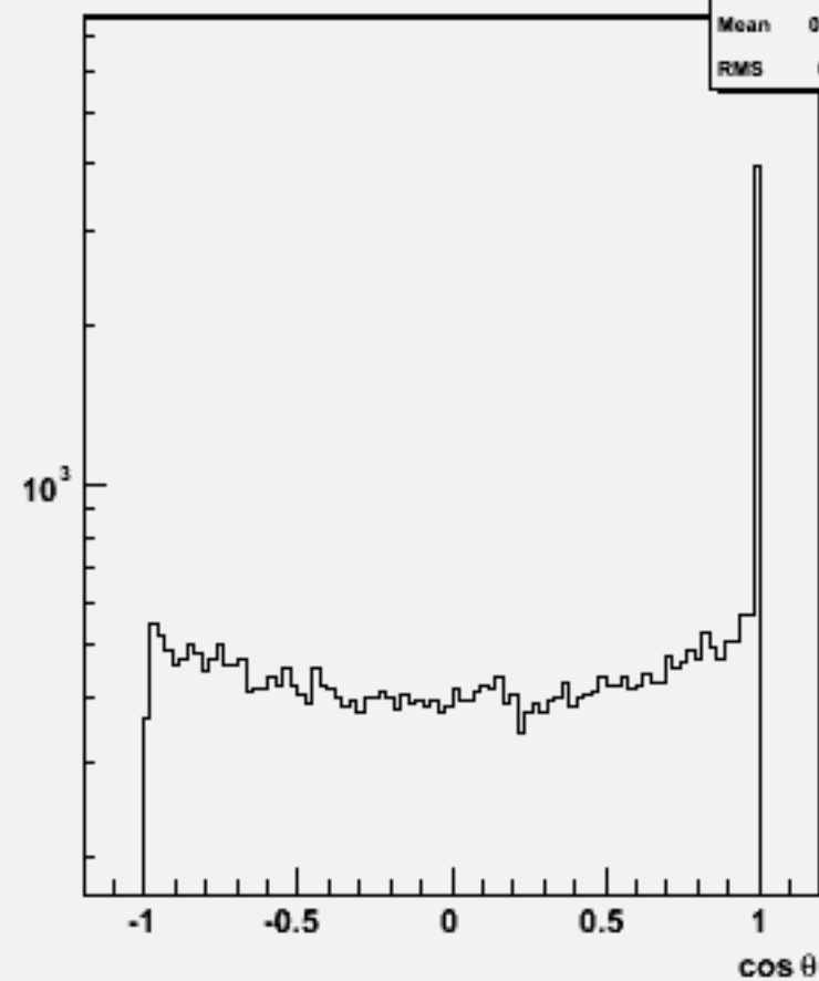
Jet cos \theta (All jets)w104571 e1e1h_o
