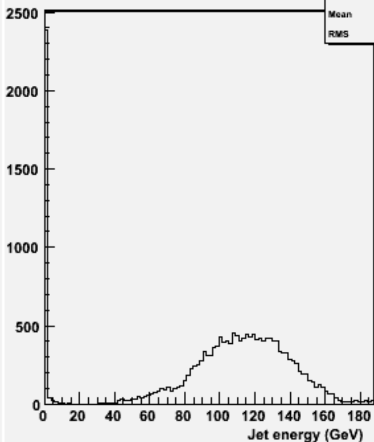
energy for 2-jets :w104571 e1e1h_o
