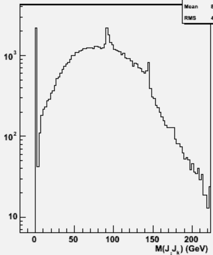
2jets mass(All comb)w104571 e1e1h_o
