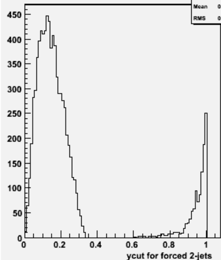
Ycut for 2-jets :w104571 e1e1h_o
