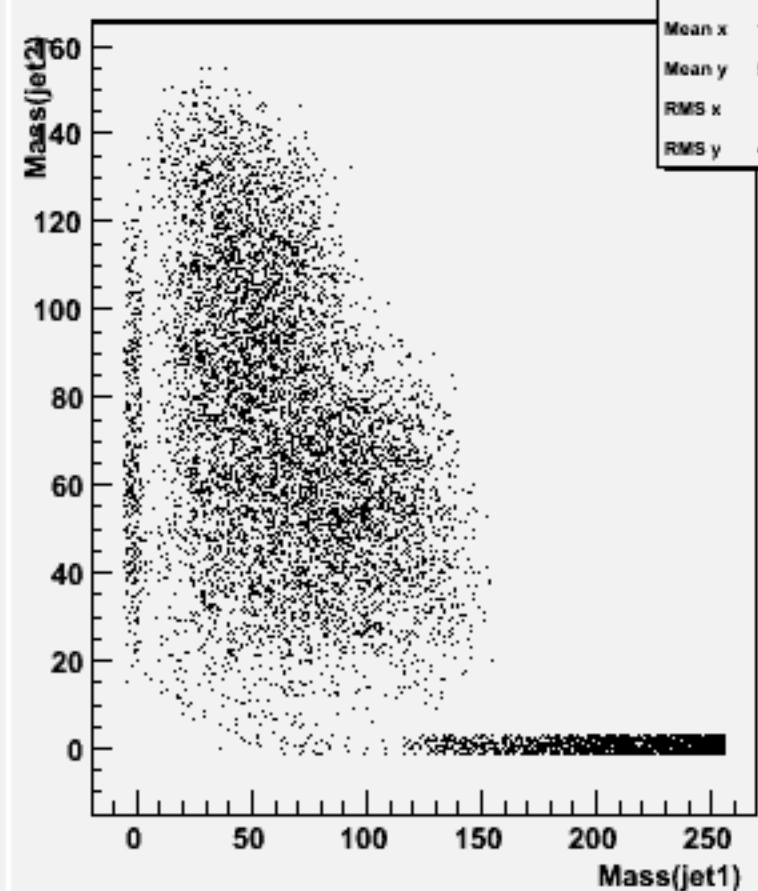
Jet mass for forced 2-jets : w104571 e1e1h_o
