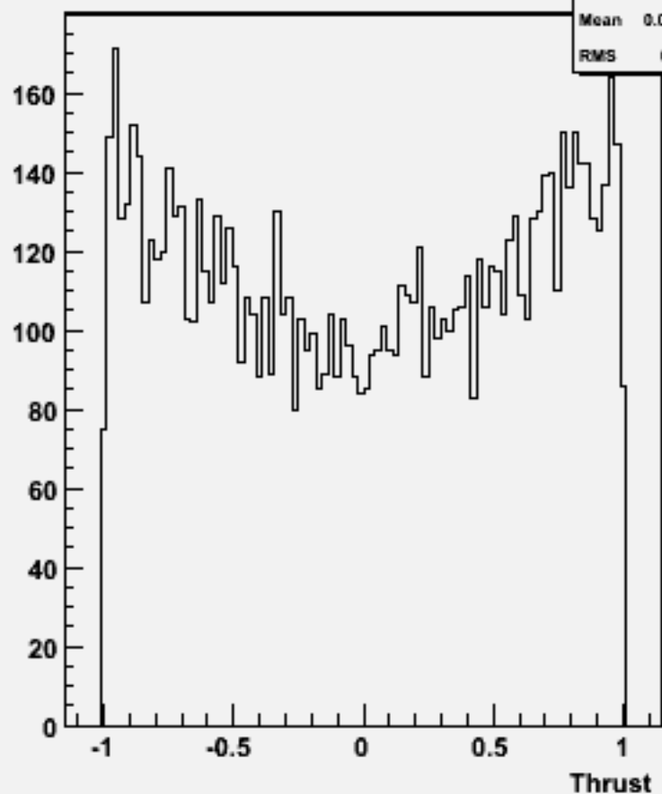
cos \Theta (thrust) w104571 e1e1h_o
