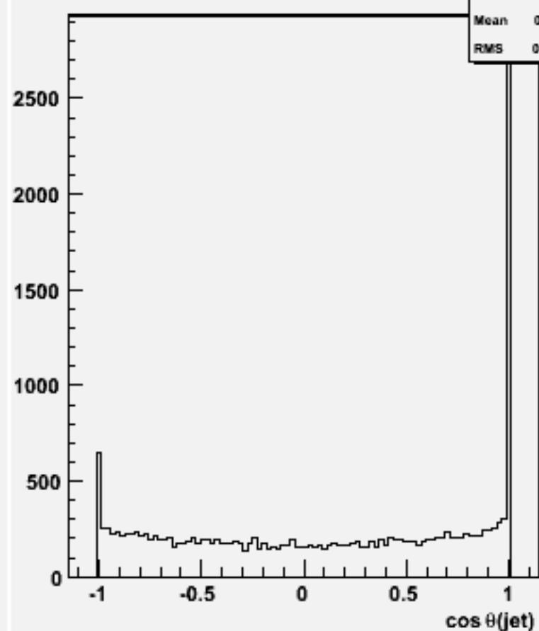
cos \theta for 2-jets :w104571 e1e1h_o
