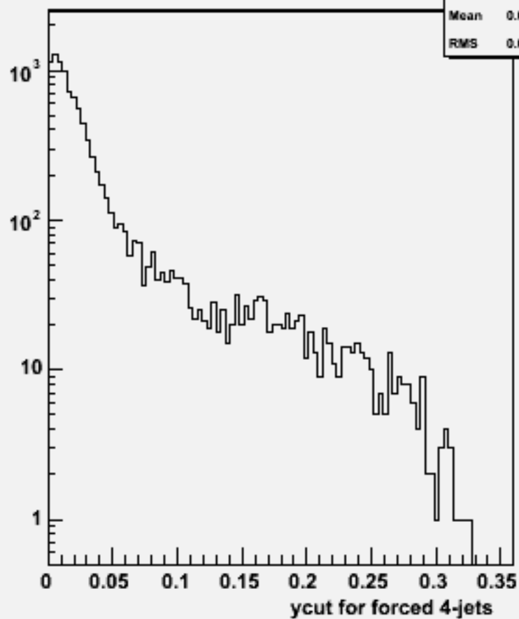
Ycut for 4-jets :w104571 e1e1h_o
