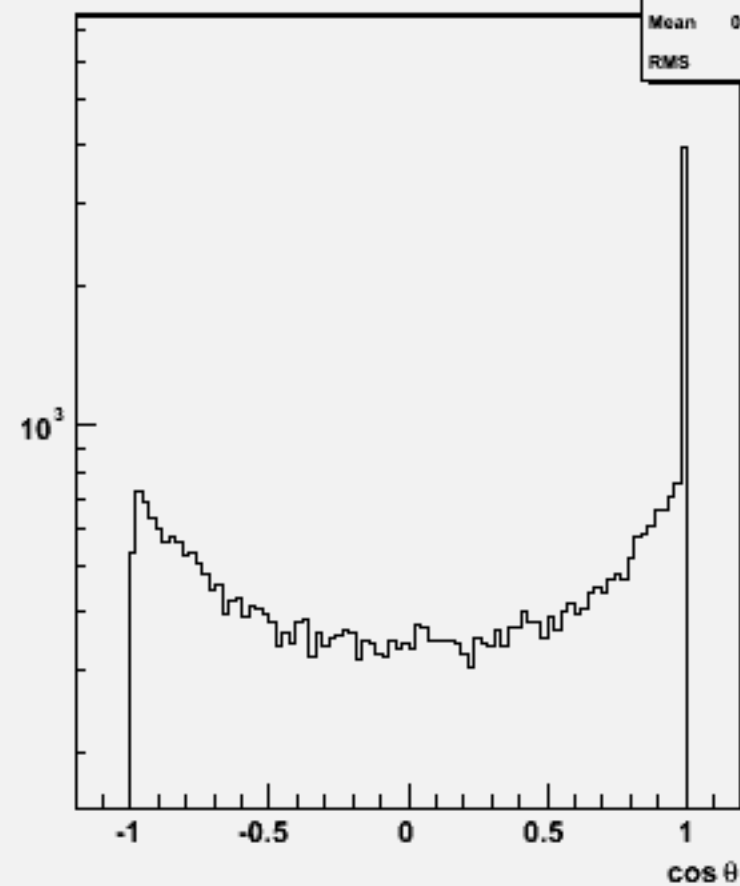
Jet cos \theta (All jets)w104570 e1e1h_o
