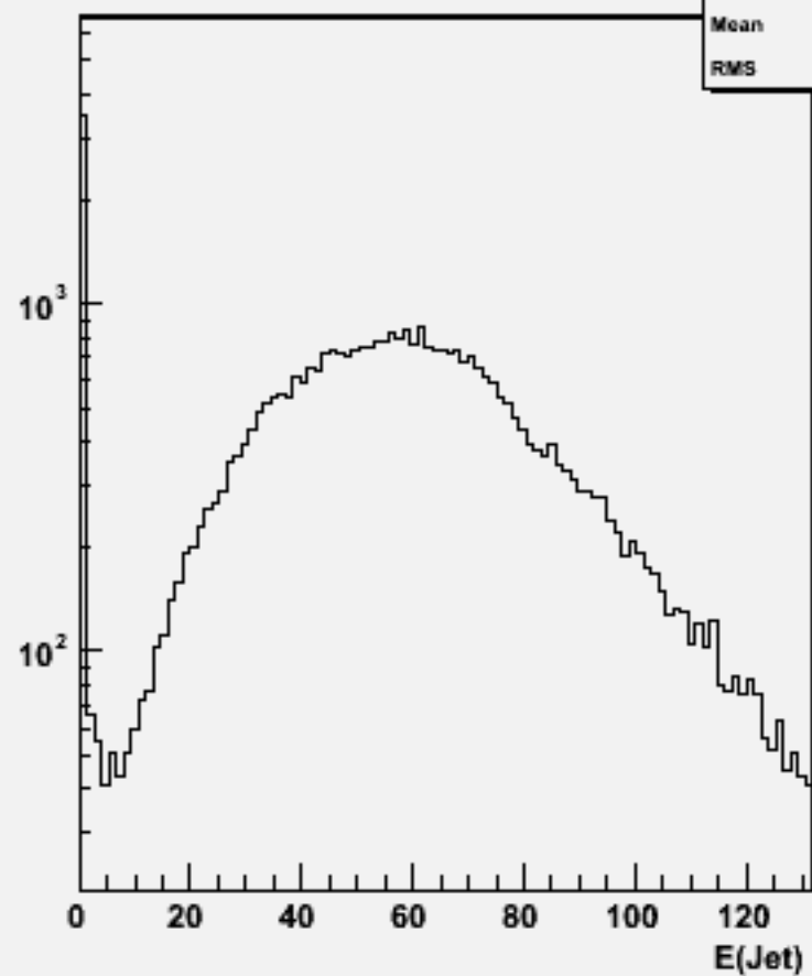
Jet energies(All jets)w104570 e1e1h_o
