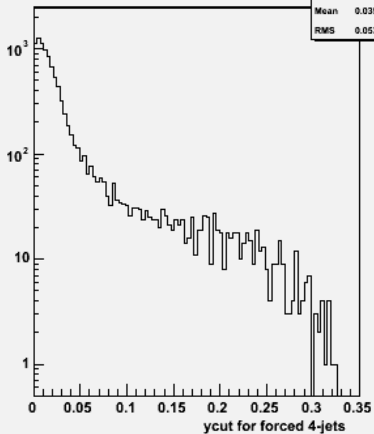
Ycut for 4-jets :w104570 e1e1h_o
