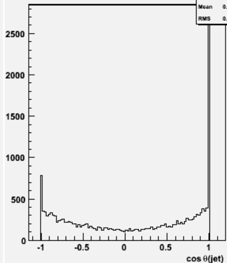
cos \theta for 2-jets :w104570 e1e1h_o
