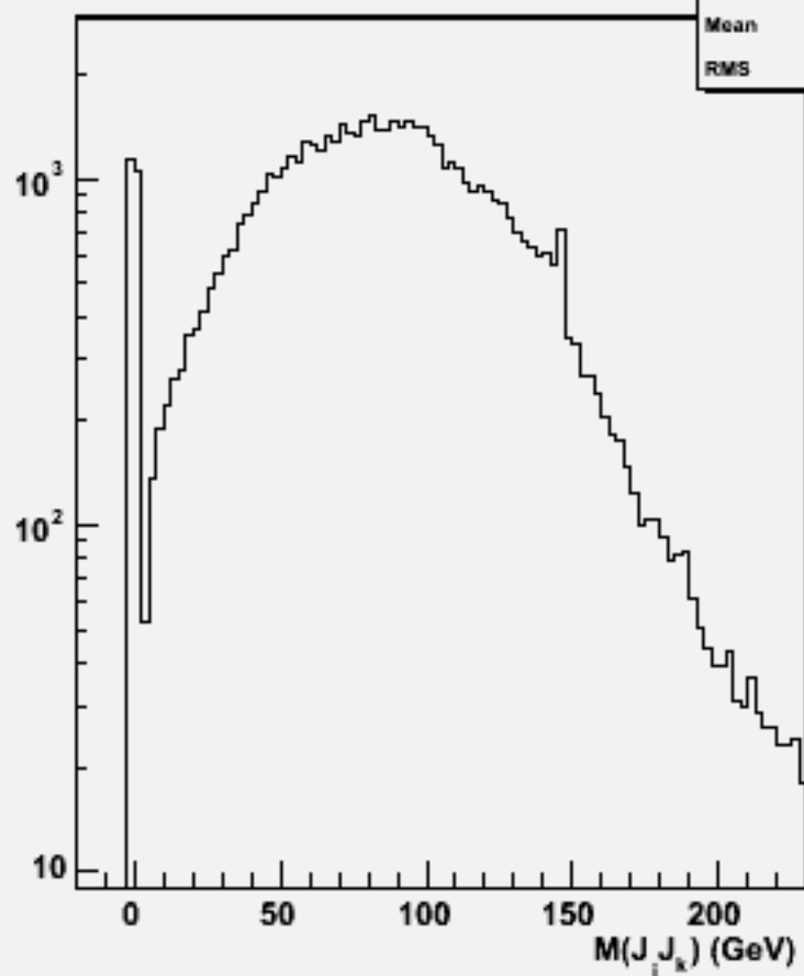
2jets mass(All comb)w104570 e1e1h_o
