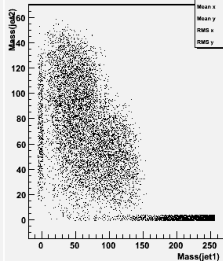
Jet mass for forced 2-jets : w104570 e1e1h_o
