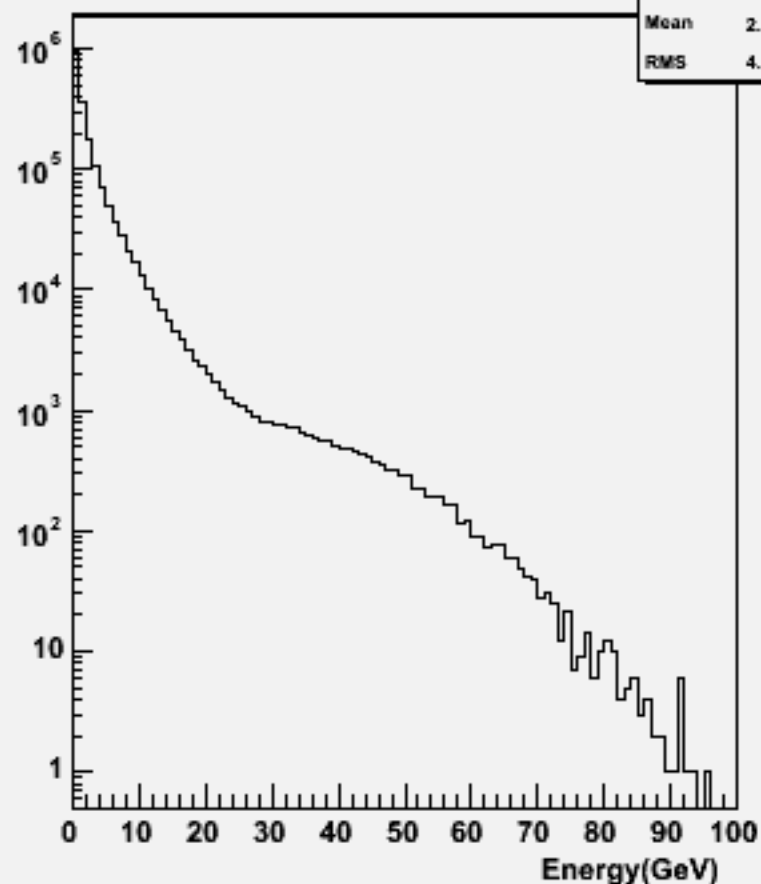
Start point R : w104568 cch_o
