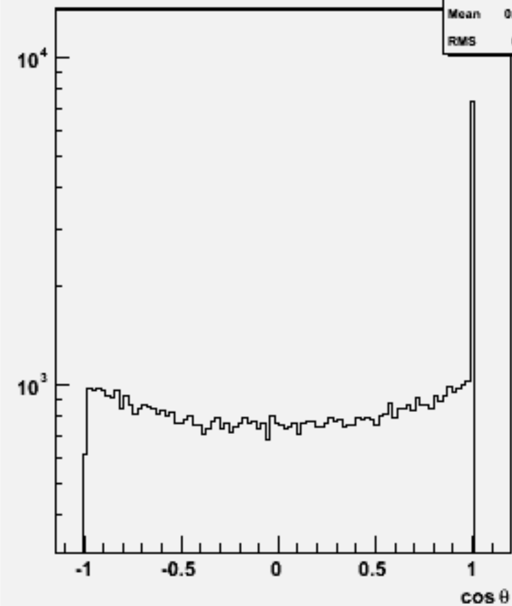
Jet cos \theta (All jets)w104568 cch_o
