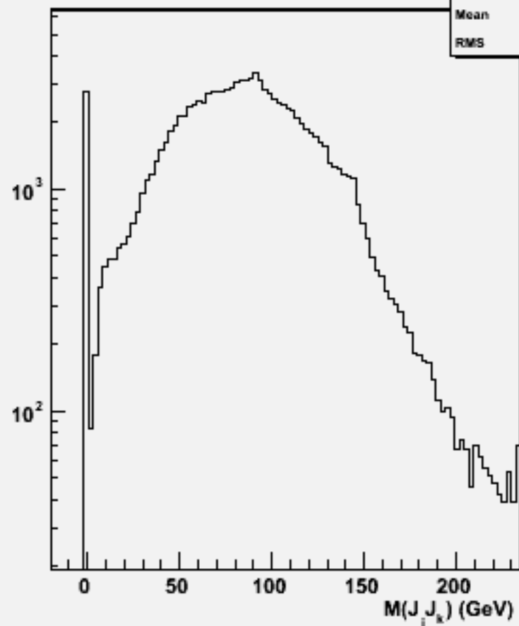
2jets mass(All comb)w104568 cch_o
