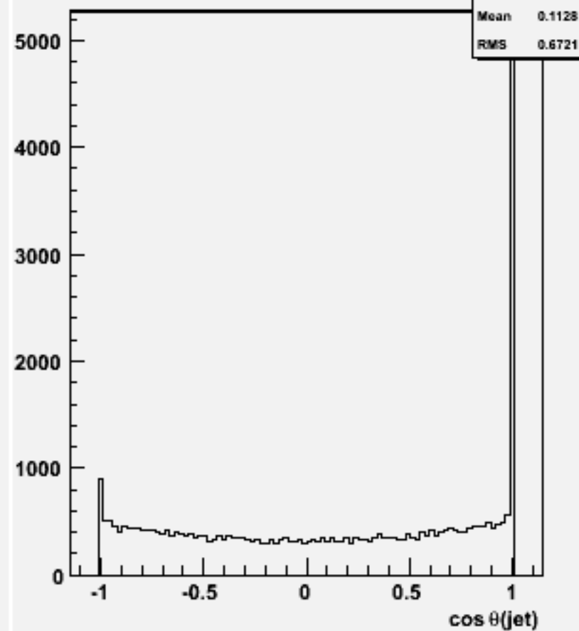
cos \Theta for 2-jets :w104568 cch_o
