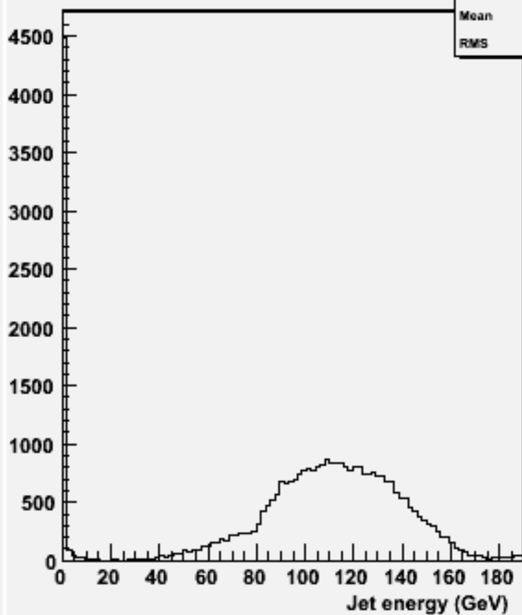
energy for 2-jets :w104568 cch_o
