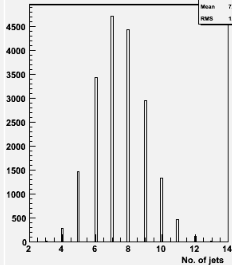
No. jets (ycut=0.001) : w104568 cch_o
