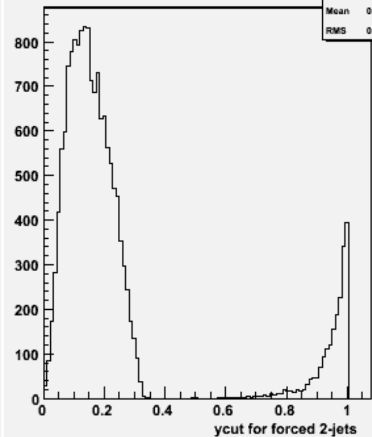
Ycut for 2-jets :w104568 cch_o
