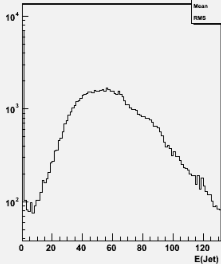
Jet energies(All jets)w104568 cch_o
