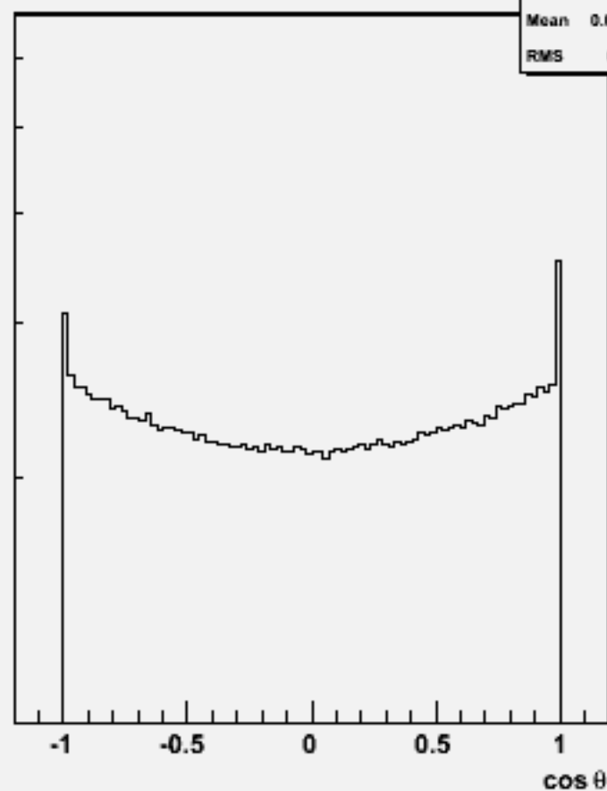
Particle cosθ : w104568 cch_o
