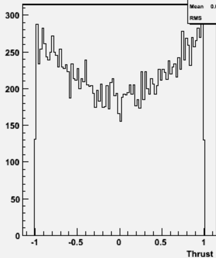
cos \Theta (thrust) w104568 cch_o
