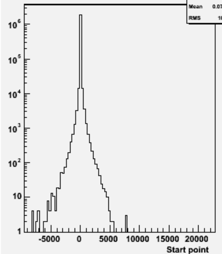
Start point Z : w104568 cch_o
