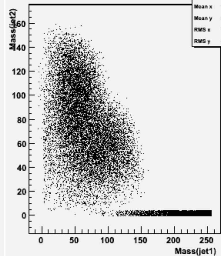
Jet mass for forced 2-jets : w104568 cch_o
