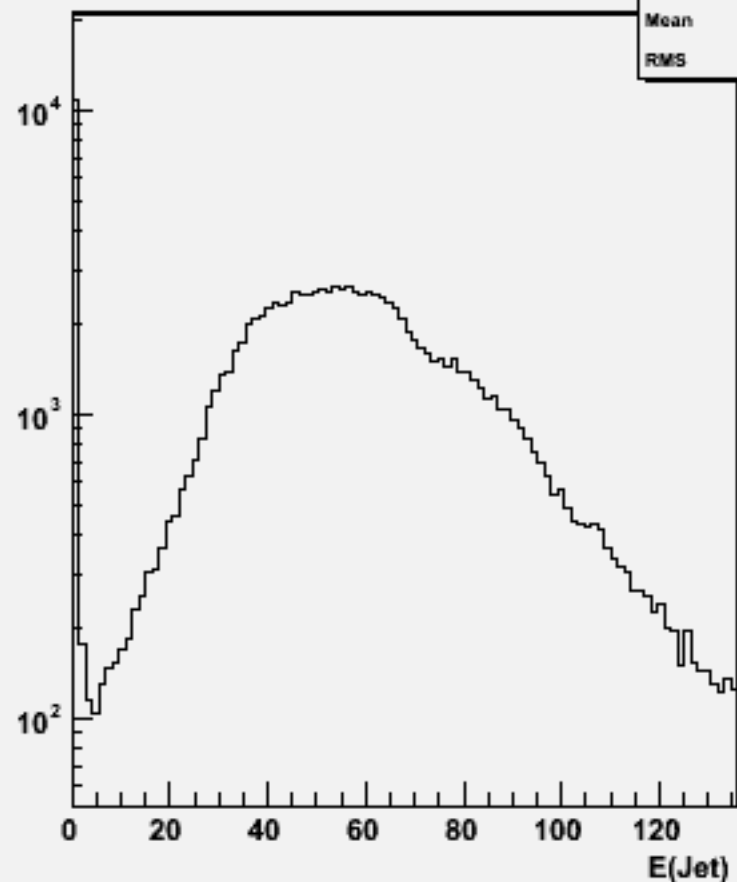
Jet energies(All jets)w104567 cch_o
