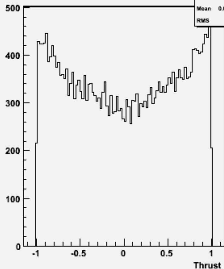
cos \Theta (thrust) w104567 cch_o
