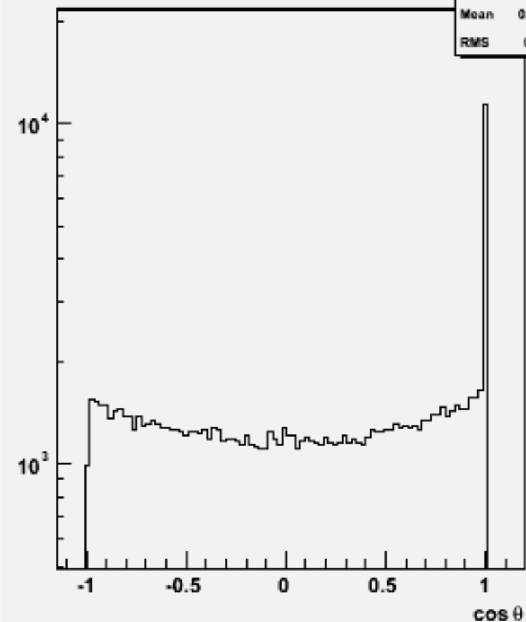
Jet cos \theta (All jets)w104567 cch_o
