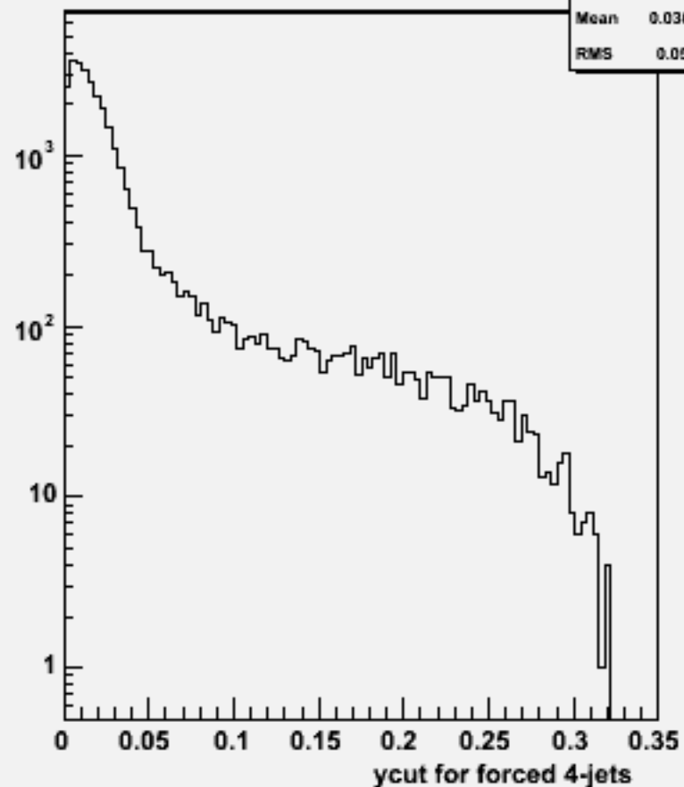
Ycut for 4-jets :w104567 cch_o
