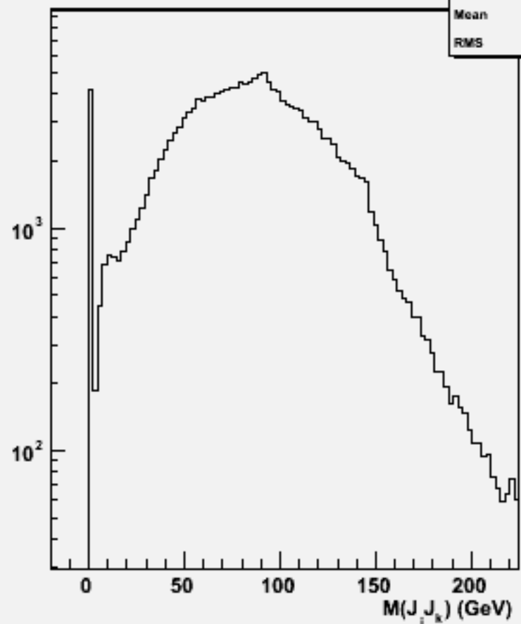
2jets mass(All comb)w104567 cch_o
