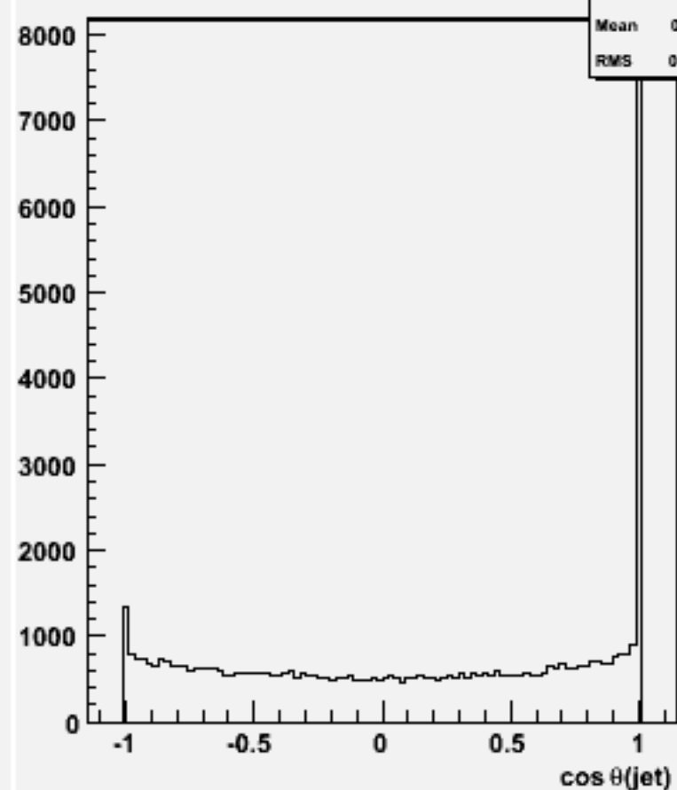
cos \theta for 2-jets :w104567 cch_o
