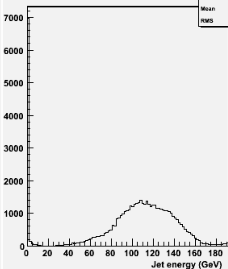
energy for 2-jets :w104567 cch_o
