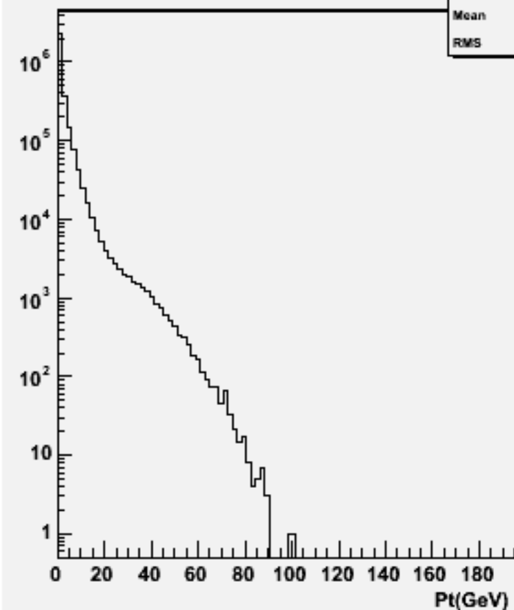
Start point Z : w104567 cch_o
