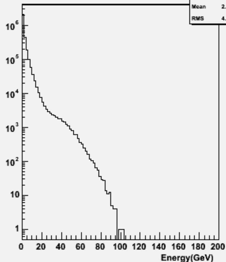
Start point R : w104567 cch_o
