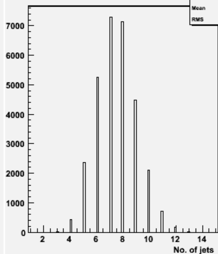
No. jets (ycut=0.001) : w104567 cch_o
