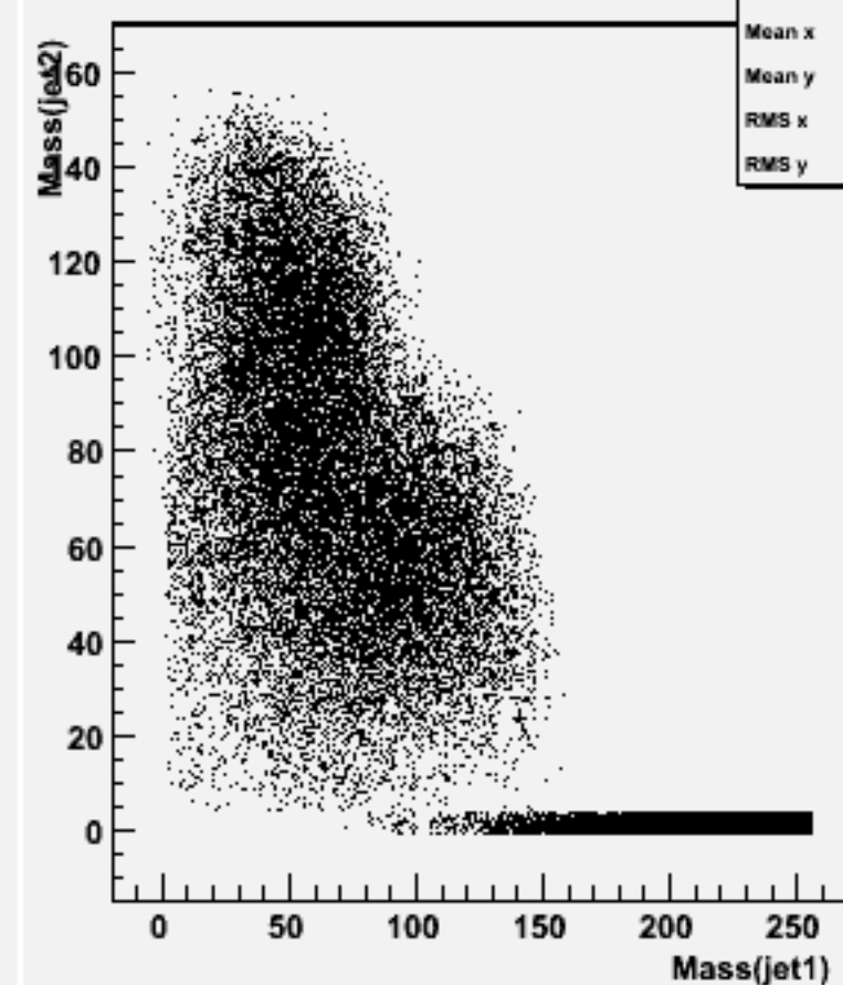
Jet mass for forced 2-jets : w104567 cch_o
