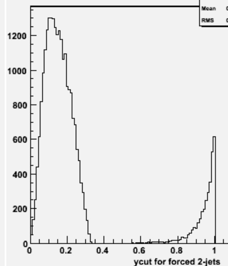
Ycut for 2-jets :w104567 cch_o
