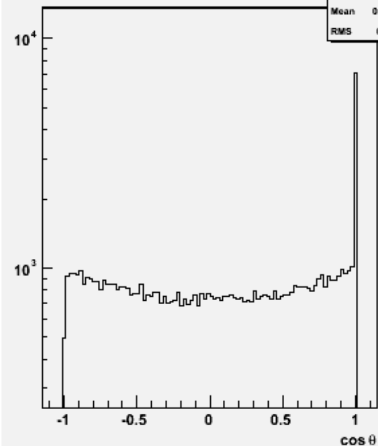
Jet cos \theta (All jets)w104564 uuh_o
