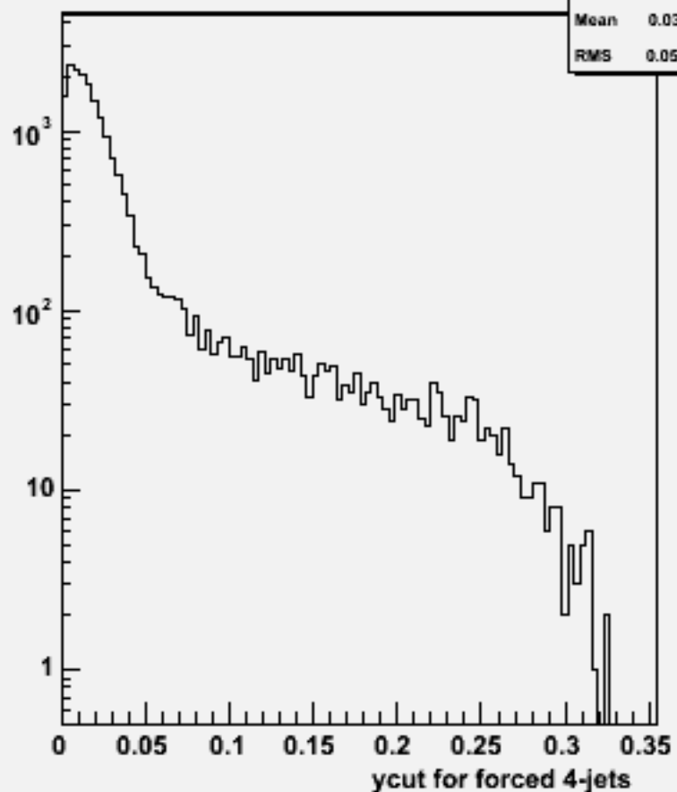
Ycut for 4-jets :w104564 uuh_o
