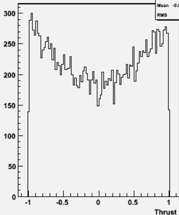
cos \Theta (thrust) w104564 uuh_o
