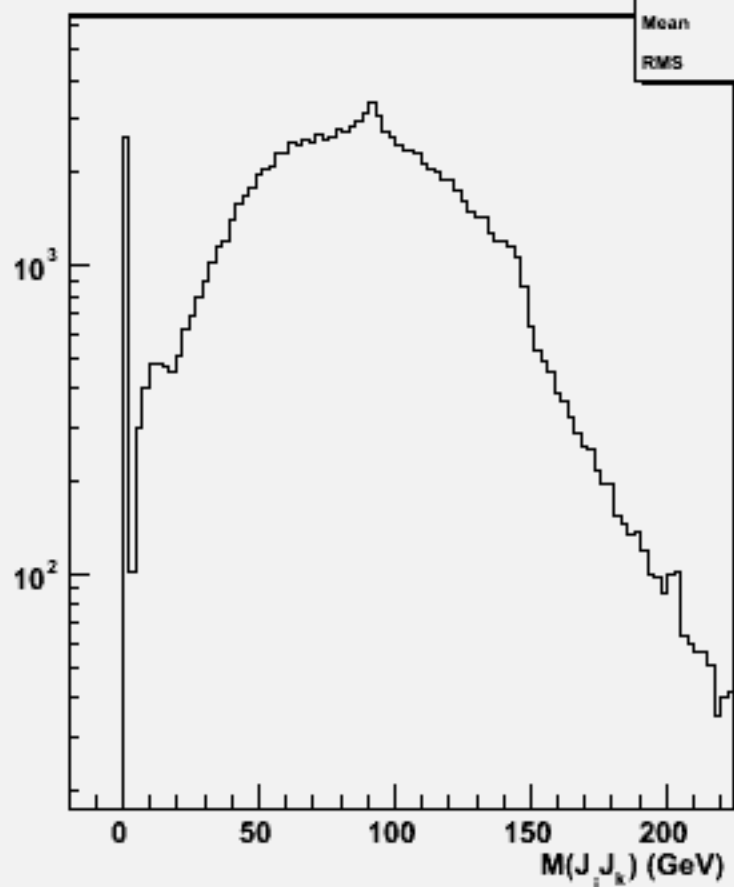
2jets mass(All comb)w104564 uuh_o
