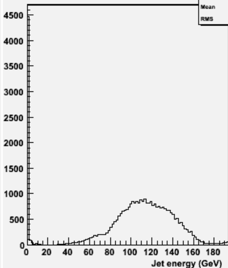
energy for 2-jets :w104564 uuh_o
