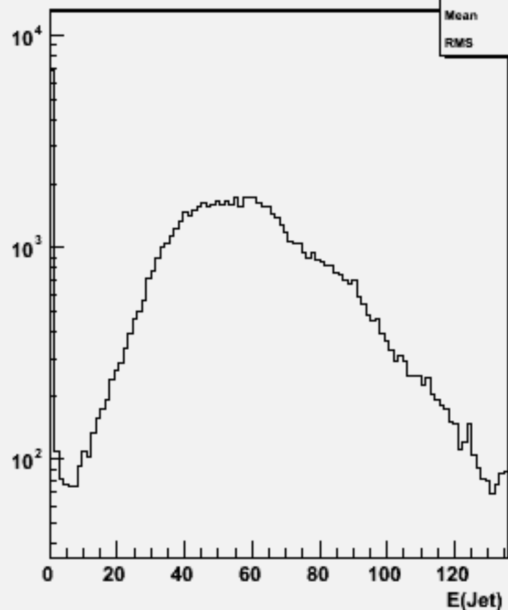
Jet energies(All jets)w104564 uuh_o
