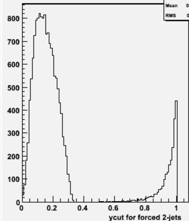
Ycut for 2-jets :w104564 uuh_o
