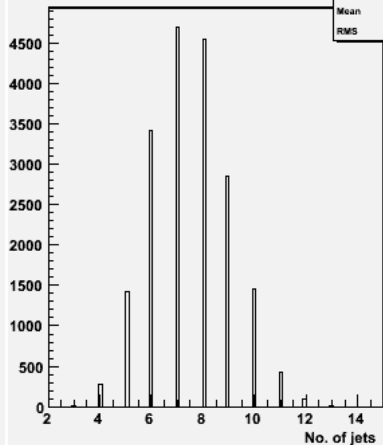
No. jets (ycut=0.001) : w104564 uuh_o
