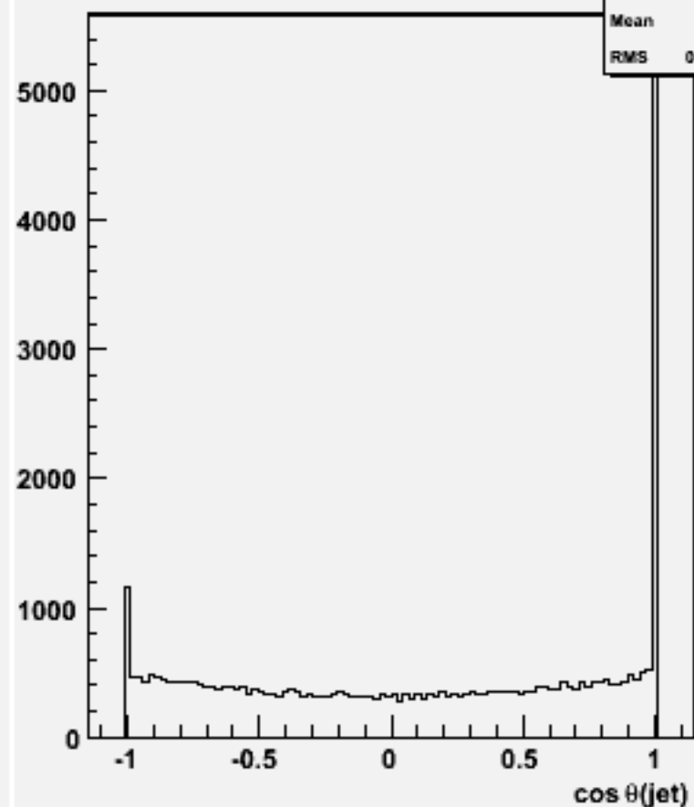
cos \theta for 2-jets :w104564 uuh_o
