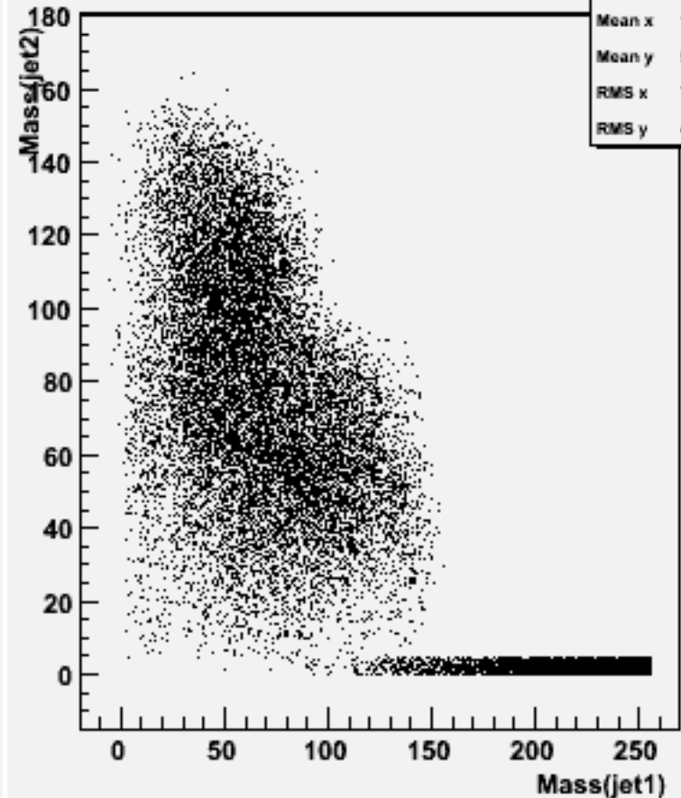
Jet mass for forced 2-jets : w104564 uuh_o
