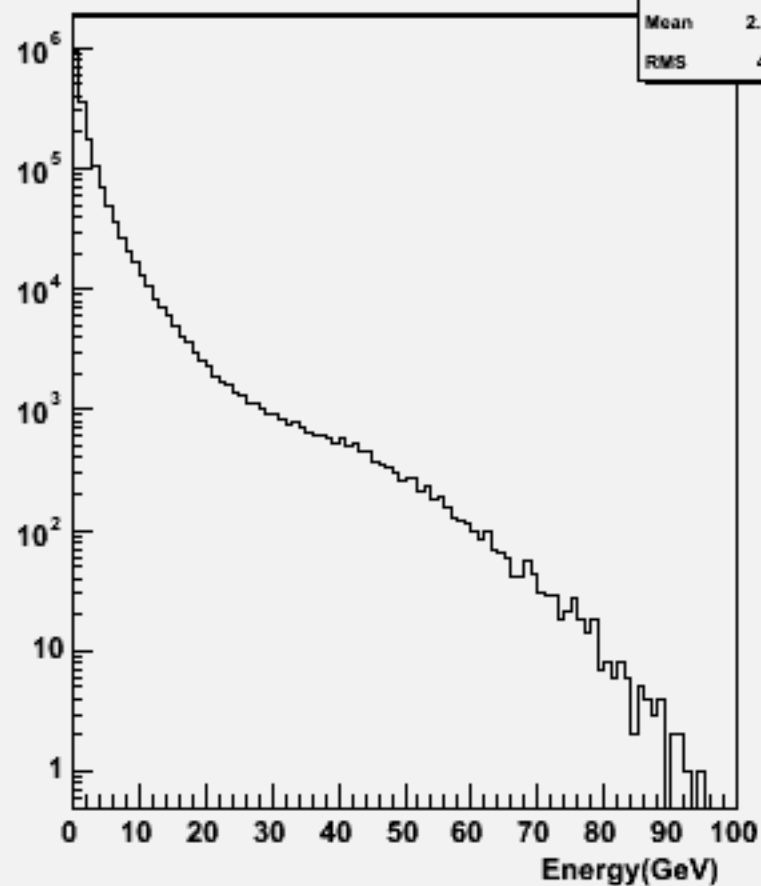
Particle Energy : w104564 uuh_o
