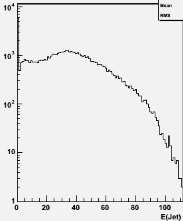
Jet energies(All jets)w104559 n3n3h_o
