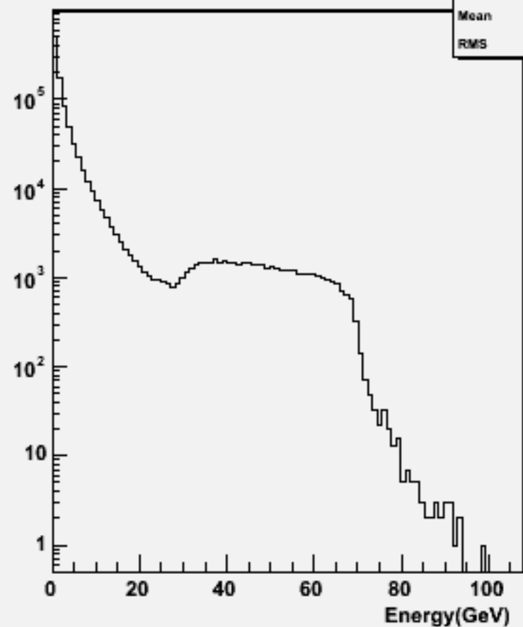
Particle Energy : w104559 n3n3h_o
