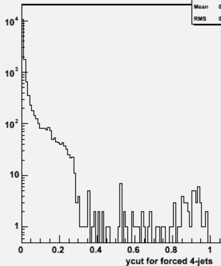
Ycut for 4-jets :w104559 n3n3h_o
