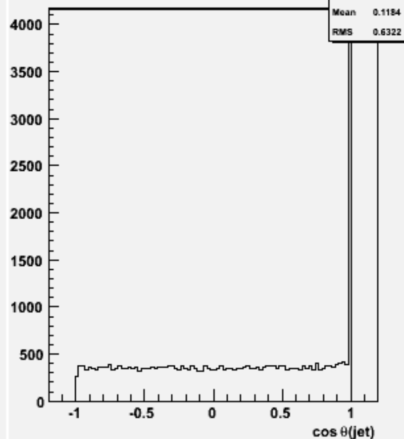
cos \theta for 2-jets :w104559 n3n3h_o
