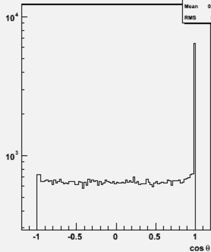
Jet cos \theta (All jets)w104559 n3n3h_o
