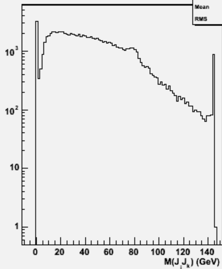
2jets mass(All comb)w104559 n3n3h_o
