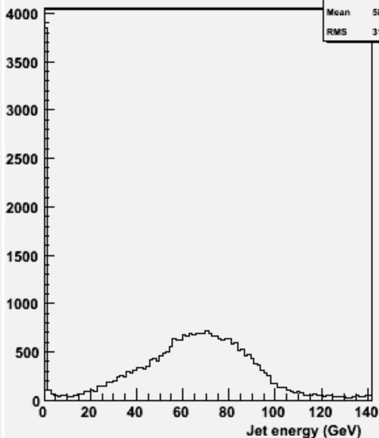
energy for 2-jets :w104559 n3n3h_o
