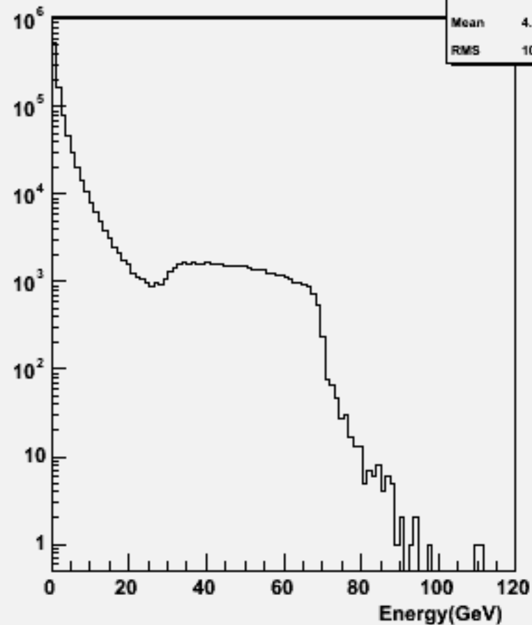
Particle Energy : w104555 n2n2h_o
