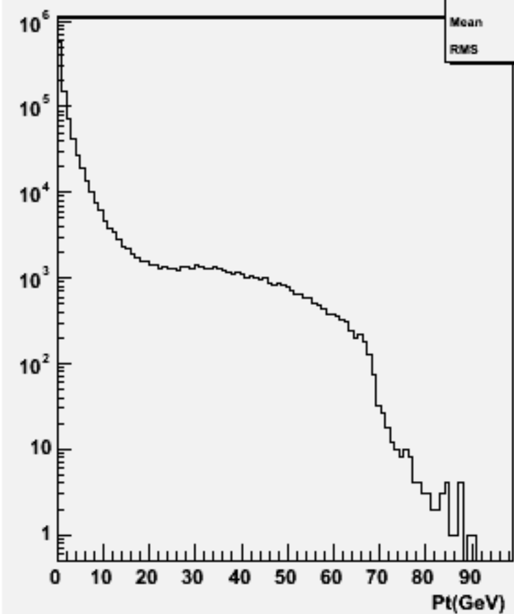
Particle Pt : w104555 n2n2h_o
