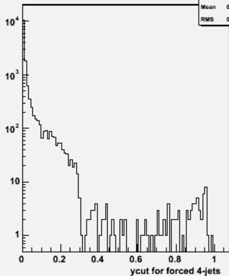
Ycut for 4-jets :w104555 n2n2h_o
