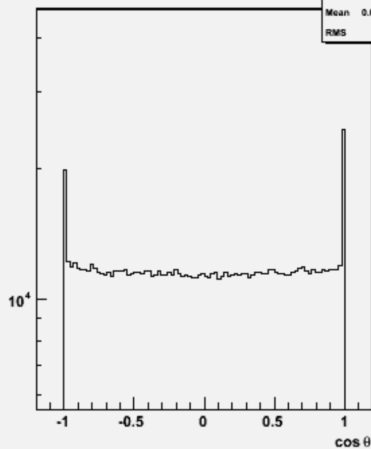
Particle cosθ : w104555 n2n2h_o
