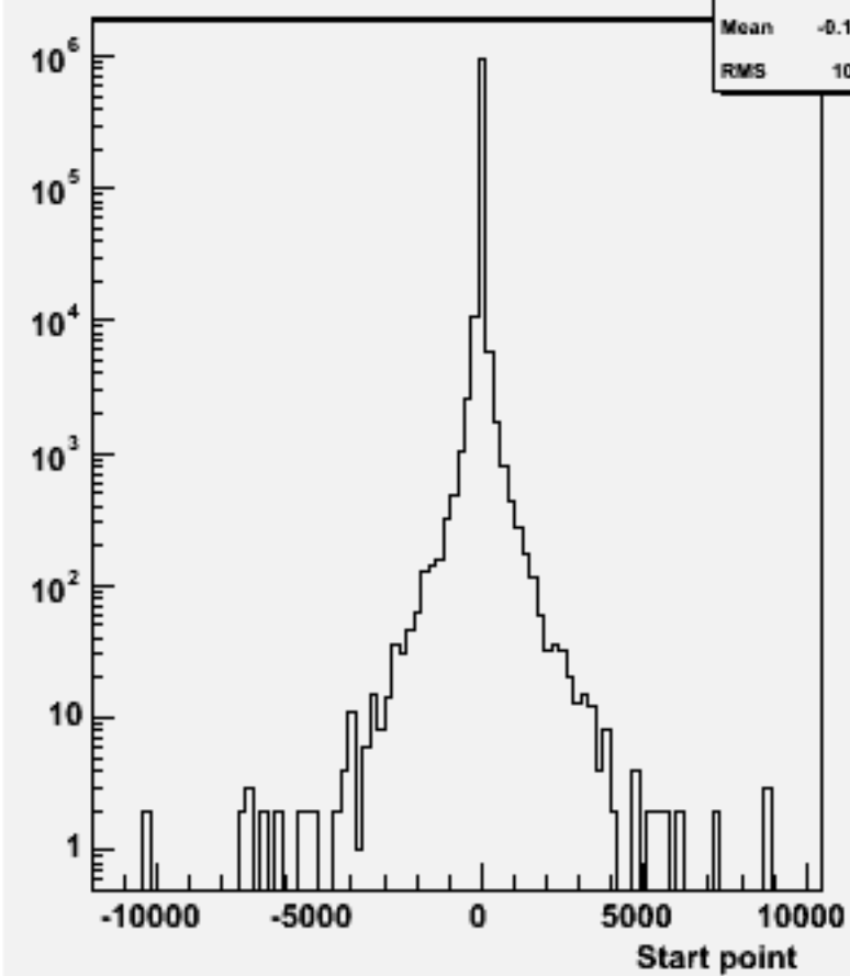
Start point Z : w104555 n2n2h_o
