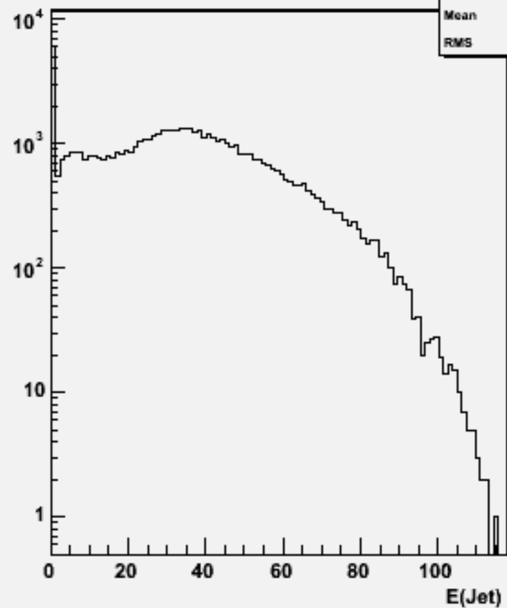
Jet energies(All jets)w104555 n2n2h_o
