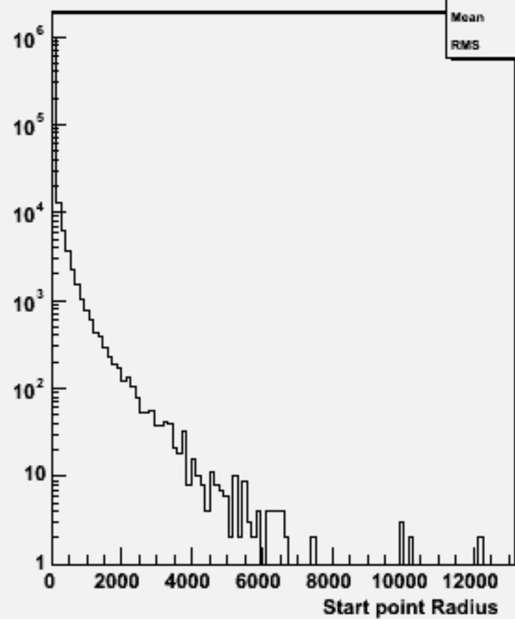
Start point R : w104555 n2n2h_o
