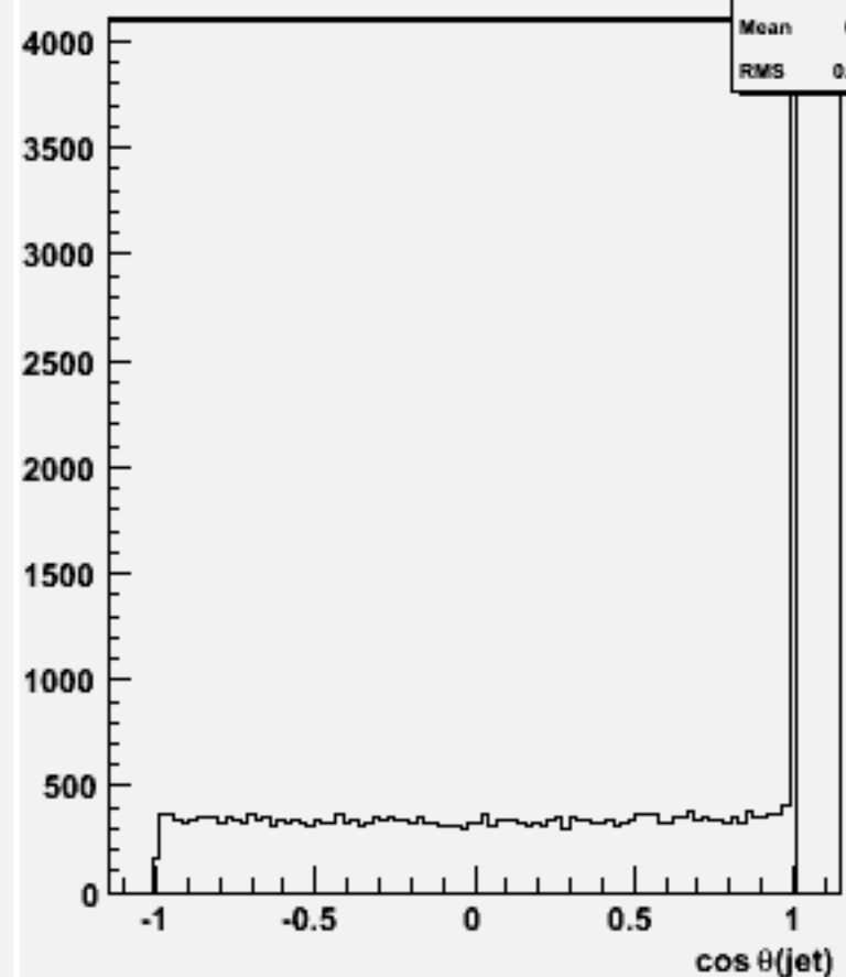
cos \theta for 2-jets :w104555 n2n2h_o
