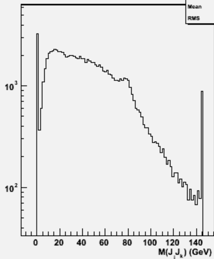
2jets mass(All comb)w104555 n2n2h_o
