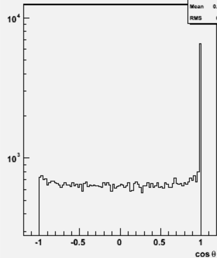
Jet cos \theta (All jets)w104555 n2n2h_o
