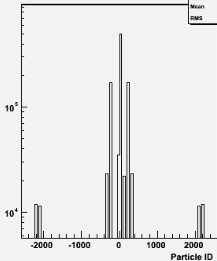
Particle ID : w104555 n2n2h_o
