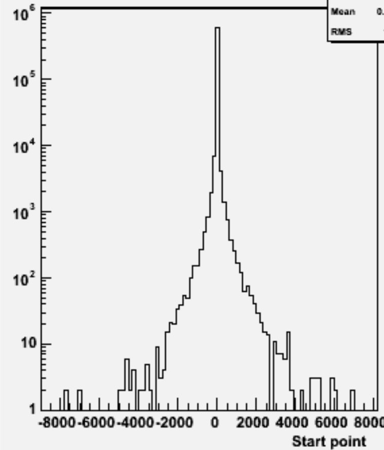
Start point Z : w104552 n1n1h_o
