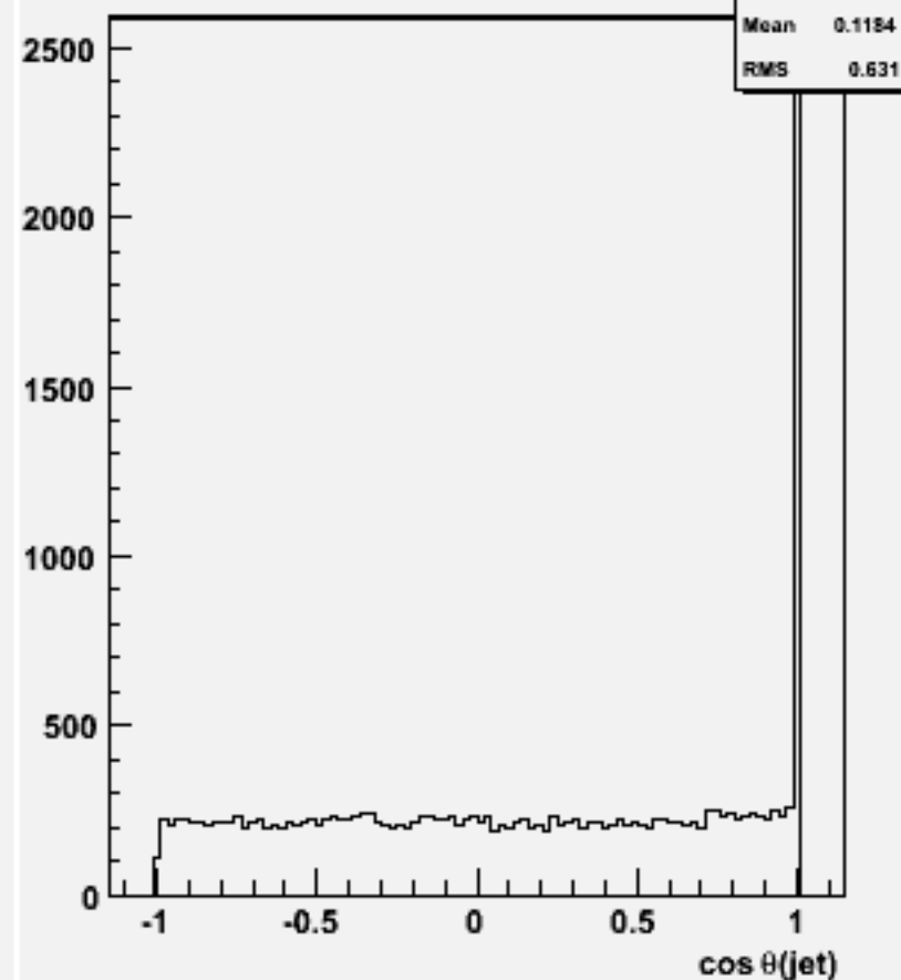
cos \theta for 2-jets :w104552 n1n1h_o
