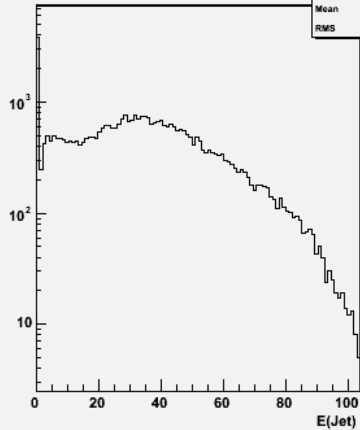
Jet energies(All jets)w104552 n1n1h_o
