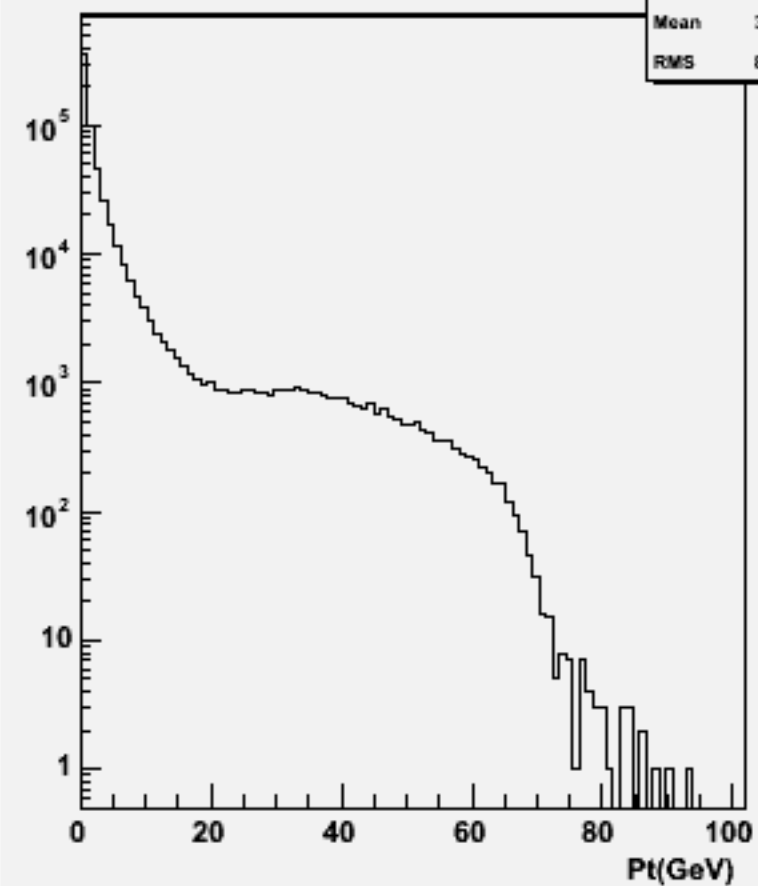
Particle Pt : w104552 n1n1h_o
