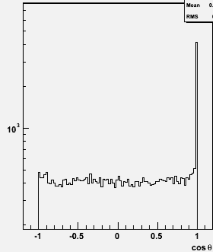
Jet cos \theta (All jets)w104552 n1n1h_o
