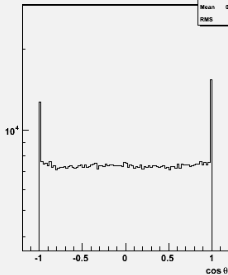
Particle cos \theta : w104552 n1n1h_o
