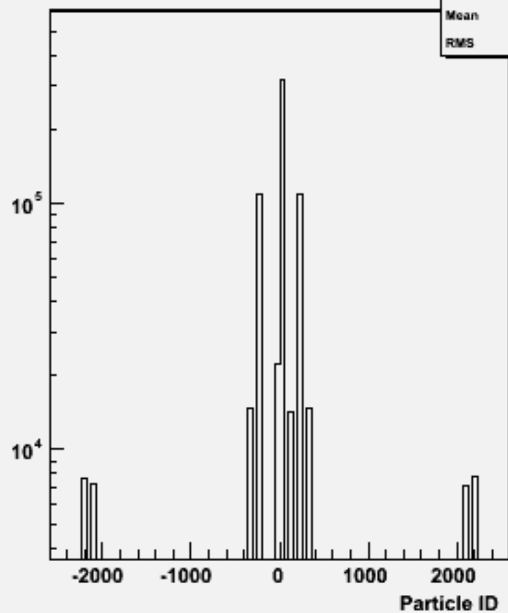
Particle ID : w104552 n1n1h_o
