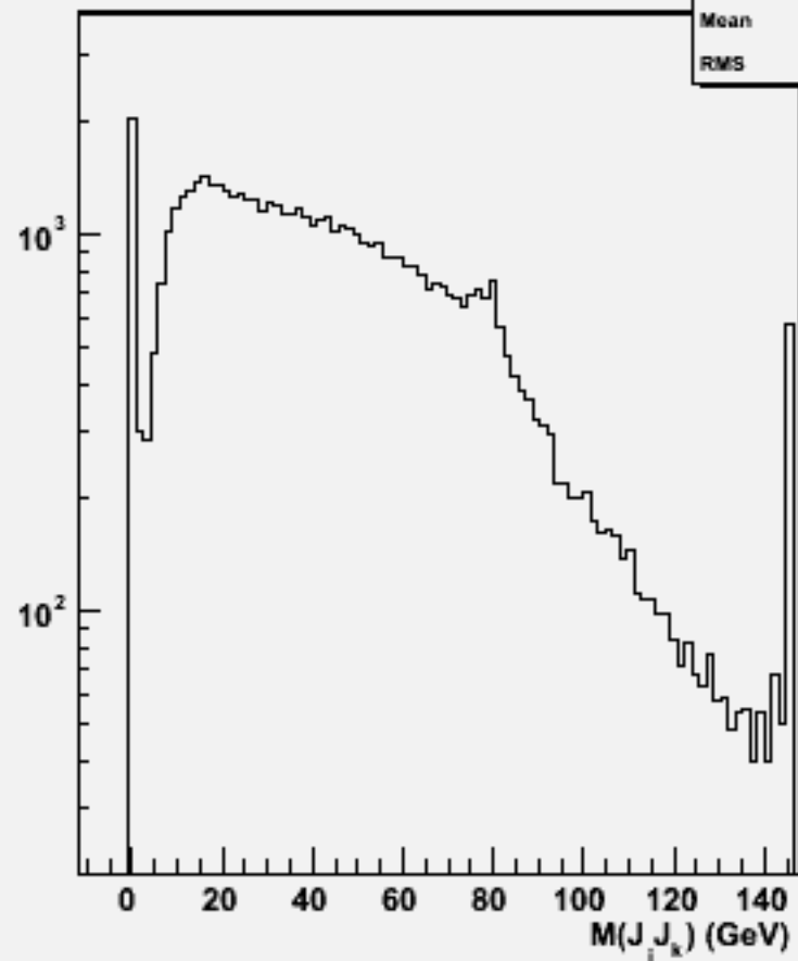
2jets mass(All comb)w104552 n1n1h_o
