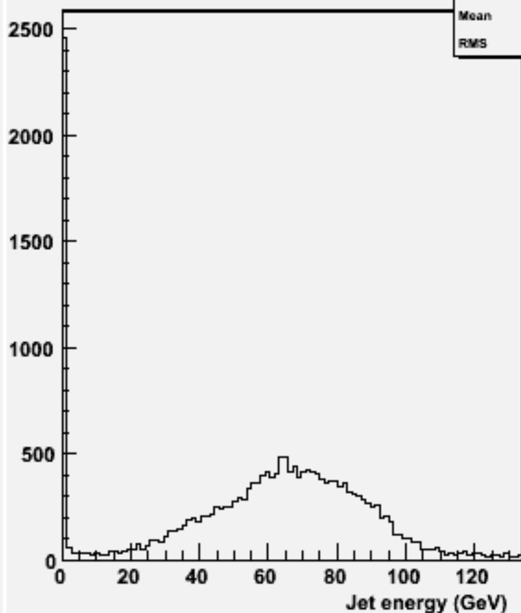
energy for 2-jets :w104552 n1n1h_o
