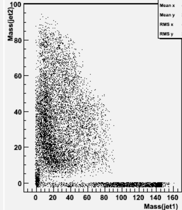
Jet mass for forced 2-jets : w104552 n1n1h_o
