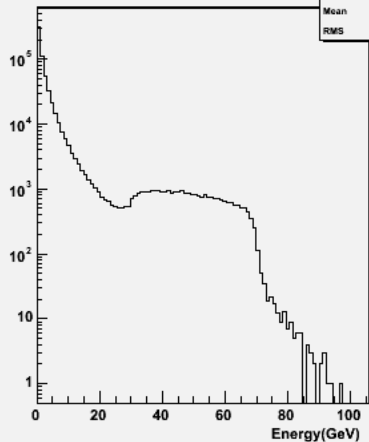
Particle Energy : w104552 n1n1h_o
