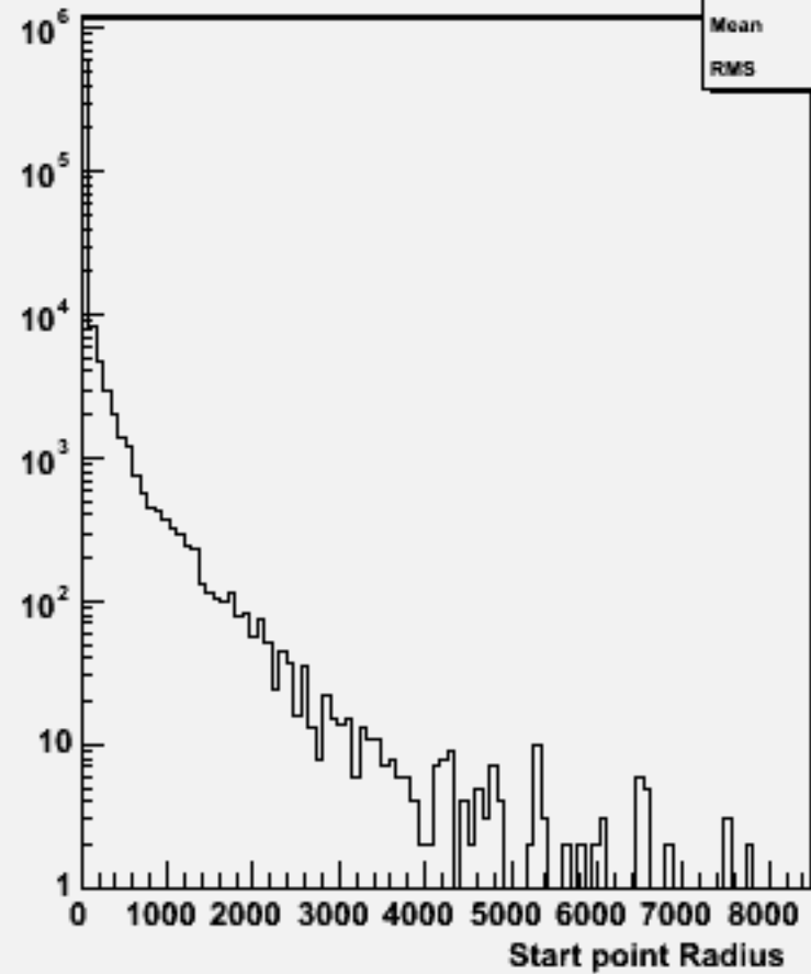
Start point R : w104552 n1n1h_o
