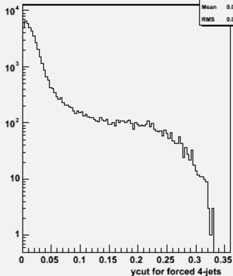
Ycut for 4-jets :w104541 bbh_o
