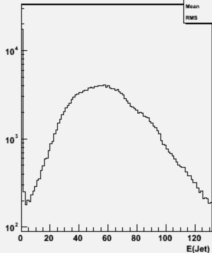
Jet energies(All jets)w104541 bbh_o
