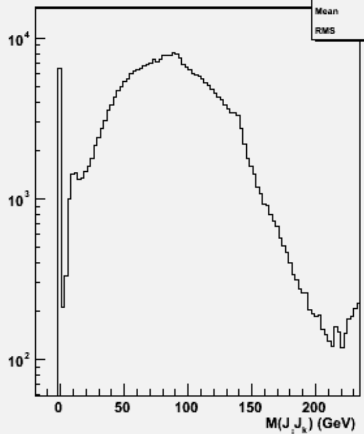
2jets mass(All comb)w104541 bbh_o
