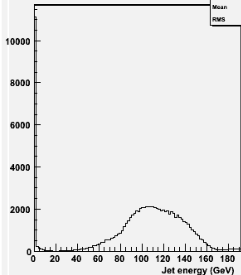
energy for 2-jets :w104541 bbh_o
