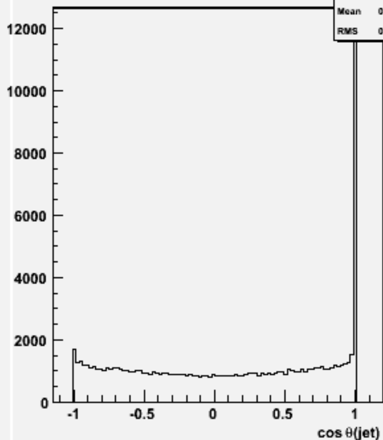
cos \theta for 2-jets :w104541 bbh_o
