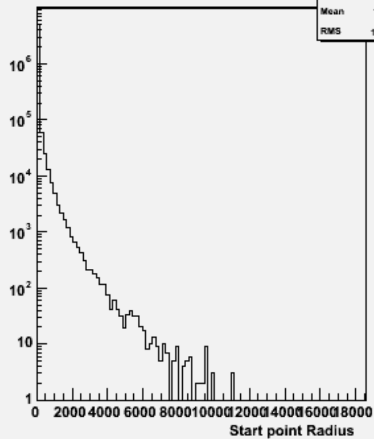
Start point R : w104541 bbh_o
