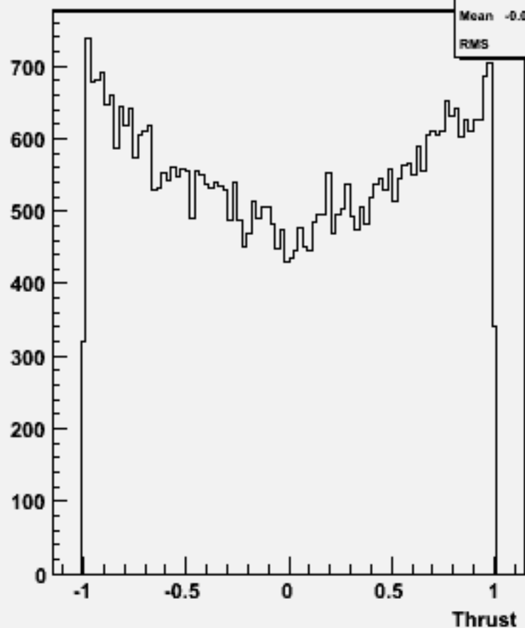
cos \Theta (thrust) w104541 bbh_o
