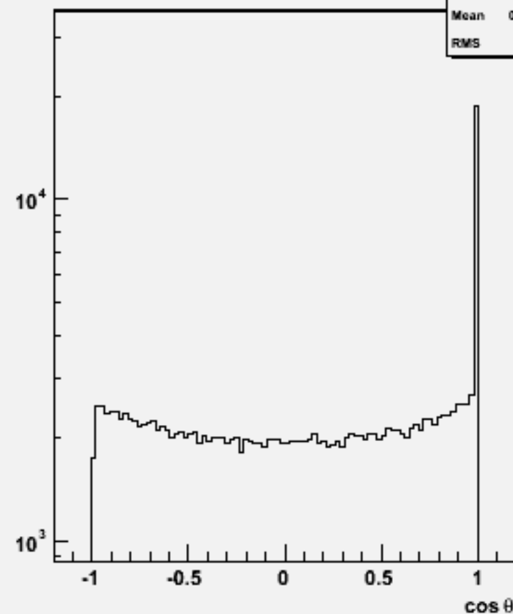
Jet cos \theta (All jets)w104541 bbh_o
