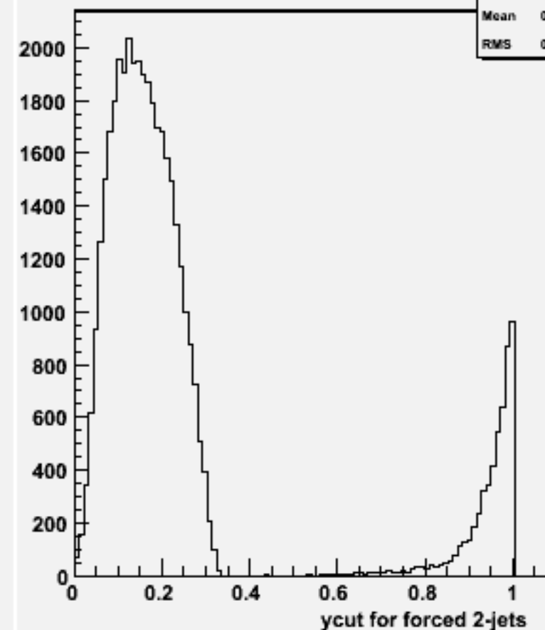
Ycut for 2-jets :w104541 bbh_o
