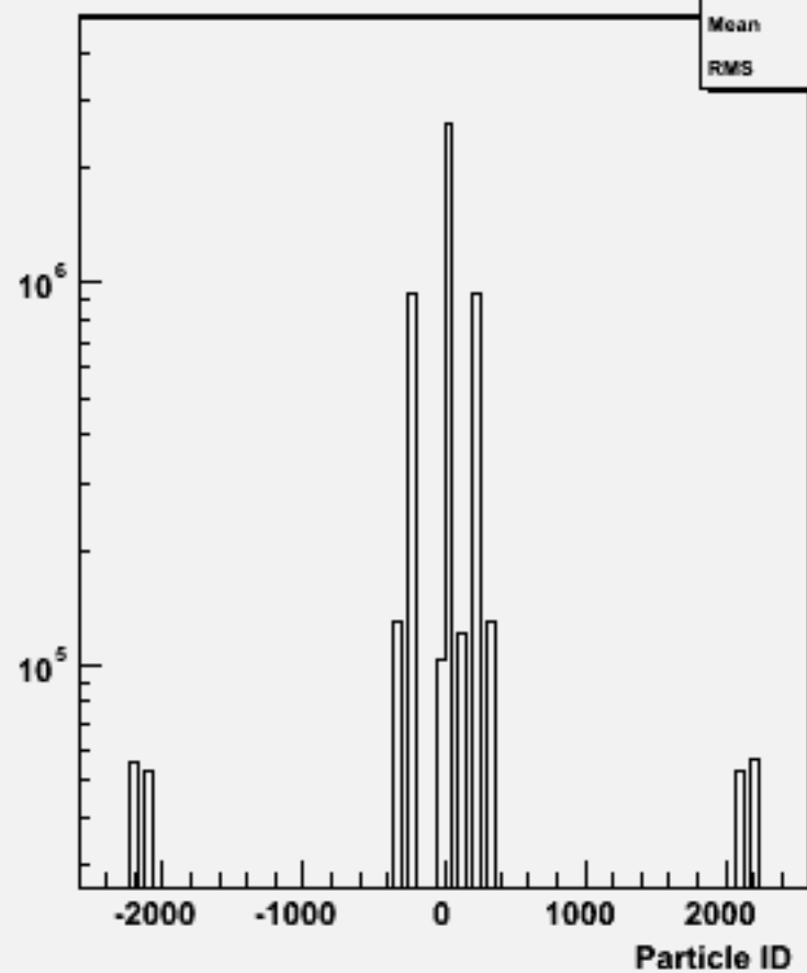
Particle ID : w104541 bbh_o
