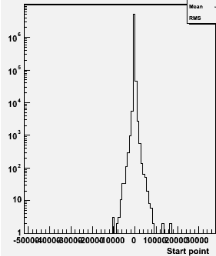
Start point Z : w104541 bbh_o
