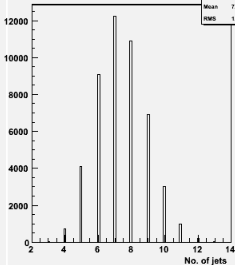
No. jets (ycut=0.001) : w104541 bbh_o
