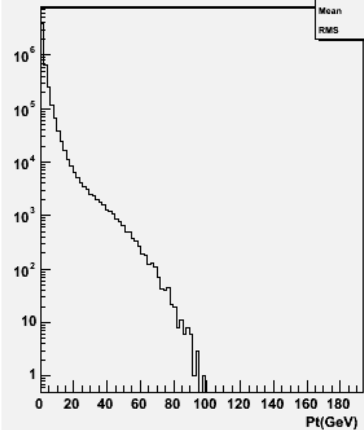
Particle Pt : w104541 bbh_o
