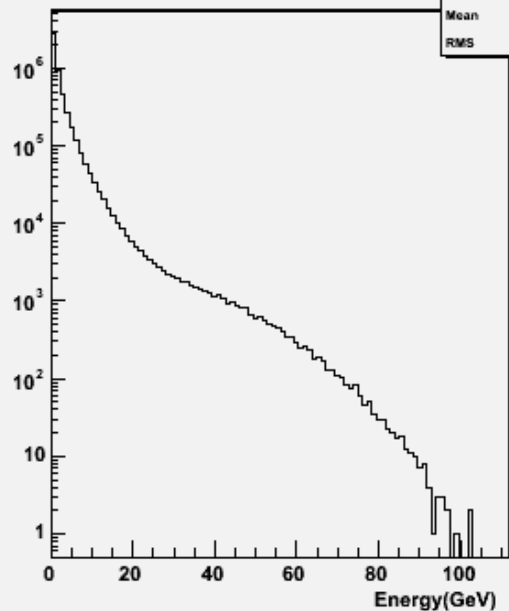
Particle Energy : w104541 bbh_o
