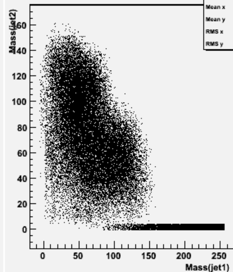
Jet mass for forced 2-jets : w104541 bbh_o
