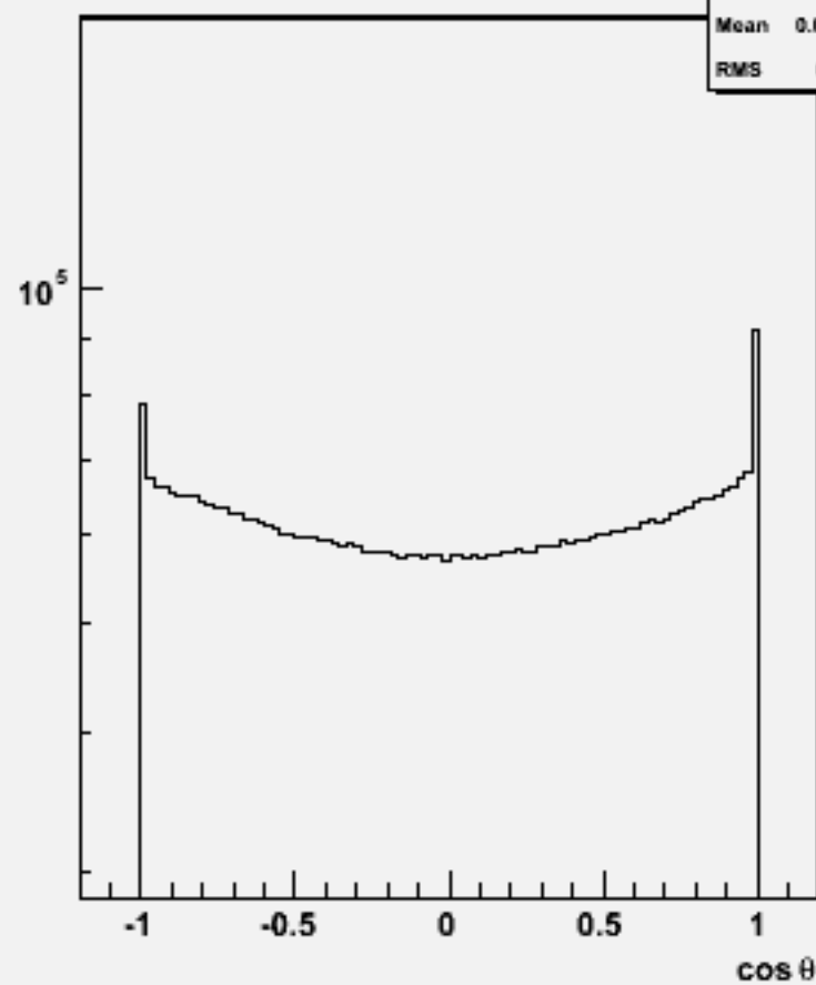
Particle cosθ : w104541 bbh_o
