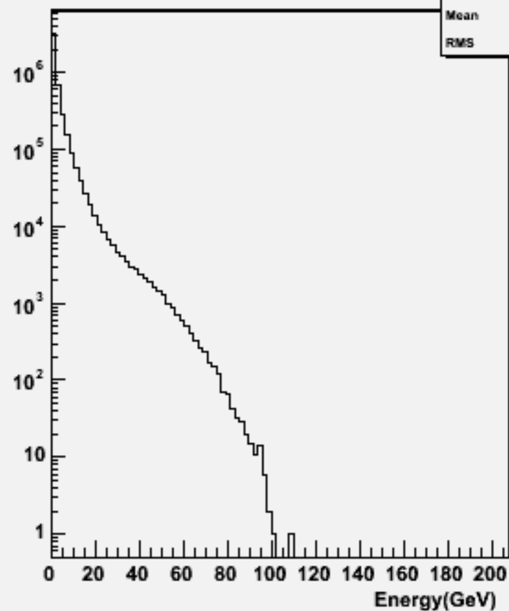
Start point R : w104537 ssh_o
