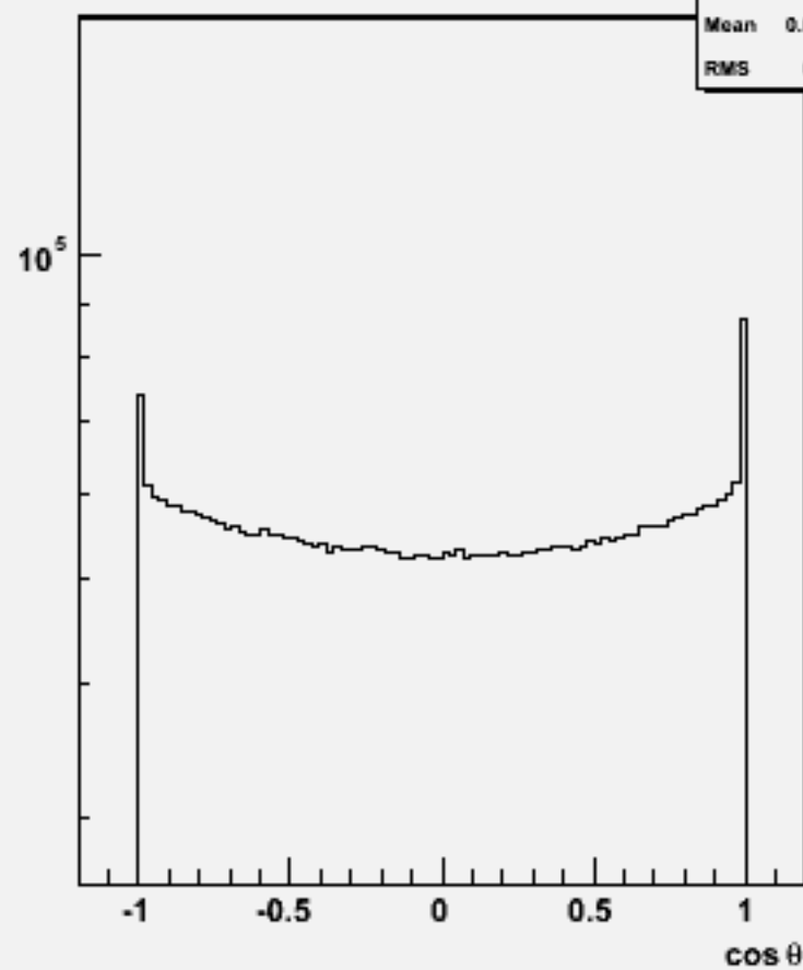
Particle \cos\theta : w104537 ssh_o
