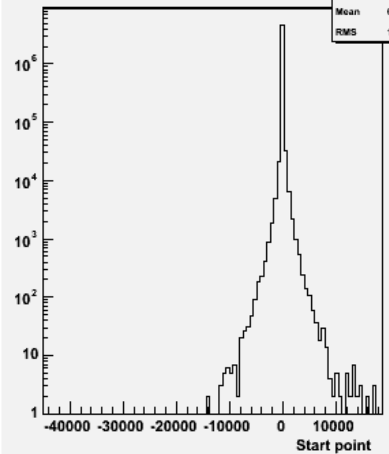
Start point Z : w104537 ssh_o
