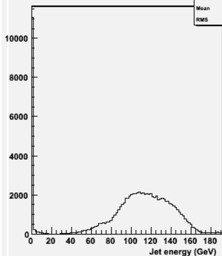
energy for 2-jets :w104537 ssh_o
