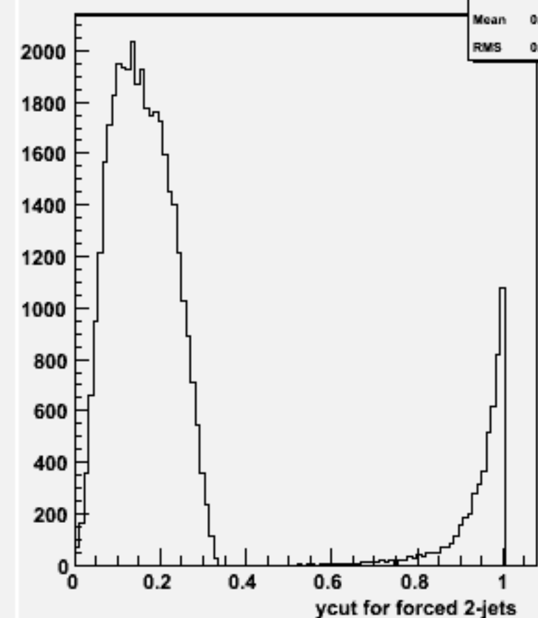
Ycut for 2-jets :w104537 ssh_o
