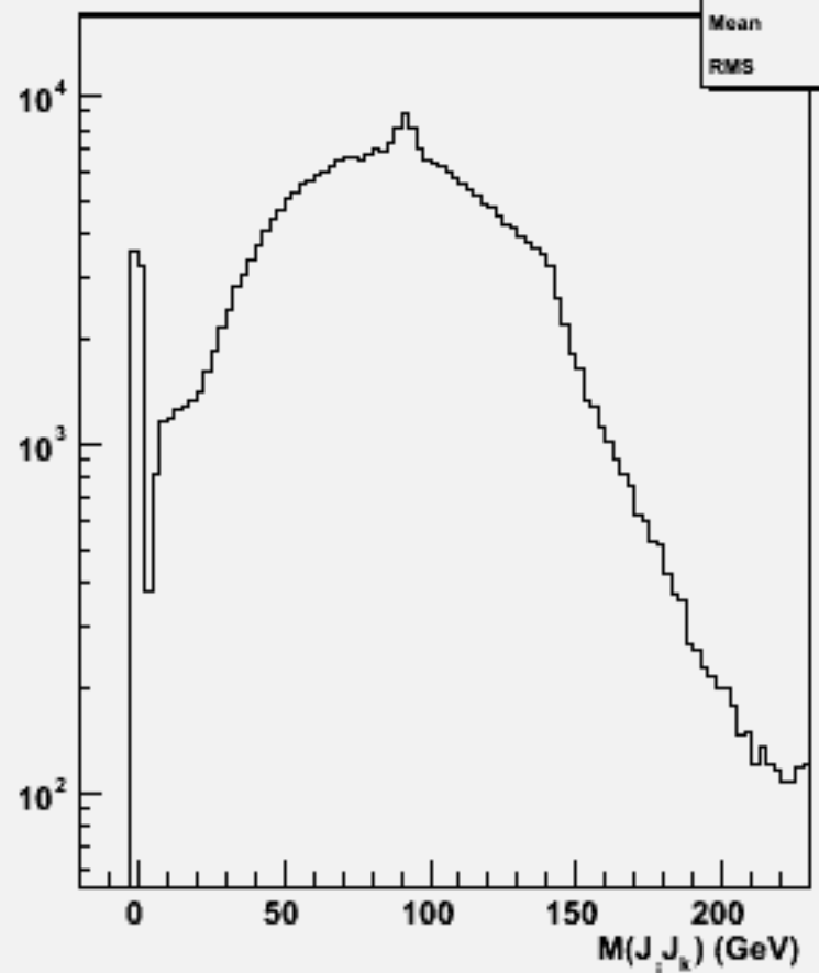
2jets mass(All comb)w104537 ssh_o
