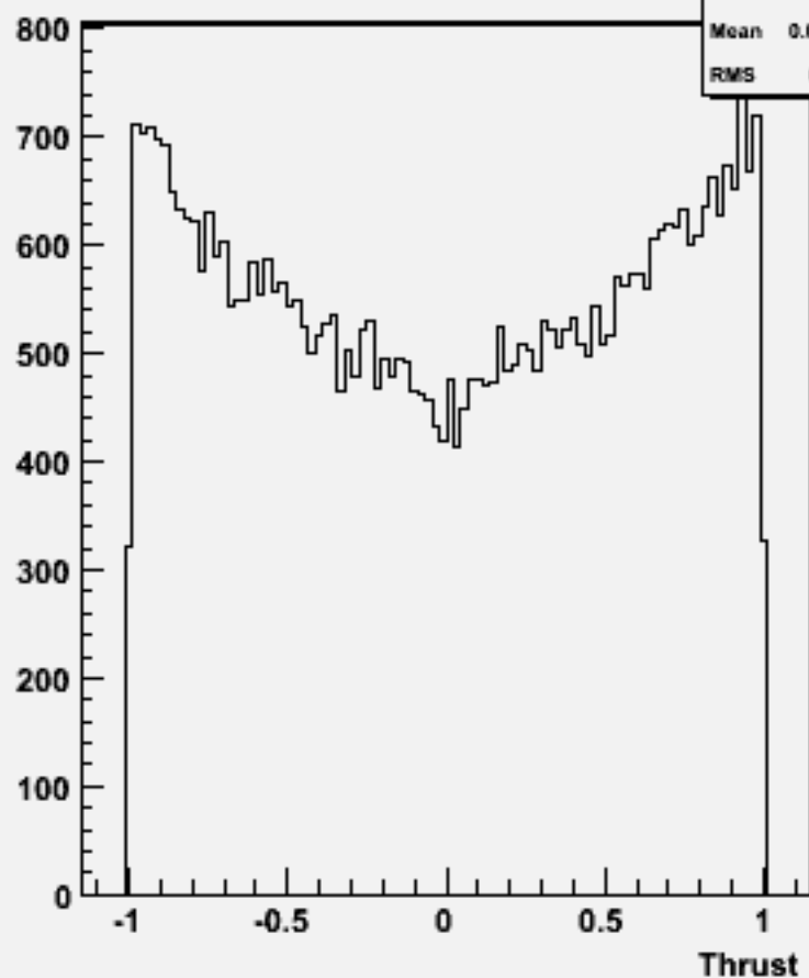
cos \Theta (thrust) w104537 ssh_o
