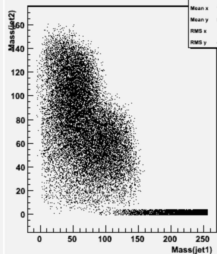
Jet mass for forced 2-jets : w104537 ssh_o
