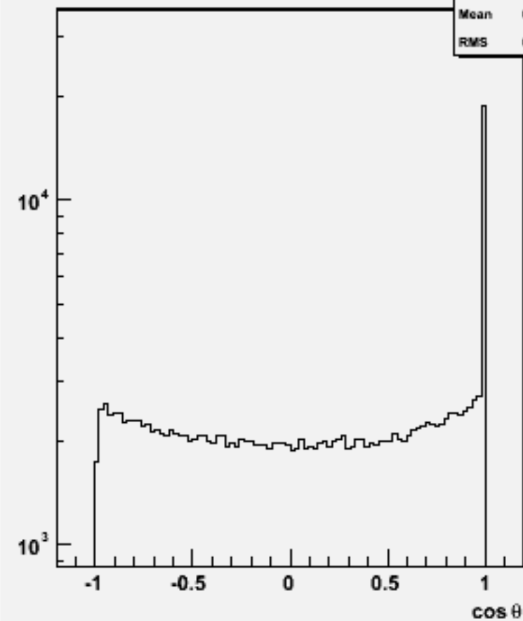
Jet cos \theta (All jets)w104537 ssh_o
