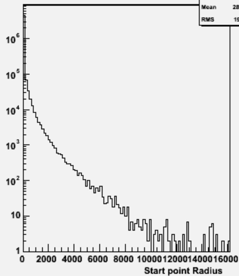
Start point R : w104537 ssh_o
