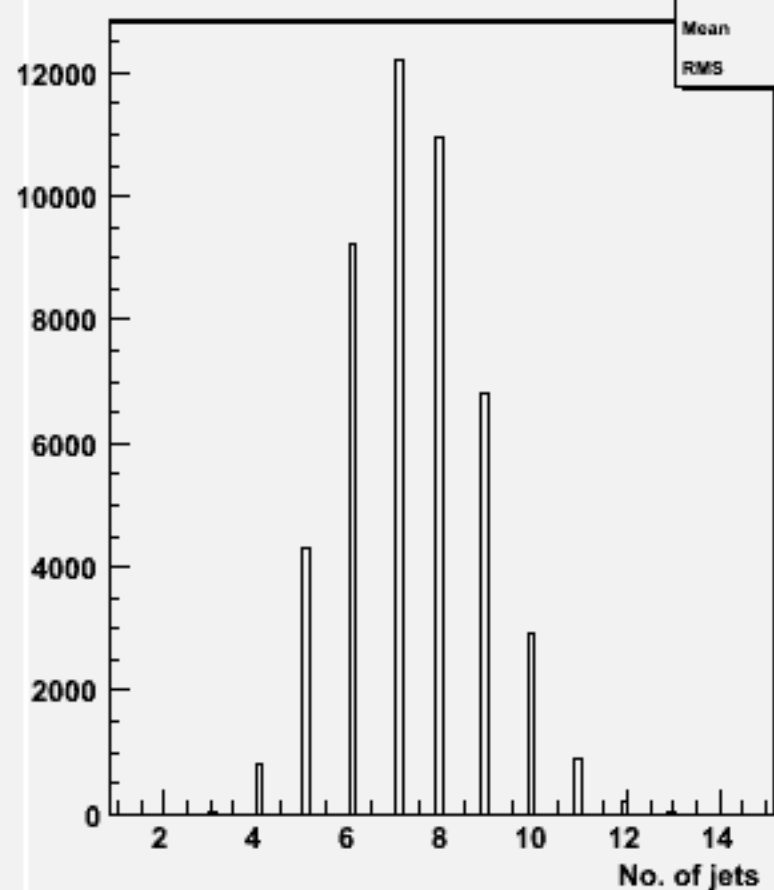
No. jets (ycut=0.001) : w104537 ssh_o
