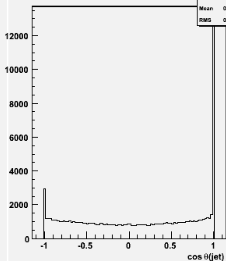
cos \theta for 2-jets :w104537 ssh_o
