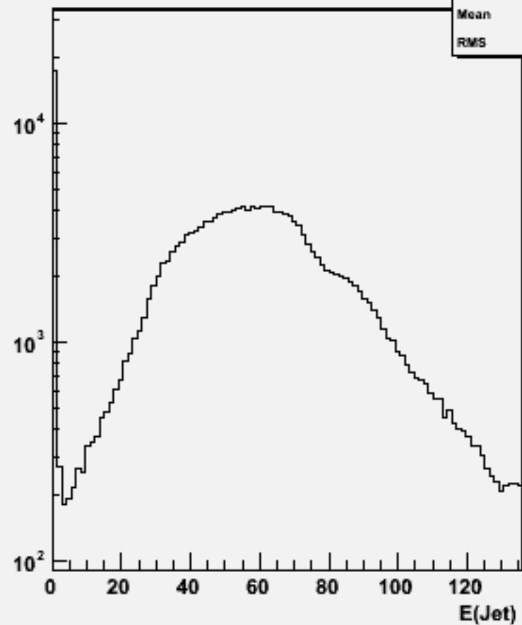
Jet energies(All jets)w104537 ssh_o
