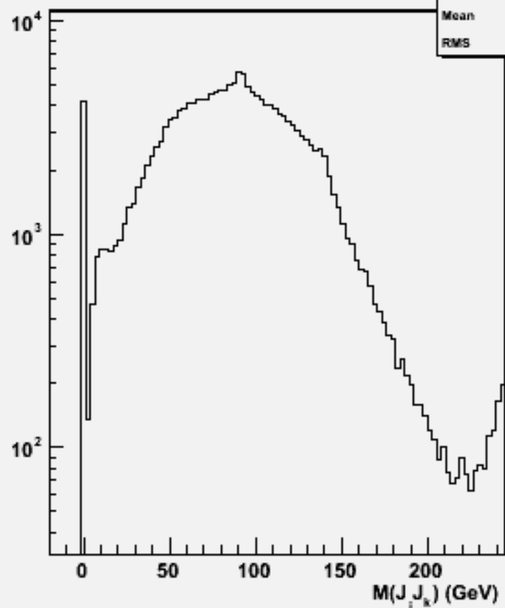
2jets mass(All comb)w104534 ddh_o
