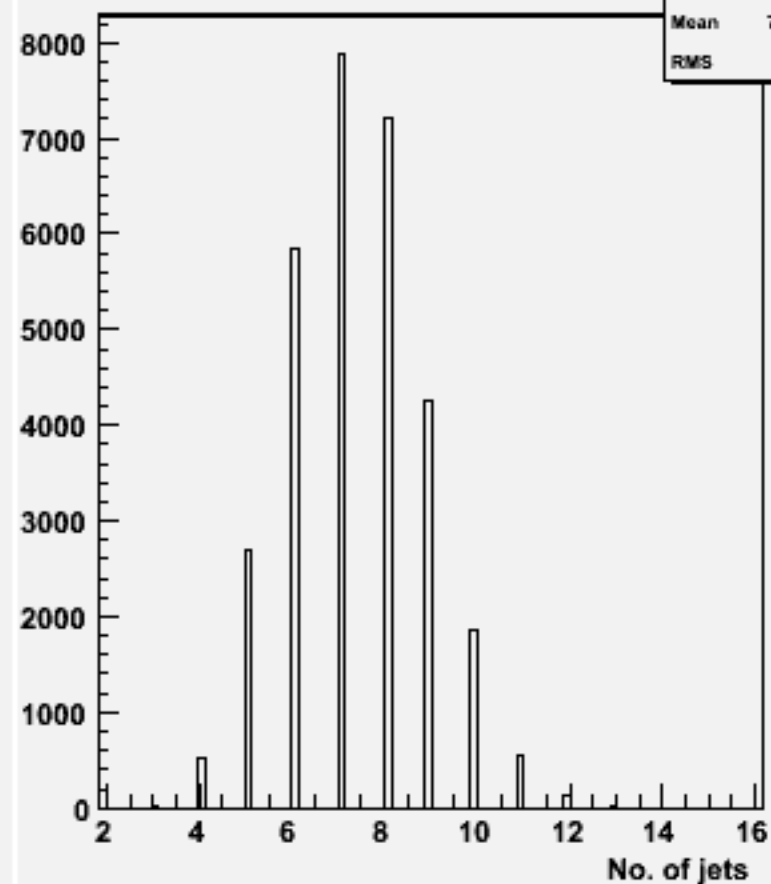
No. jets (ycut=0.001) : w104534 ddh_o
