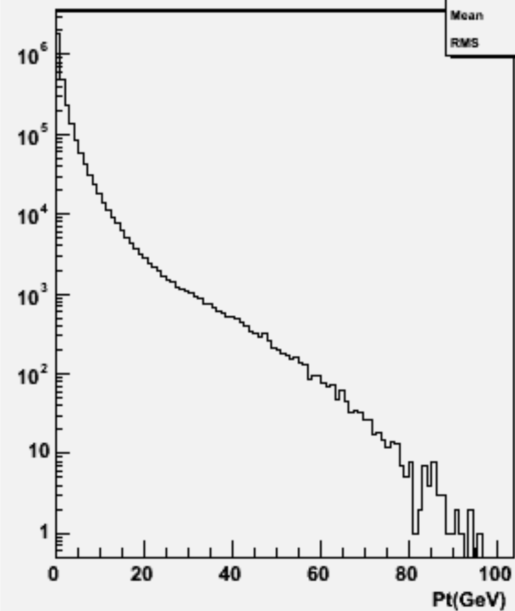
Particle Pt : w104534 ddh_o
