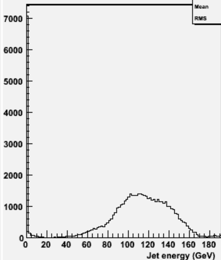
energy for 2-jets :w104534 ddh_o
