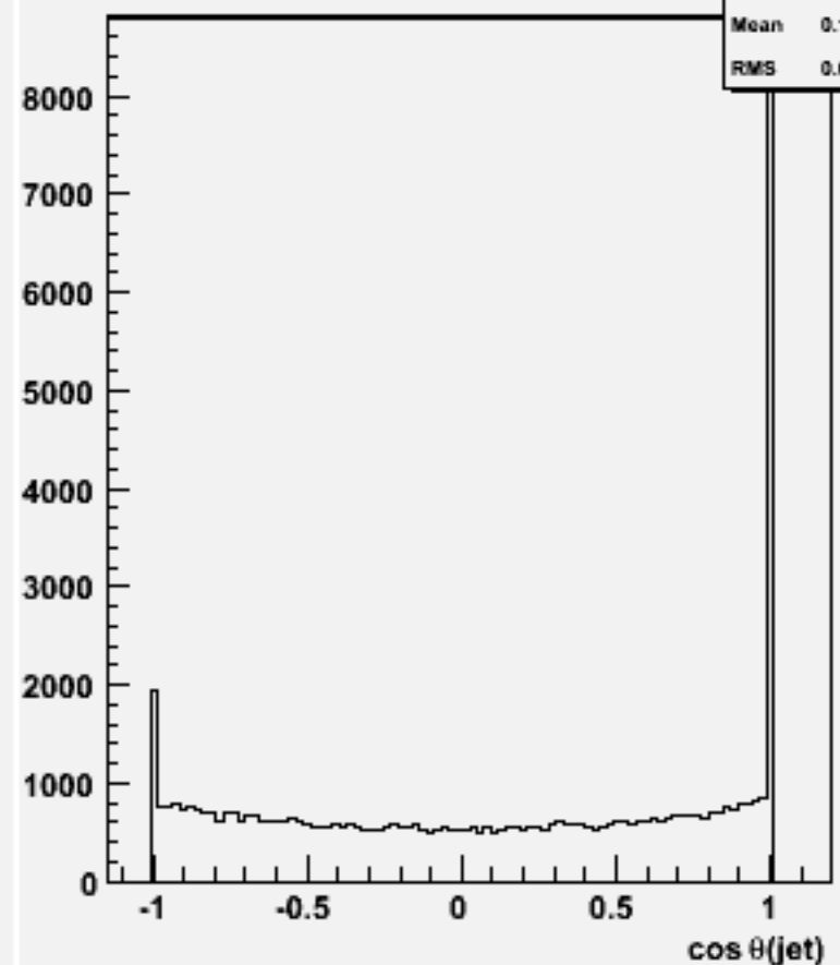
cos \theta for 2-jets :w104534 ddh_o
