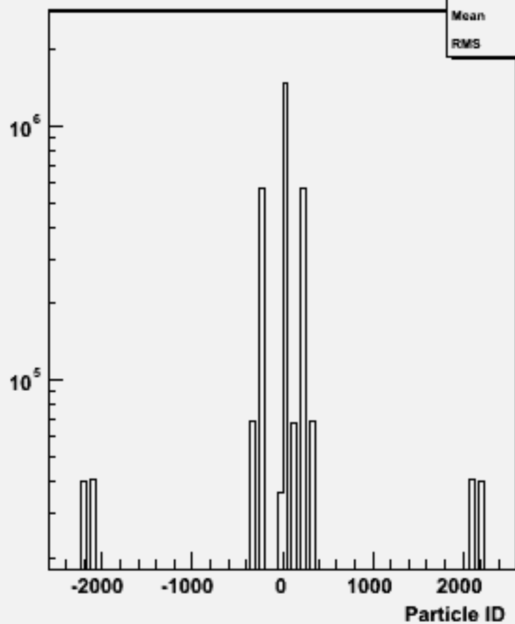
Particle ID : w104534 ddh_o
