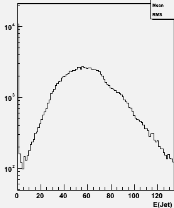
Jet energies(All jets)w104534 ddh_o
