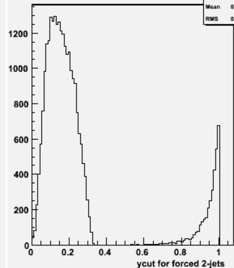
Ycut for 2-jets :w104534 ddh_o
