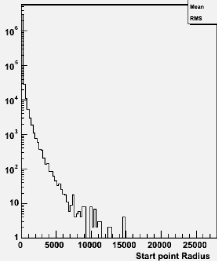
Start point R : w104534 ddh_o
