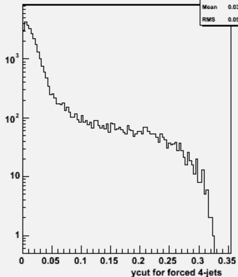
Ycut for 4-jets :w104534 ddh_o
