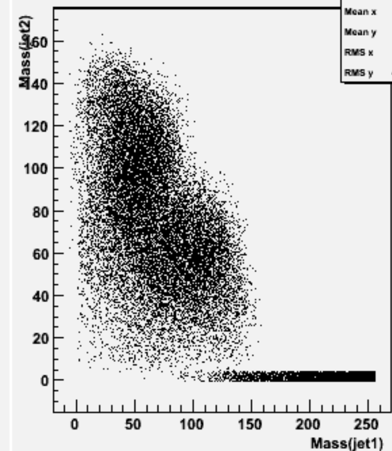
Jet mass for forced 2-jets : w104534 ddh_o
