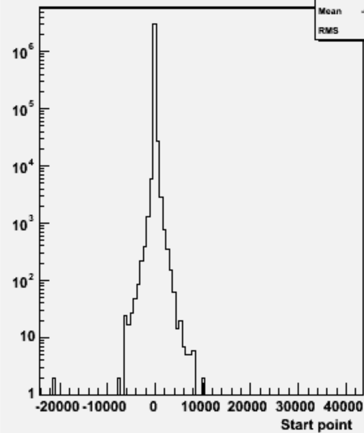
Start point Z : w104534 ddh_o
