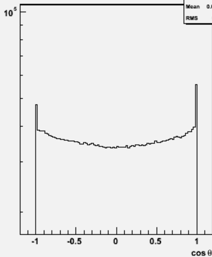
Particle \cos\theta : w104534 ddh_o
