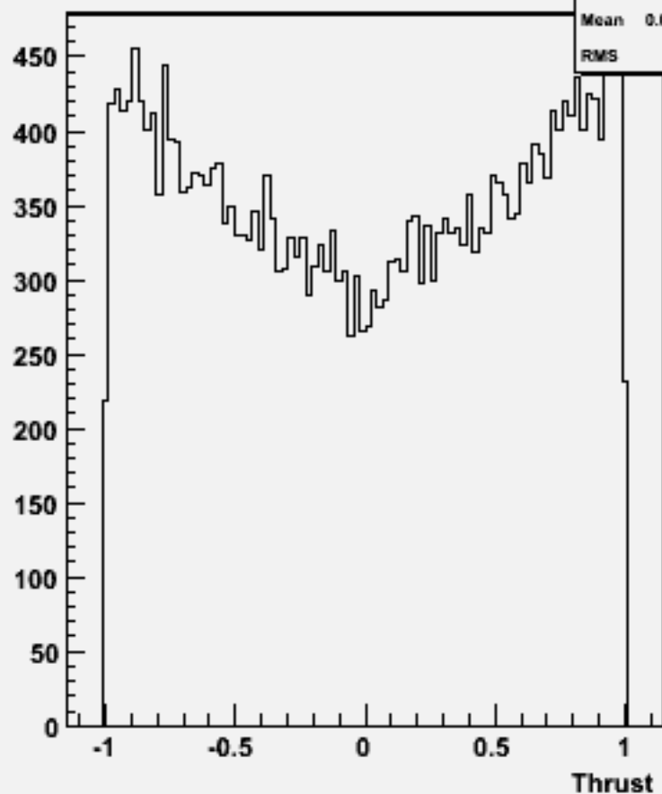
cos \Theta (thrust) w104534 ddh_o
