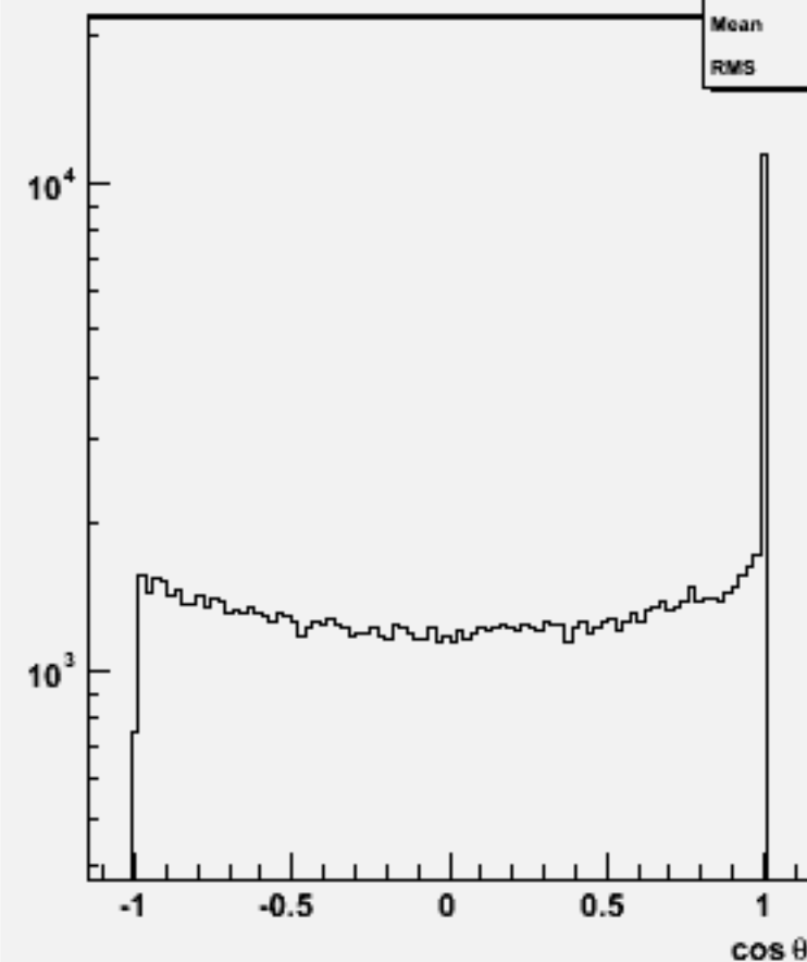
Jet cos \theta (All jets)w104534 ddh_o
