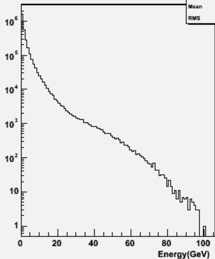
Particle Energy : w104534 ddh_o
