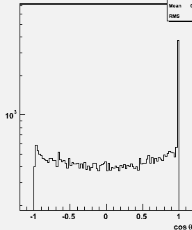
Jet cos \theta (All jets)w104530 e3e3h_o
