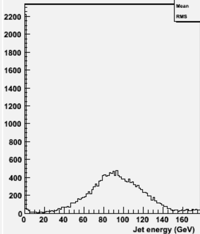
energy for 2-jets :w104530 e3e3h_o
