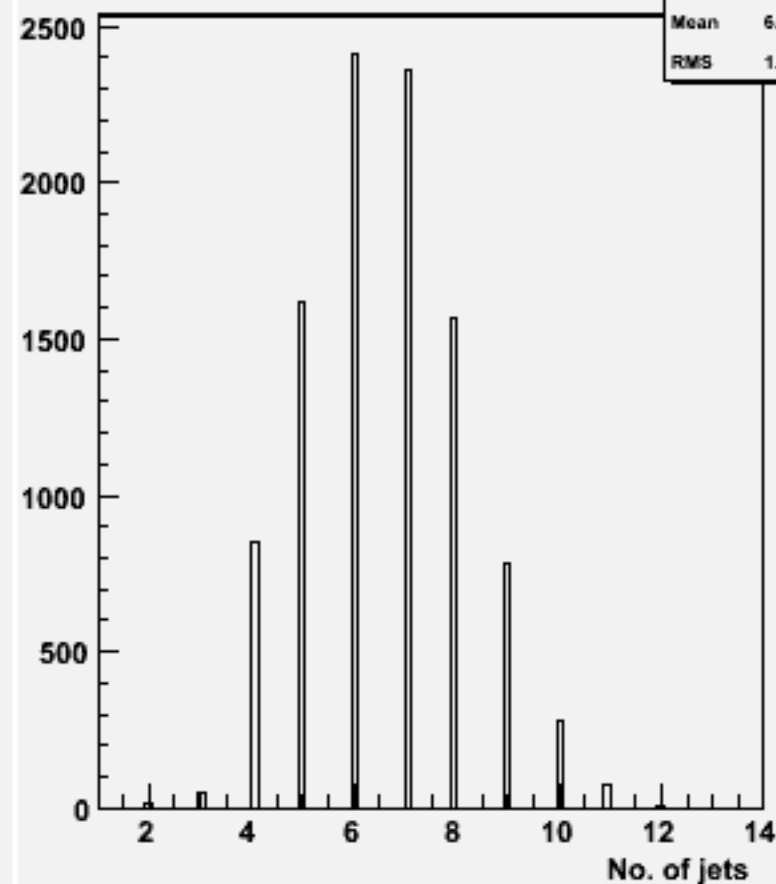
No. jets (ycut=0.001) : w104530 e3e3h_o
