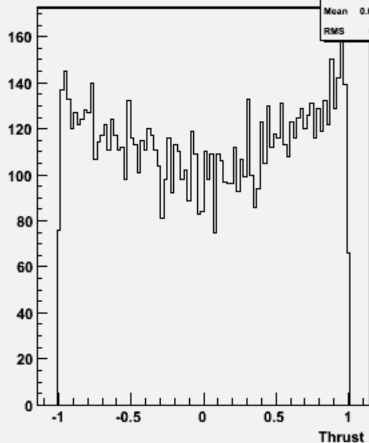
cos \Theta (thrust) w104530 e3e3h_o
