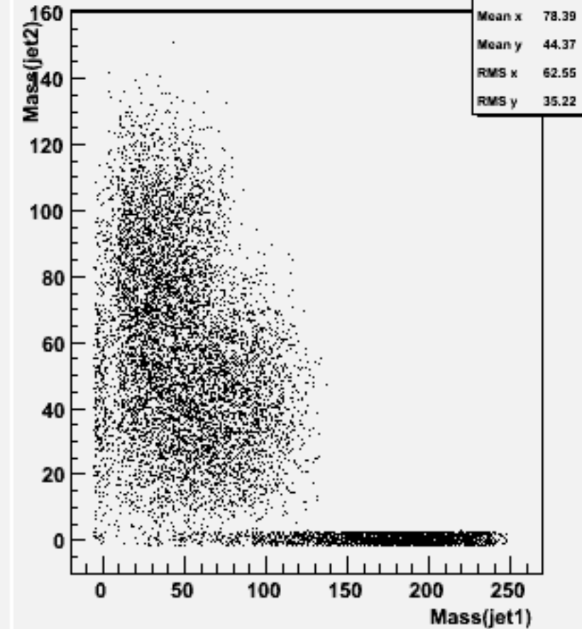
Jet mass for forced 2-jets : w104530 e3e3h_o
