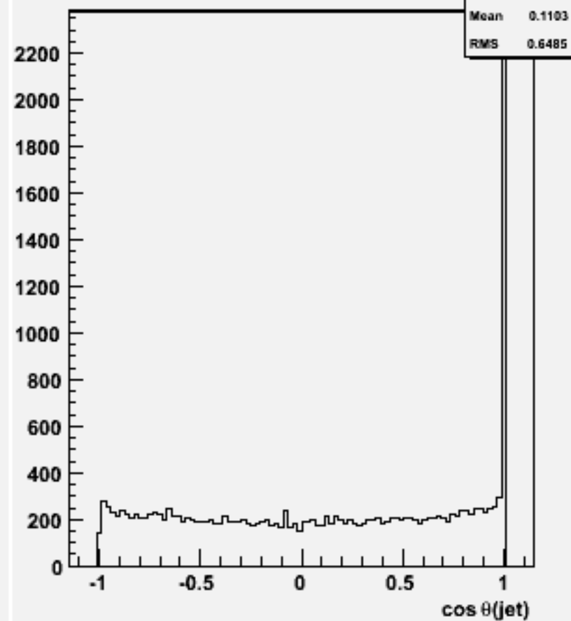
cos \theta for 2-jets :w104530 e3e3h_o
