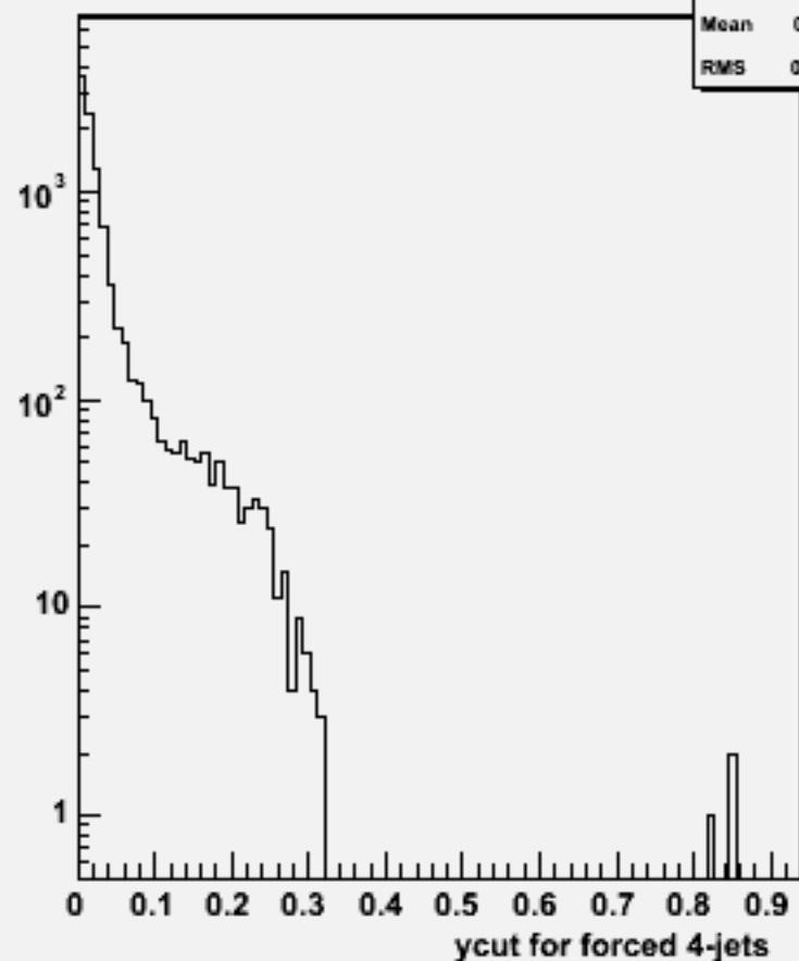
Ycut for 4-jets :w104530 e3e3h_o
