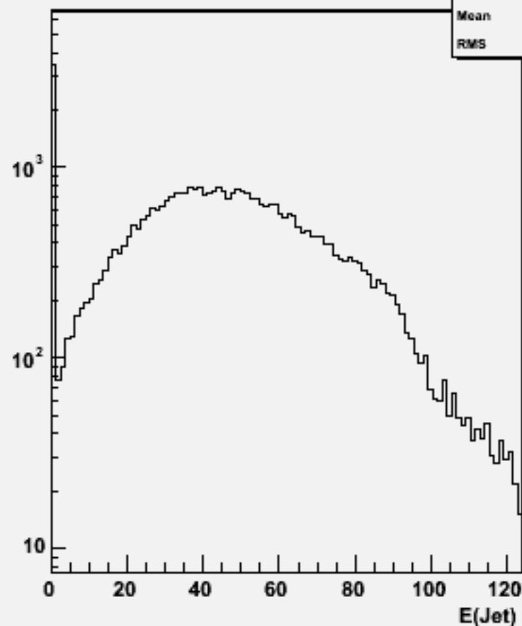
Jet energies(All jets)w104530 e3e3h_o
