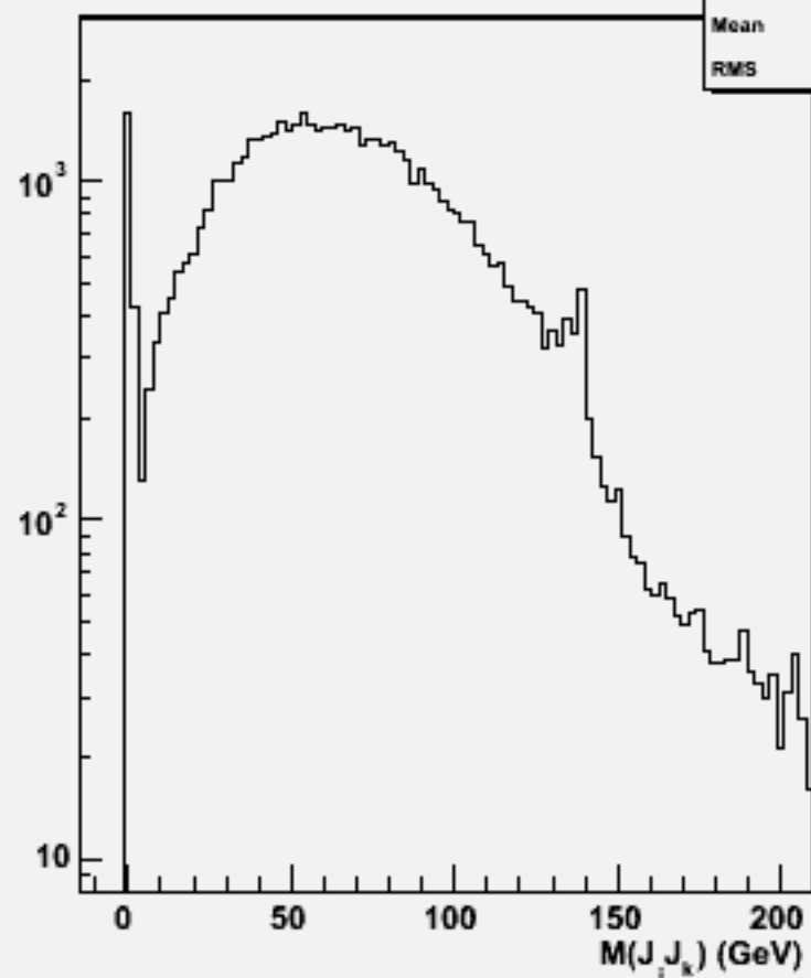
2jets mass(All comb)w104530 e3e3h_o
