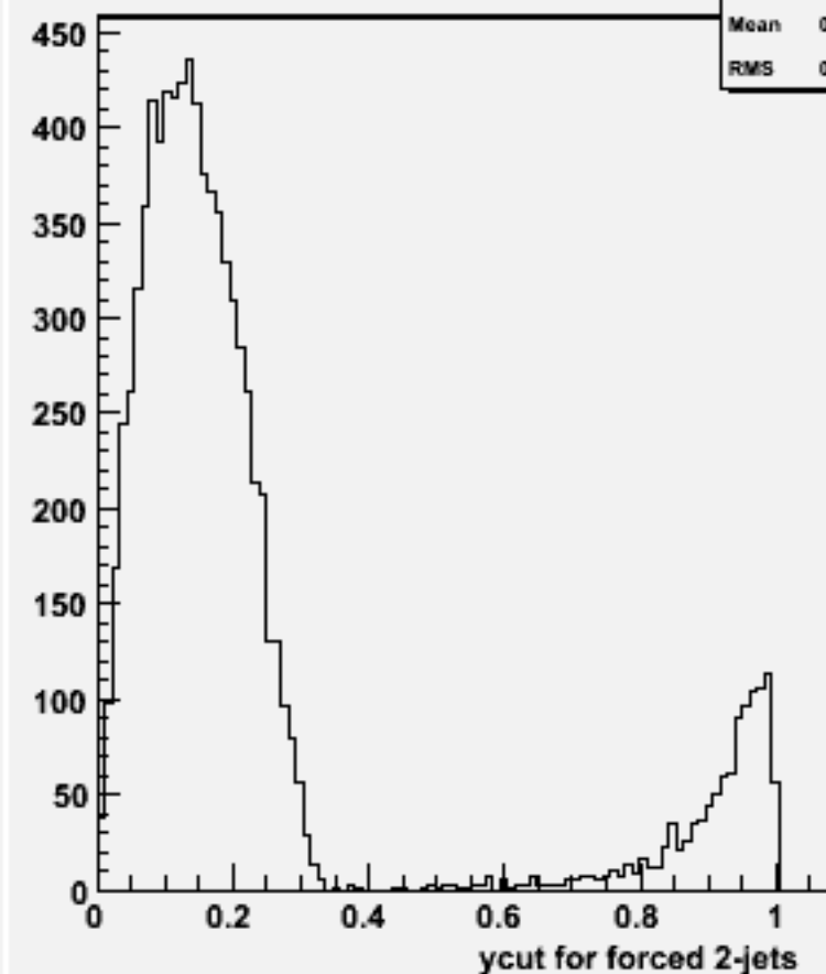
Ycut for 2-jets :w104530 e3e3h_o
