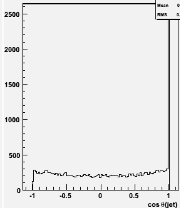
cos \theta for 2-jets :w104529 e3e3h_o
