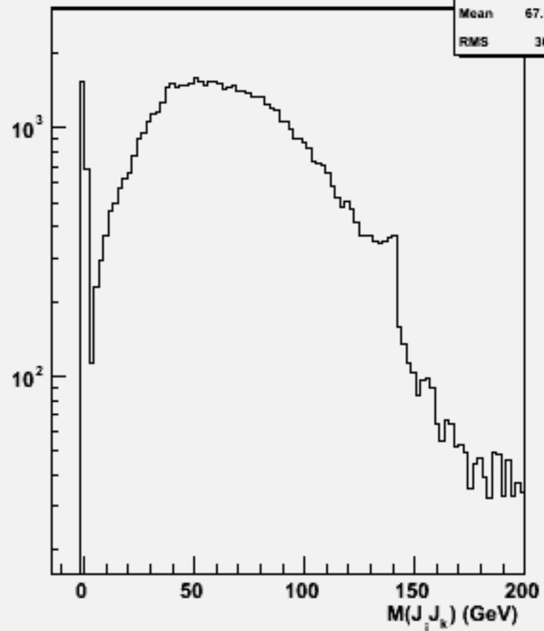
2jets mass(All comb)w104529 e3e3h_o
