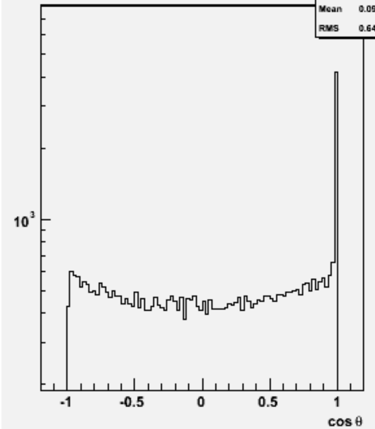
Jet cos \theta (All jets)w104529 e3e3h_o
