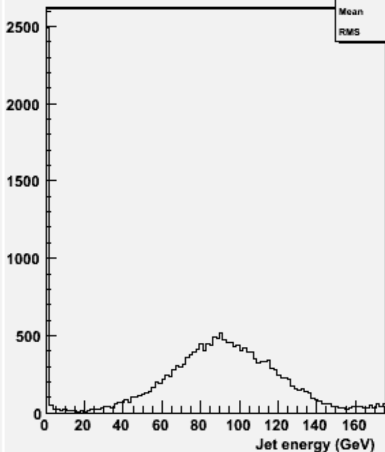
energy for 2-jets :w104529 e3e3h_o
